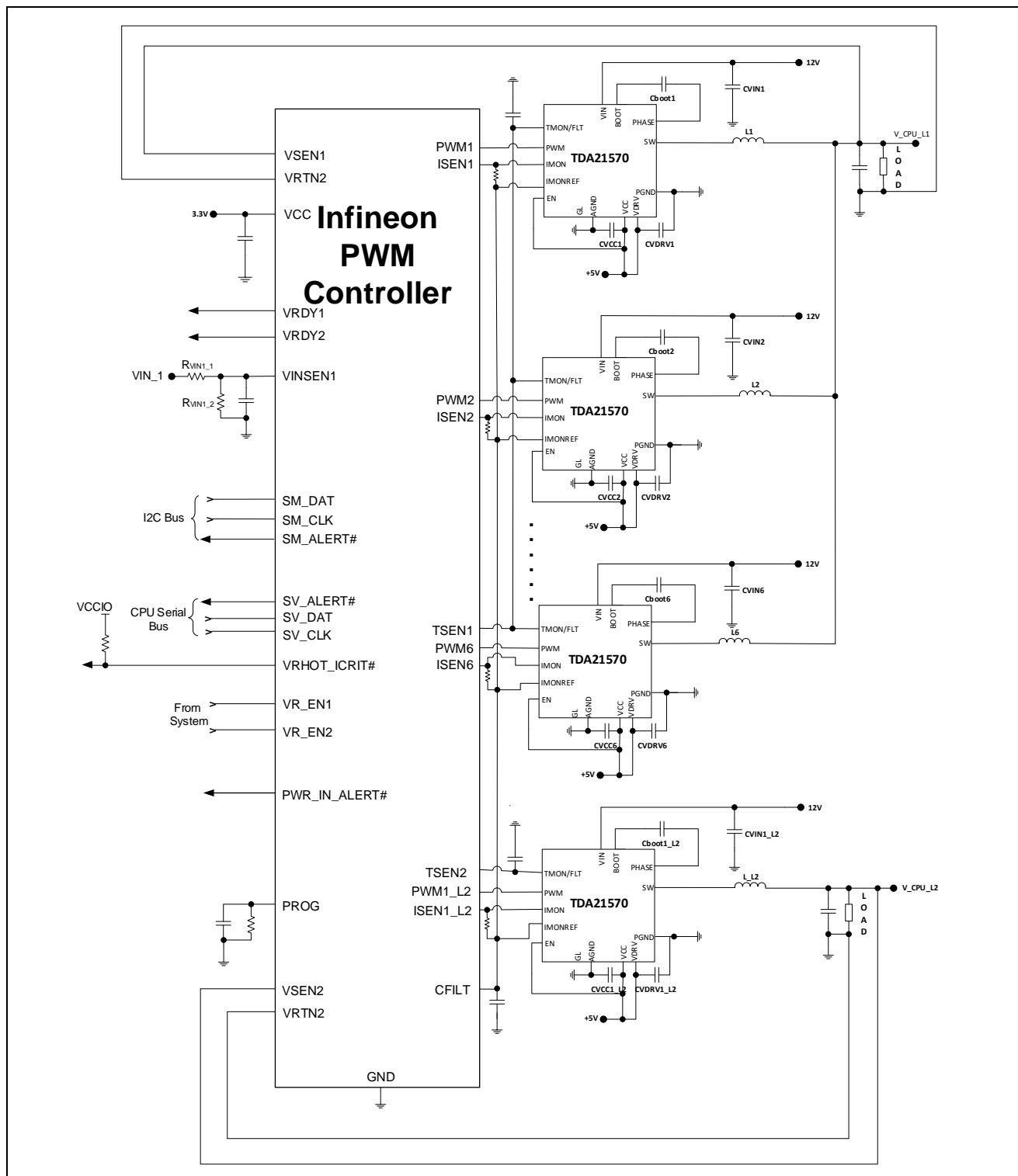
Figure 6 6+1 - Phase Voltage Regulator - Typical Application (simplified schematic)
