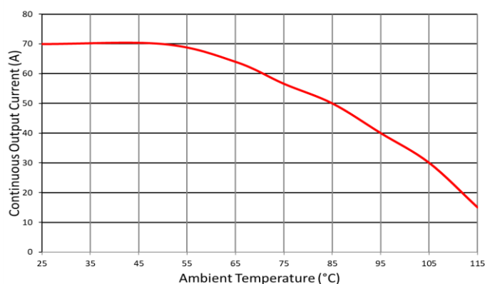
Figure 6 Thermal derating, T_{case} \leq 125\text{ °C}
