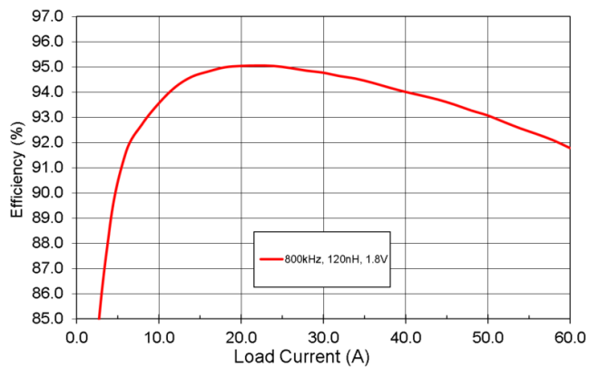
Figure 3 Powerstage Efficiency
