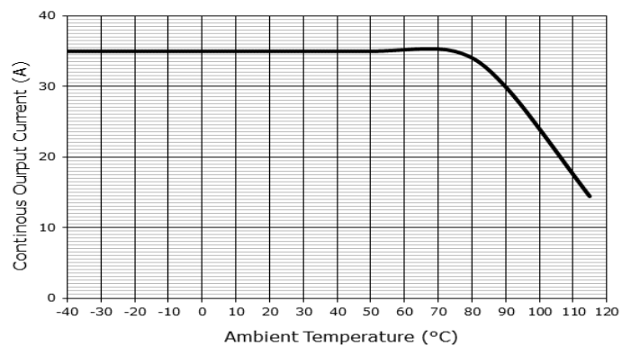
Figure 6 Thermal derating, T_{case} \leq 125\text{ °C}
