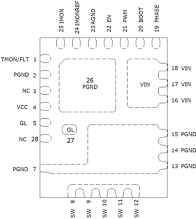
Figure 2 Pinout, Numbering and Name of Pins (transparent top view)
