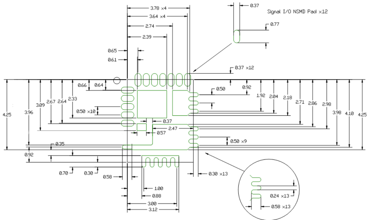
Figure 11 Solder Resist
