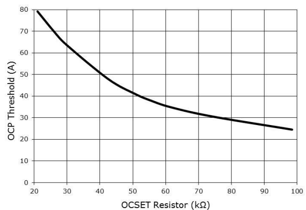
Figure 8 Programmable OCP Threshold
