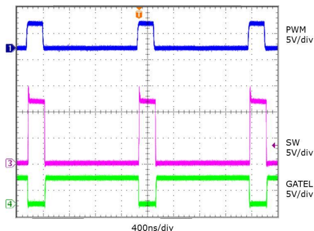
Figure 9 Switching Waveform at 0 A
