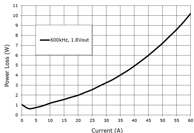
Figure 7 Power Stage Loss
