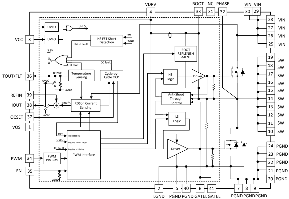
Figure 3 Block Diagram
