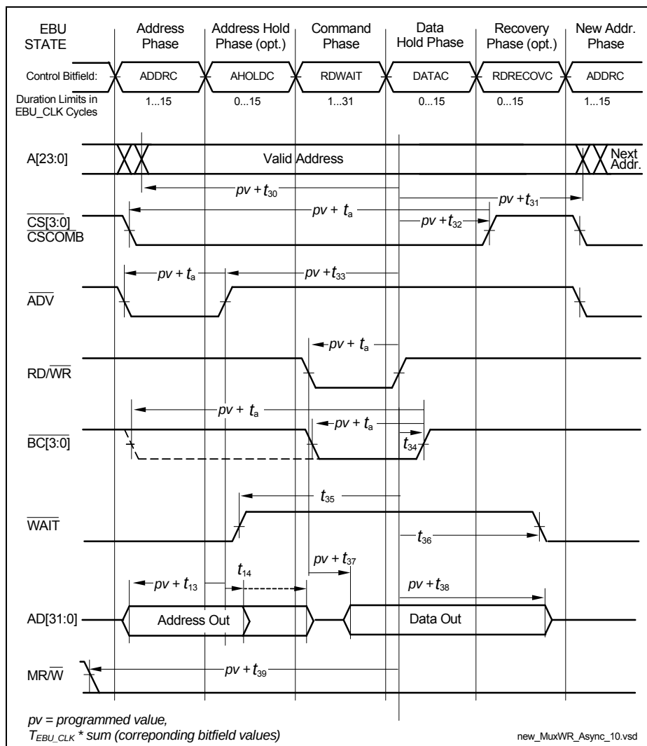
Figure 27 Multiplexed Write Access
