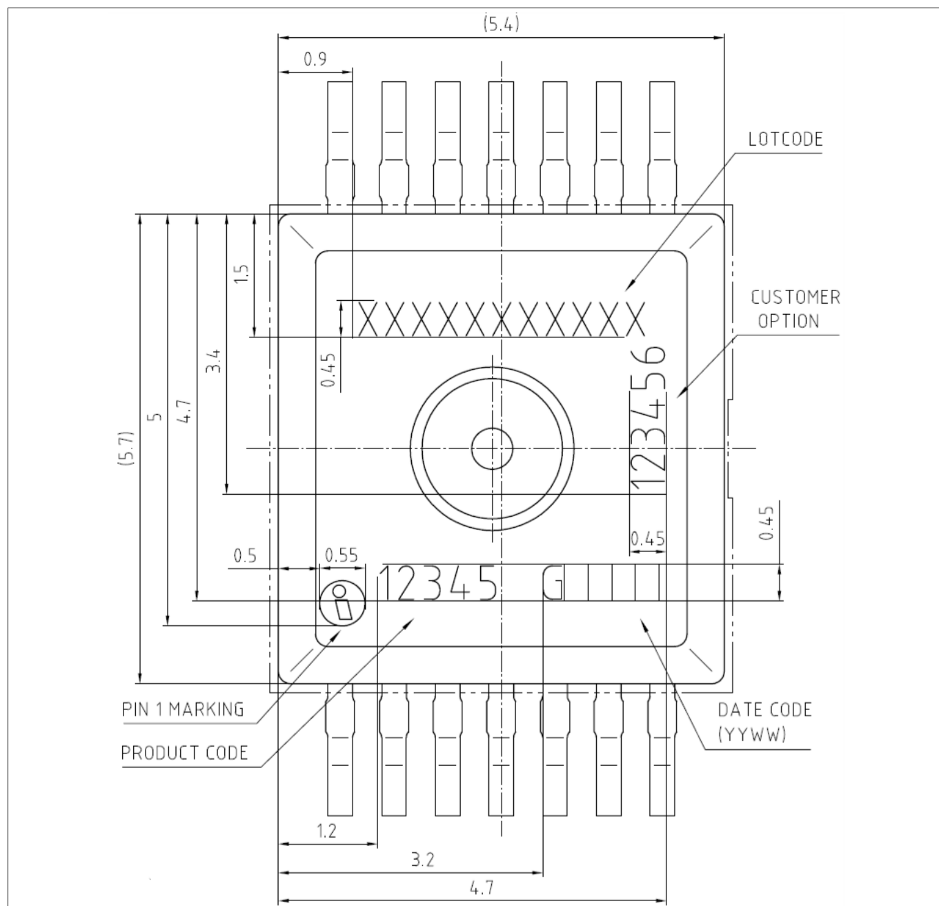
Figure 8-2 Marking information
