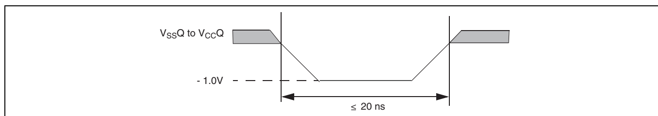
Figure 17 Maximum negative overshoot waveform
