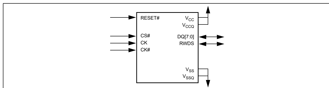
Figure 5 HYPERRAM™ interface [4]
