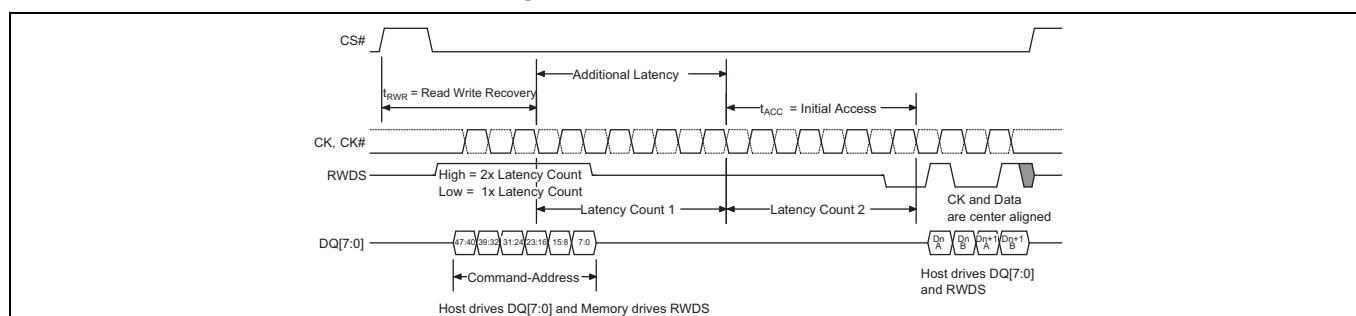
Figure 10 Write transaction with initial latency [32-38]
