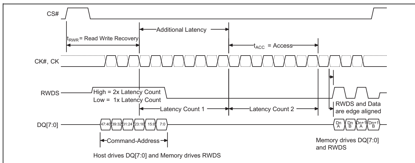
Figure 9 Read transaction with initial latency [23-31]
