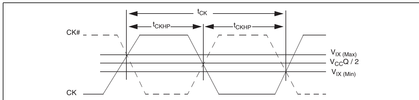
Figure 26 Clock characteristics [65]
