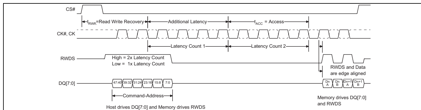
Figure 2 Read transaction
