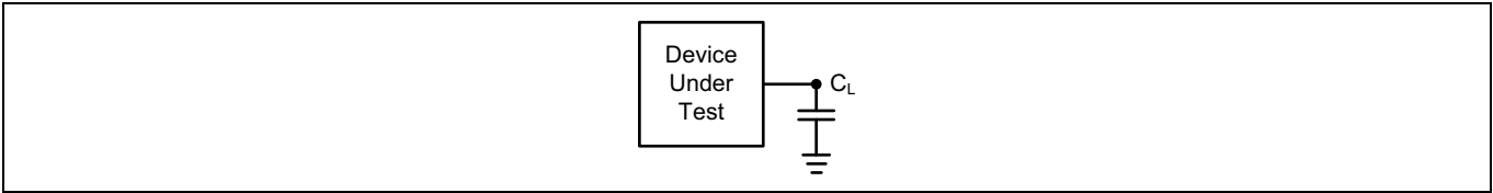
Figure 24 Test setup
