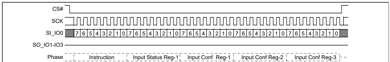
Figure 53 Write Register (WRR) command sequence
