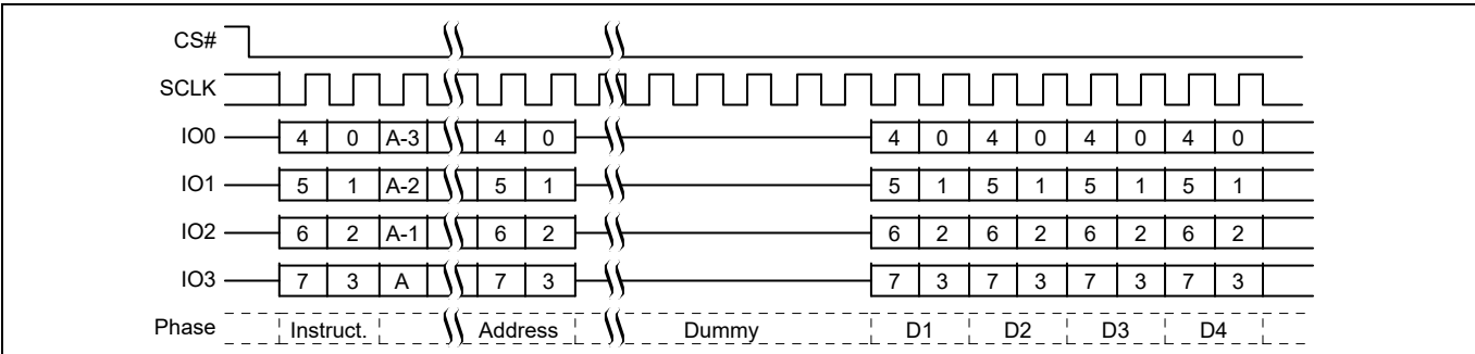
Figure 46 RSFDP QPI mode command sequence
