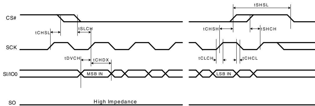
Figure 9.4 Input Timing
