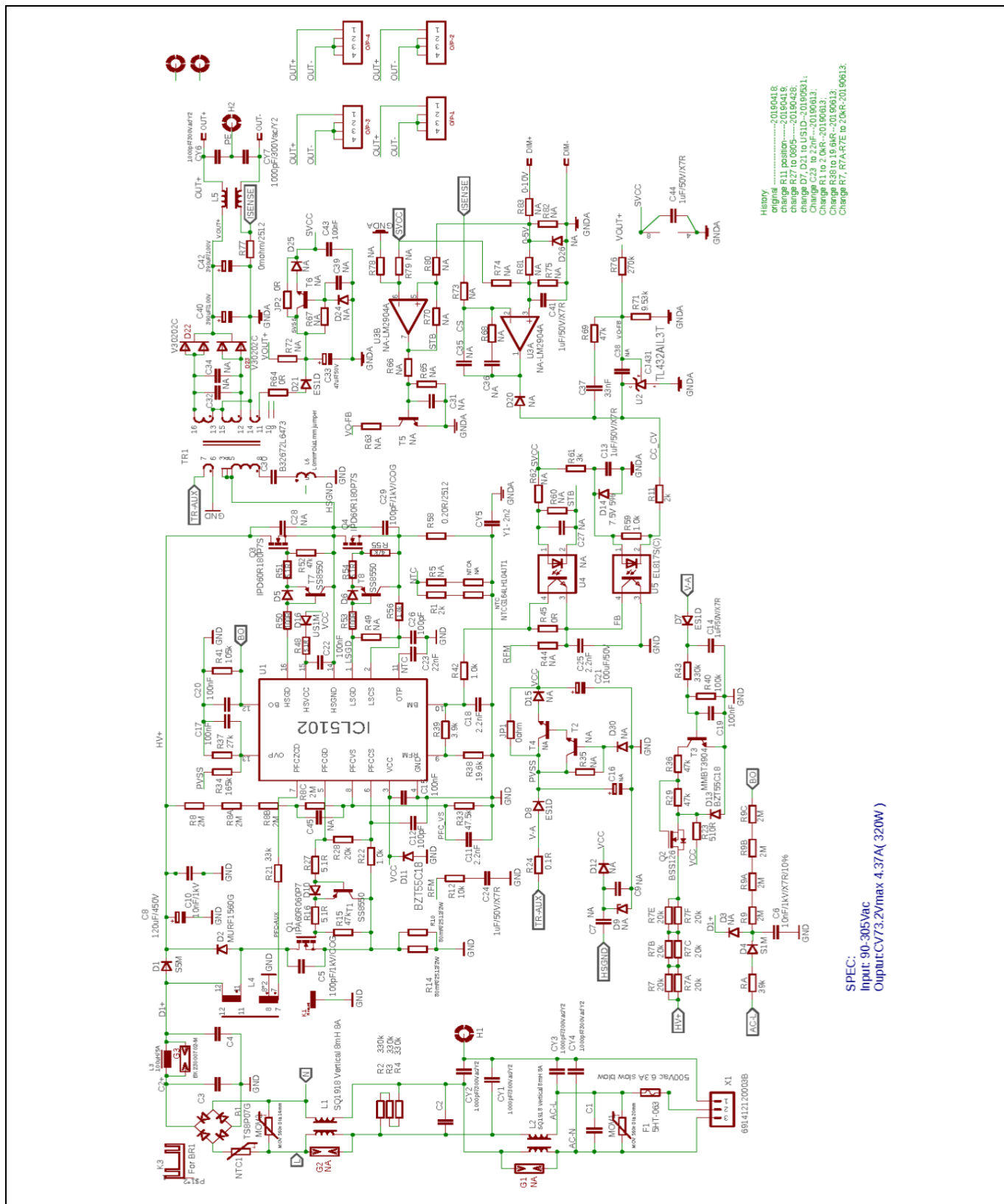
Figure 5 Schematic of the ICL5102 320 W reference design
