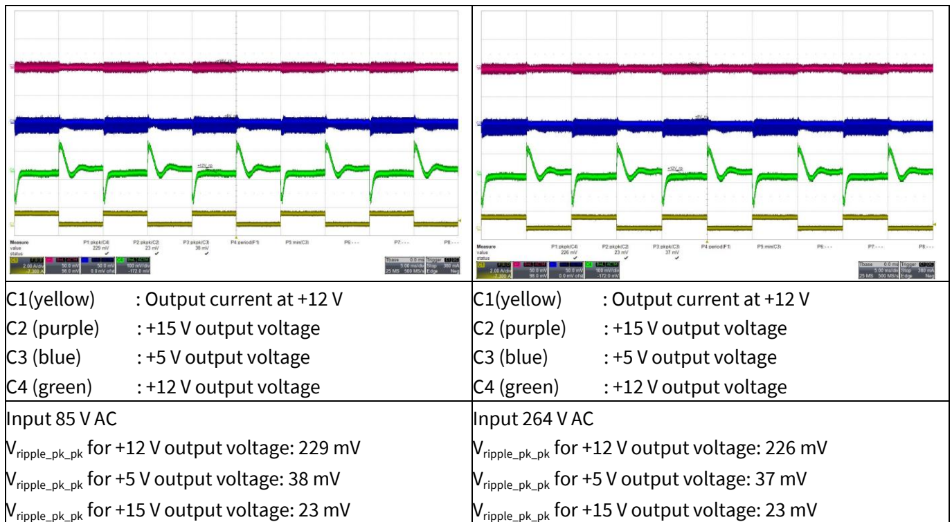
Figure 23 Load-transient response (+12 V output load change from 10 percent to 100 percent at 0.4 A/μs slew rate, 100 Hz, +15 V output and +5 V output load are fixed at full load; 20 MHz bandwidth and 10 μF electrolytic capacitor in parallel with 0.1 μF ceramic capacitor)
