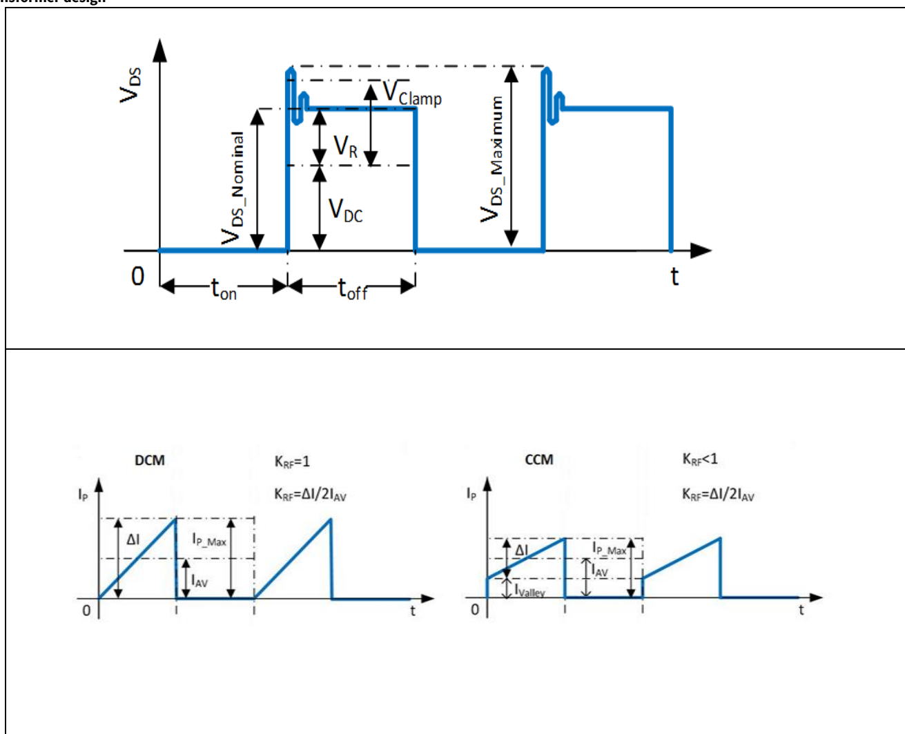
Figure 31 Drain voltage and current waveform
