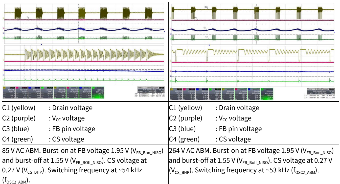
Figure 27 During ABM
