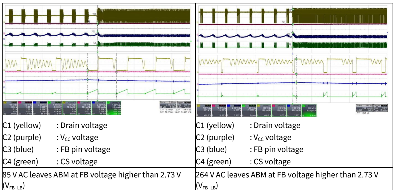
Figure 28 Leaving ABM
