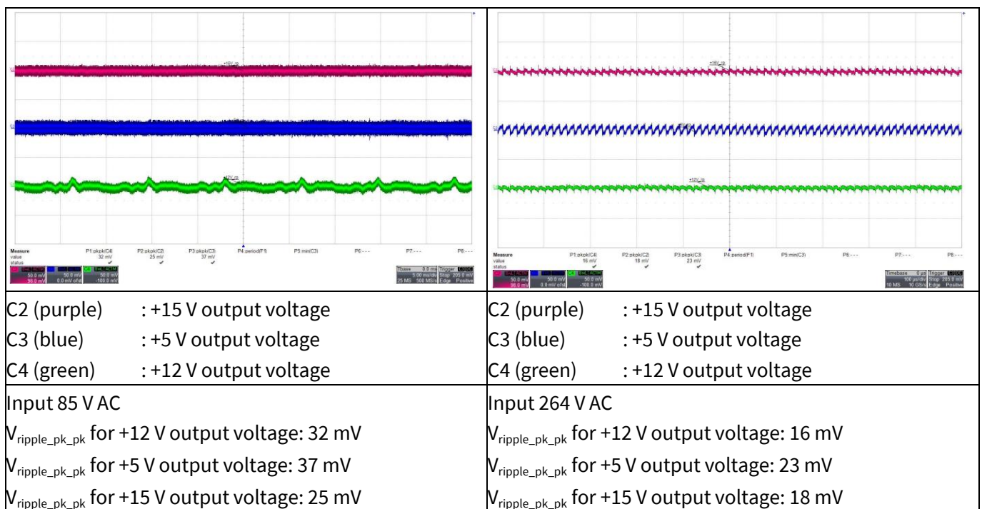
Figure 24 Output ripple voltage at full load. Probe terminals are decoupled with 10 μF electrolytic and 0.1 μF ceramic capacitors. Oscilloscope is bandwidth filter limited to 20 MHz
