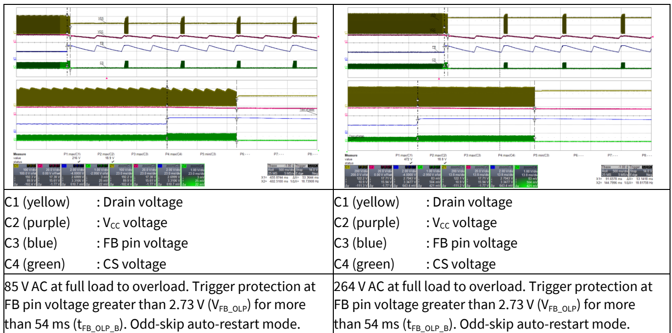
Figure 30 Overload protection
