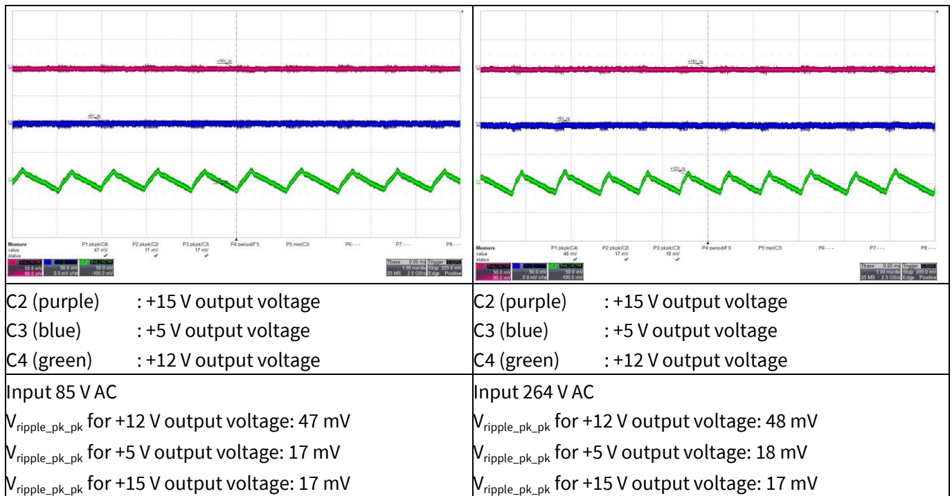
Figure 25 Output ripple voltage at minimum load. Probe terminals are decoupled with 10 \mu\text{F} electrolytic and 0.1 \mu\text{F} ceramic capacitors. Oscilloscope is bandwidth filter limited to 20 MHz
