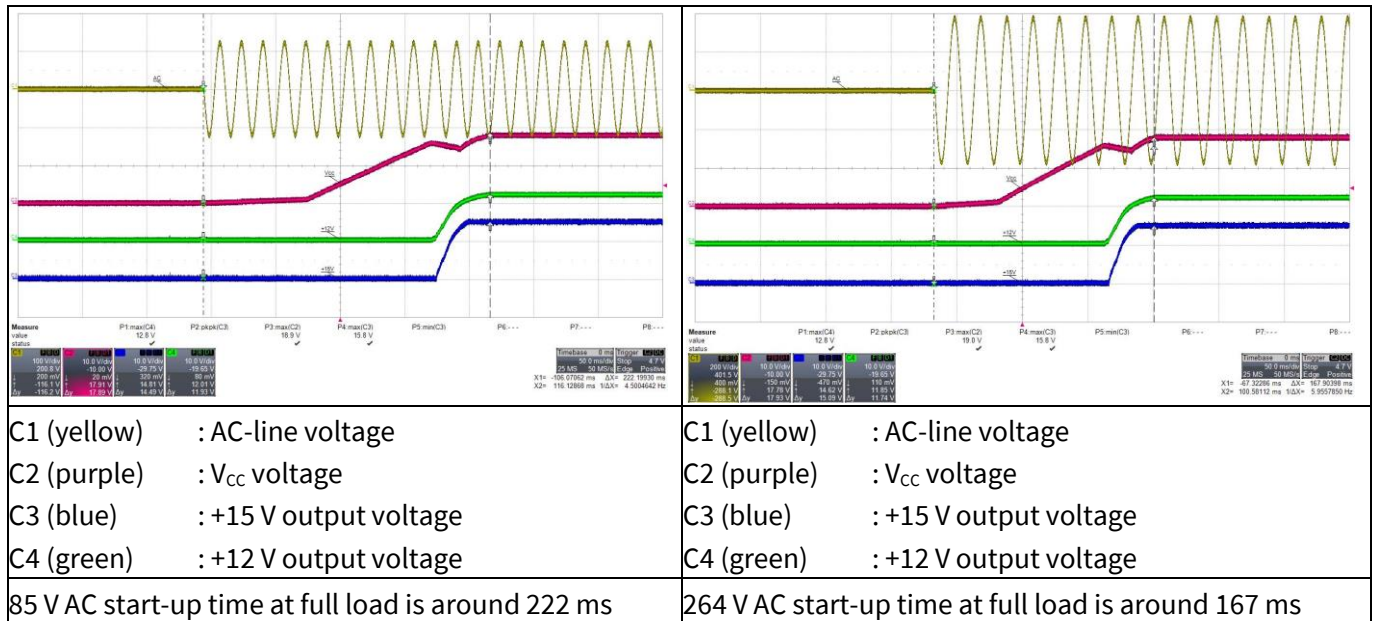
Figure 19 Start-up
