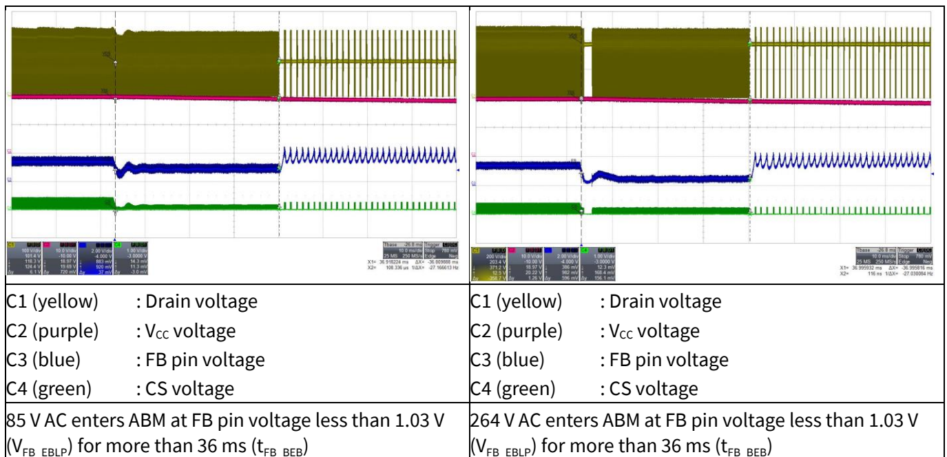
Figure 26 Entering ABM
