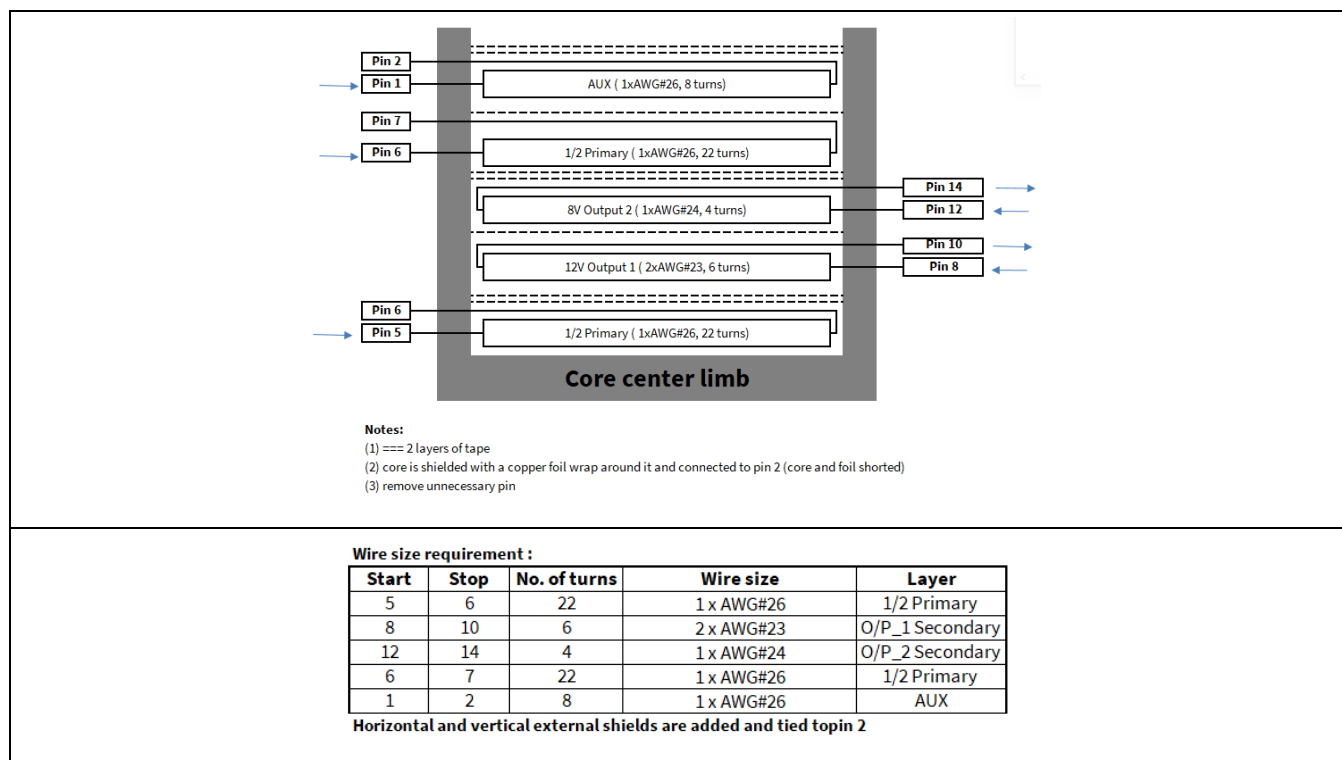
Figure 8 Transformer structure
