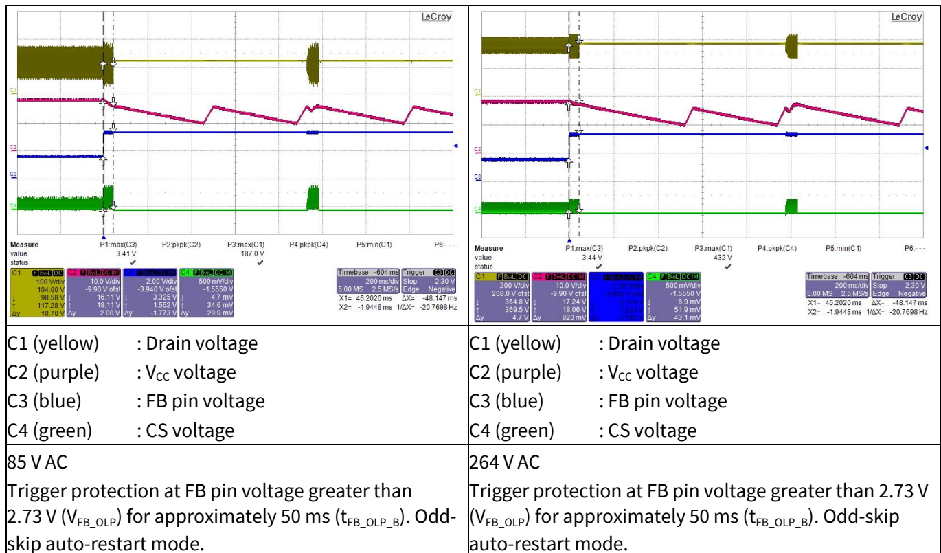
Figure 30 Overload protection
