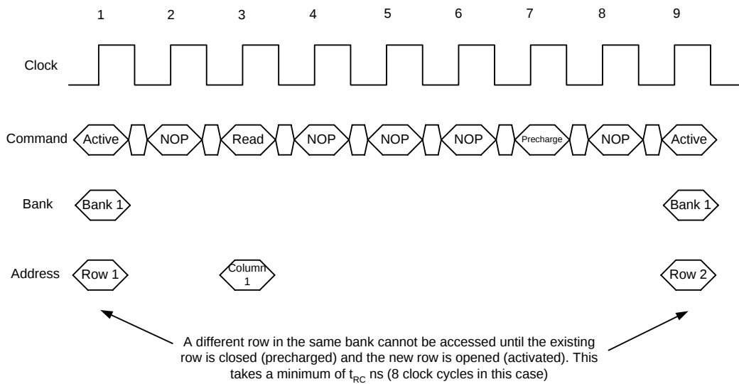
Figure 2. The t_{RC} limitation
