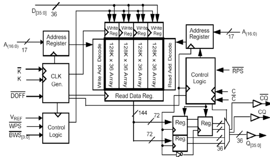
Fig. 1 Block diagram of a QDR-II burst-of-4 device
