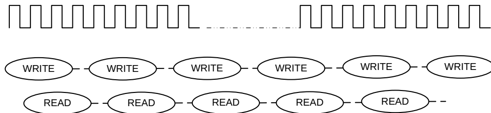
Figure 6. READ/WRITE patterns
