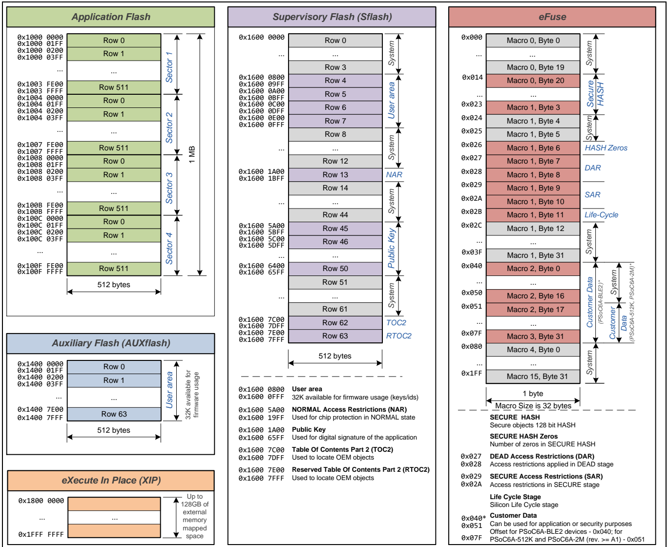
Figure 2 Nonvolatile subsystem
