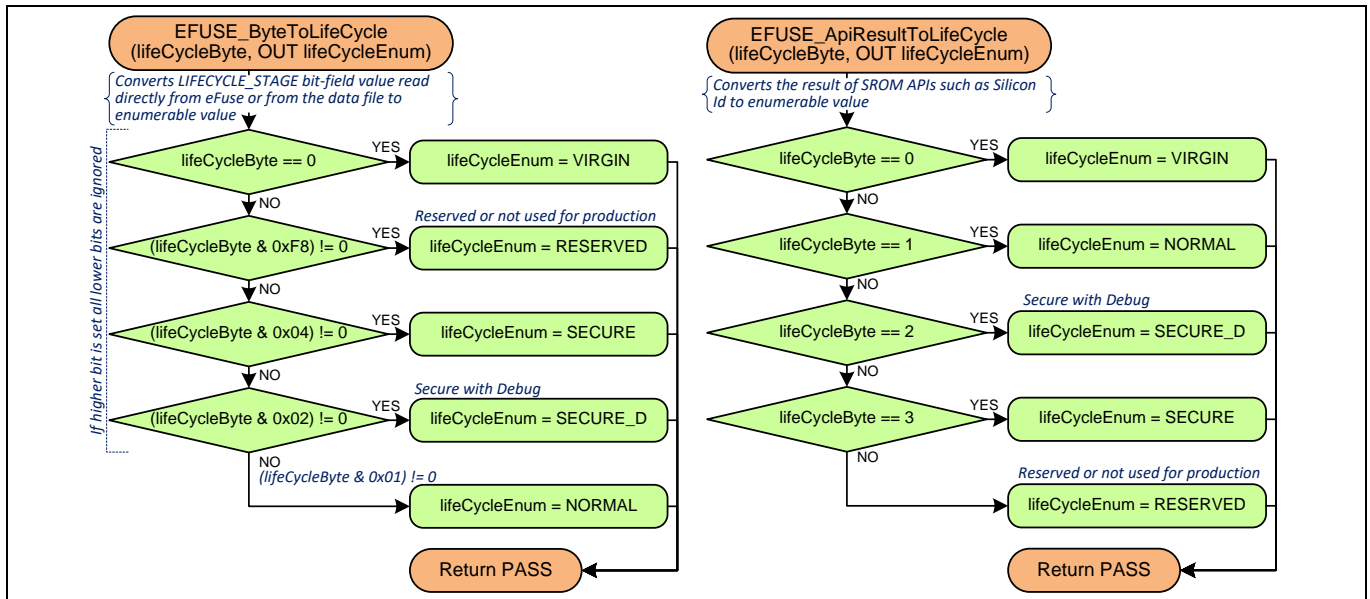
Figure 19 Life cycle parsing subroutines
