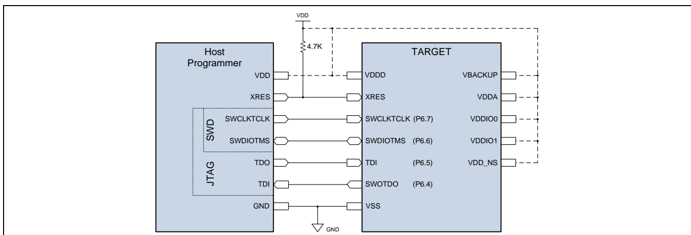
Figure 8 Connection Schematic of Programmer
