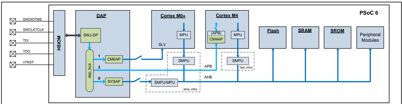
Figure 5 Top-level silicon architecture
