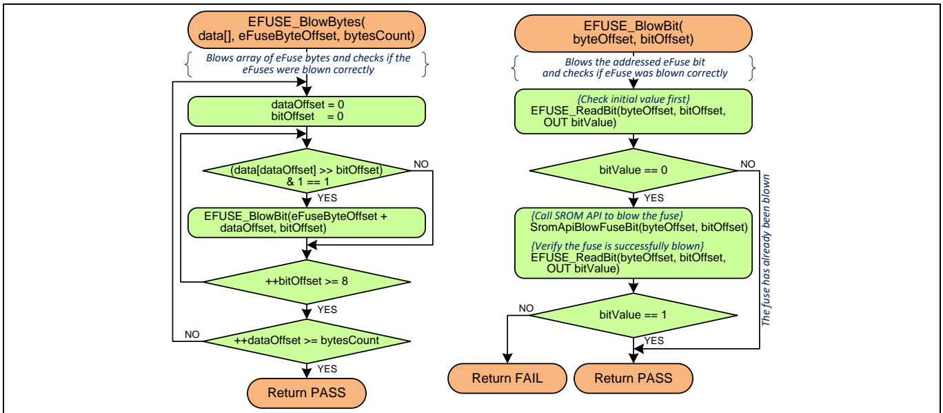
Figure 21 eFuse Read/Write subroutines
