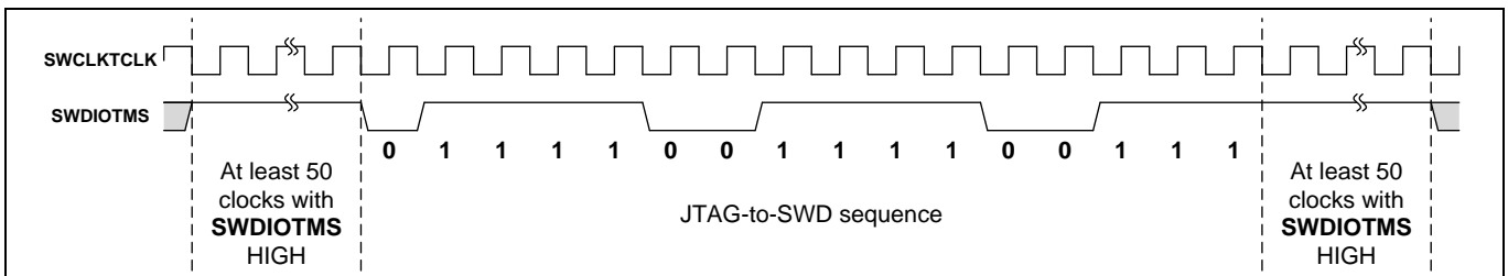
Figure 6 JTAG-to-SWD sequence timing
