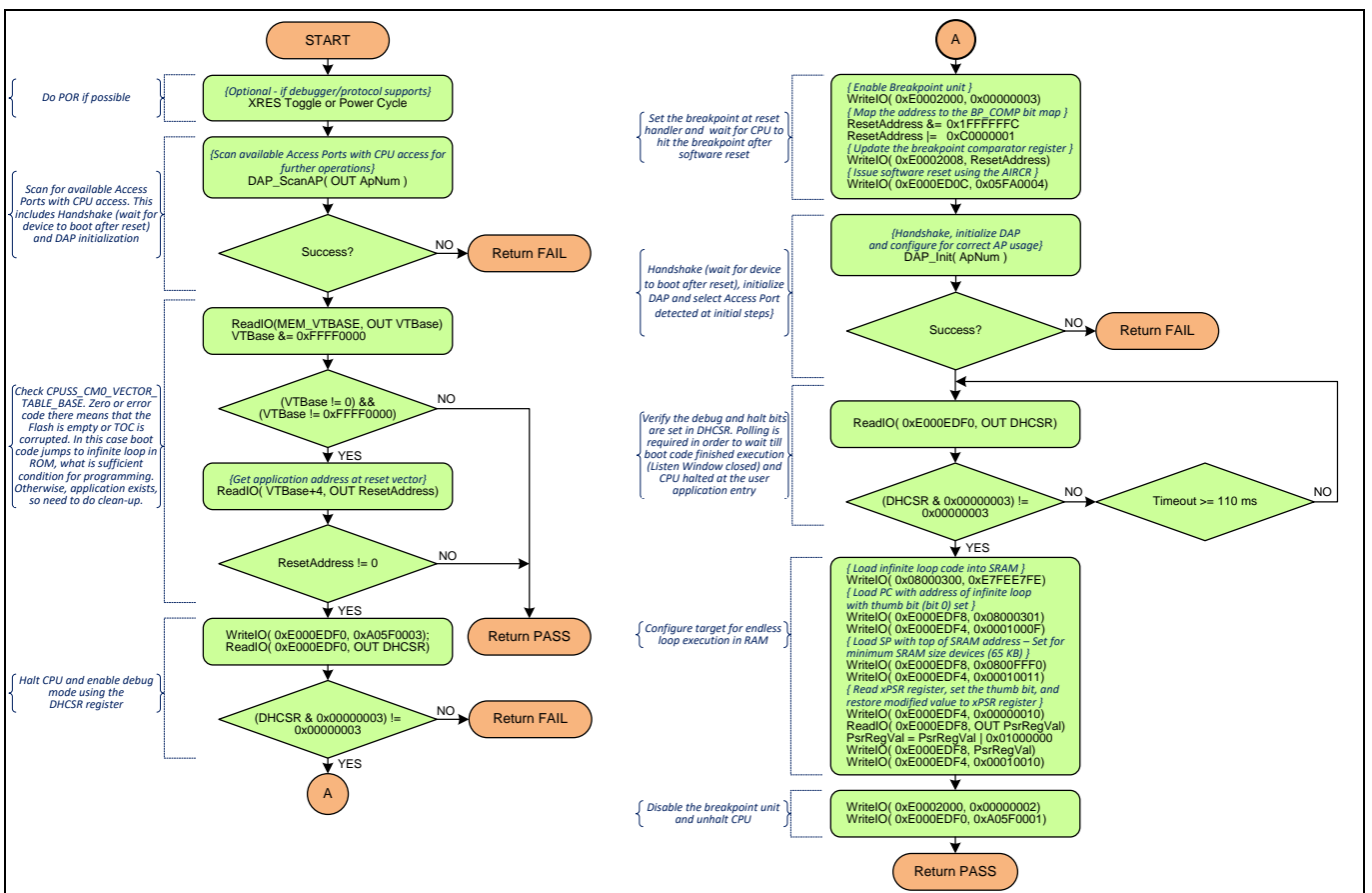
Figure 13 Flowchart of the acquire chip step (alternate method)
