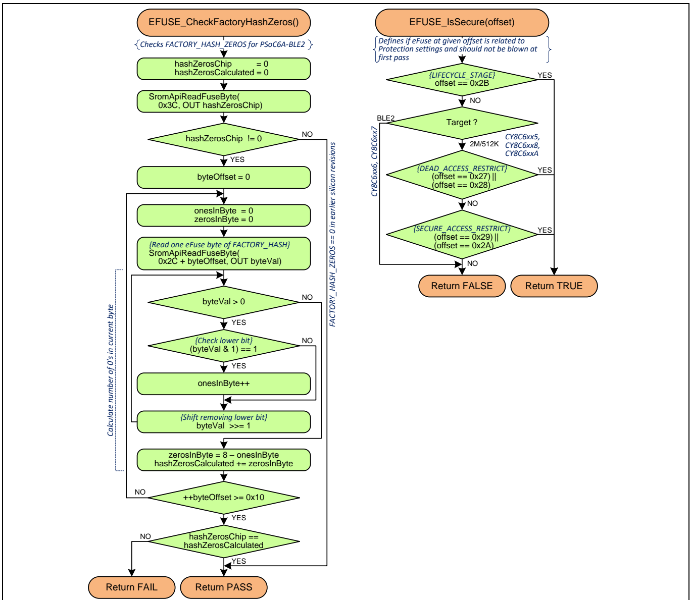
Figure 18 eFuse verification subroutines
