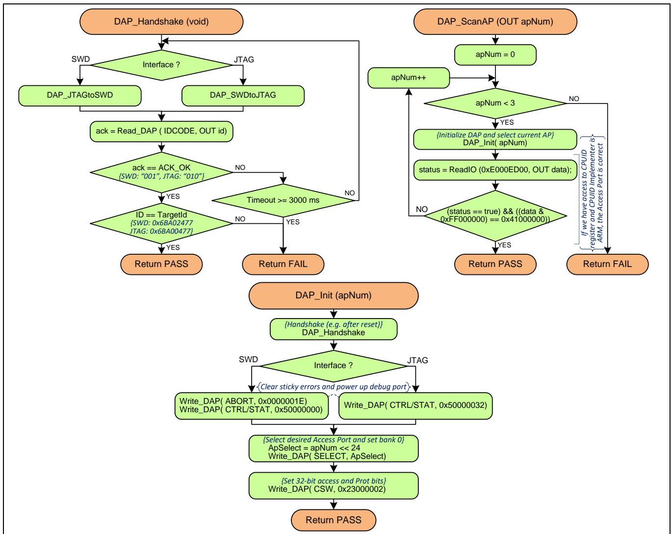
Figure 10 DAP initialization subroutines
