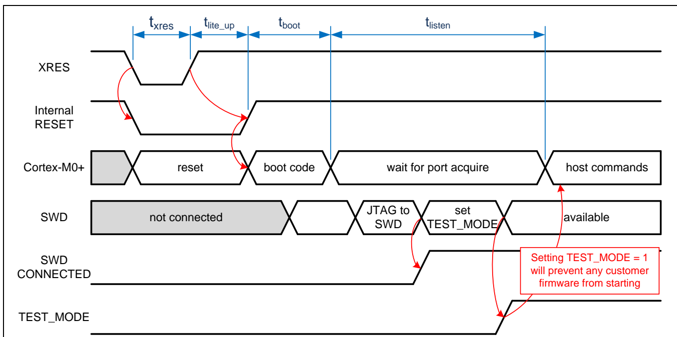
Figure 11 Timing diagram for entering test mode
