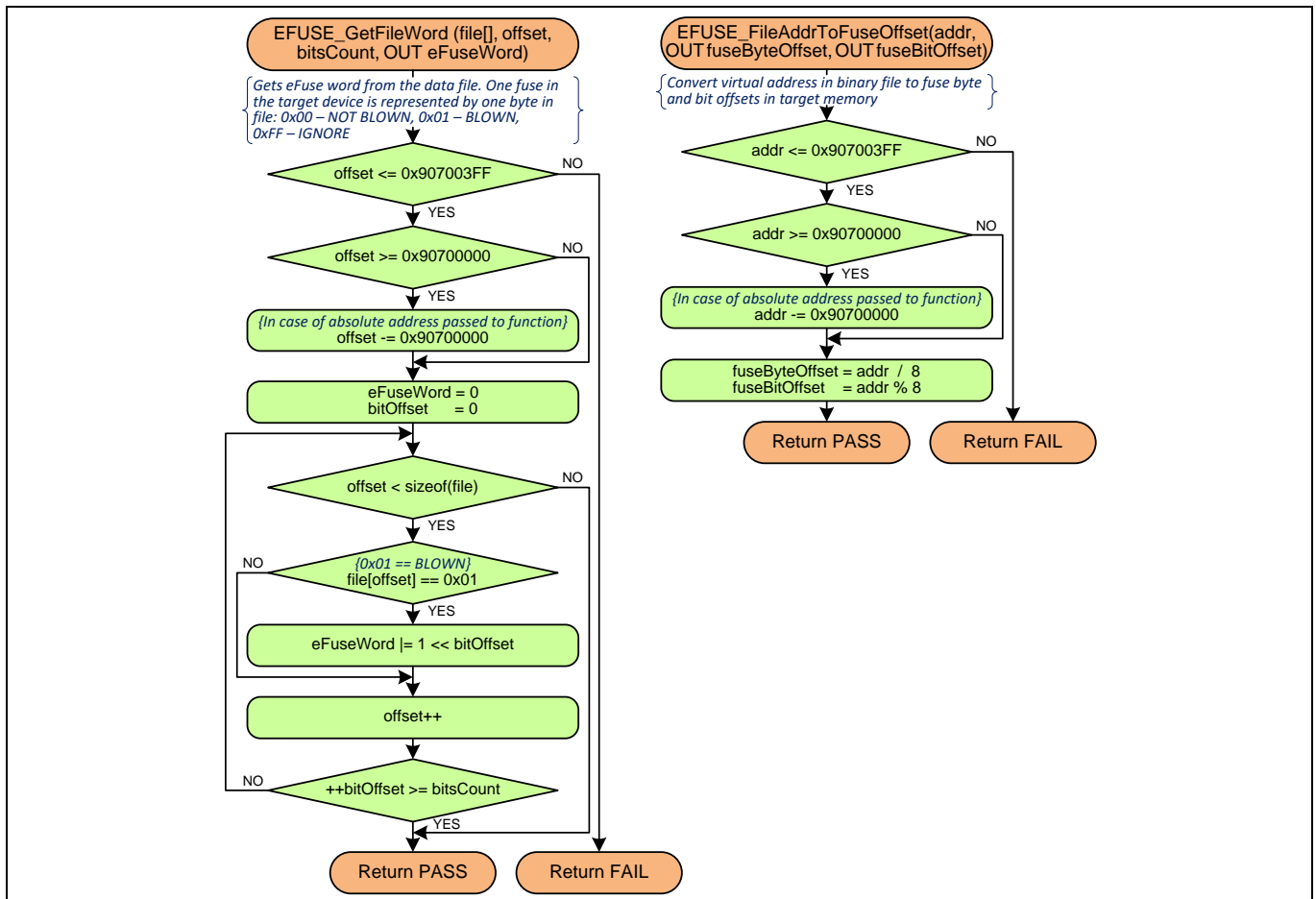
Figure 20 eFuse file parsing subroutines
