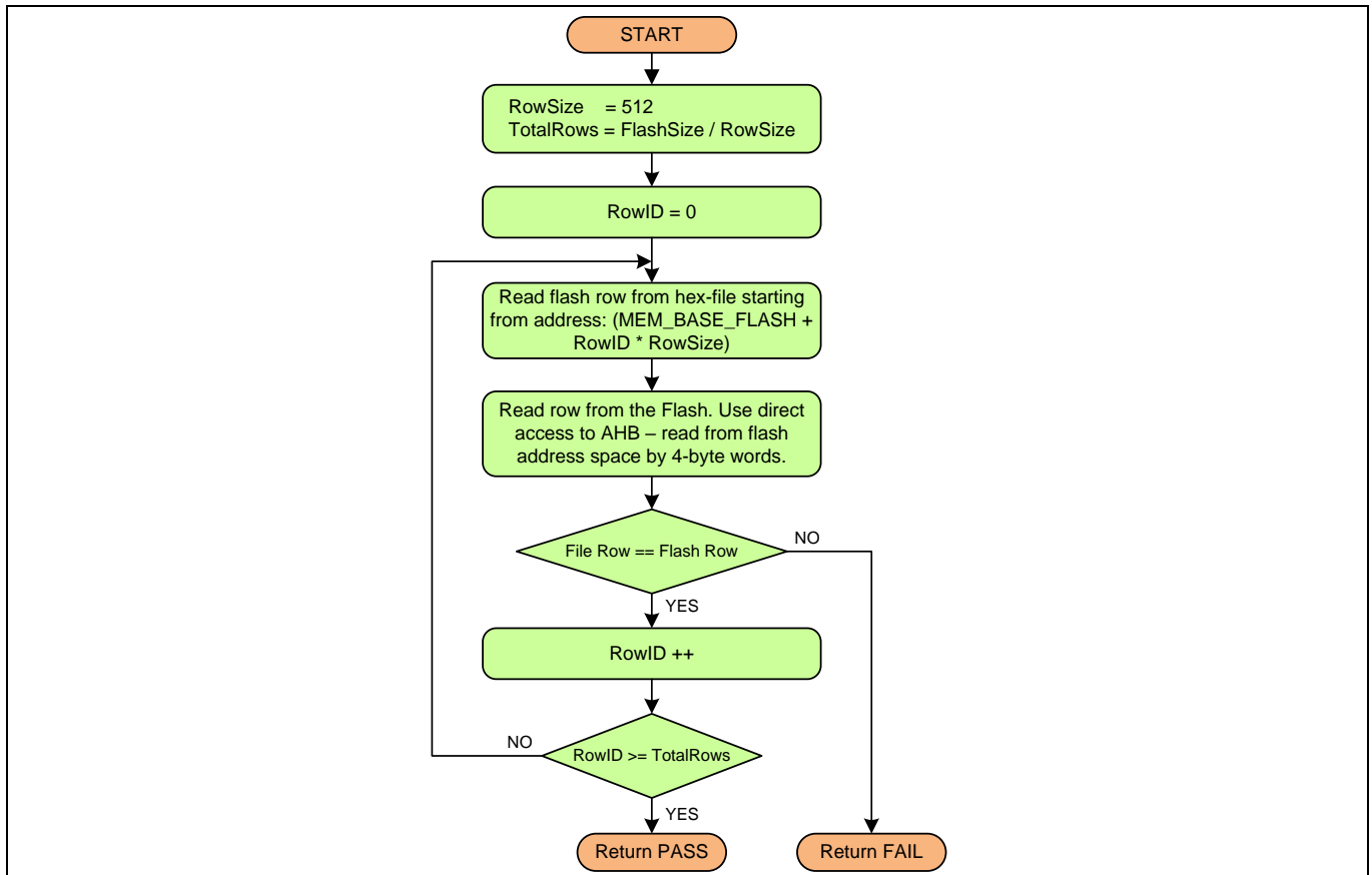
Figure 15 Flowchart of the “verify application flash” step
