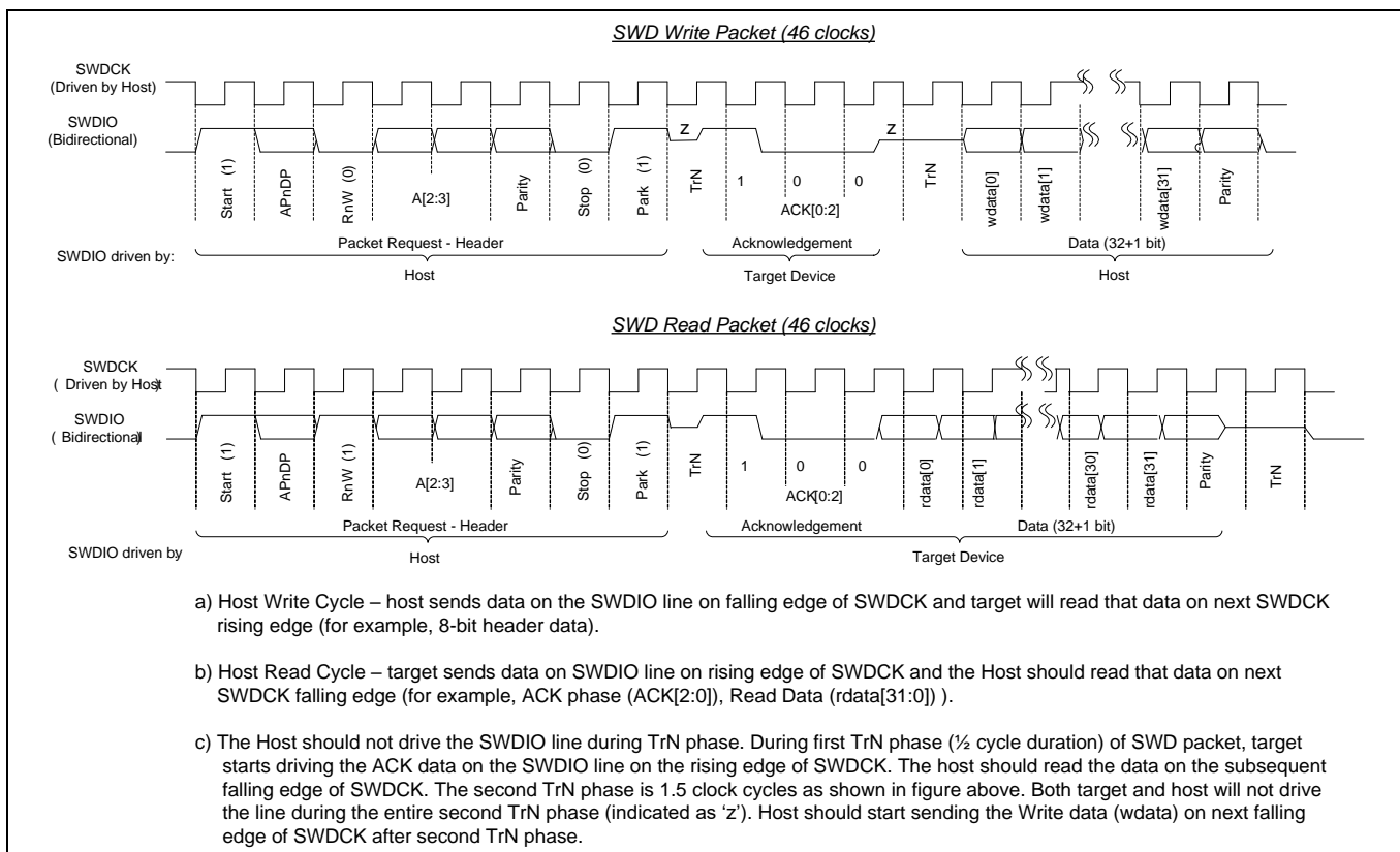
Figure 23 Write and Read SWD packet timing diagrams
