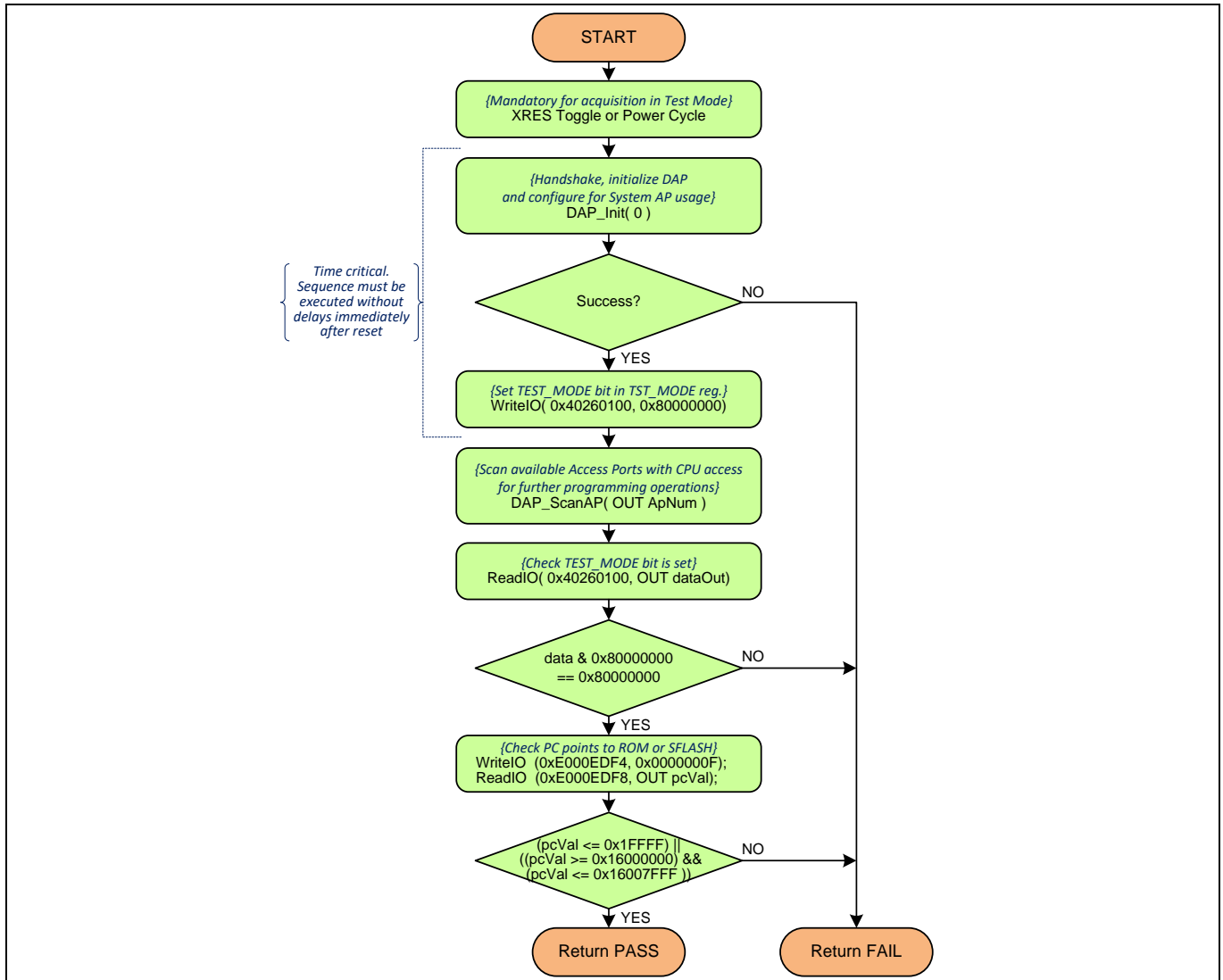
Figure 12 Flowchart of the acquire chip step
