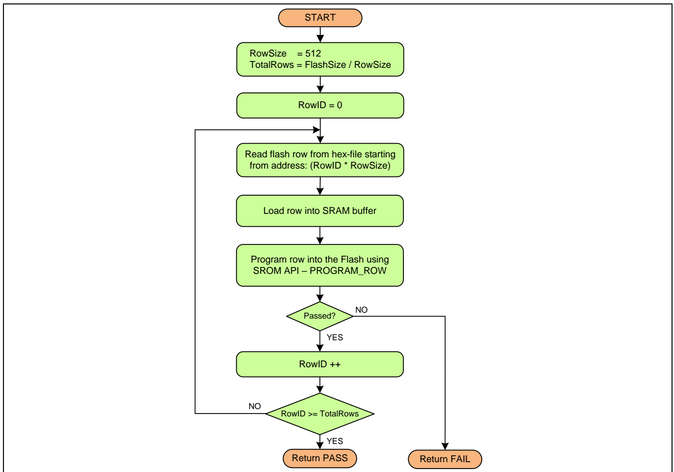
Figure 14 Flowchart of the “program application flash” step
