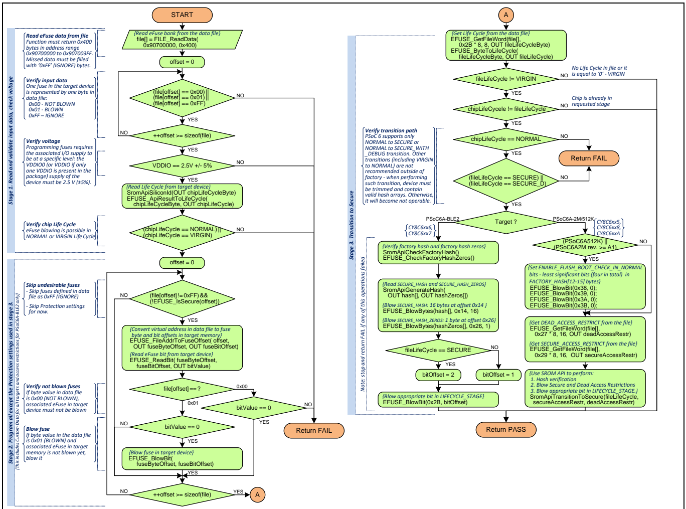
Figure 17 Flowchart of the “program eFuse” step
