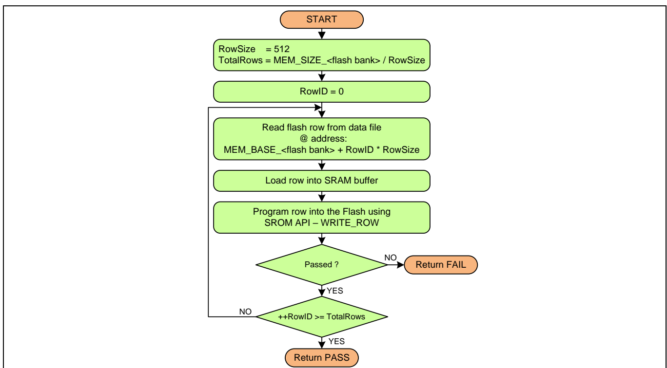
Figure 16 Flowchart of "program and verify AUXflash" step
