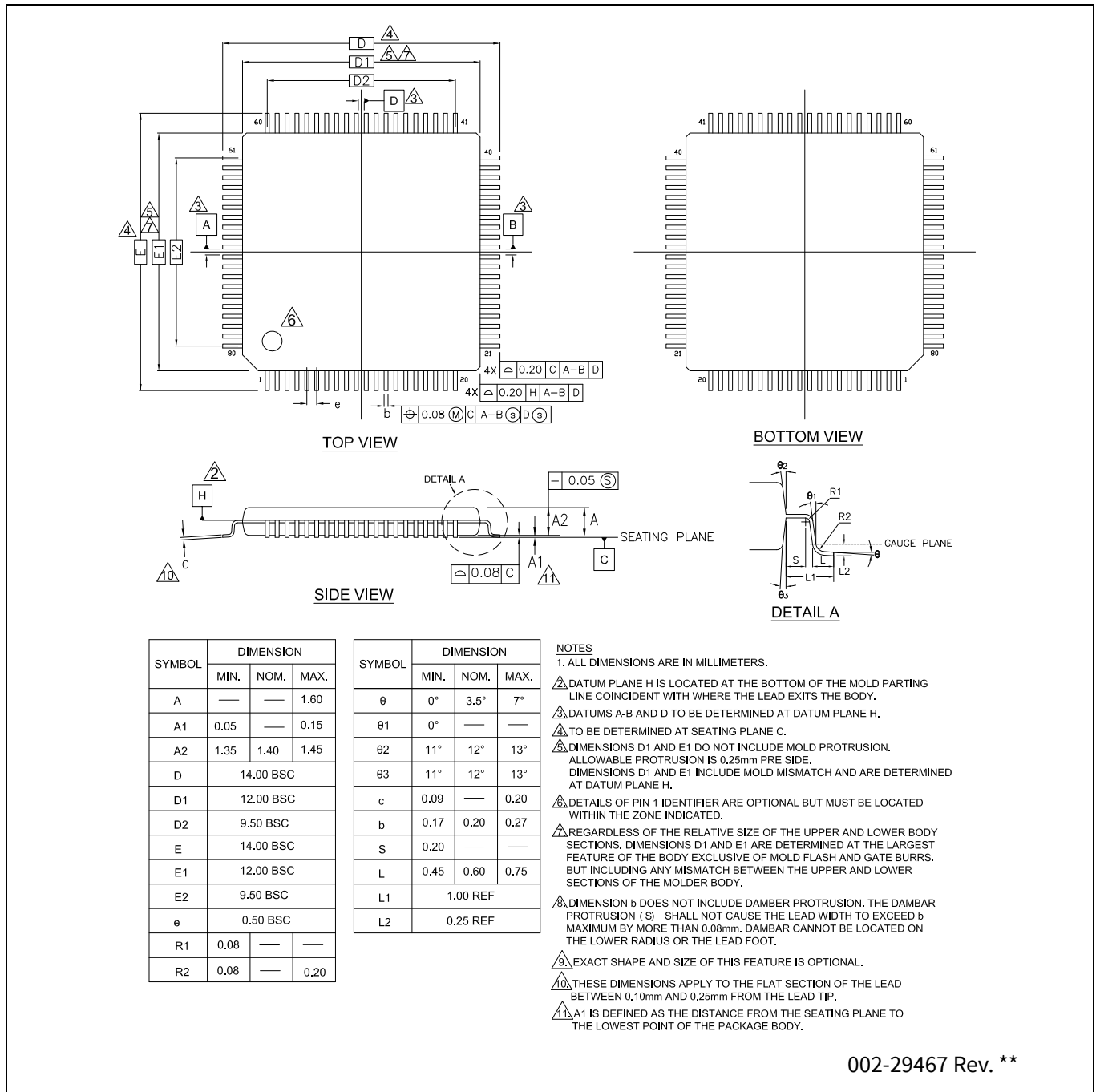
Figure 20 80-pin TQFP ((12.0 × 12.0 × 1.6 mm) AZ80A) package outline (PG-TQFP-80)
