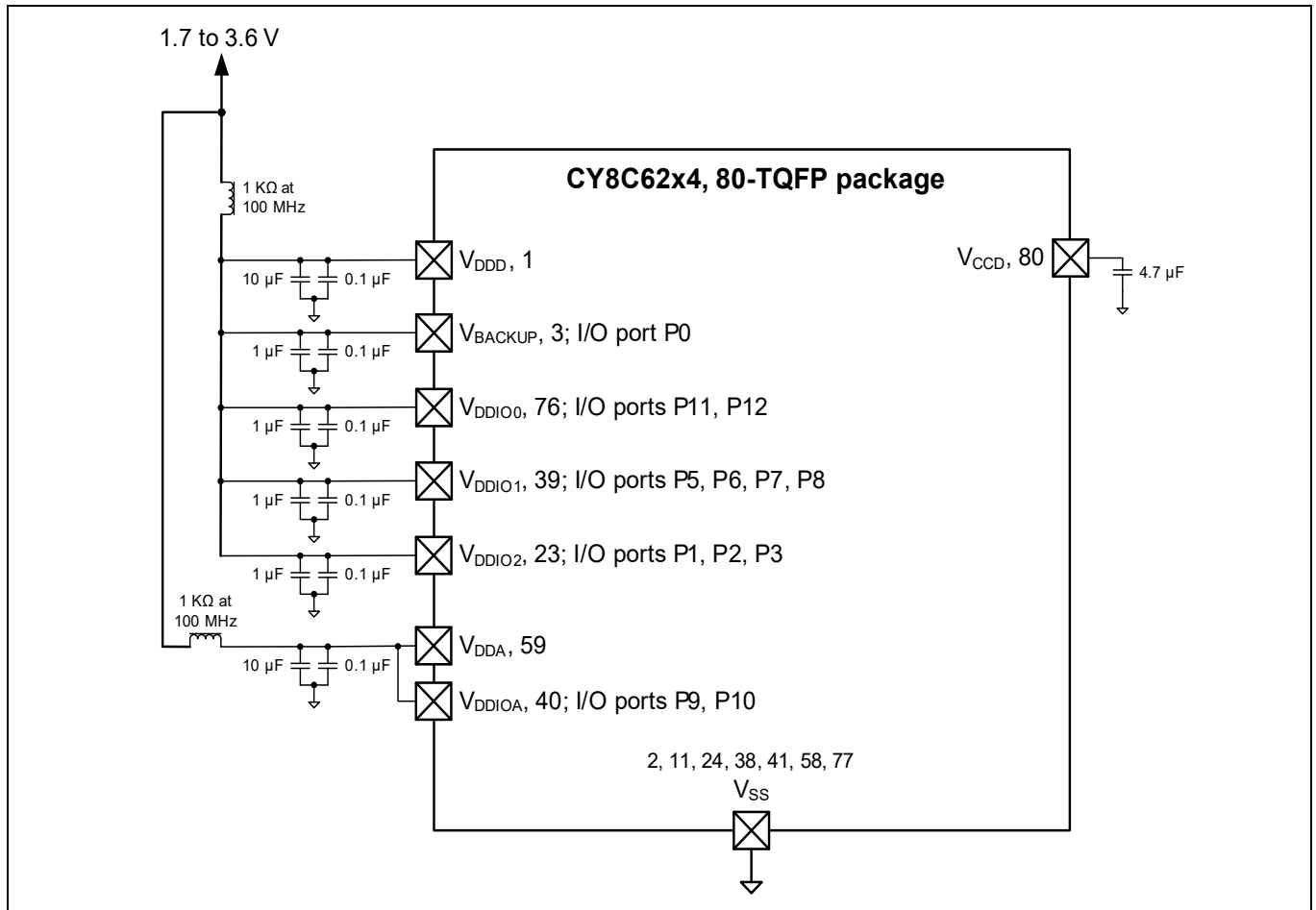
Figure 12 80-pin TQFP Power Connection diagram
