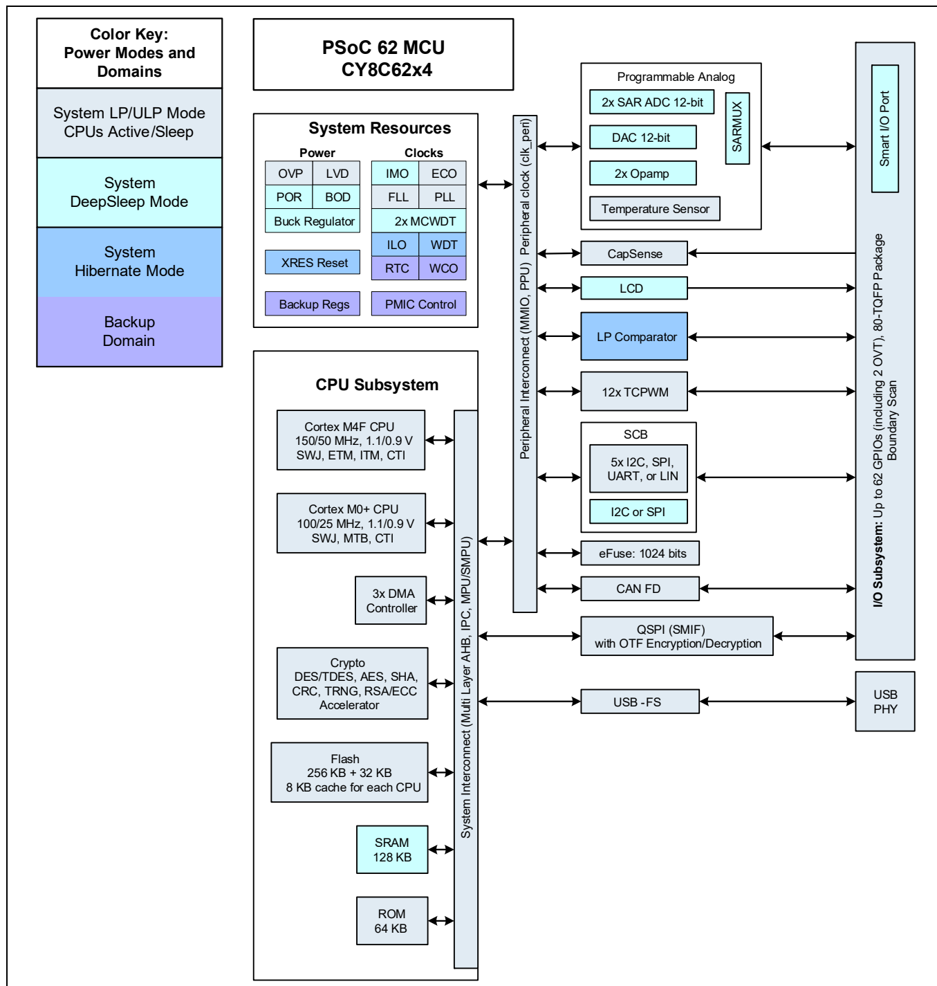
Figure 2 Block diagram
