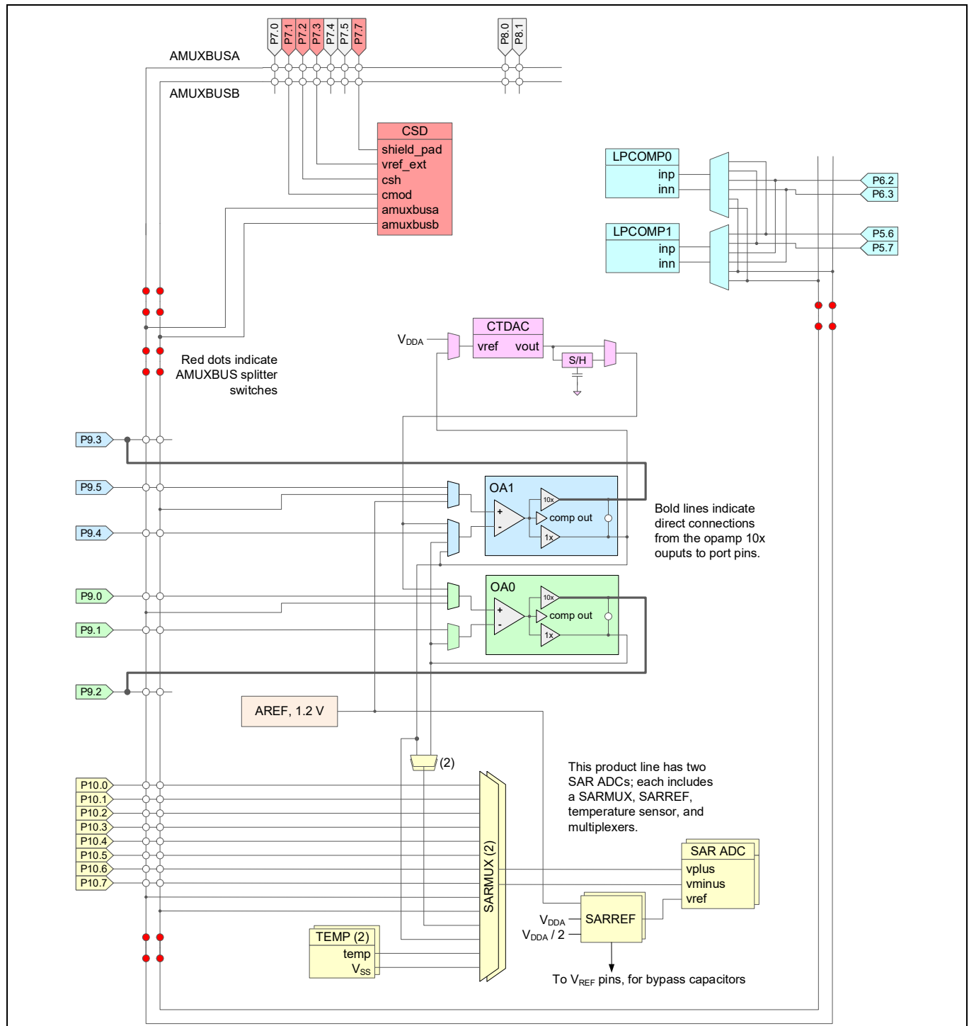
Figure 6 Analog subsystem
