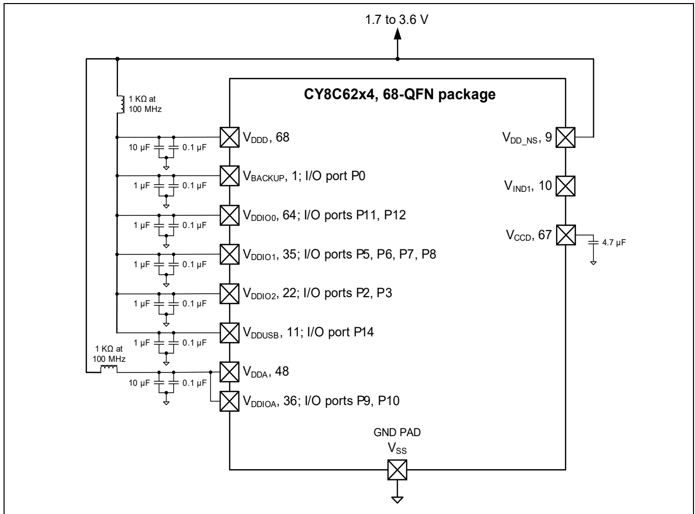
Figure 14 68-pin QFN (No Buck) Power Connection diagram
