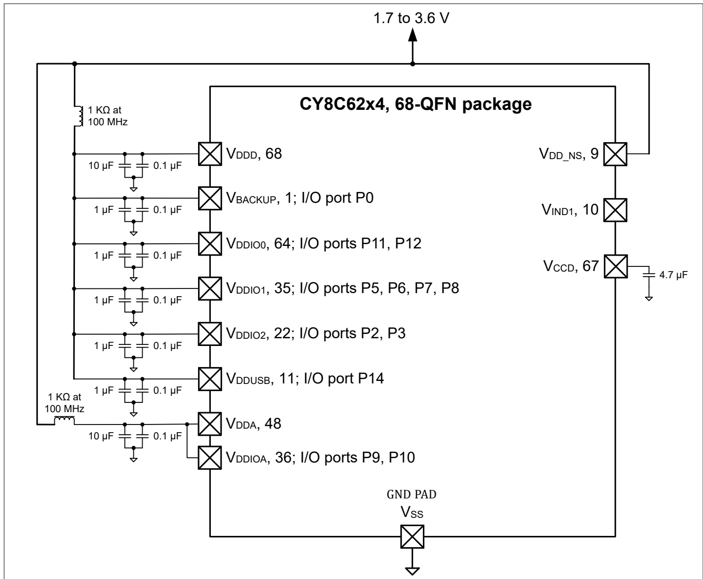
Figure 14 68-pin QFN (No Buck) Power Connection diagram
