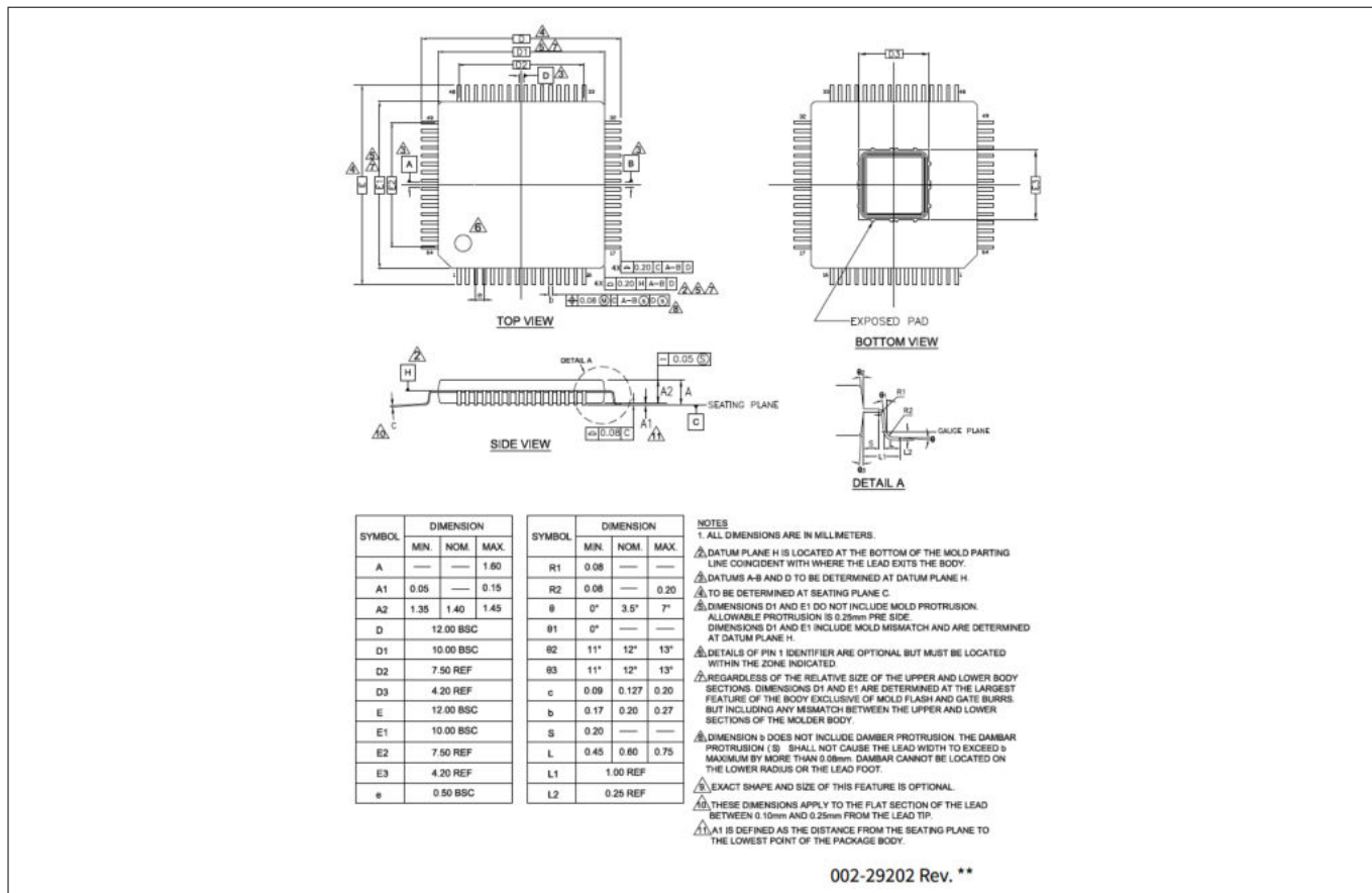
Figure 21 64-pin E-TQFP ((10.0 × 10.0 × 1.6 mm) AE64A 4.2 × 4.2 mm E-Pad package outline (PG-TQFP-64)
