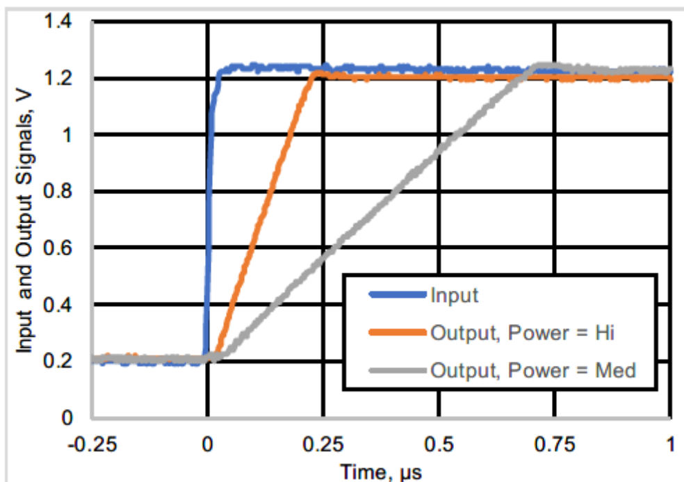
Figure 17 Opamp step response, rising
