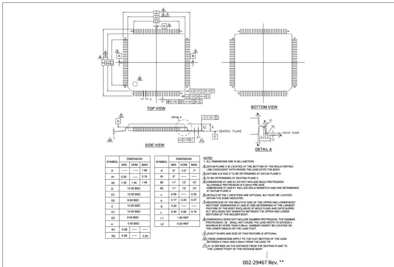
Figure 20 80-pin TQFP ((12.0 x 12.0 x 1.6 mm) AZ80A) package outline (PG-TQFP-80)
