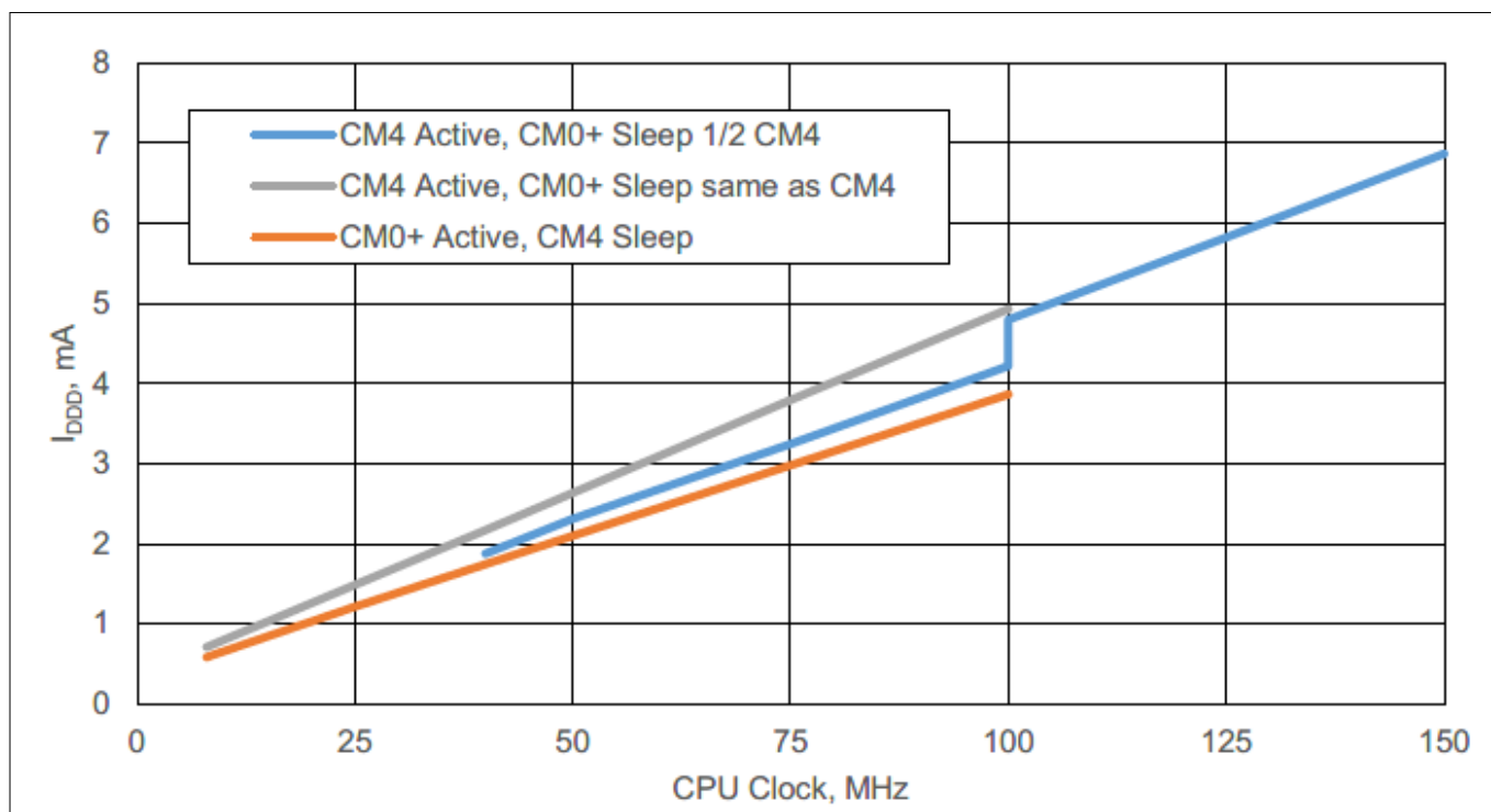
Figure 16 Typical device currents vs. CPU frequency; System low power (LP) mode 1)
