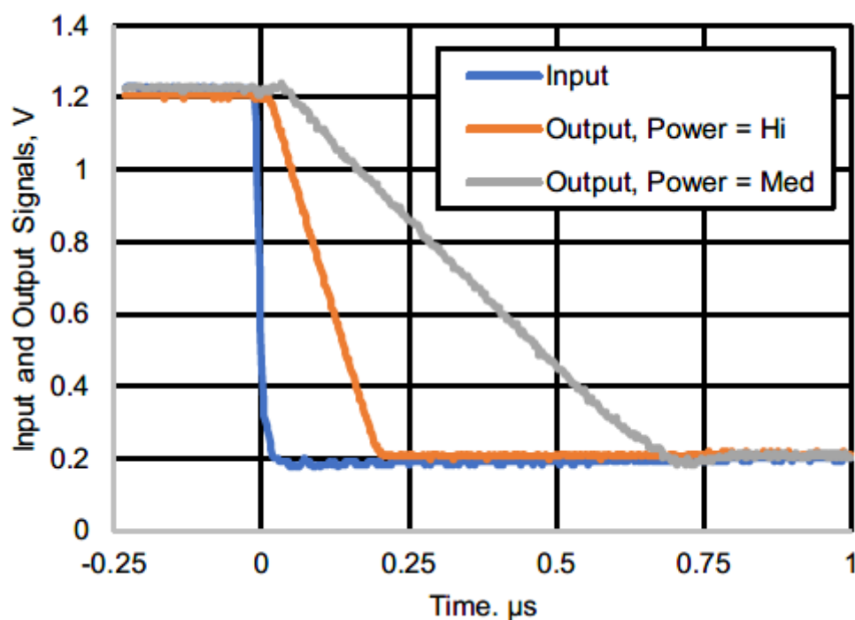
Figure 18 Opamp step response, falling
