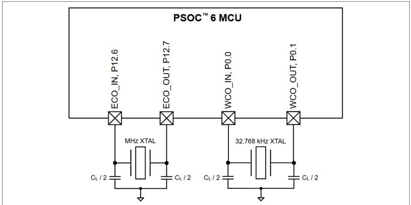
Figure 4 Oscillator circuits
