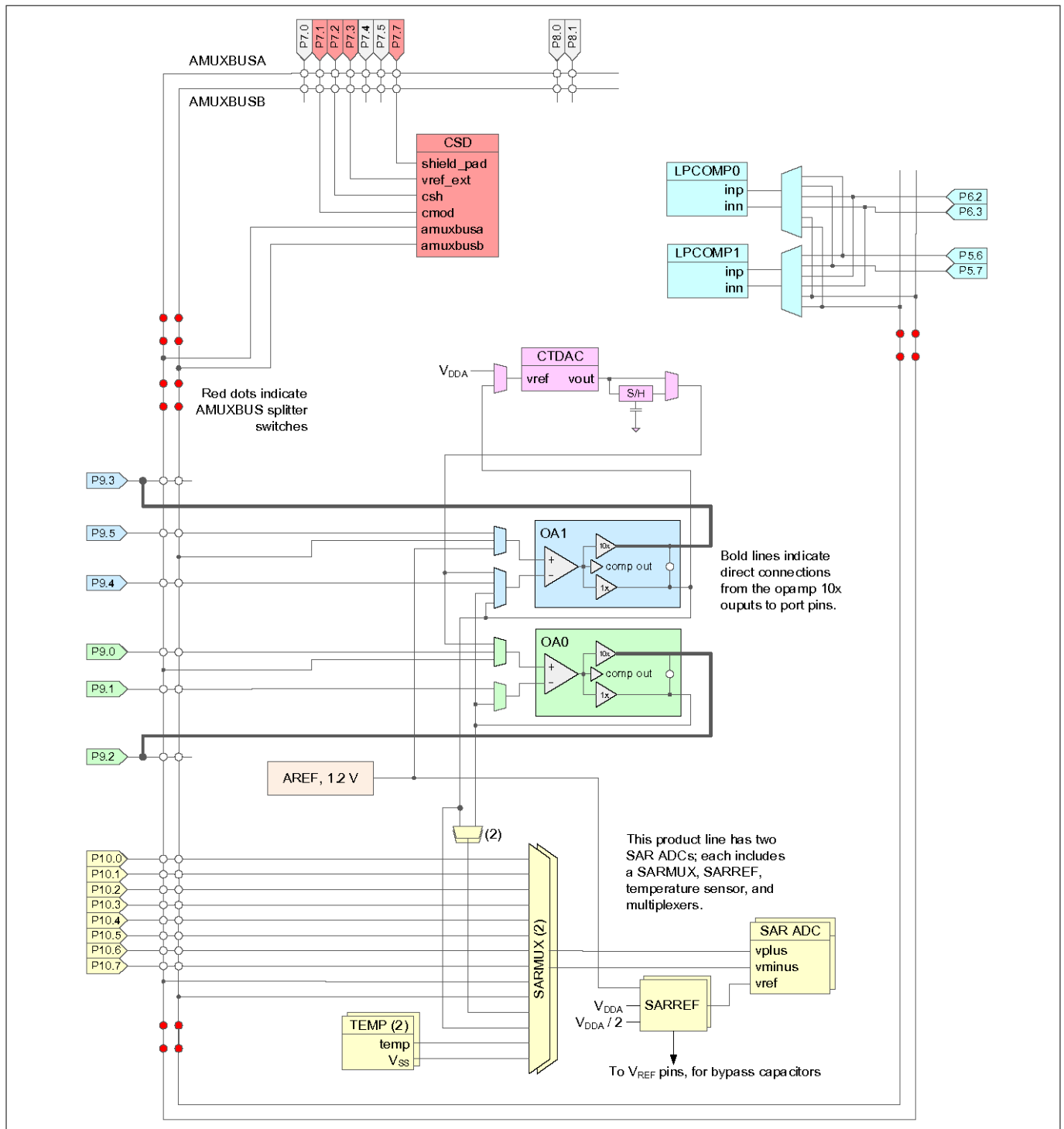
Figure 6 Analog subsystem
