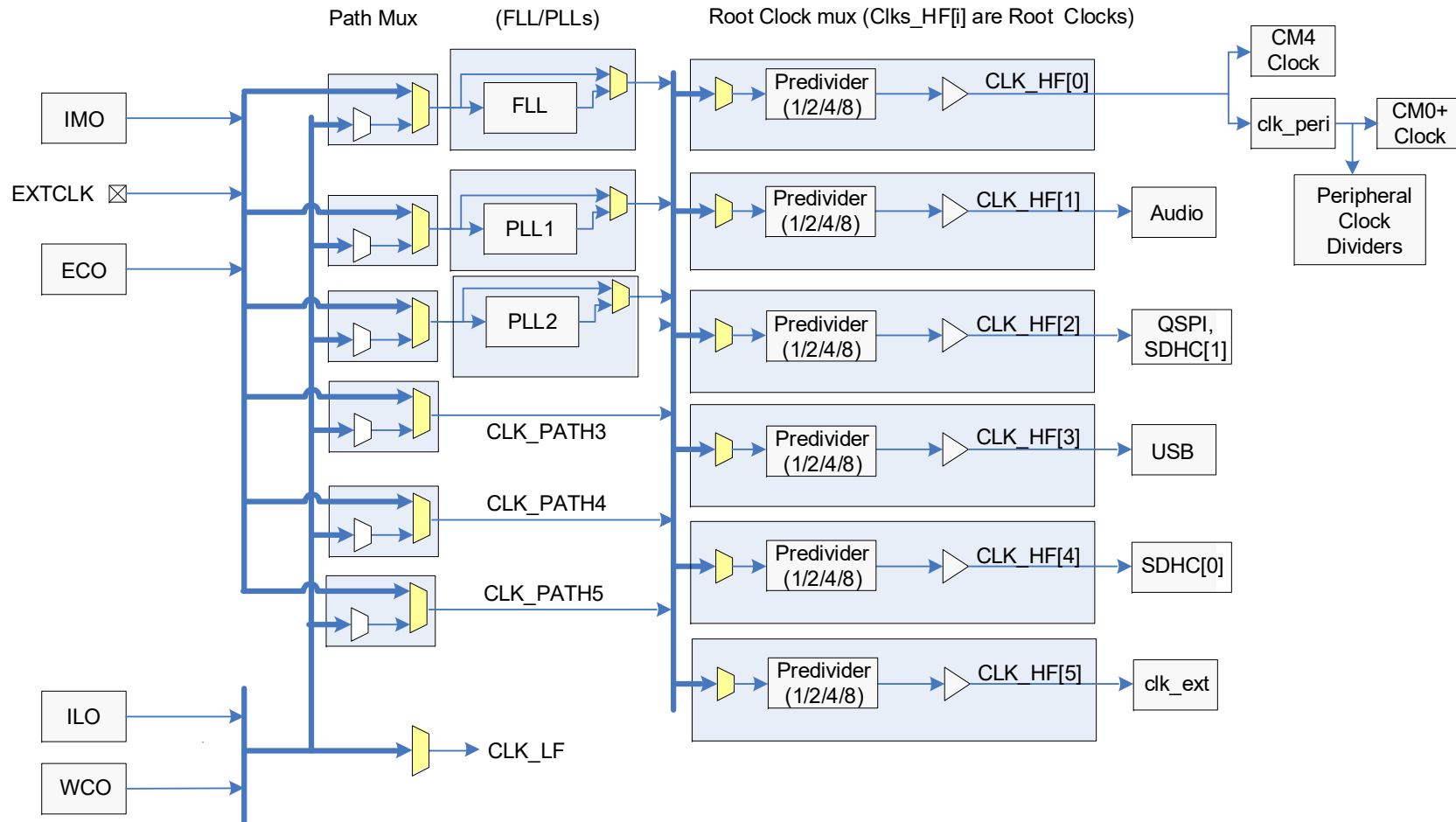
Figure 20-1. Clocking System Block Diagram
