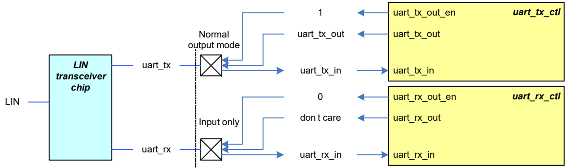
Figure 27-33. LIN Mode I/O Pad Connections
