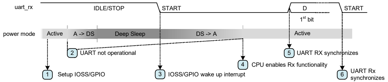
Figure 27-18. UART Start Skip and Wakeup from Deep Sleep
