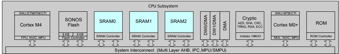
Figure 4-1. CPU Subsystem Block Diagram
