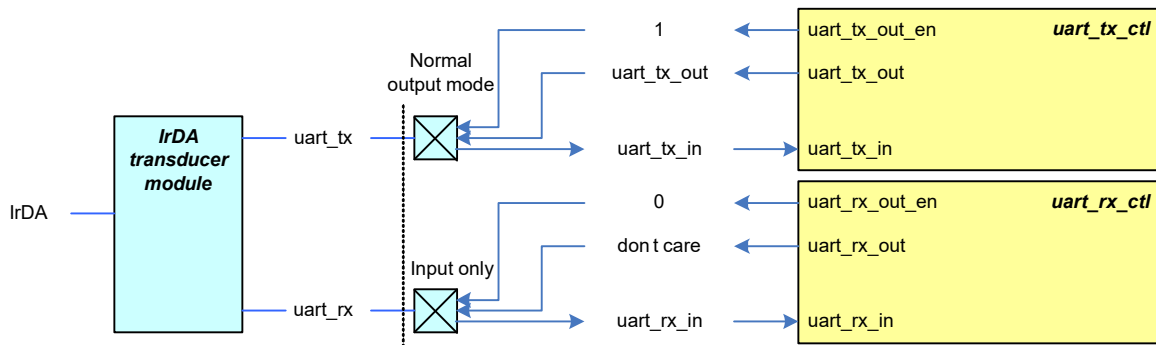
Figure 27-34. IrDA Mode I/O Pad Connections
