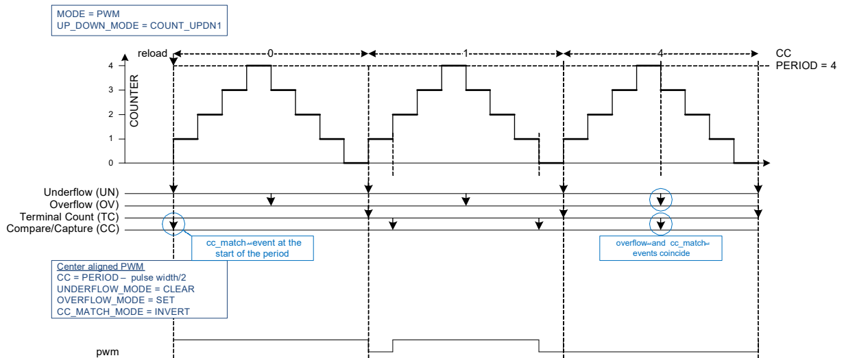
Figure 29-28. Up/Down Counting Center-Aligned PWM
