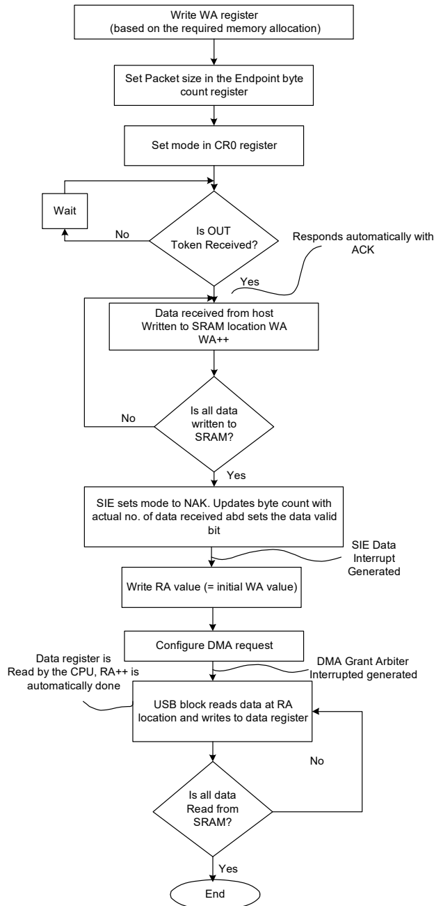
Figure 32-6. Manual DMA OUT Transaction
