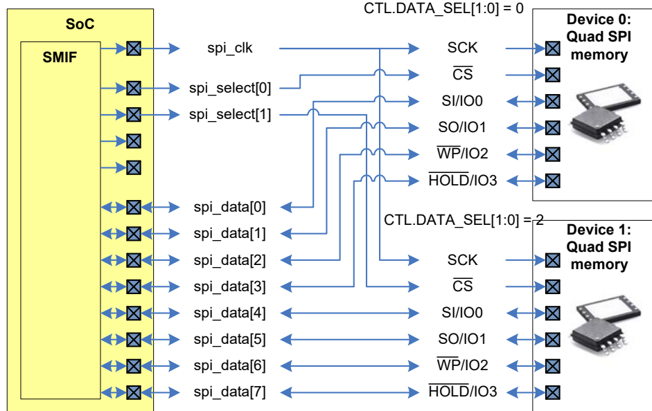
Figure 28-13. Setting up SMIF
