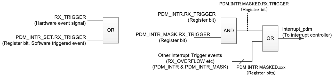
Figure 31-5. PDM Interrupt Signal Generation
