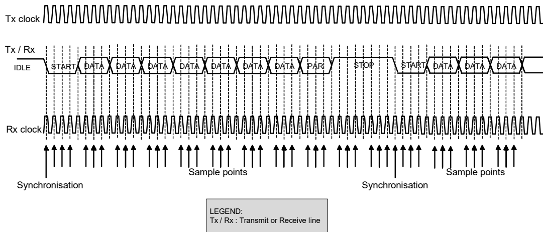
Figure 27-16. UART, Standard Protocol (Multiple Samples)
