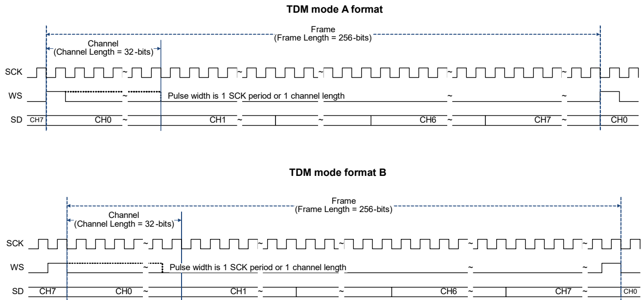
Figure 30-4. TDM Digital Audio Interface Format
