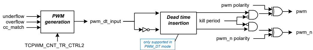
Figure 29-22. PWM Output Generation
