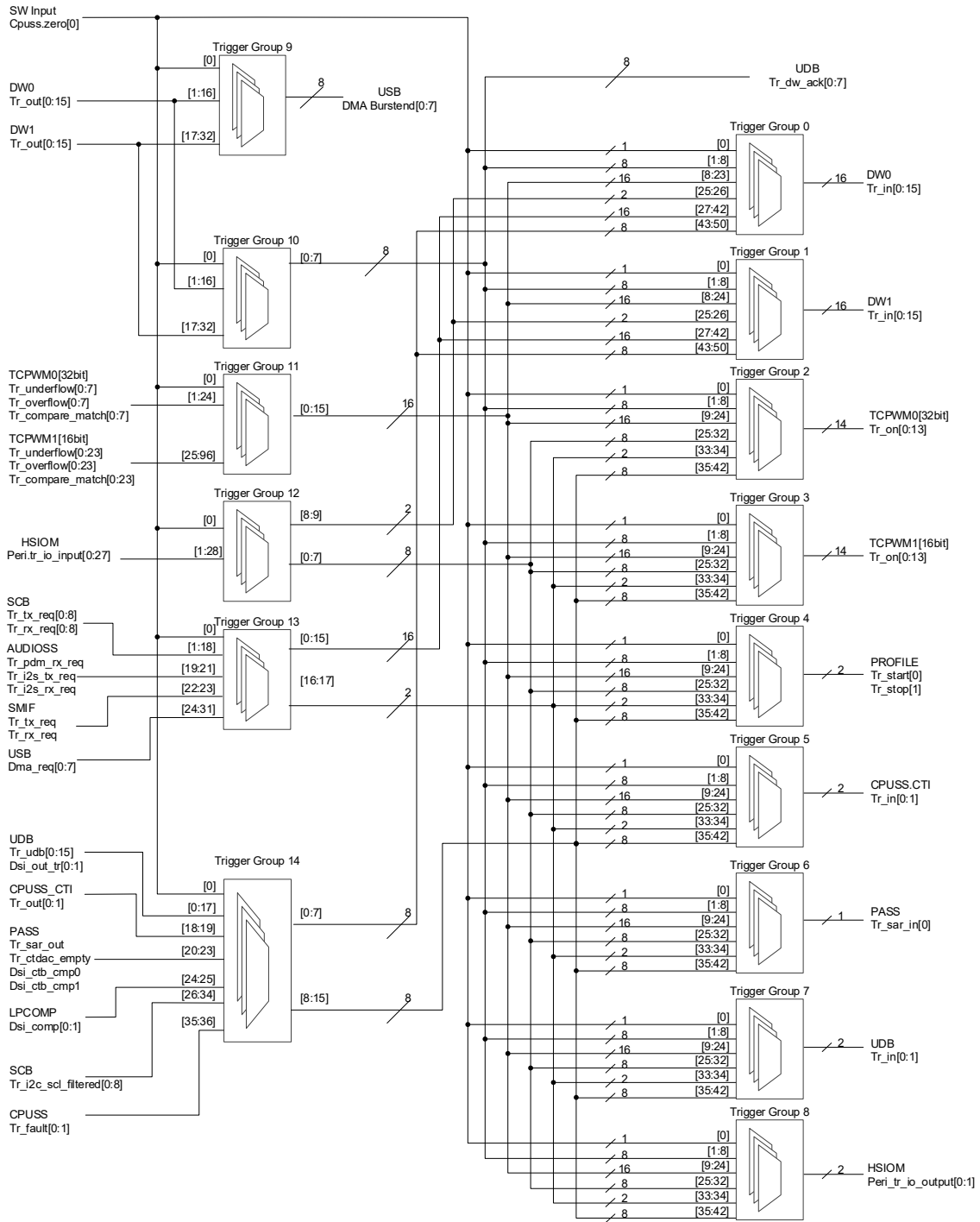
Figure 24-5. PSoC 6 MCU Trigger Multiplexer Block Architecture
