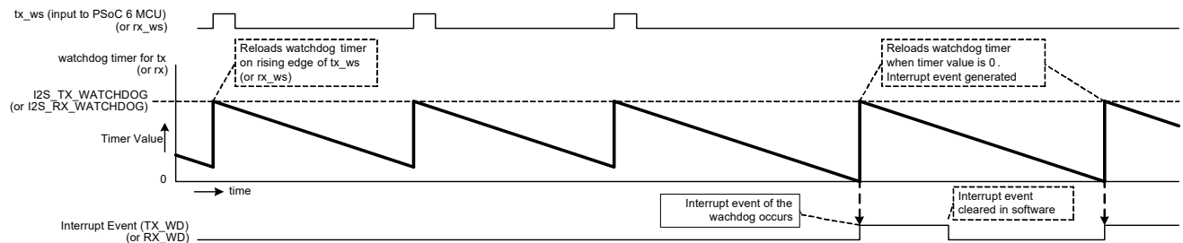
Figure 30-10. Watchdog Timer Working
