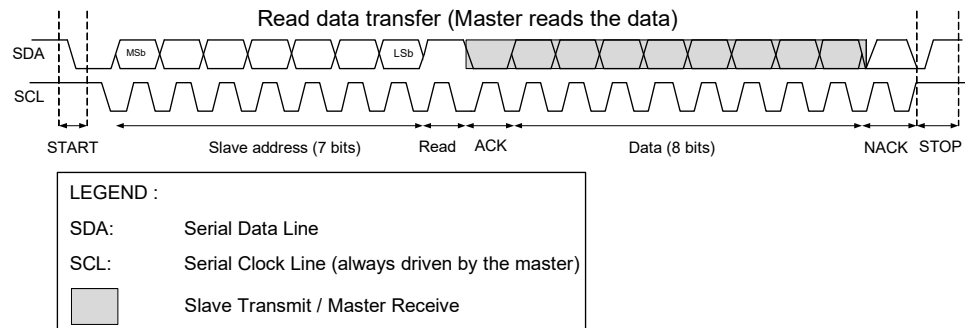
Figure 27-38. Master Read Data Transfer
