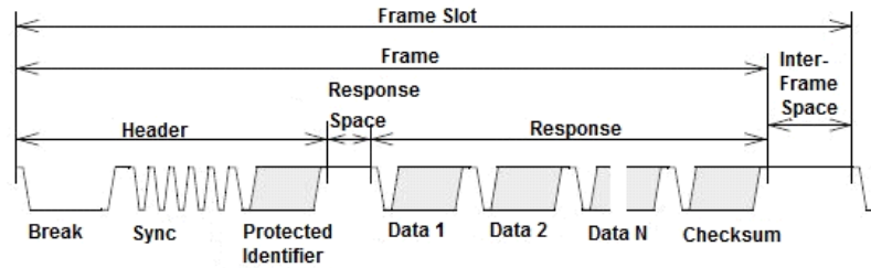
Figure 27-25. LIN Frame Structure
