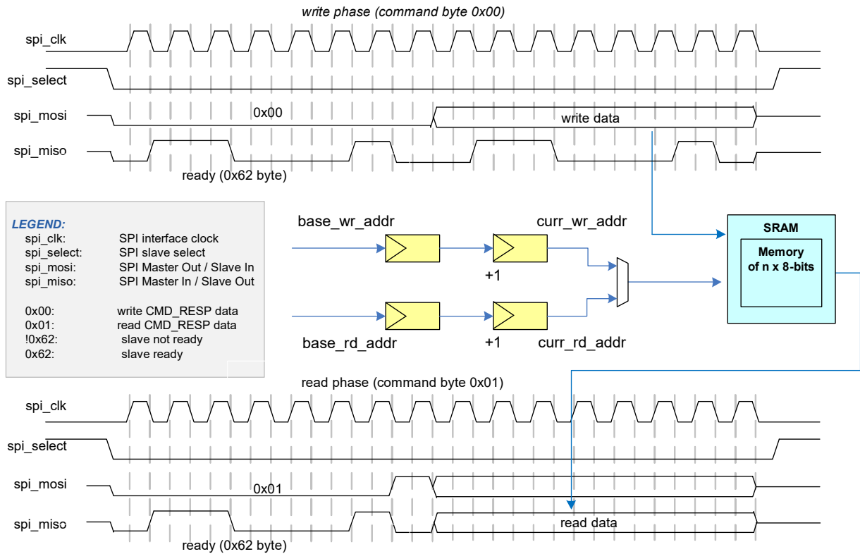
Figure 27-9. Command-Response Mode Example
