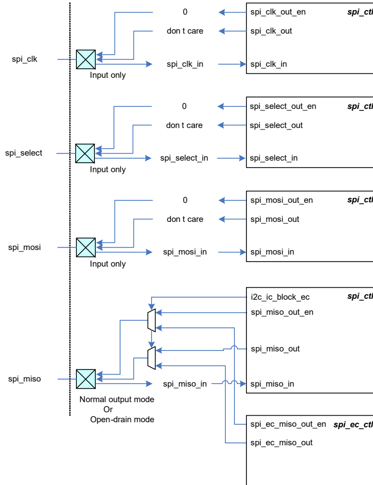
Figure 27-12. SPI Slave I/O Pad Connections
