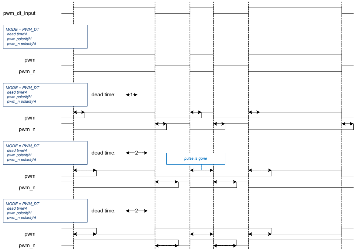
Figure 29-37. Dead-time Timing
