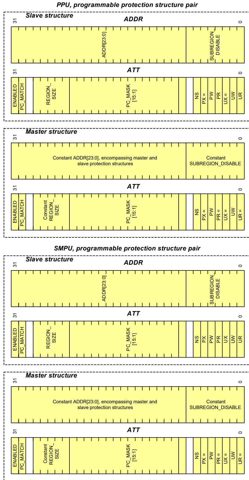
Figure 9-8. Programmable Protection Structure Pair
