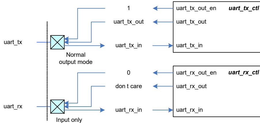
Figure 27-31. Standard UART Mode I/O Pad Connections
