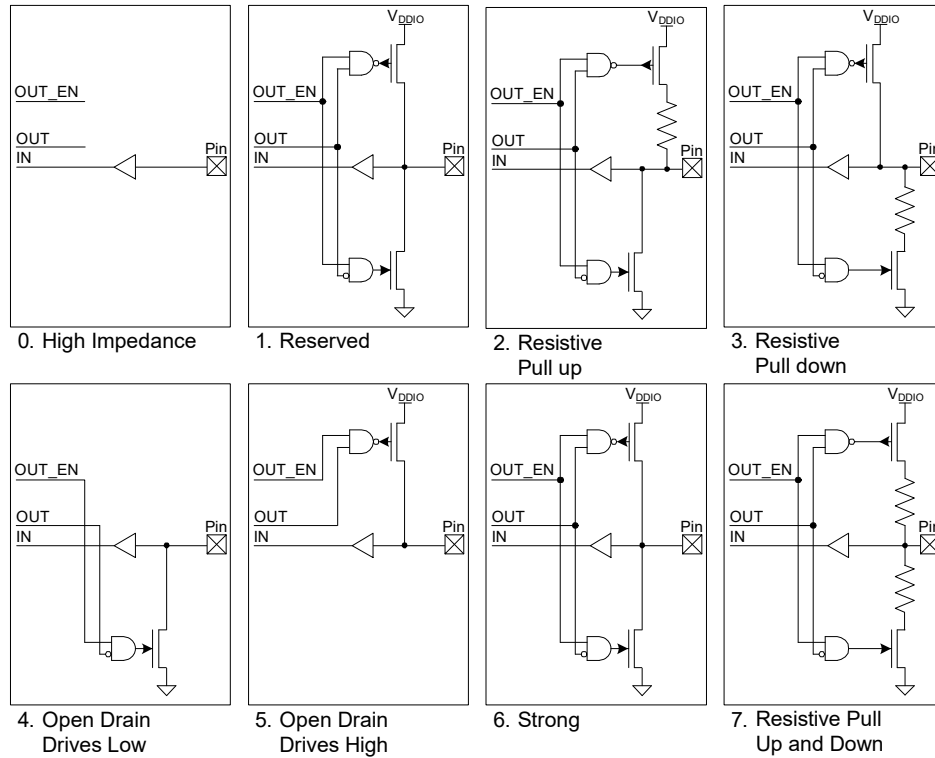
Figure 22-3. CPU I/O Drive Mode Block Diagram
