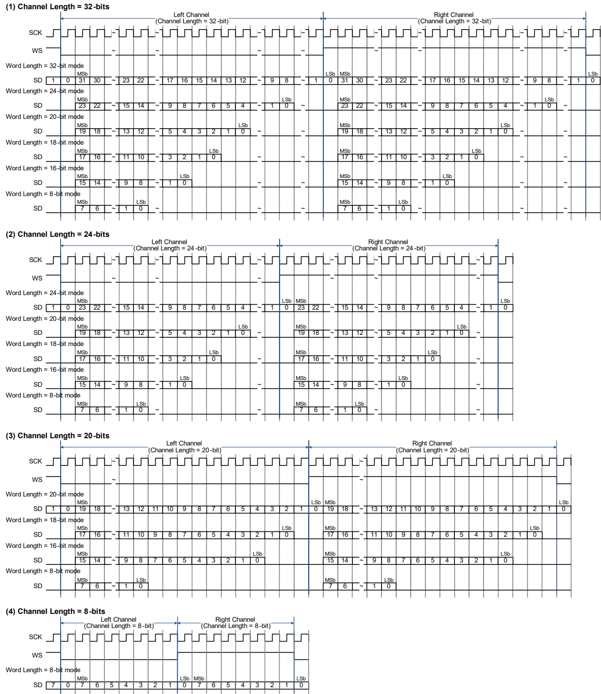
Figure 30-2. Standard I 2 S Format (Word Length and Channel Length Combination Timing Diagrams)
