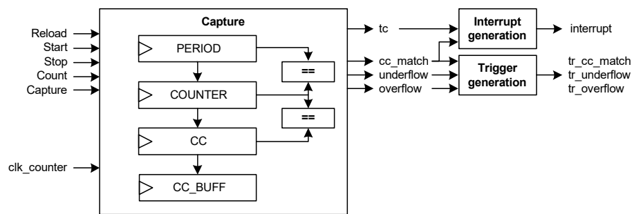
Figure 29-14. Capture Functionality
