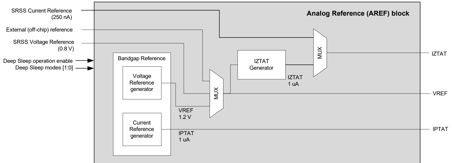
Figure 34-1. AREF Block Diagram
