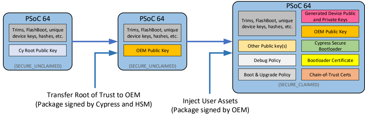
Figure 16-2. Provisioning Scheme
