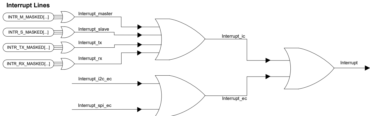
Figure 27-44. Interrupt Lines
