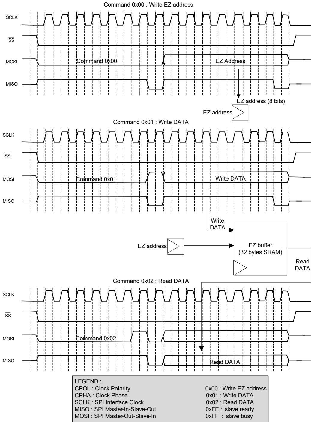
Figure 27-8. EZSPI Example
