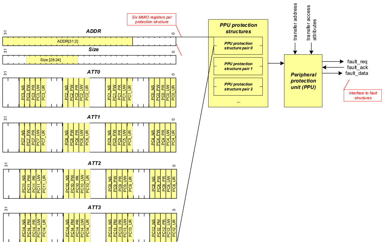
Figure 9-5. PPU Functionality
