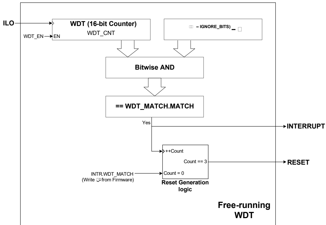
Figure 23-2. Free-running WDT Functional Diagram
