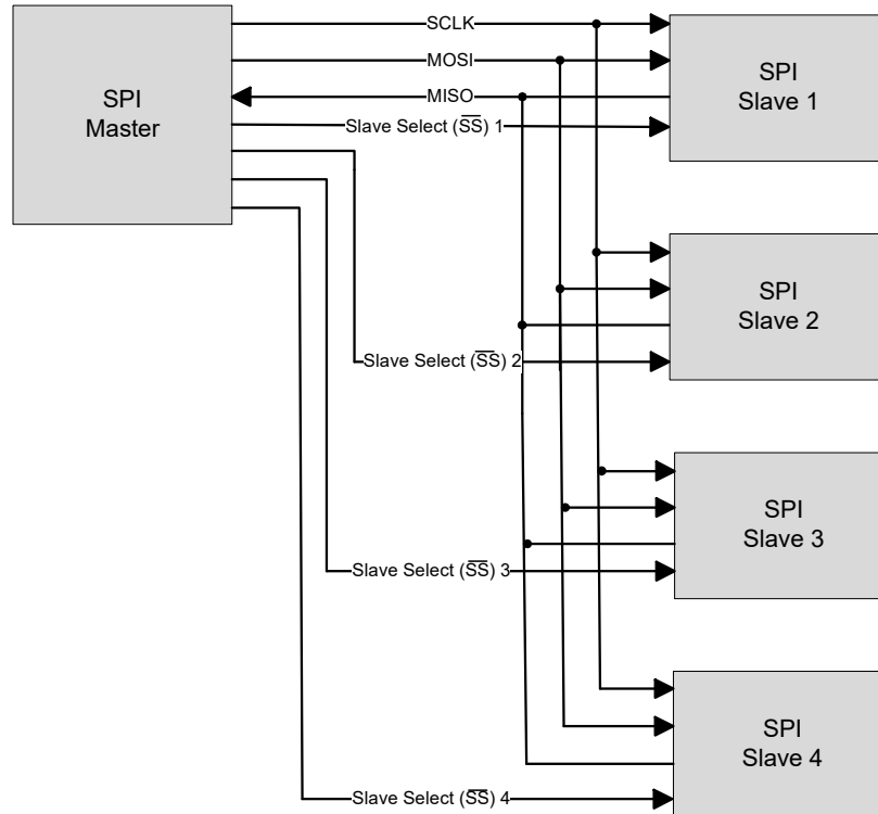
Figure 27-1. SPI Example
