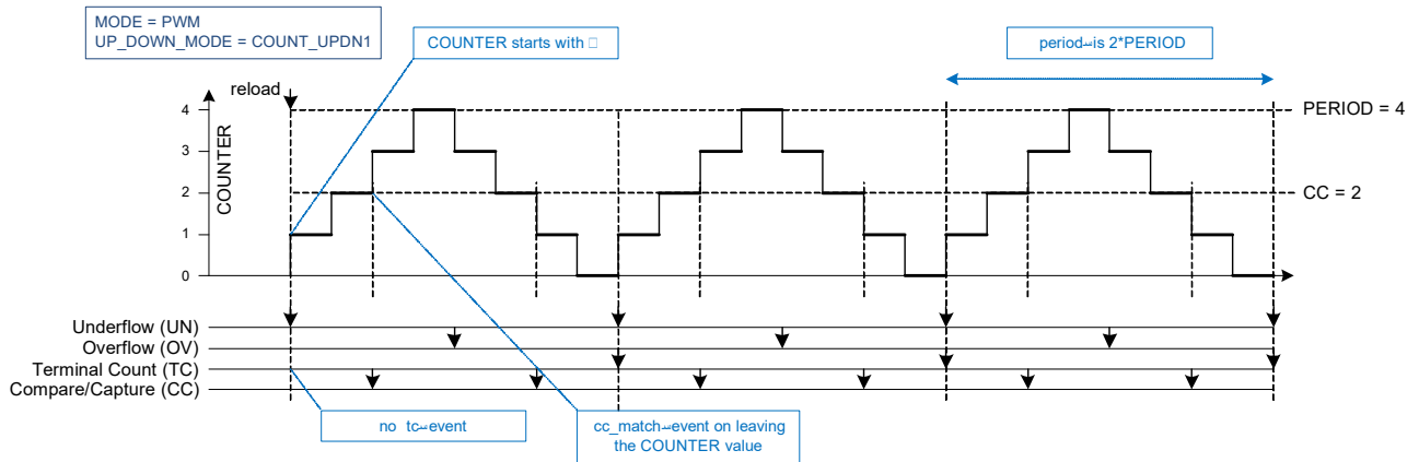
Figure 29-27. Up/Down Counting PWM
