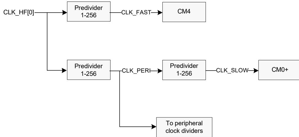
Figure 20-4. CLK_HF[0] Distribution
