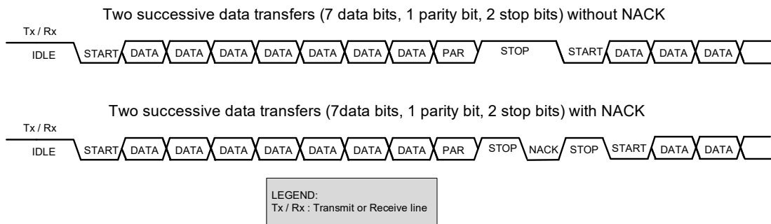
Figure 27-29. SmartCard Example
