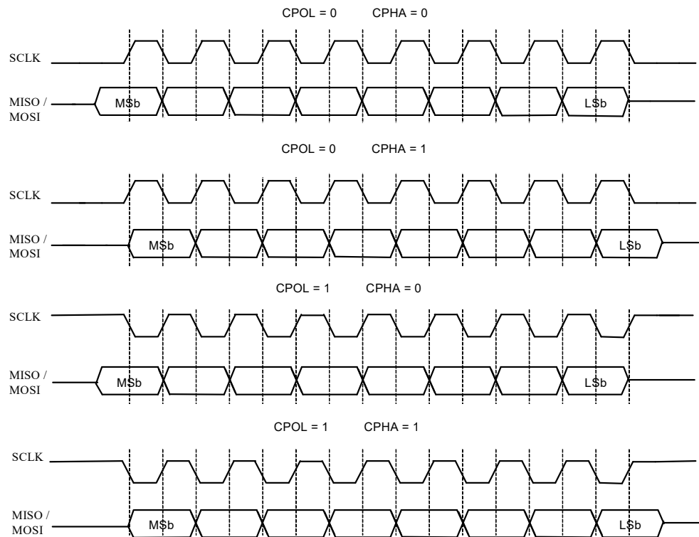
Figure 27-2. SPI Motorola, 4 Modes
