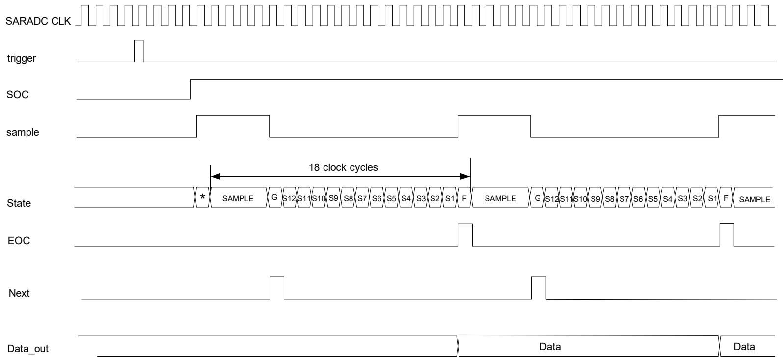
Figure 36-4. SAR ADC Timing
