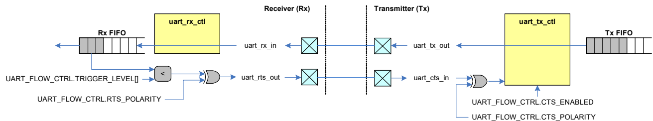
Figure 27-20. UART Flow Control Connection
