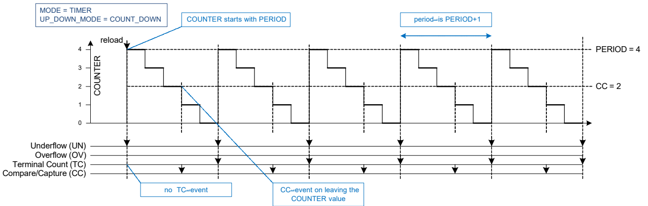
Figure 29-10. Timer in Down-counting Mode
