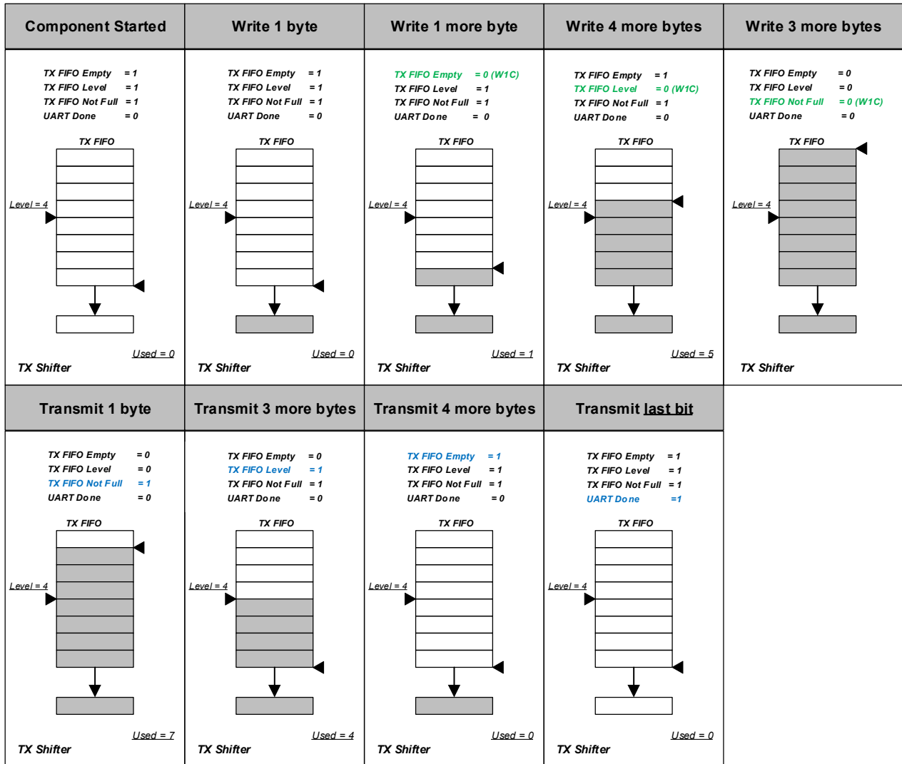
Figure 27-47. TX Interrupt Source Operation
