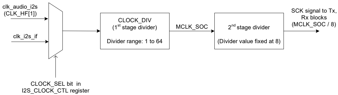
Figure 30-6. Clocking Divider Structure
