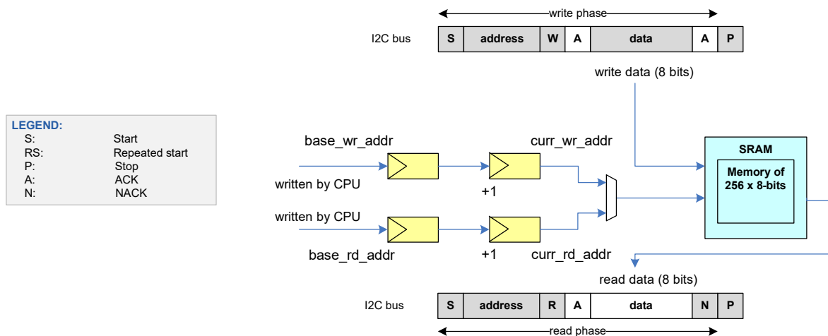
Figure 27-40. I 2 C Command-Response Mode
