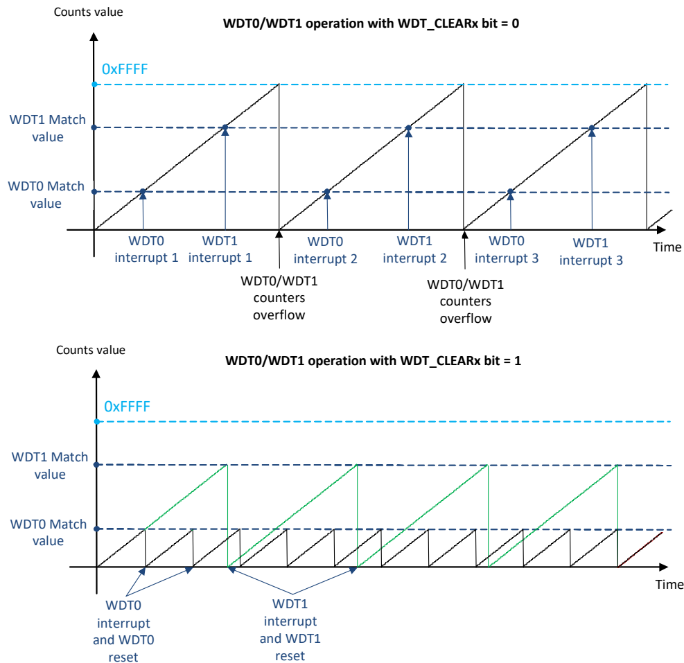
Figure 23-4. WDT0/WDT1 Operation
