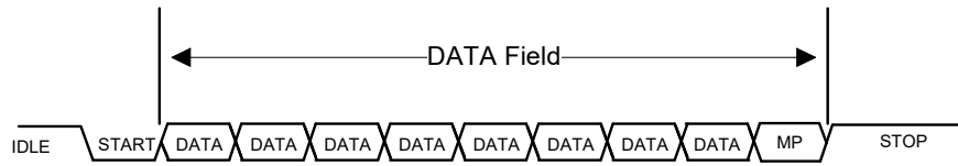
Figure 27-22. UART MP Address and Data Frame
