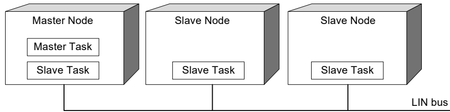
Figure 27-24. LIN Bus Nodes and Tasks
