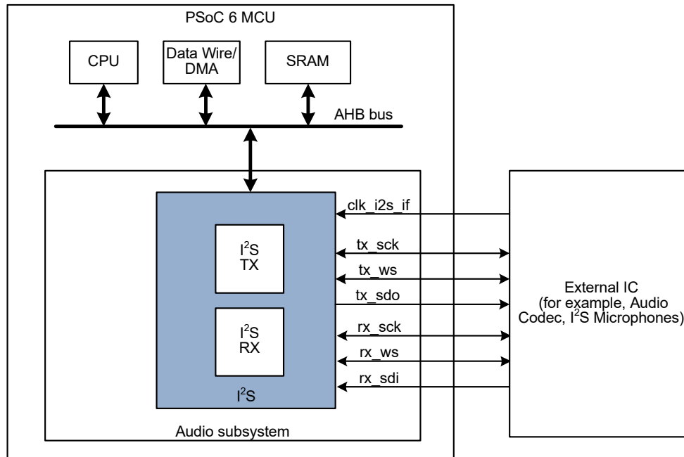
Figure 30-1. I 2 S Block Diagram
