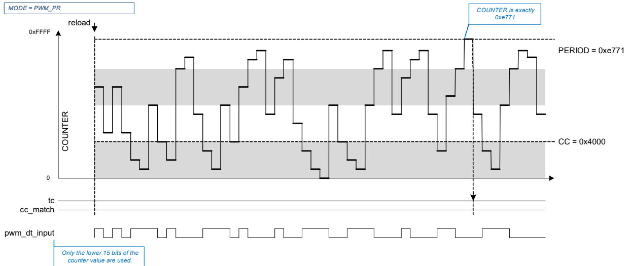
Figure 29-40. PWM_PR Output
