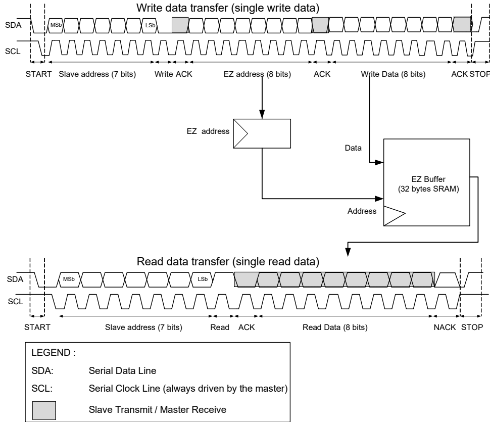
Figure 27-39. EZI2C Write and Read Data Transfer
