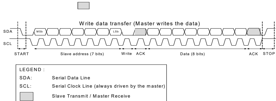
Figure 27-37. Master Write Data Transfer
