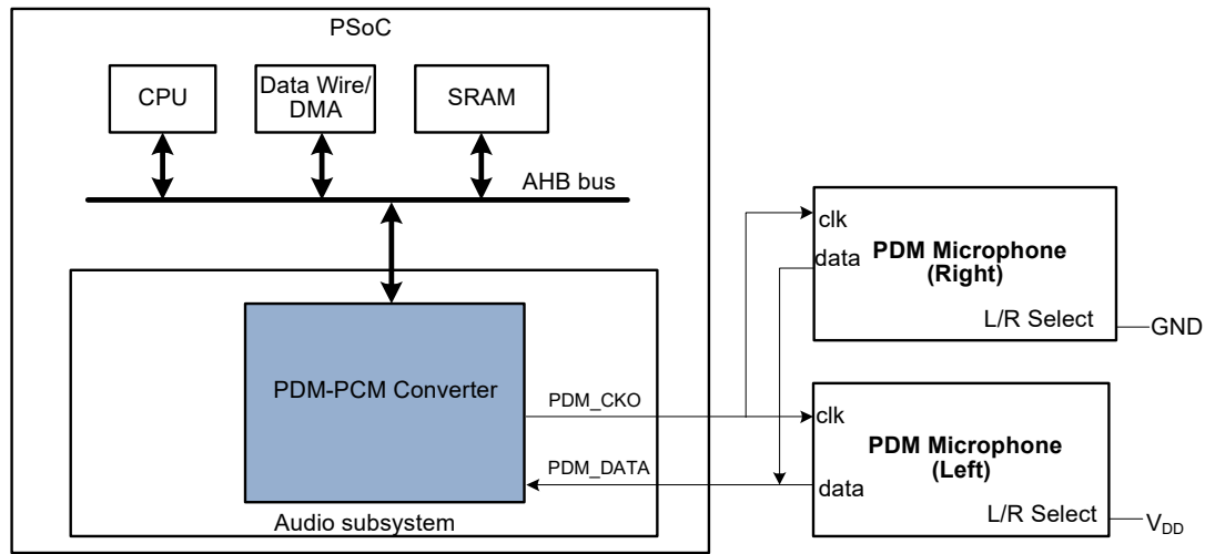
Figure 31-1. Block Diagram
