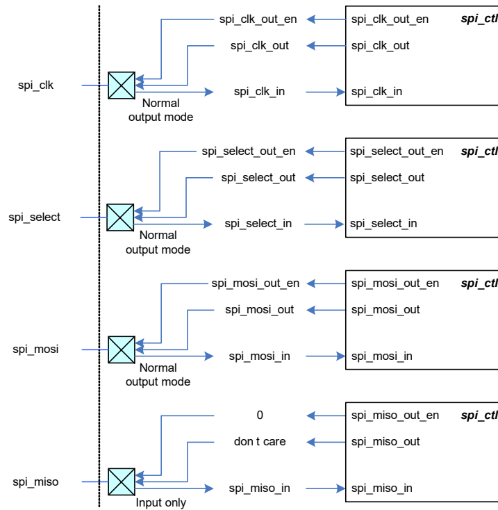
Figure 27-11. SPI Master I/O Pad Connections
