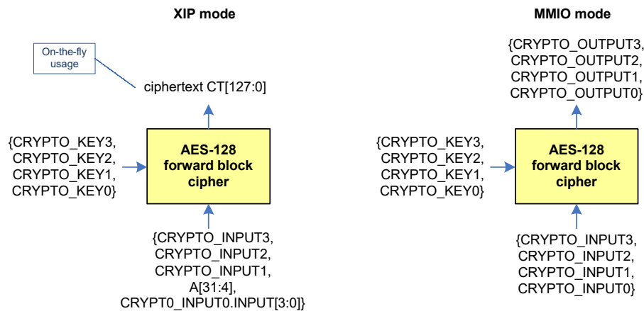
Figure 28-2. Cryptography in XIP and MMIO Modes
