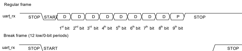
Figure 27-19. UART – Regular Frame and Break Frame
