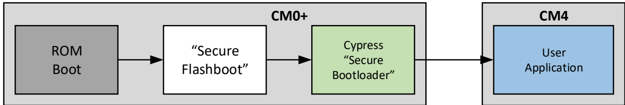
Figure 16-4. Boot Sequence
