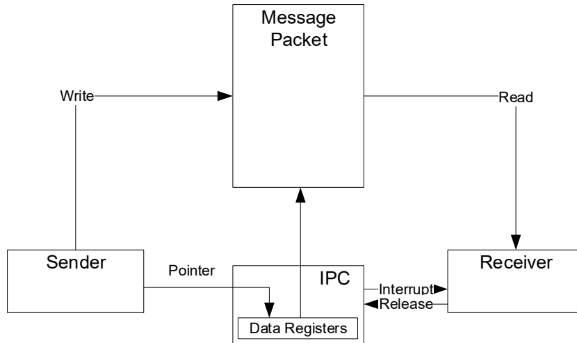
Figure 6-5. Communicating Larger Messages
