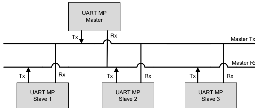
Figure 27-21. UART MP Mode Bus Connections
