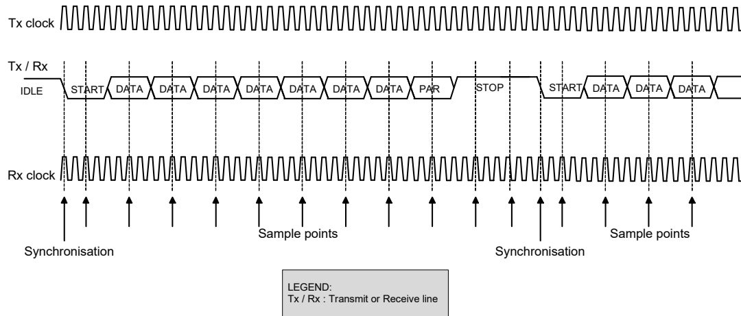
Figure 27-15. UART, Standard Protocol Example (Single Sample)
