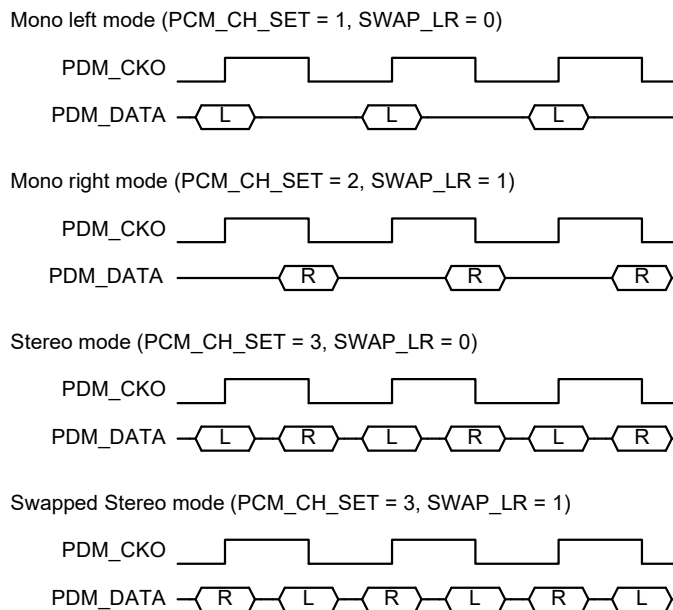
Figure 31-3. PDM Mono/Stereo Timing
