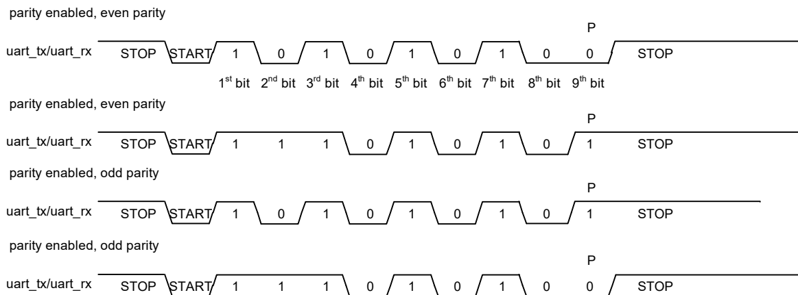
Figure 27-17. UART Parity Examples
