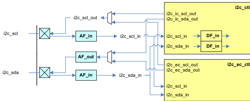
Figure 27-41. I 2 C Glitch Filtering Connection
