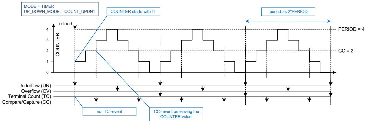
Figure 29-11. Timer in Up/Down Counting Mode 1
