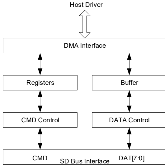
Figure 26-4. Data Flow
