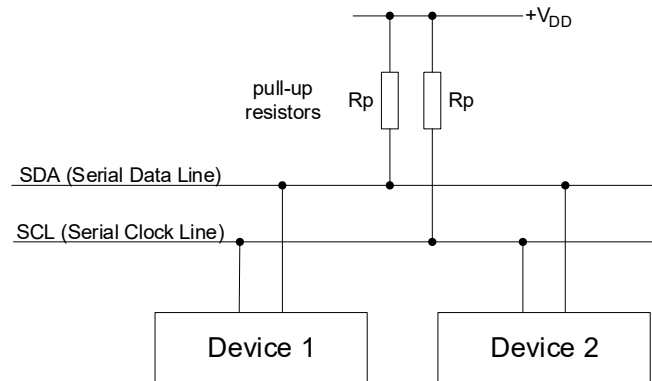
Figure 27-36. Connection of Devices to the I 2 C Bus
