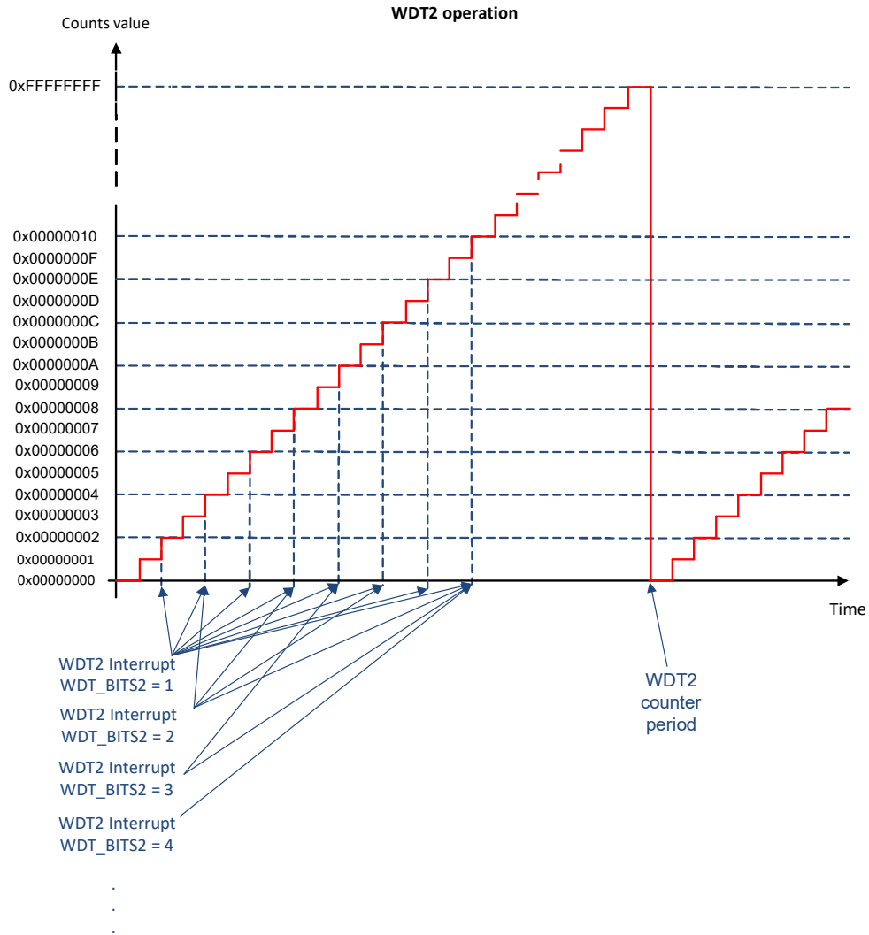
Figure 23-5. WDT2 Operation
