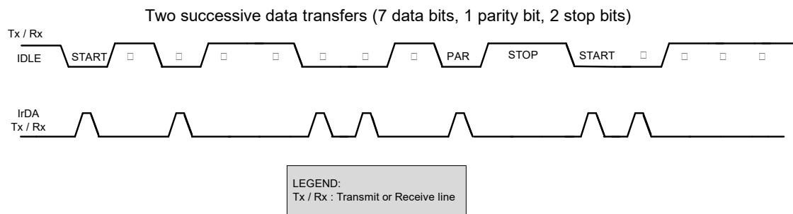
Figure 27-30. IrDA Example
