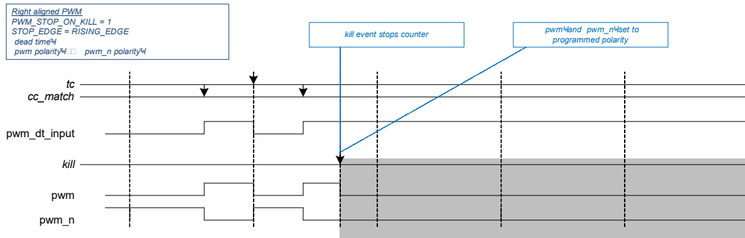
Figure 29-29. PWM Stop on Kill
