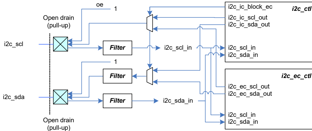
Figure 27-43. I 2 C I/O Pad Connections
