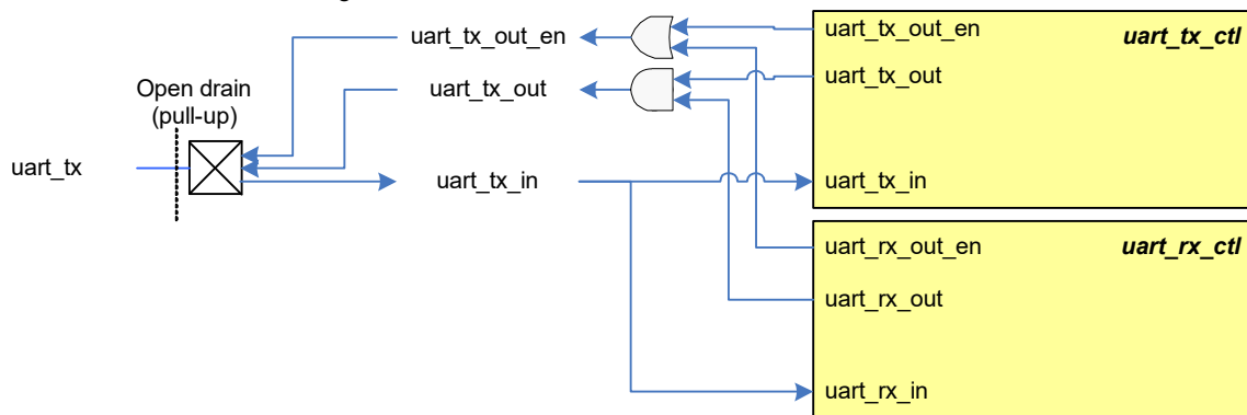
Figure 27-32. SmartCard Mode I/O Pad Connections
