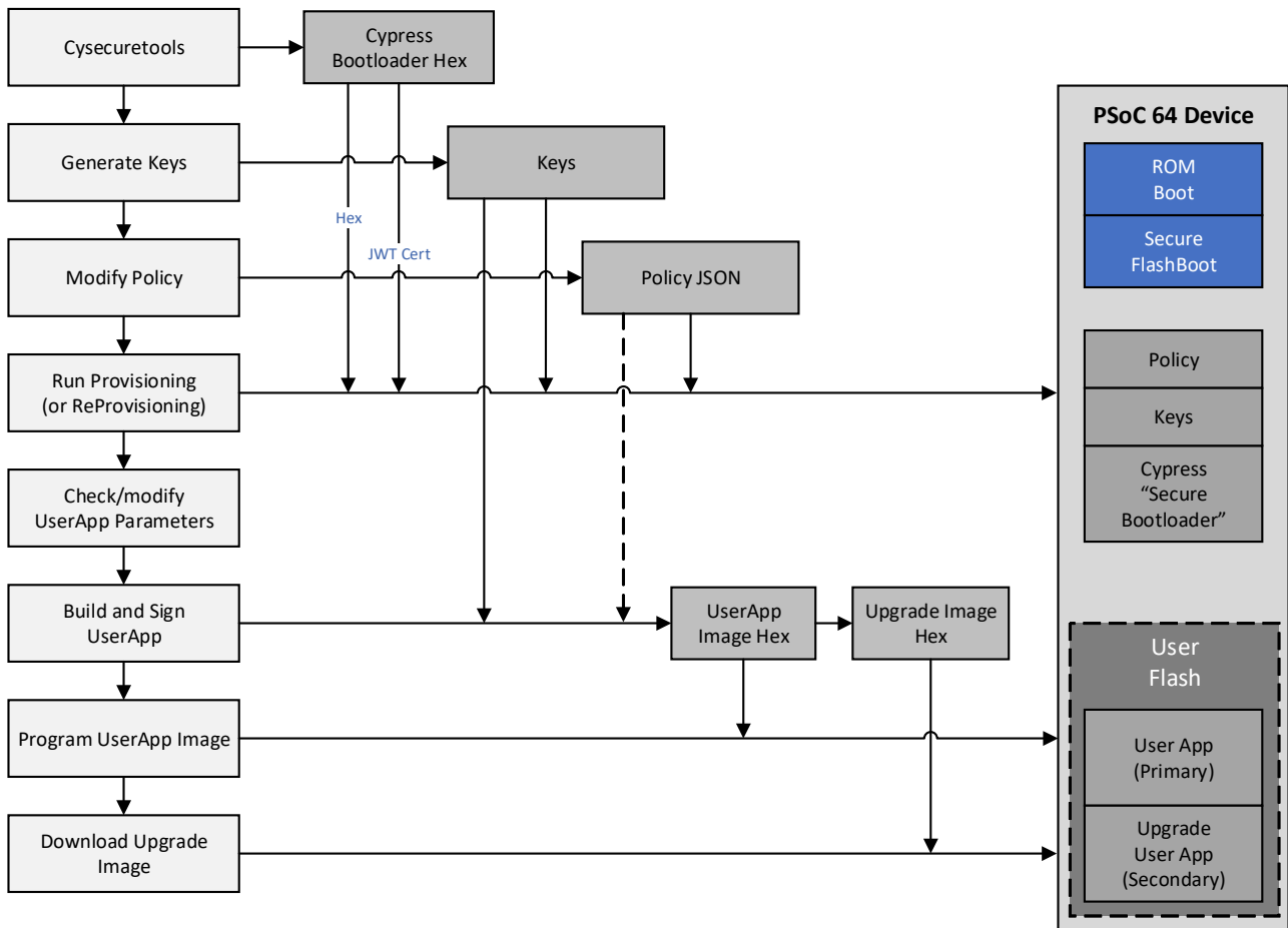
Figure 16-3. OEM Provisioning and Programming Flow
