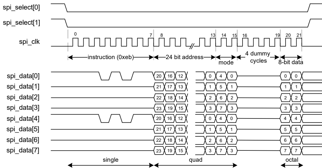
Figure 28-14. Two-Byte Transfer in Dual Quad SPI Mode
