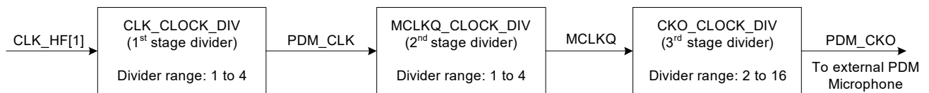
Figure 31-2. PDM-PCM Clocking Dividers
