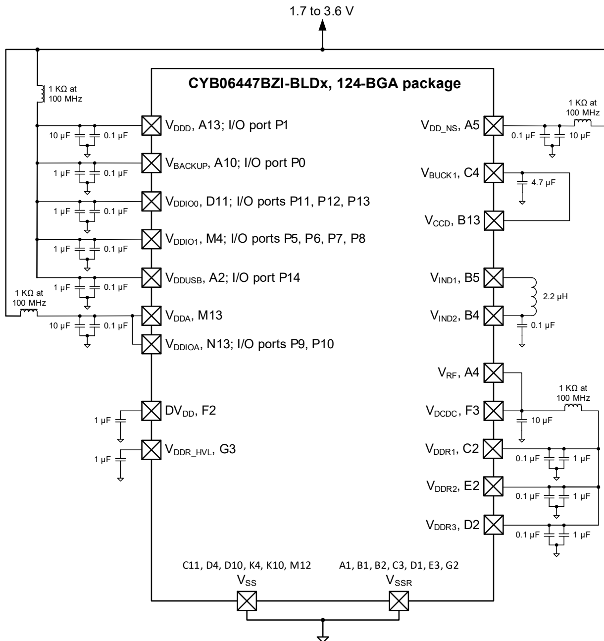
Figure 14. 124-BGA Power Connection Diagram
