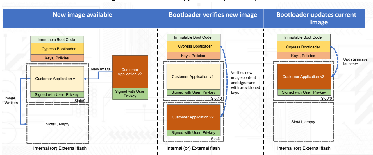
Figure 13. Bootloader Application Update Sequence
