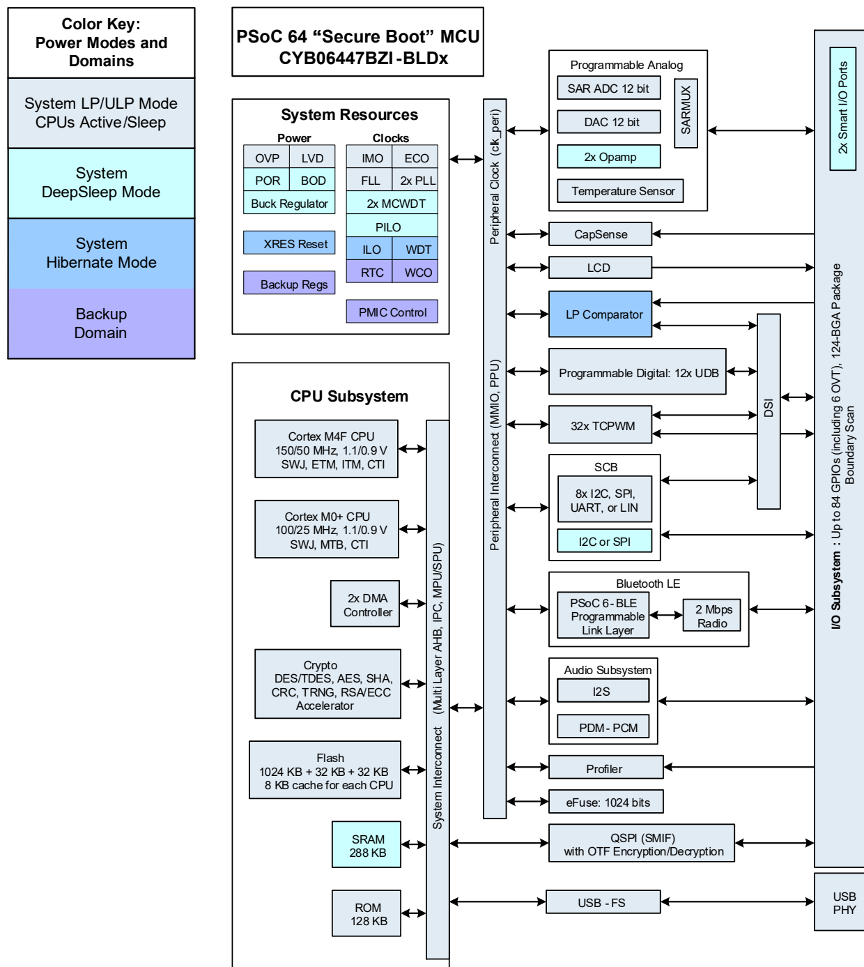
Figure 2. Block Diagram
