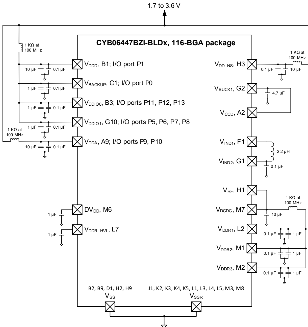
Figure 15. 116-BGA Power Connection Diagram
