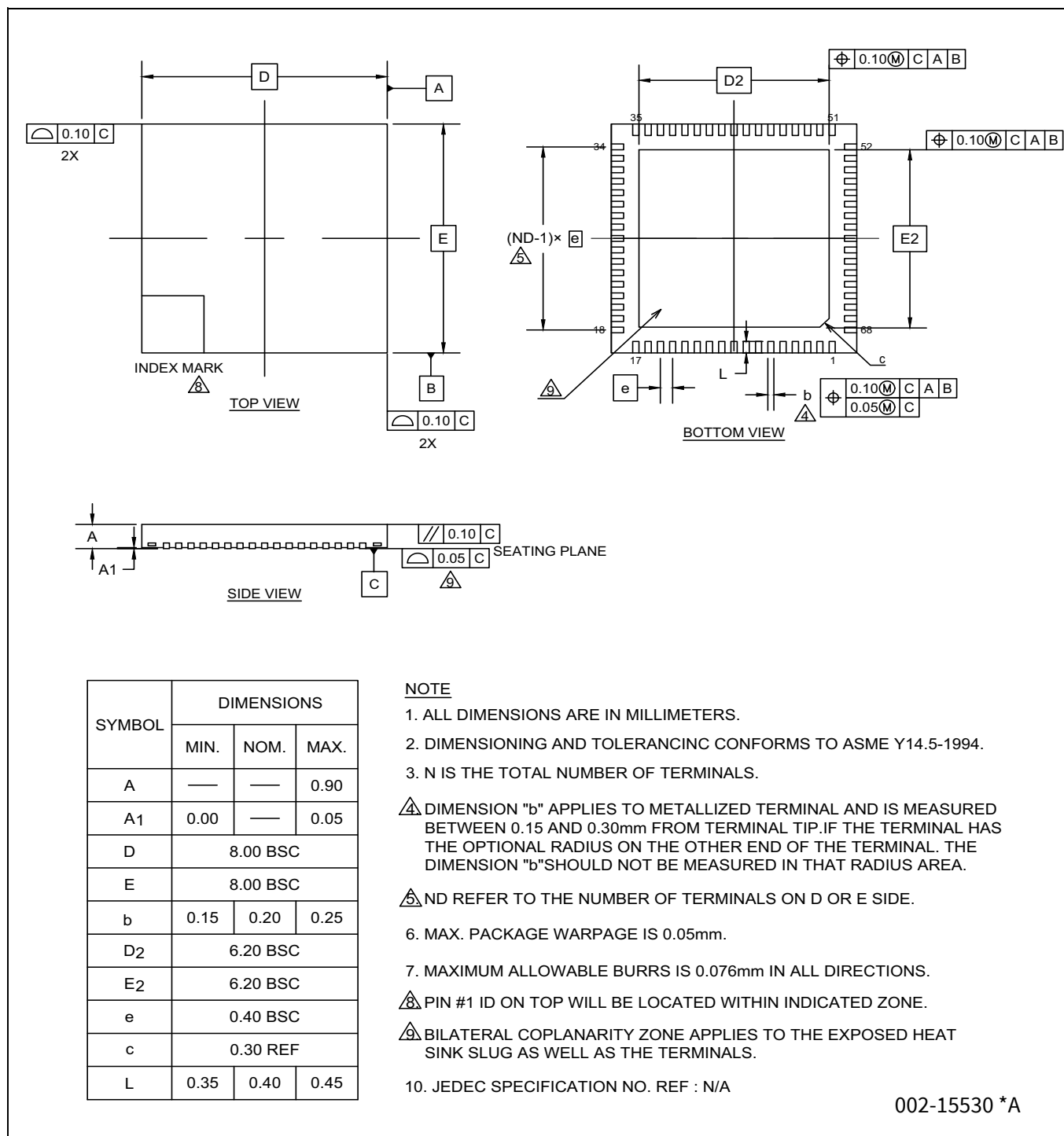
Figure 10 68-pin QFN package (0.5 mm pitch) outline
