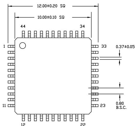
Figure 18. 44-pin TQFP Package Outline
