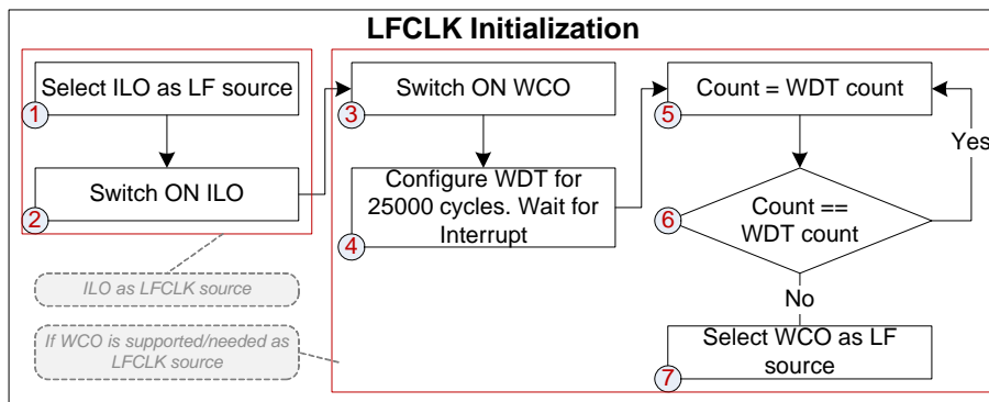
Figure 18-2. LFCLK Initialization
