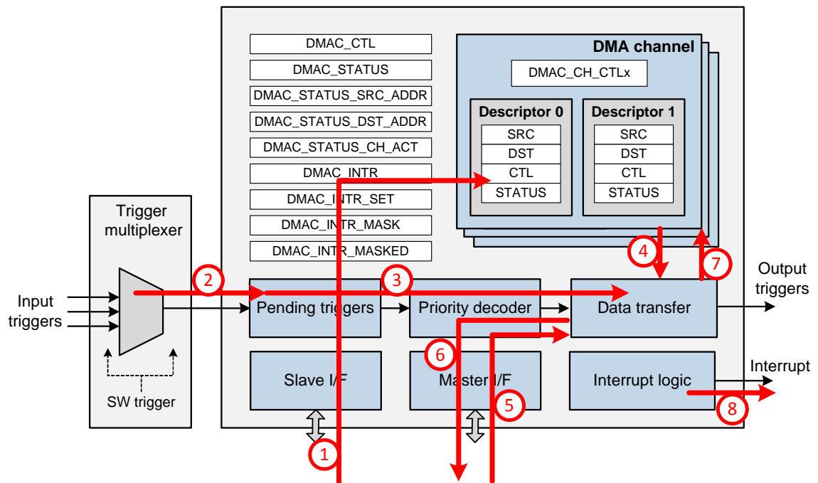
Figure 5-11. Operational Flow
