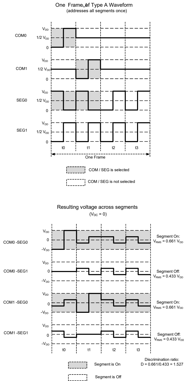
Figure 23-2. PWM1/2 Type-A Waveform Example
