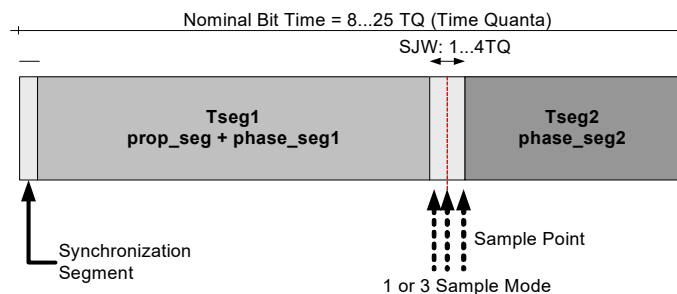
Figure 17-13. Bit Time
