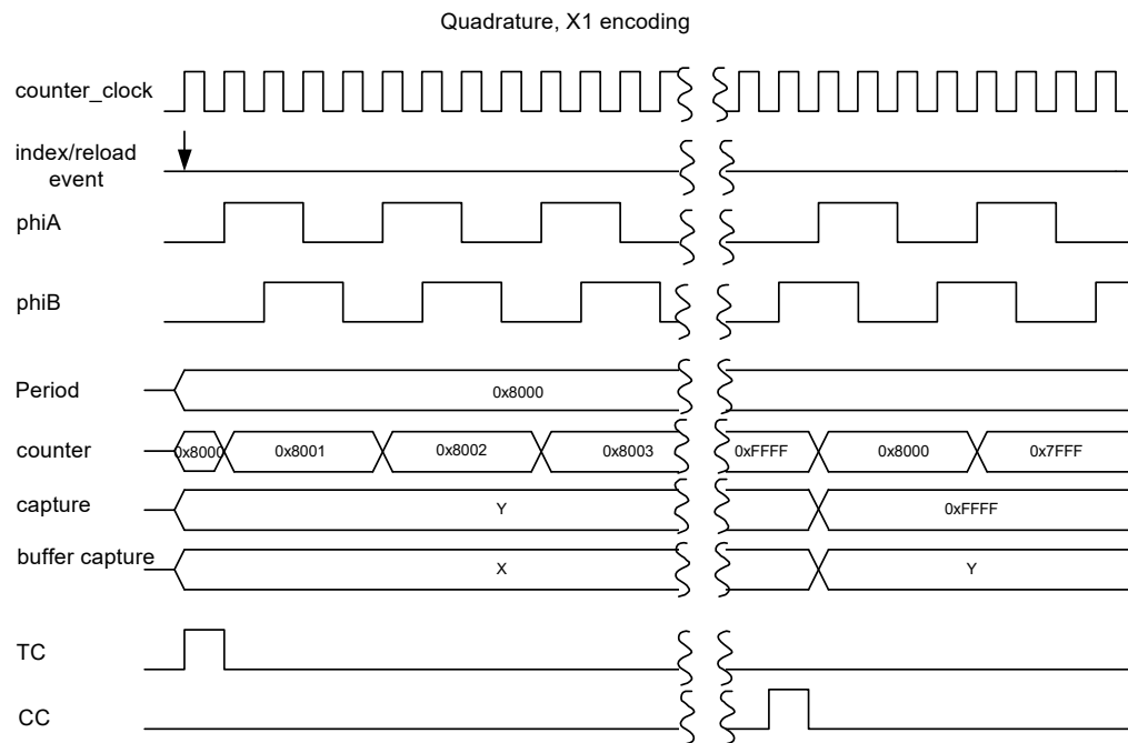
Figure 18-9. Timing Diagram for Quadrature Mode, X1 Encoding
