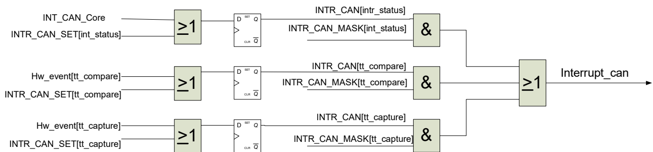
Figure 17-17. CAN Interrupts with CAN_CNTL.TT_ENABLE = 1
