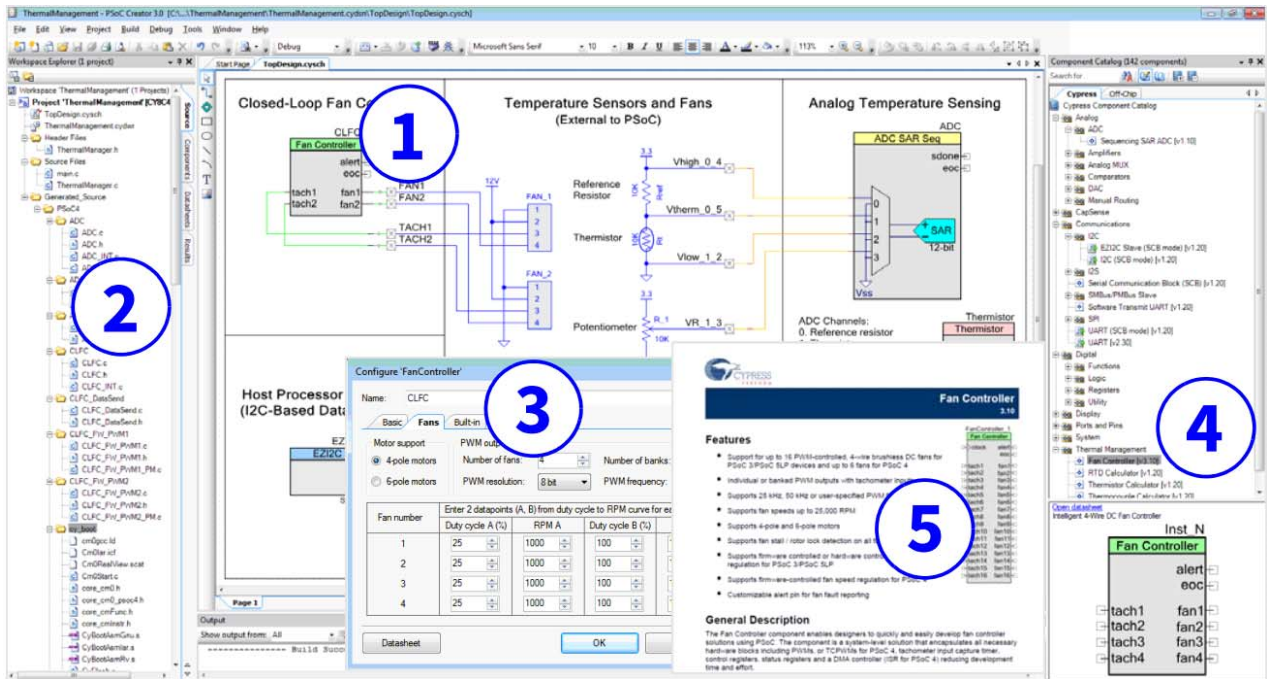
Figure 2-1. Multiple-sensor example project in PSoC Creator
