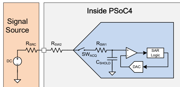
Figure 20-2. Acquisition Time
