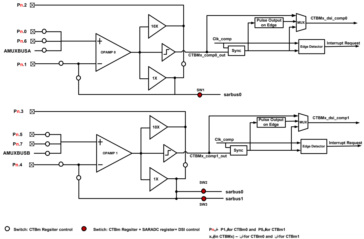
Figure 22-1 shows the block diagram for the CTBmx - CTBm0 and CTBm1 block available in PSoC 4 devices.
