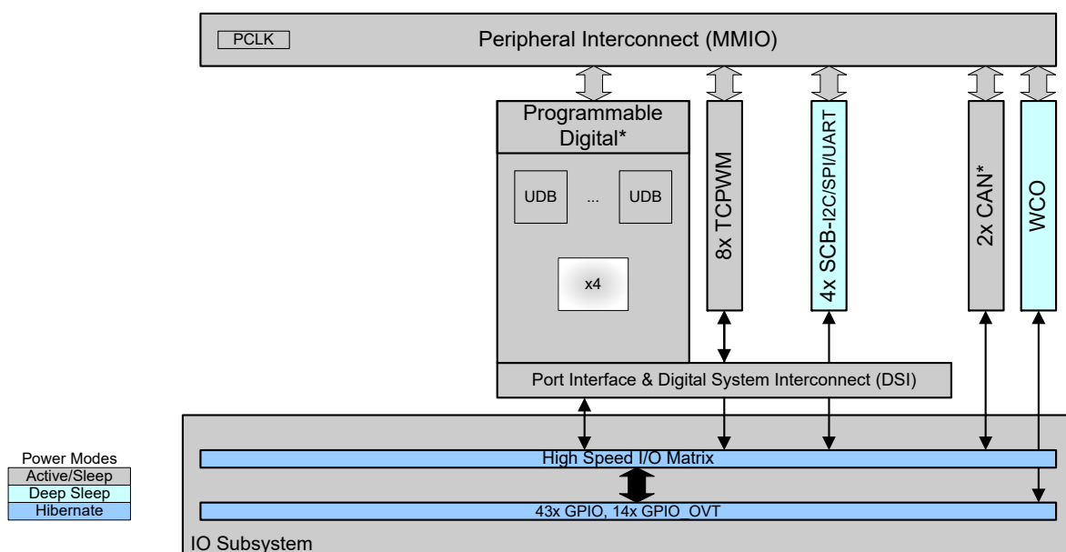
Digital System Block Diagram
