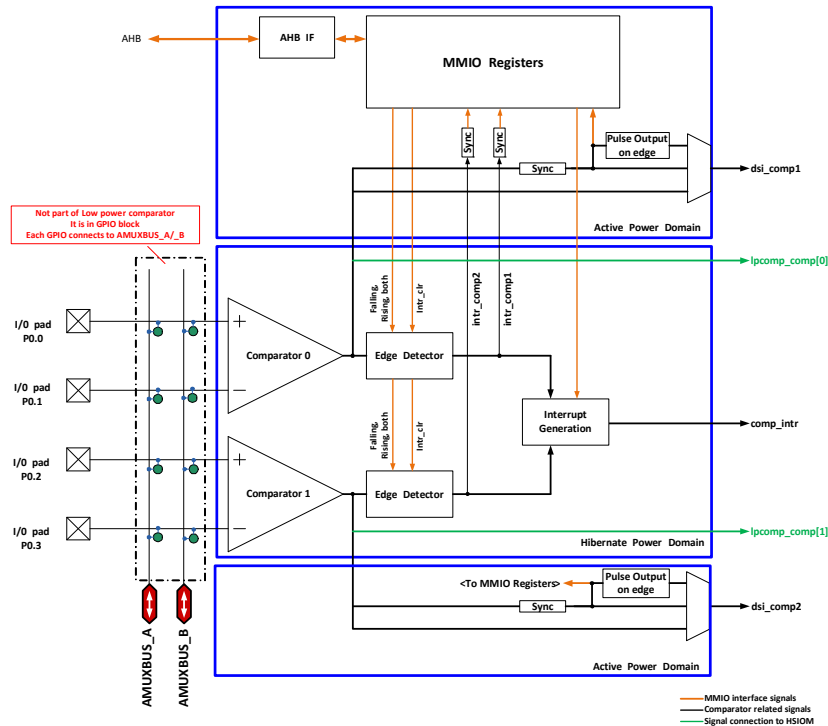
Figure 21-1. Low-Power Comparator Block Diagram
