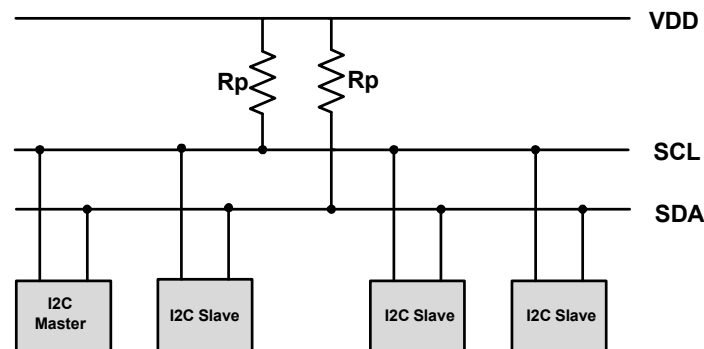
Figure 15-22. I 2 C Interface Block Diagram
