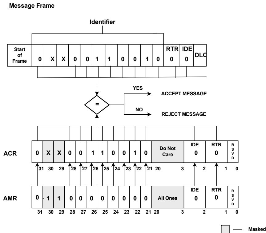
Figure 17-9. Acceptance Filter
