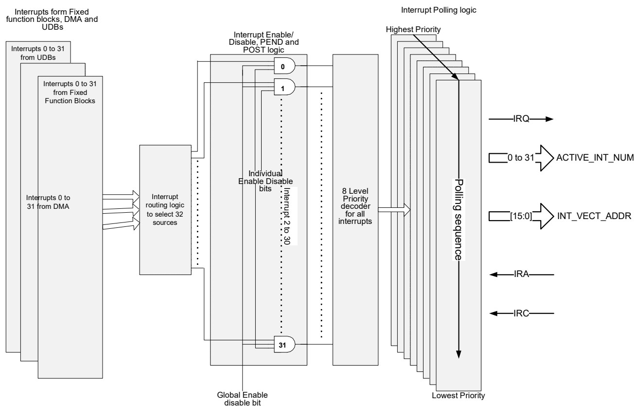
Figure 4-3. Interrupt Structure
