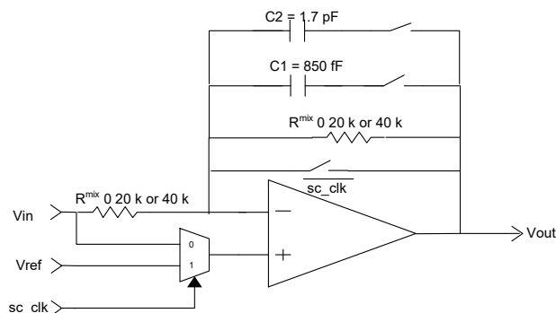
Figure 8-12. Mixer Configuration
