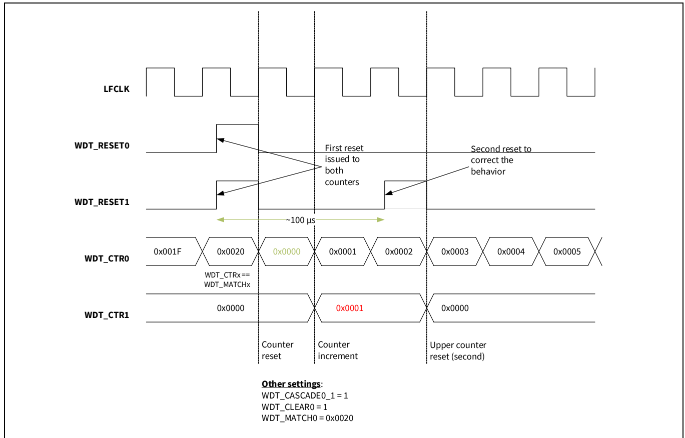
Figure 24-6. MCWDT reset behavior in cascaded mode
