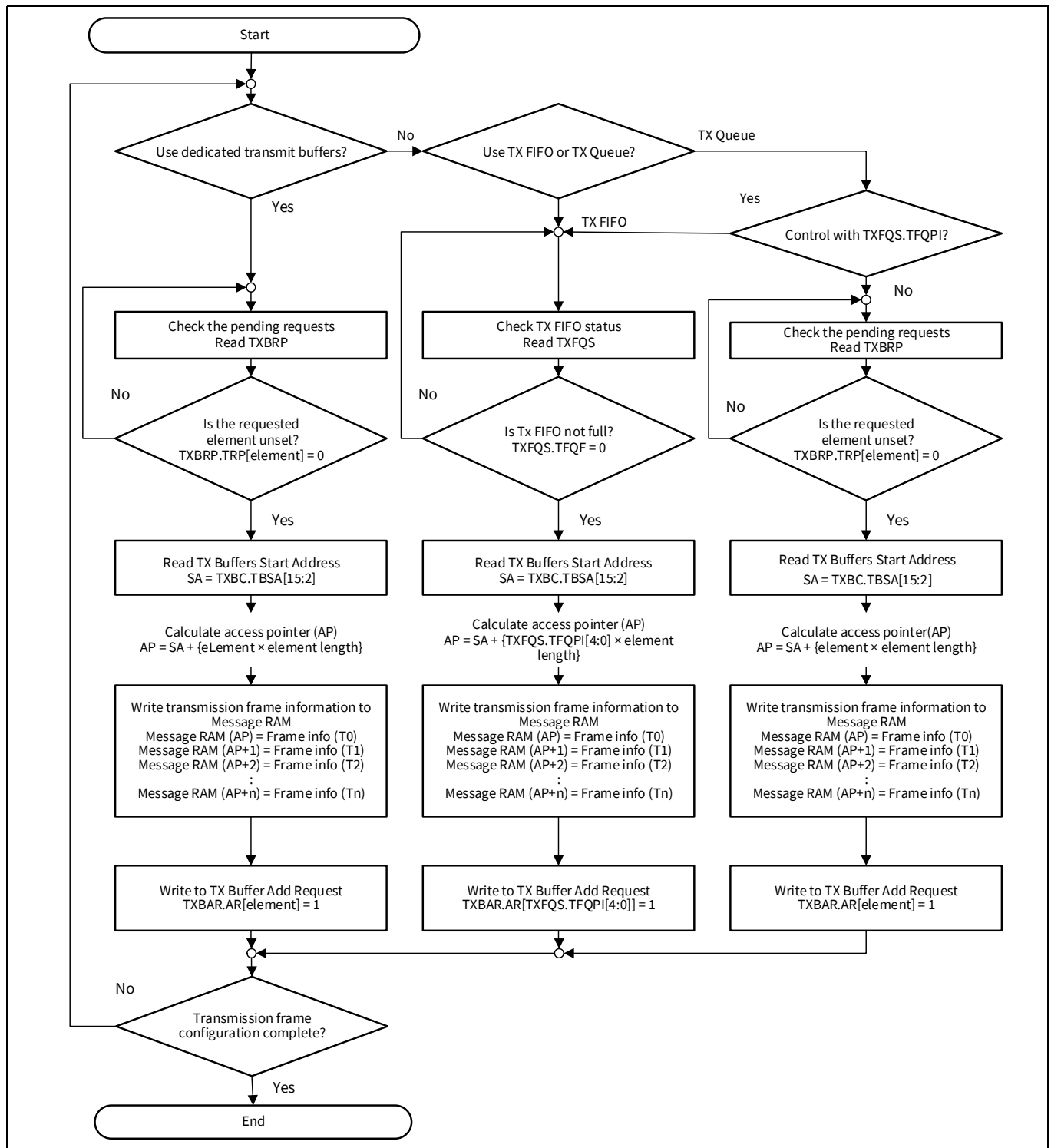
Figure 29-38. Transmit frame configuration
