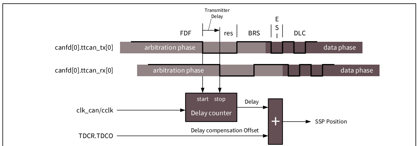
Figure 29-2. Transmitter delay measurement
