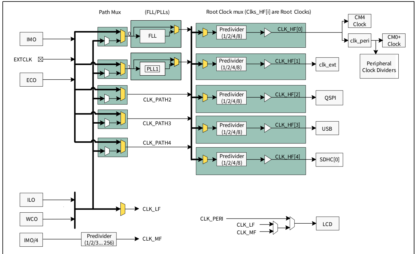
Figure 21-1. Clocking system block diagram
