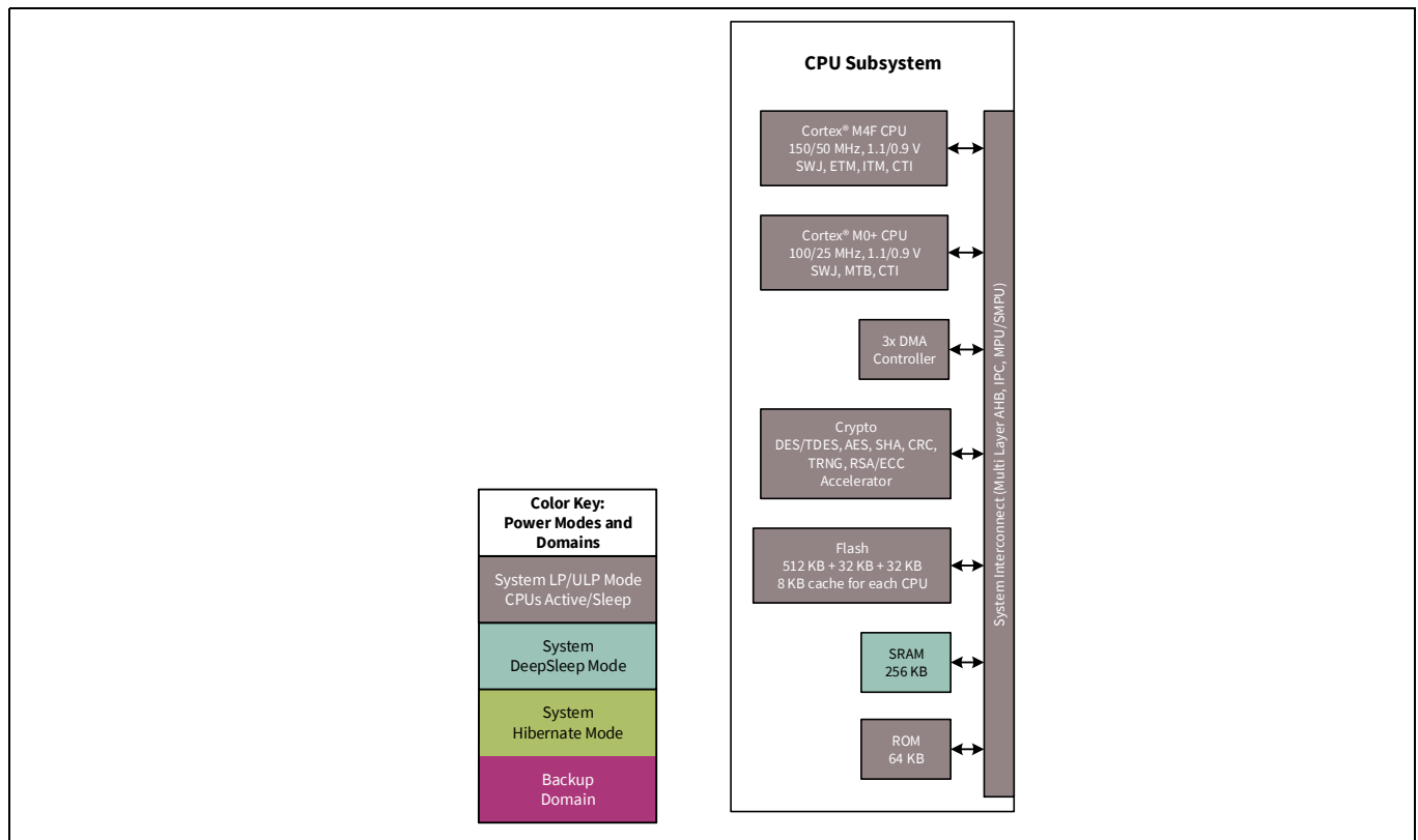
Figure 4-1. CPU subsystem block diagram
