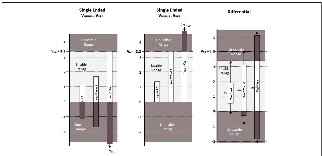
Figure 36-2. Input range
