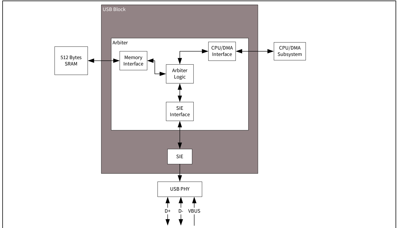
Figure 32-1. USB device block diagram
