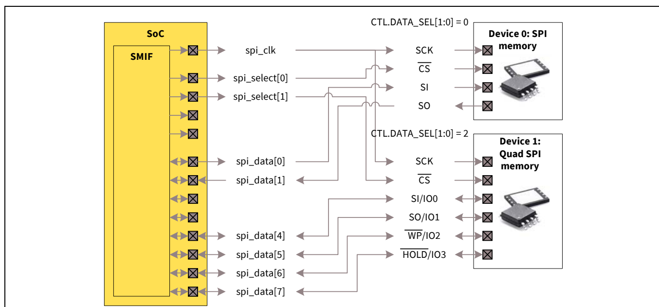
Figure 28-9. Single SPI memory 0 and Quad SPI memory 1 - Dedicated data signal
