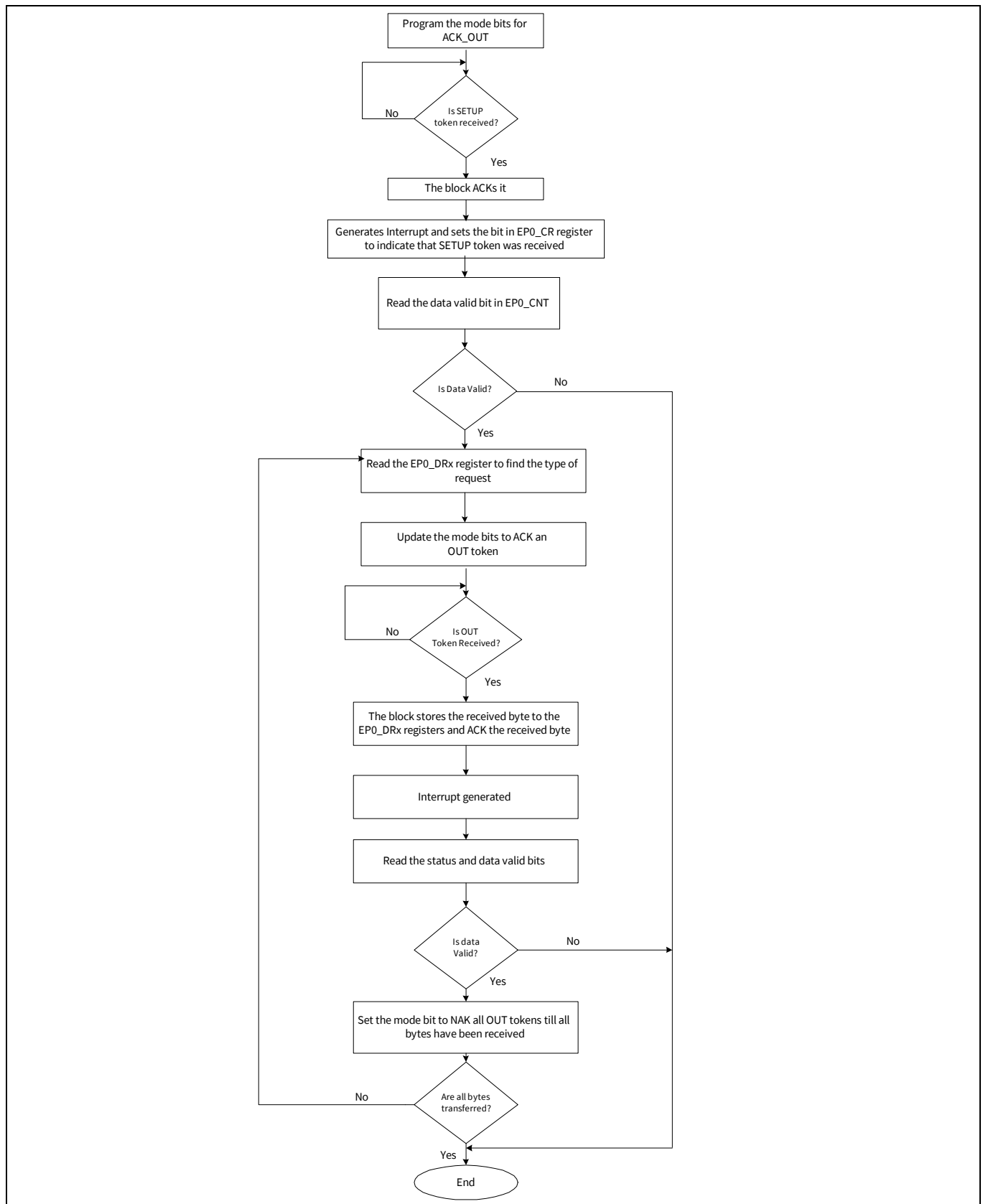
Figure 32-10. Control endpoint OUT transaction
