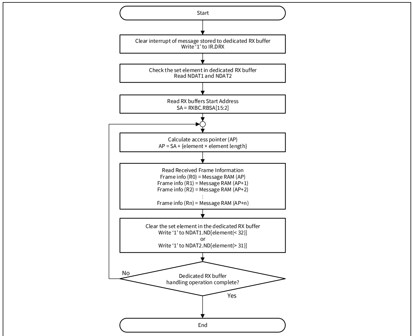
Figure 29-43. Dedicated RX buffer handling
