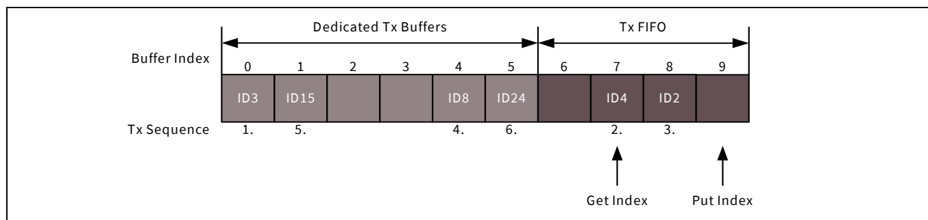
Figure 29-10. Example of mixed configuration dedicated TX buffers/TX FIFO
