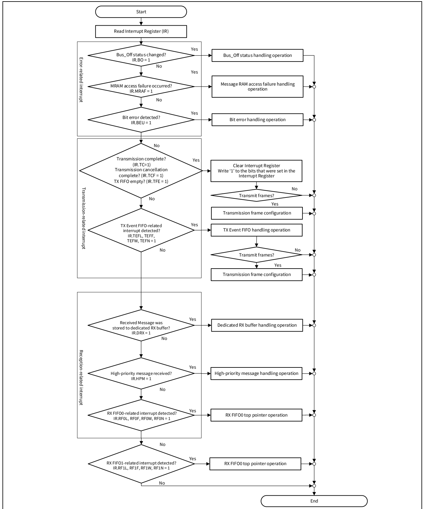
Figure 29-39. Interrupt handling
