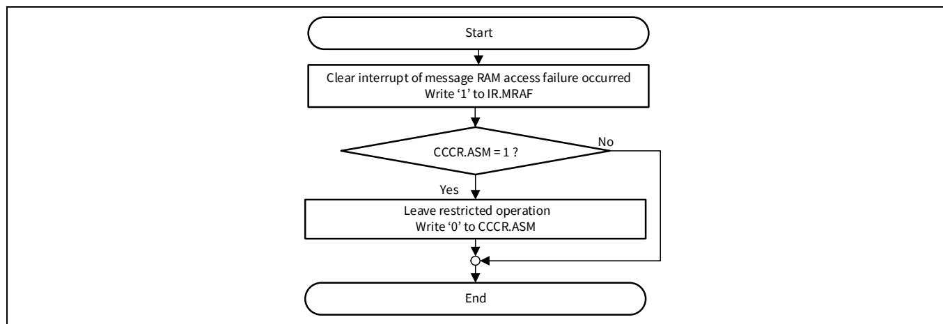
Figure 29-41. Message RAM access failure handling
