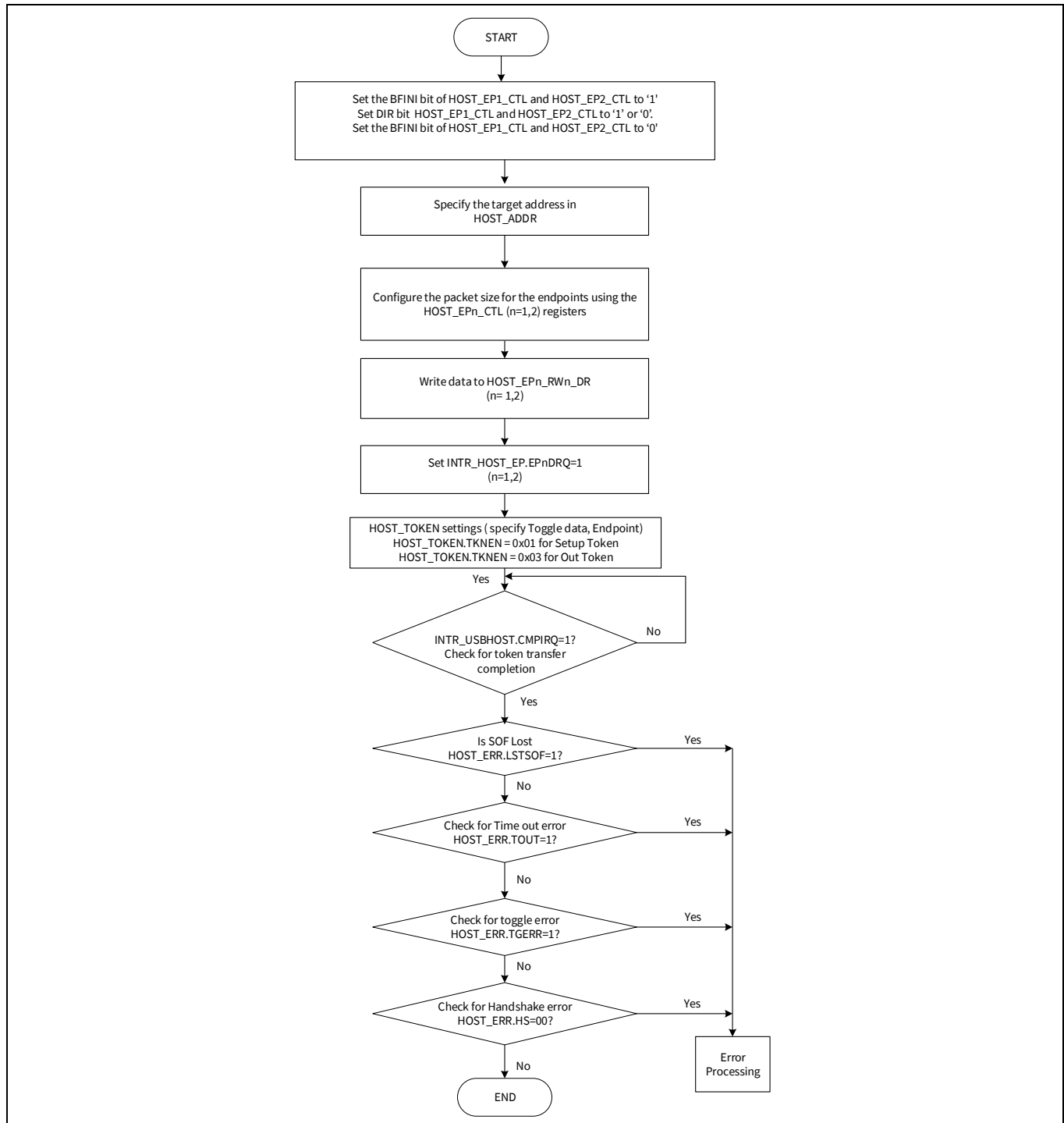
Figure 31-6. SETUP/OUT token flow chart
