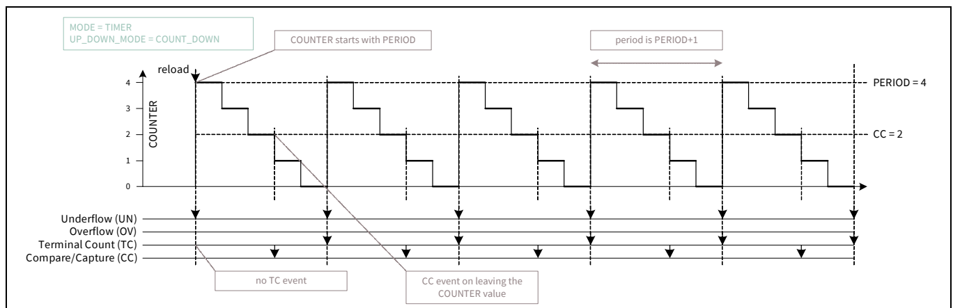
Figure 30-12. Timer in down-counting mode
