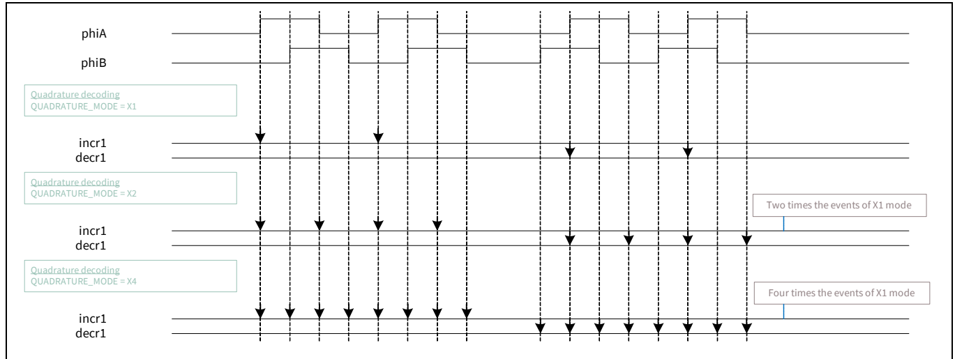
Figure 30-20. Quadrature mode waveforms
