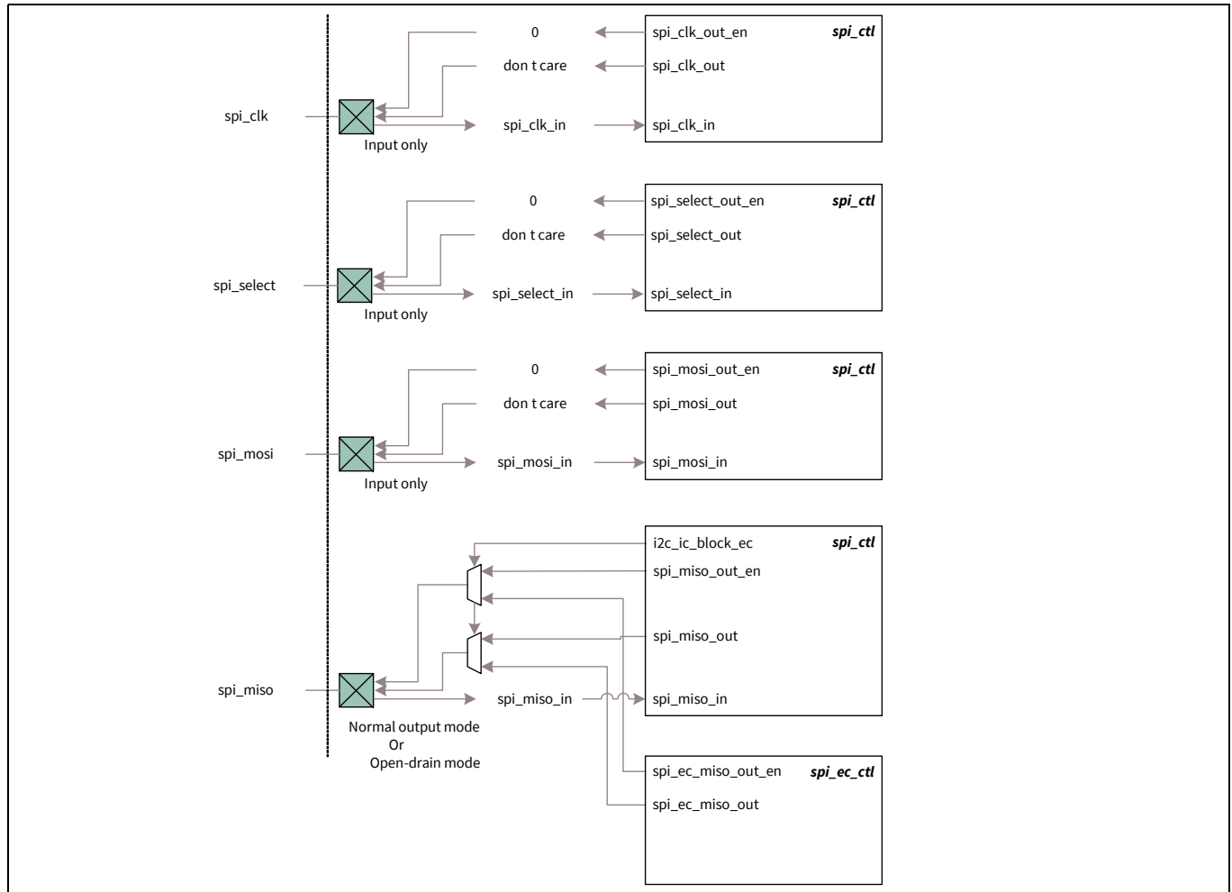
Figure 27-13. SPI slave I/O pad connections
