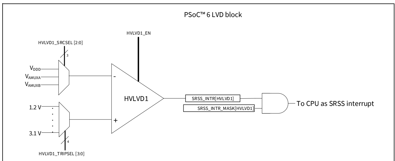
Figure 18-2. PSoC™ 6 MCU LVD block
