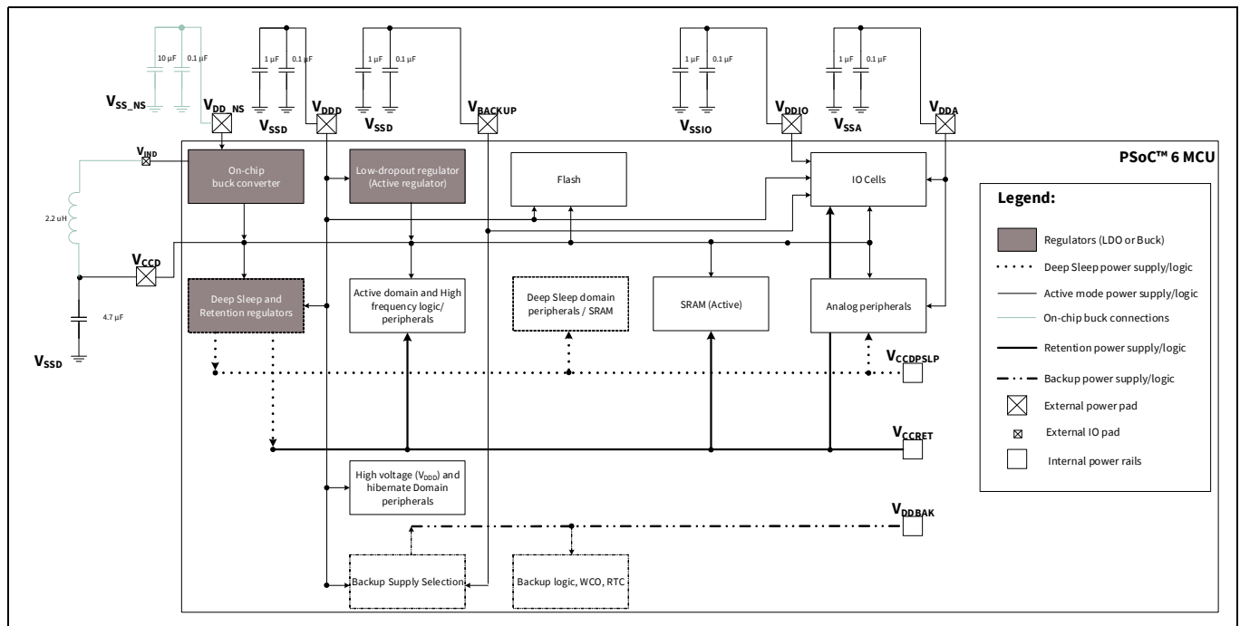
Figure 18-1. Power system block diagram
