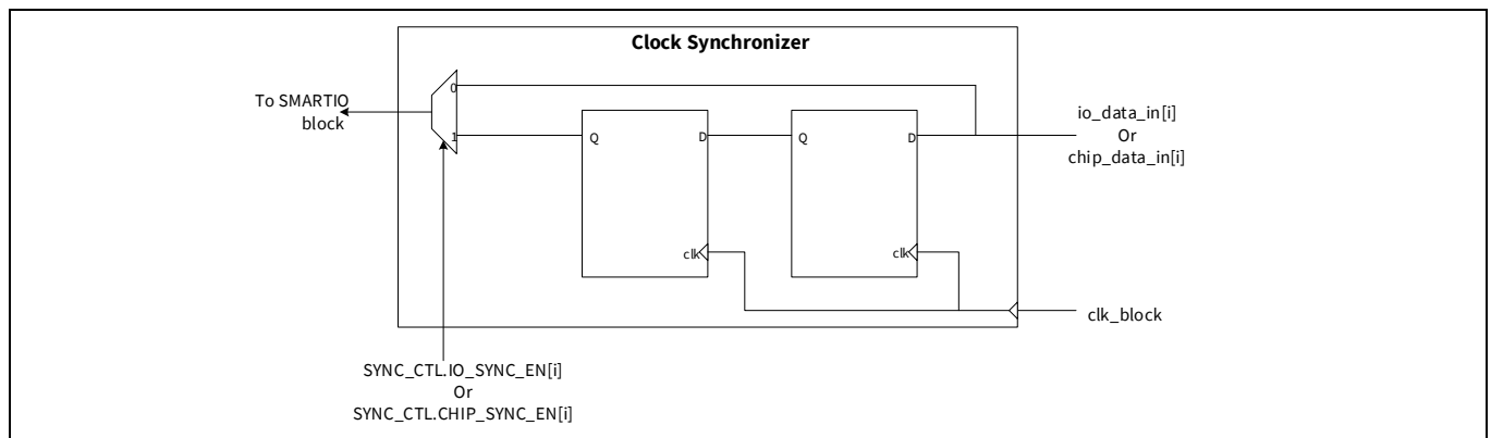
Figure 23-8. Smart I/O clock synchronizer
