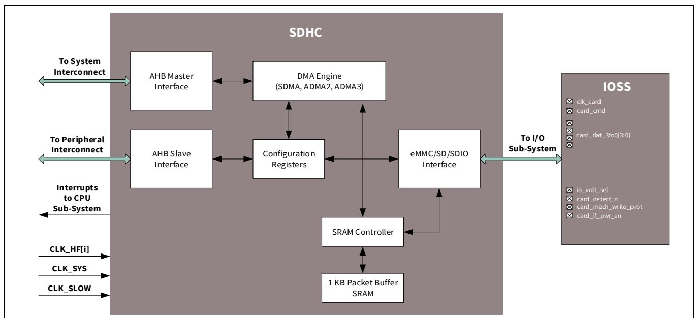
Figure 26-2. SDHC block diagram
