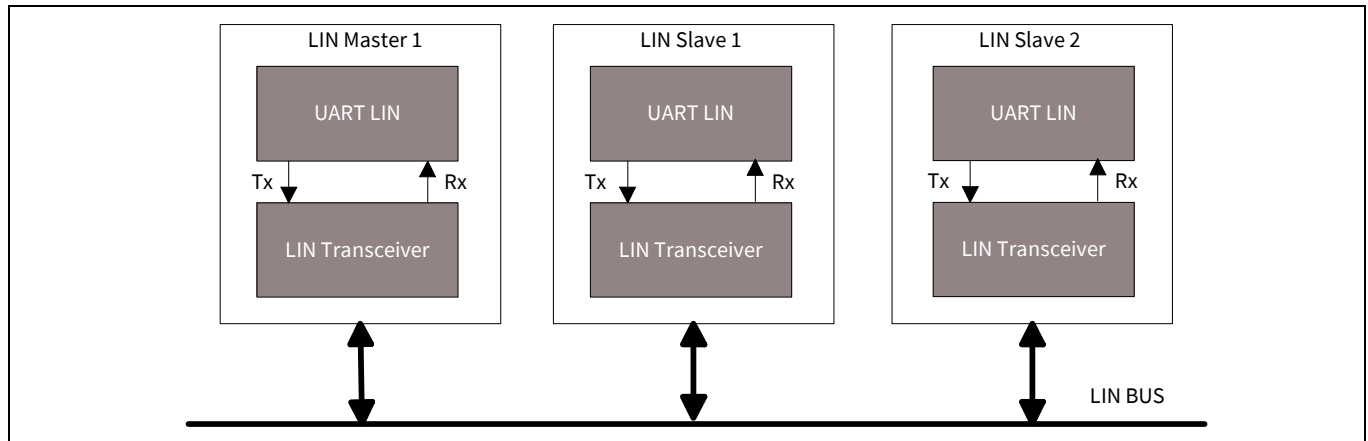
Figure 27-24. UART_LIN and LIN transceiver
