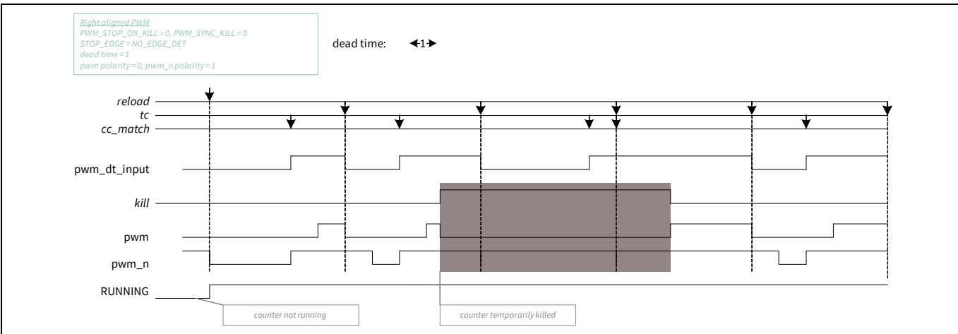
Figure 30-40. Dead time and kill
