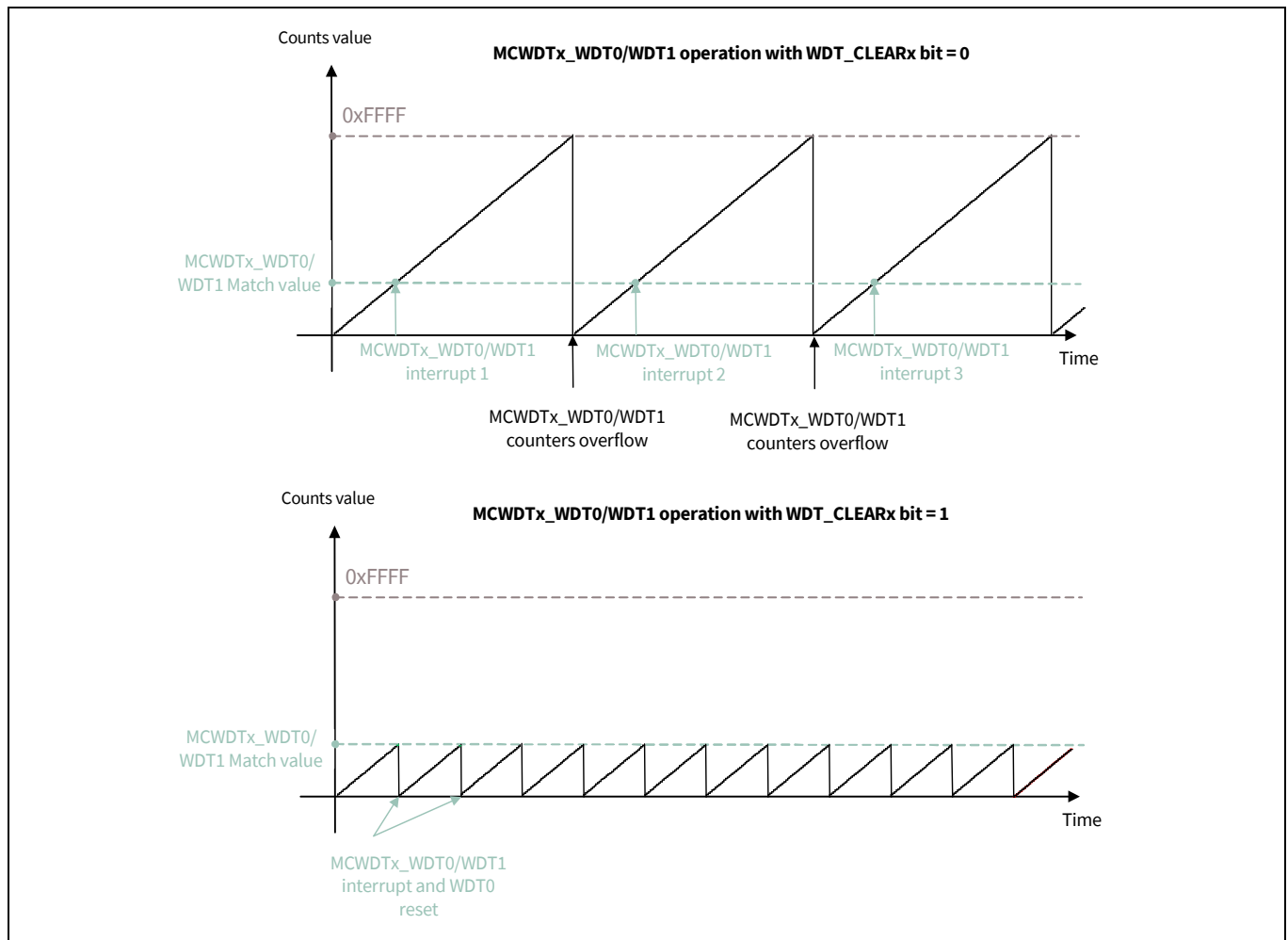
Figure 24-4. MCWDTx_WDT0/WDT1 operation
