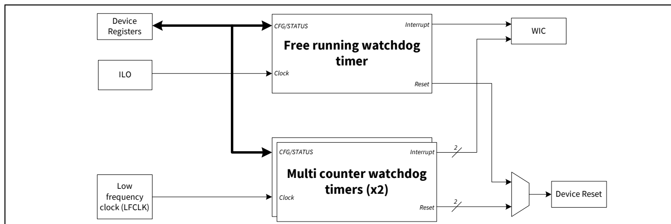
Figure 24-1. Watchdog timer block diagram
