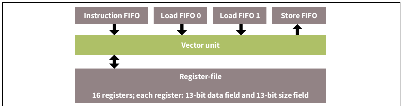
Figure 12-16. Vector unit
