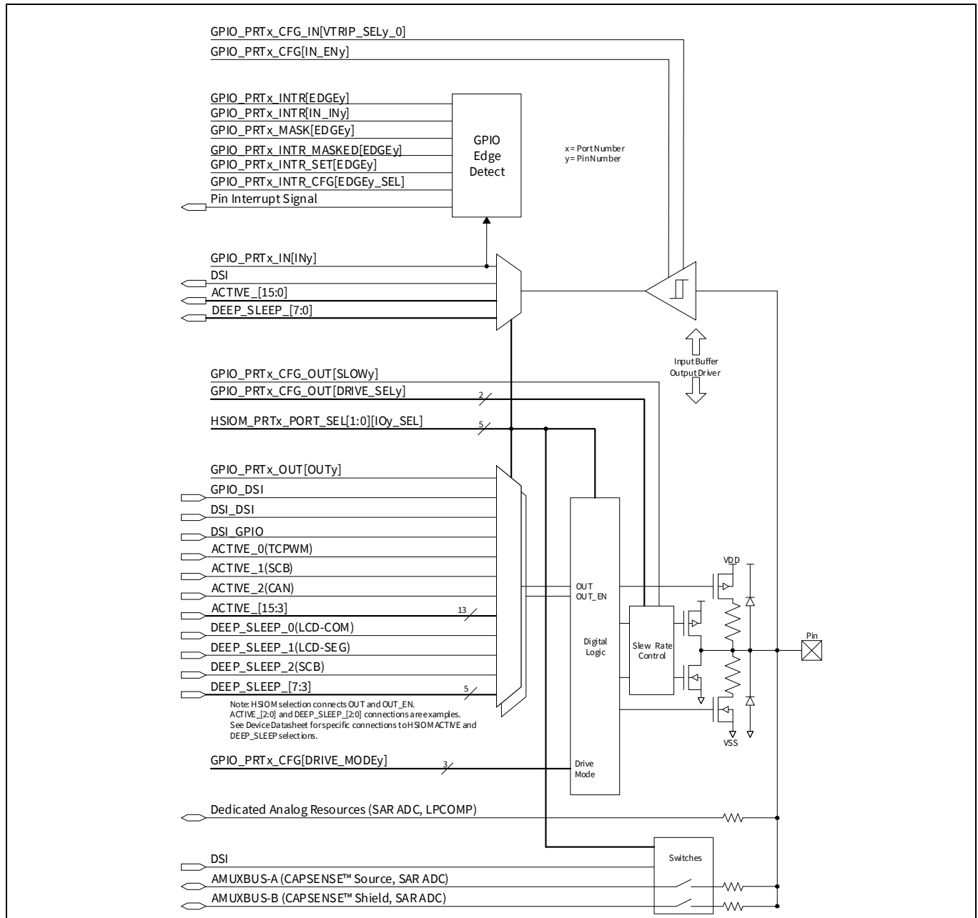
Figure 23-2. GPIO and GPIO_OVT cell architecture
