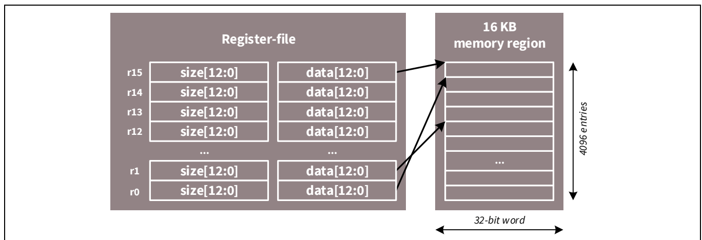
Figure 12-17. Register file
