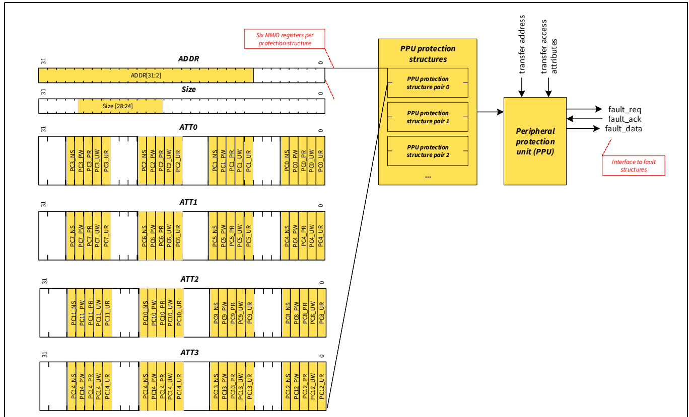
Figure 9-5. PPU functionality
