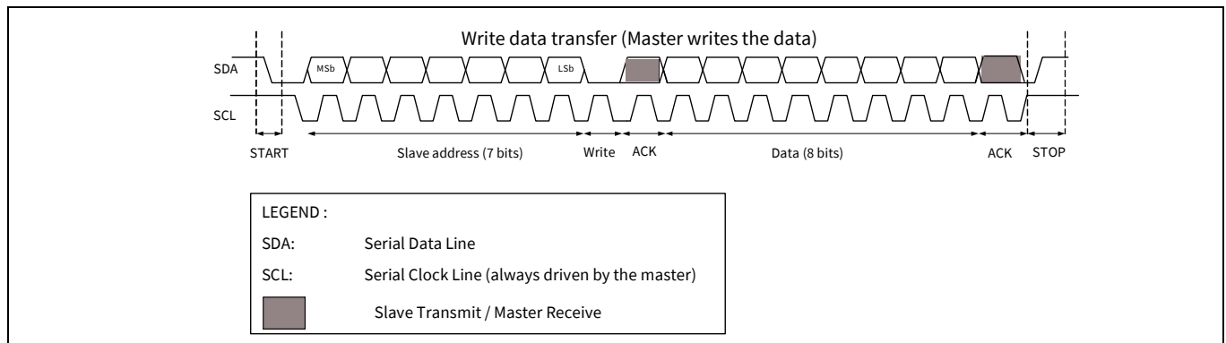
Figure 27-38. Master write data transfer
