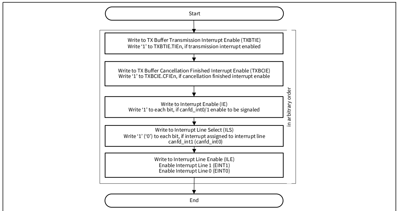
Figure 29-37. Interrupt configuration
