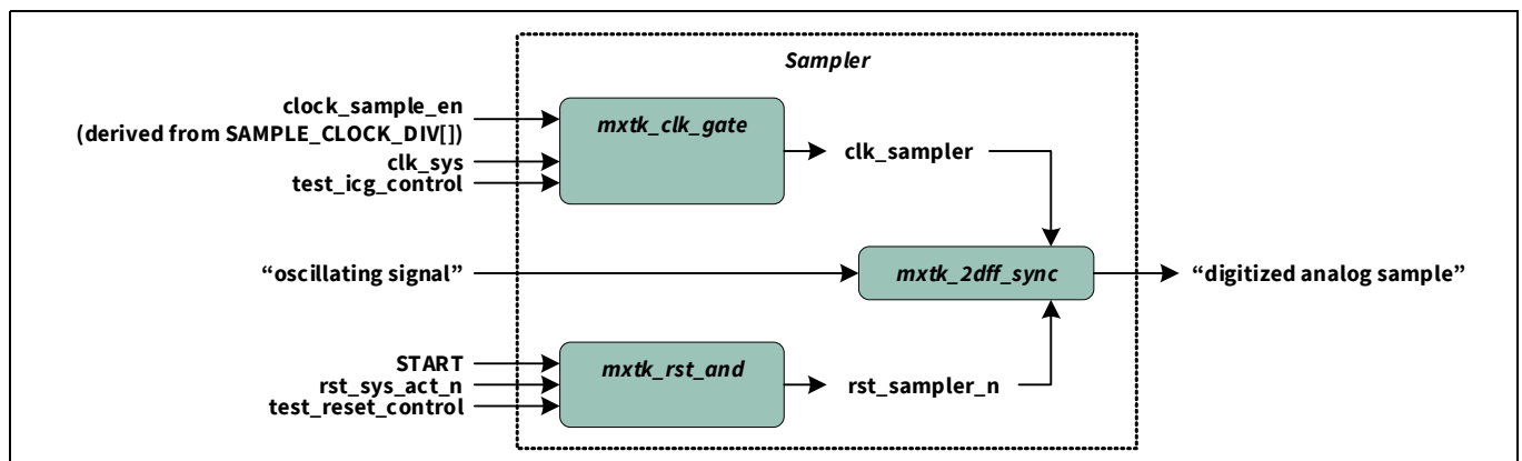
Figure 12-7. Sampler logic
