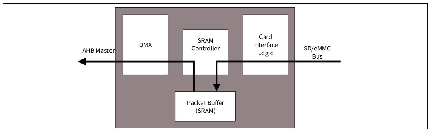
Figure 26-3. Data flow in a read transfer
