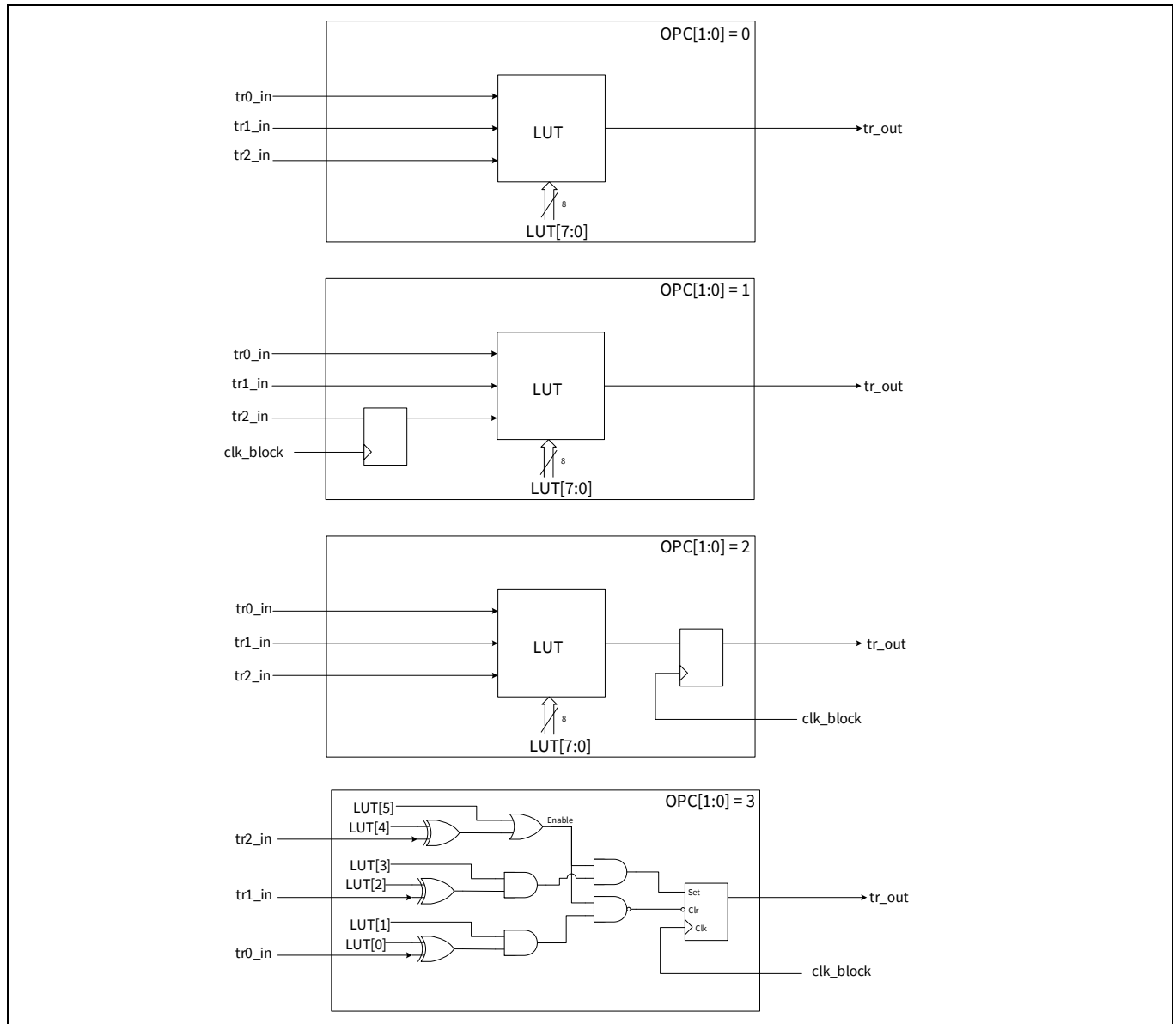
Figure 23-9. Smart I/O LUT configuration
