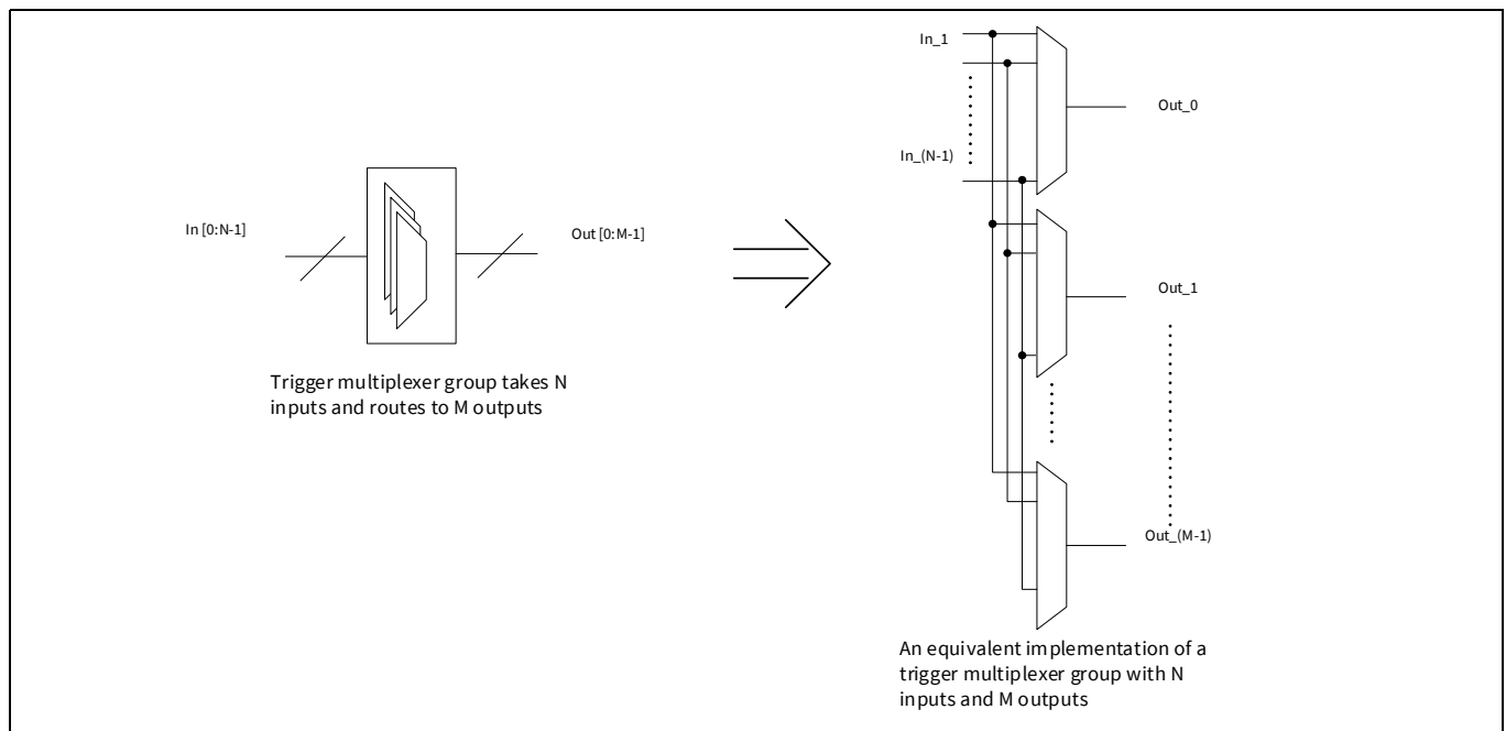
Figure 25-2. Trigger multiplexer groups
