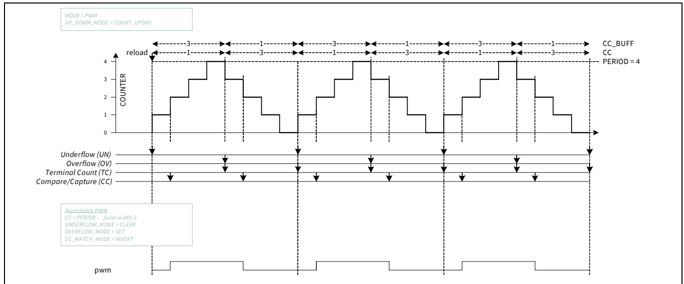
Figure 30-36. Asymmetric PWM
