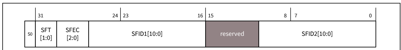
Figure 29-19. Standard Message ID filter
