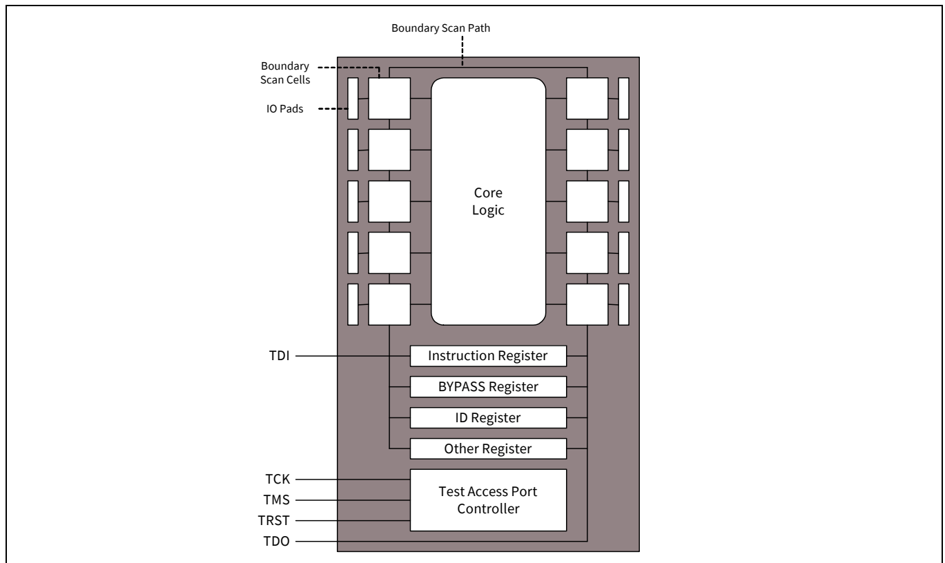
Figure 13-4. JTAG interface architecture
