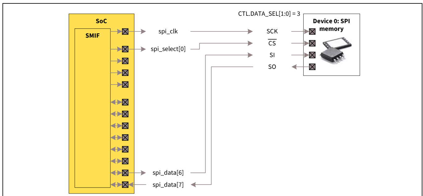
Figure 28-5. Single SPI memory device 0 connected to spi_data[7:6]
