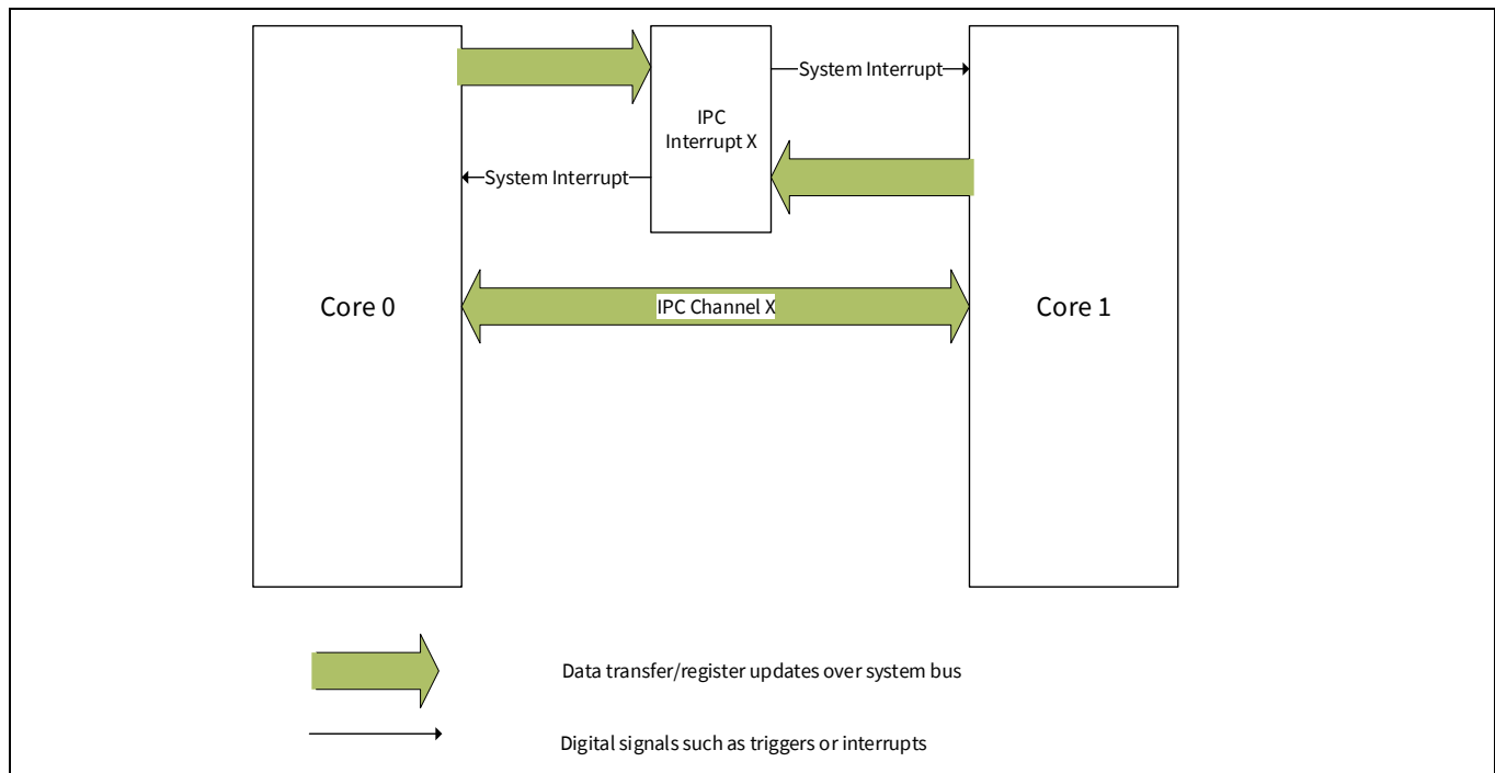
Figure 6-9. Half duplex with shared event handling
