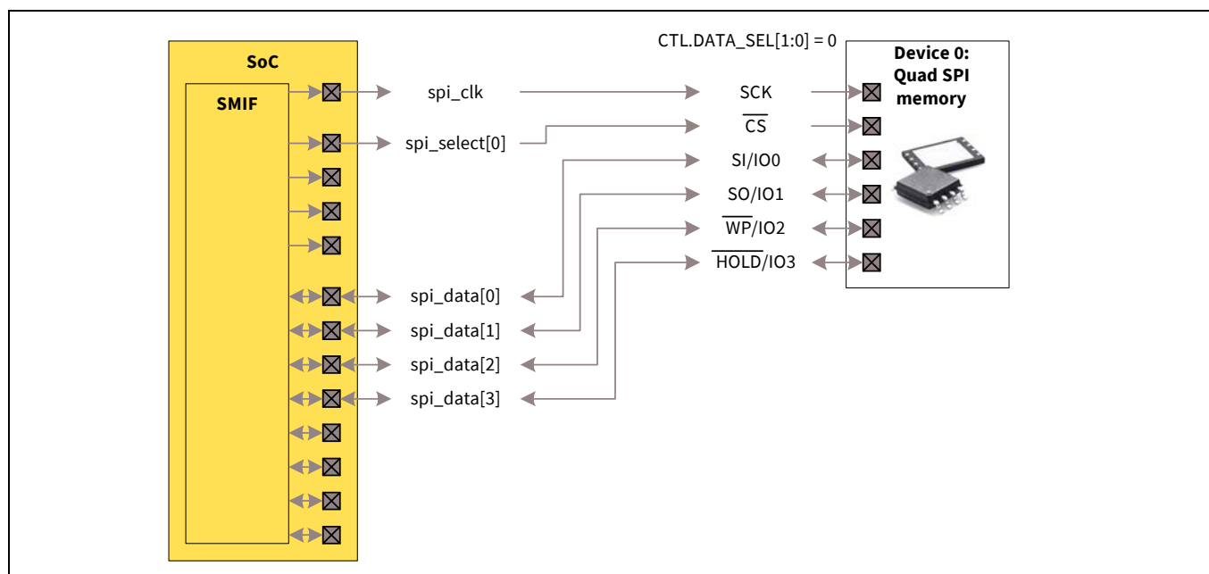
Figure 28-8. Quad SPI memory device 0
