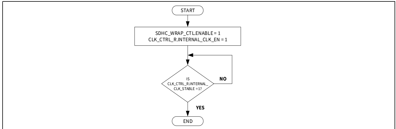
Figure 26-6. SDHC enable sequence
