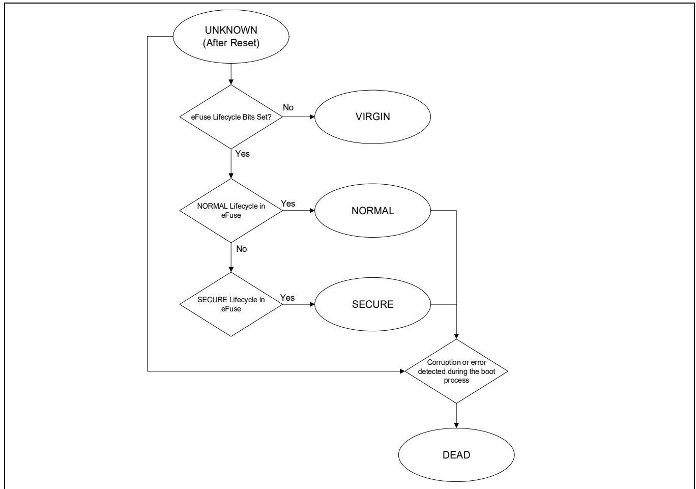
Figure 17-2. Protection state transitions
