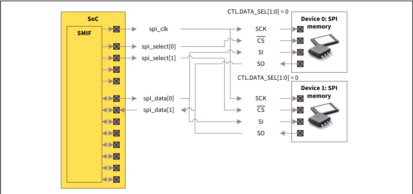
Figure 28-7. Single SPI memory devices 0 and 1 - Shared data signal
