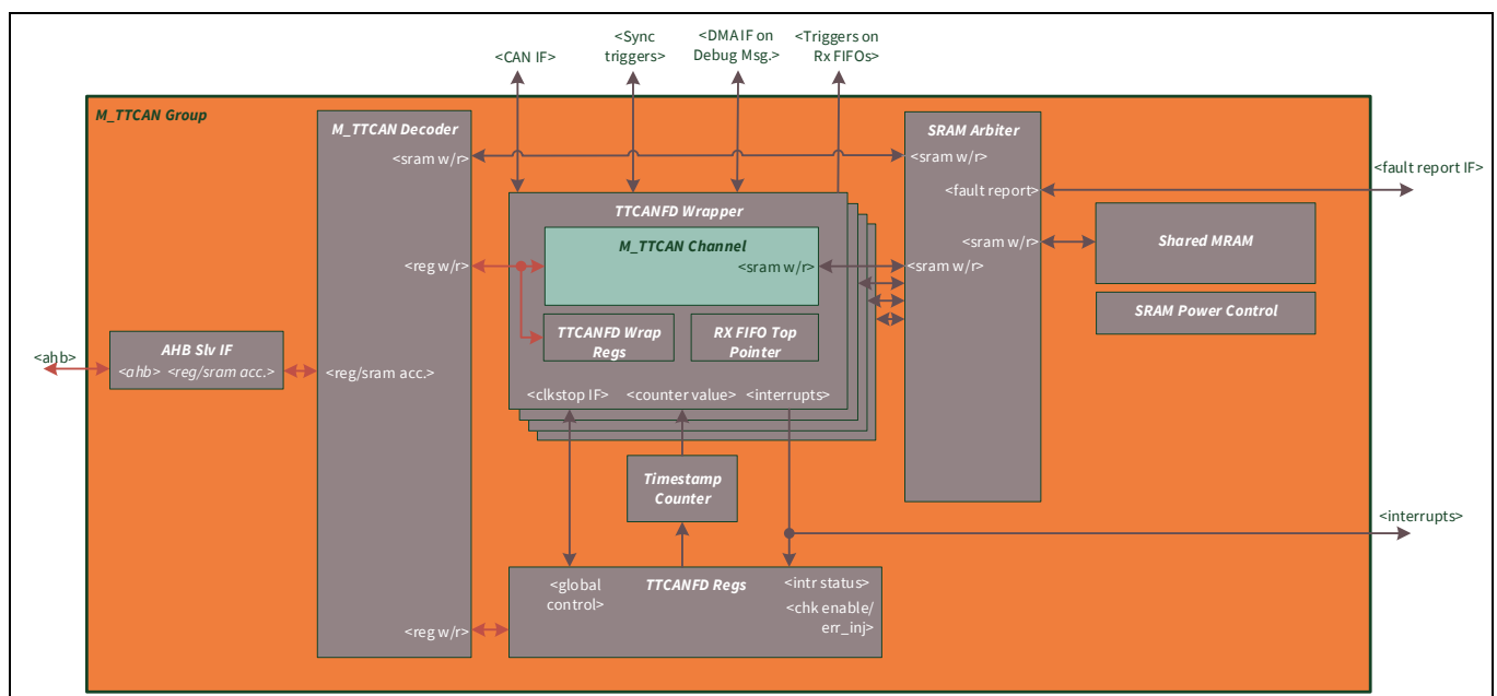
Figure 29-1. M_TTCAN block diagram
