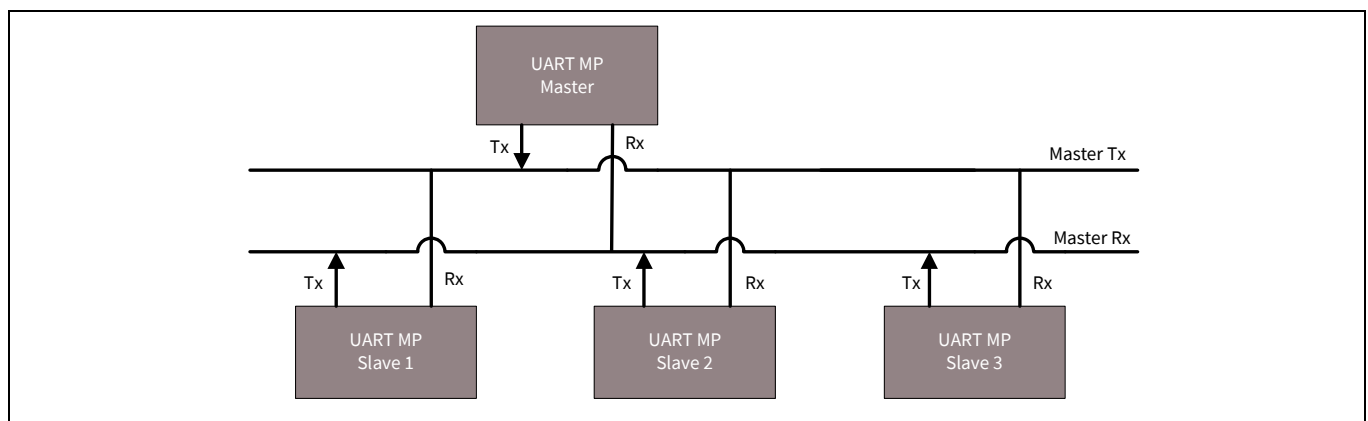
Figure 27-22. UART MP mode bus connections
