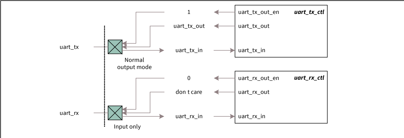
Figure 27-32. Standard UART mode I/O pad connections
