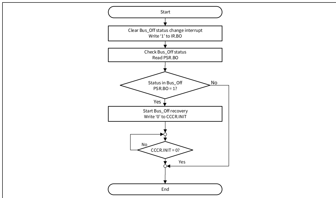
Figure 29-40. Bus OFF error handling
