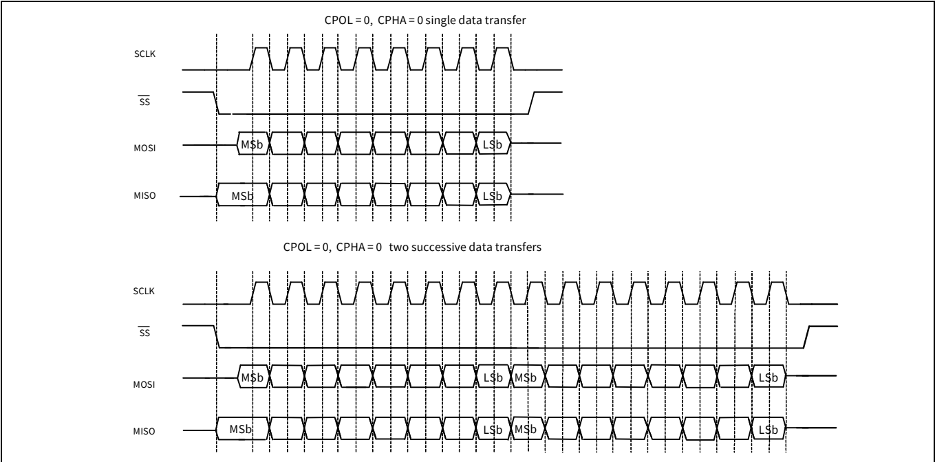
Figure 27-3. SPI Motorola data transfer example
