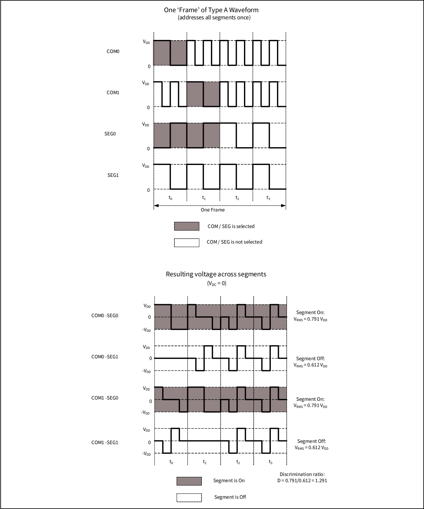
Figure 33-6. Digital correlation Type-A waveform
