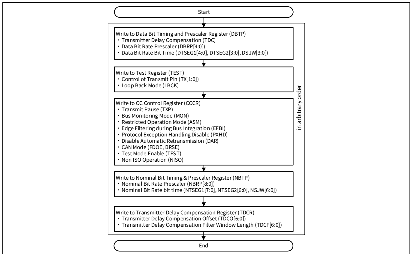
Figure 29-31. Configuration required for CAN bus
