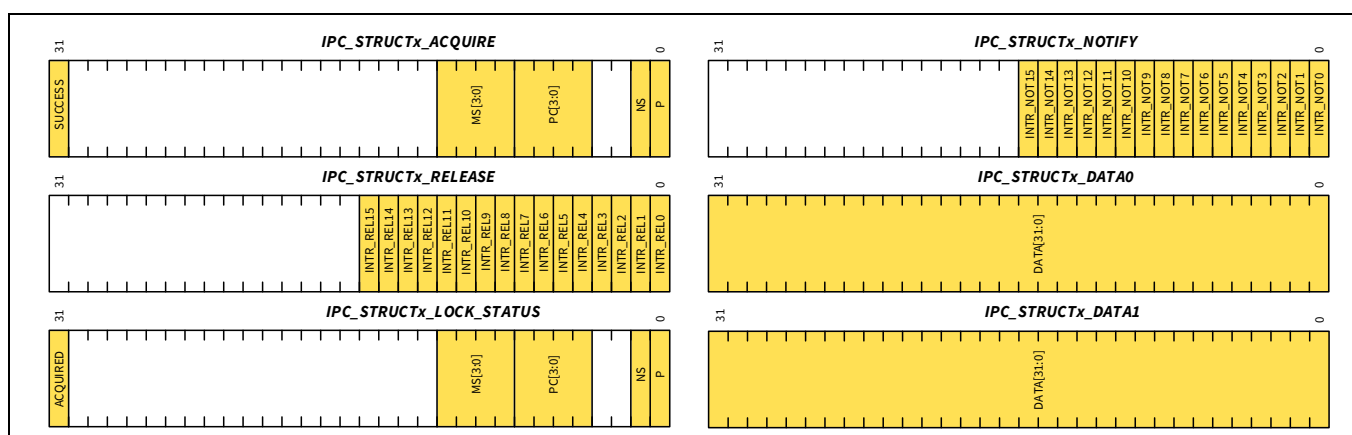
Figure 6-2. IPC channel structure
