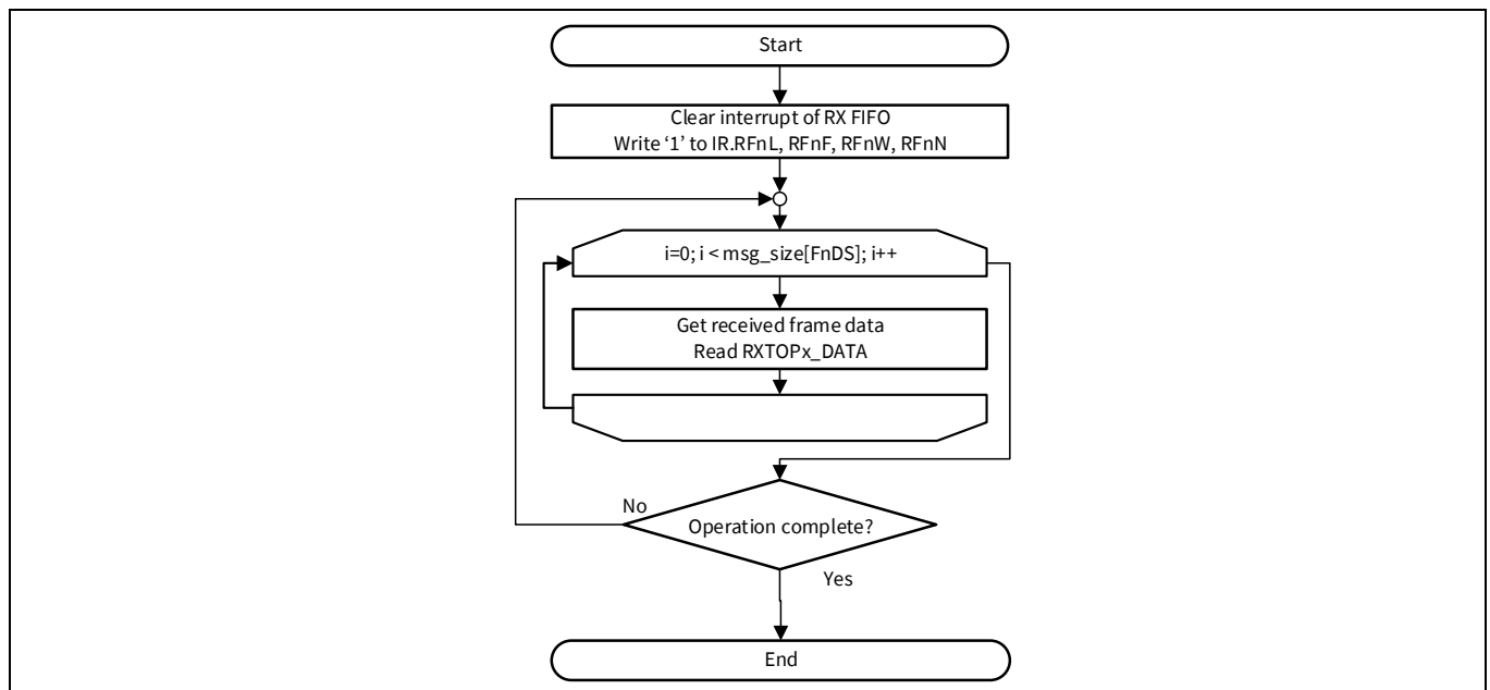
Figure 29-45. RX FIFO top pointer handling
