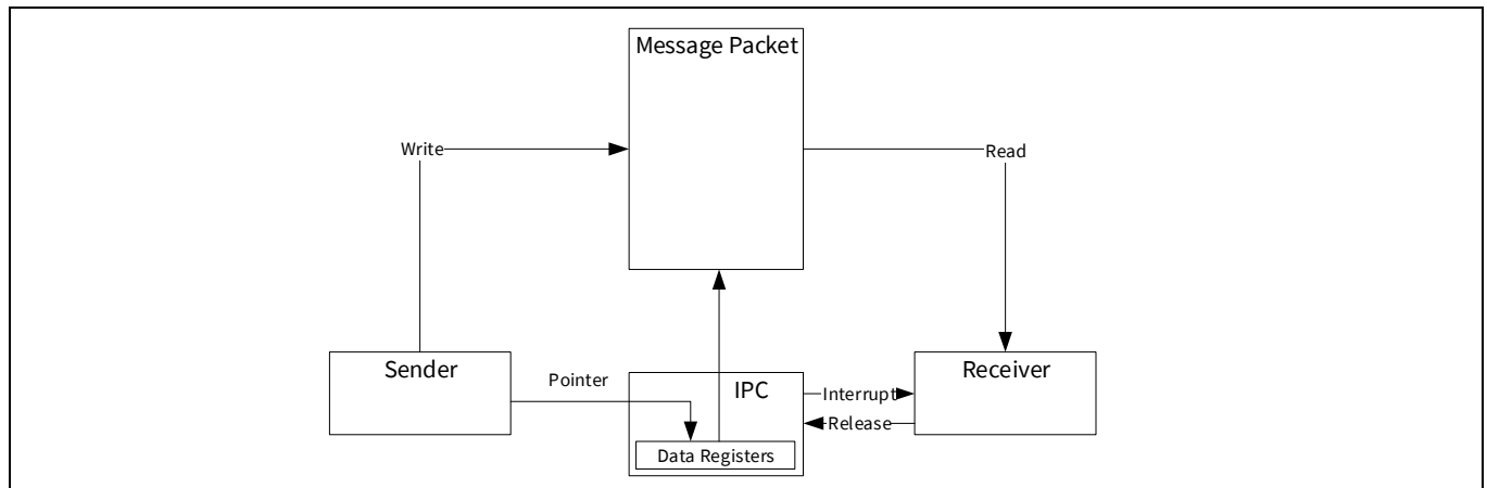
Figure 6-6. Communicating larger messages
