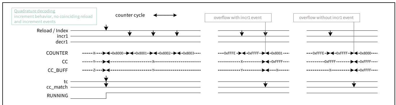
Figure 30-21. Quadrature mode reload/index timing
