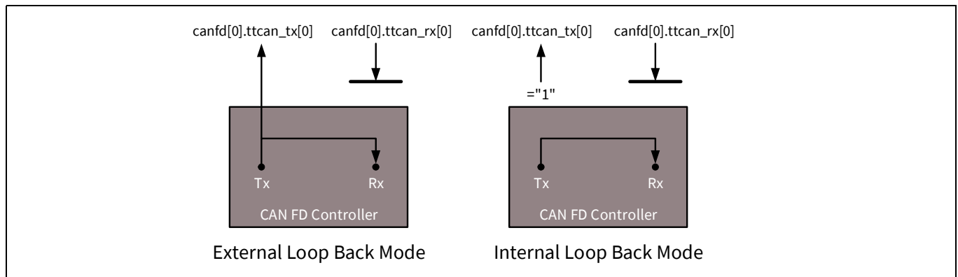
Figure 29-4. Pin control in Loop Back modes
