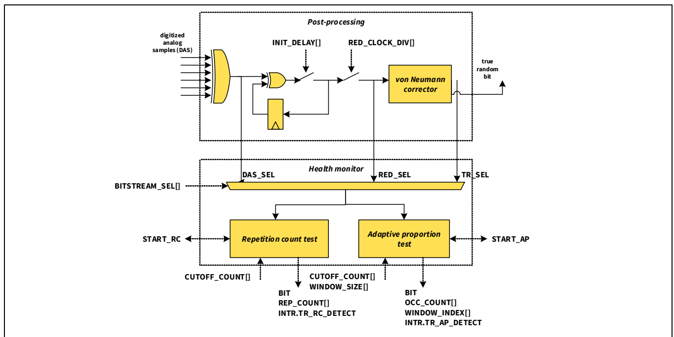
Figure 12-15. Health monitor functionality
