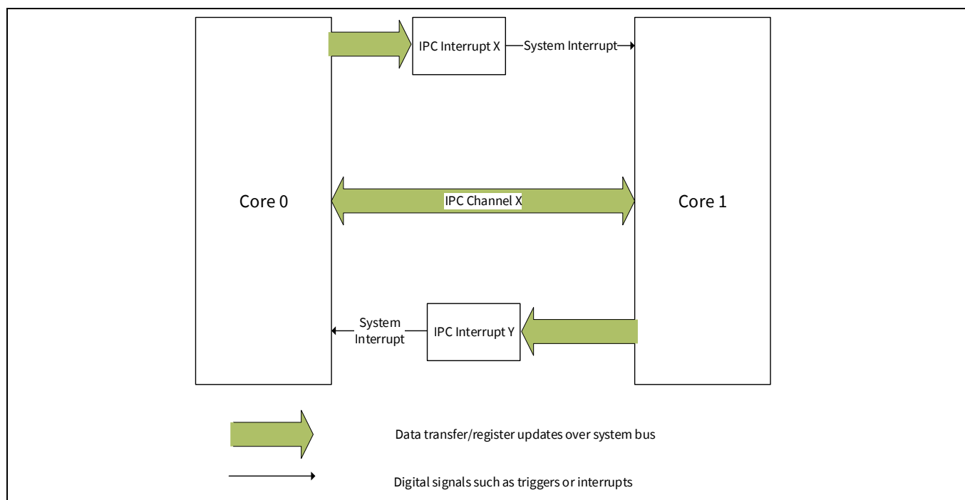
Figure 6-8. Half duplex with independent event handling
