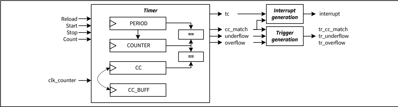
Figure 30-6. Timer functionality
