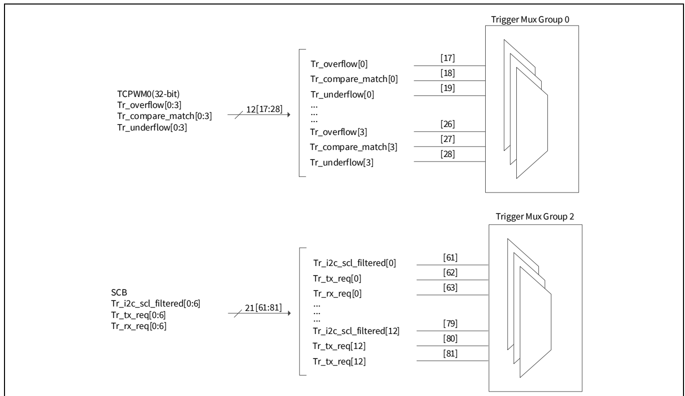
Figure 25-4. TCPWM and multiplexer SCB input layout
