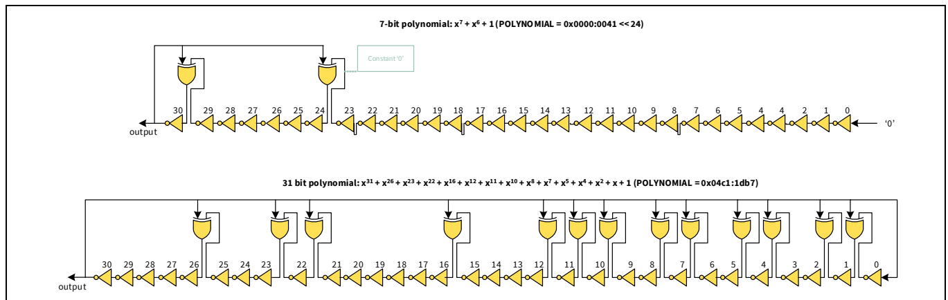
Figure 12-11. GARO31 – Two examples
