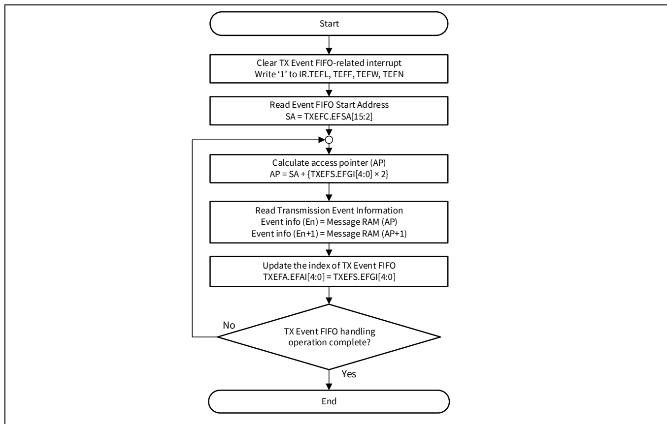
Figure 29-42. TX event FIFO handling
