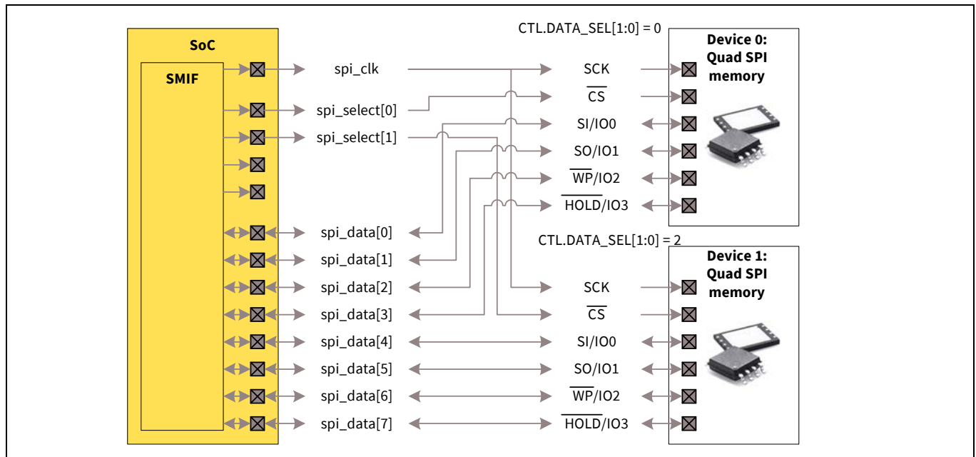
Figure 28-11. Quad SPI memory devices 0 and 1
