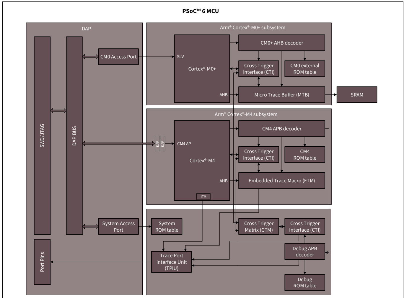
Figure 13-1. Program and debug interface
