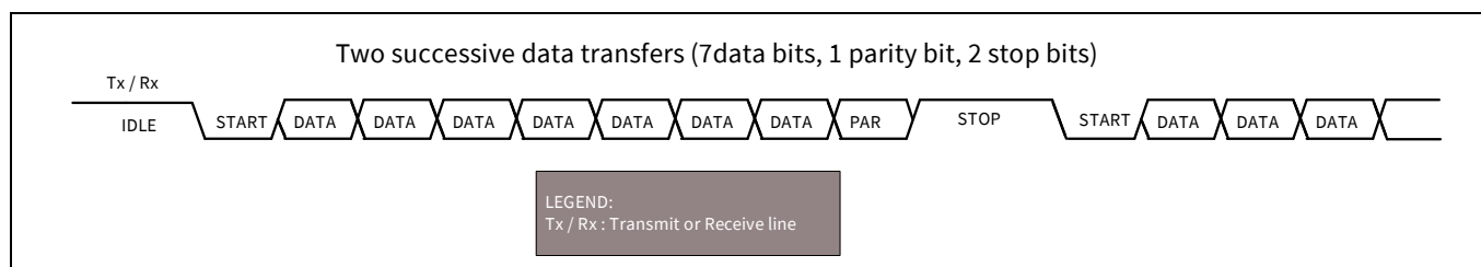
Figure 27-15. UART, standard protocol example
