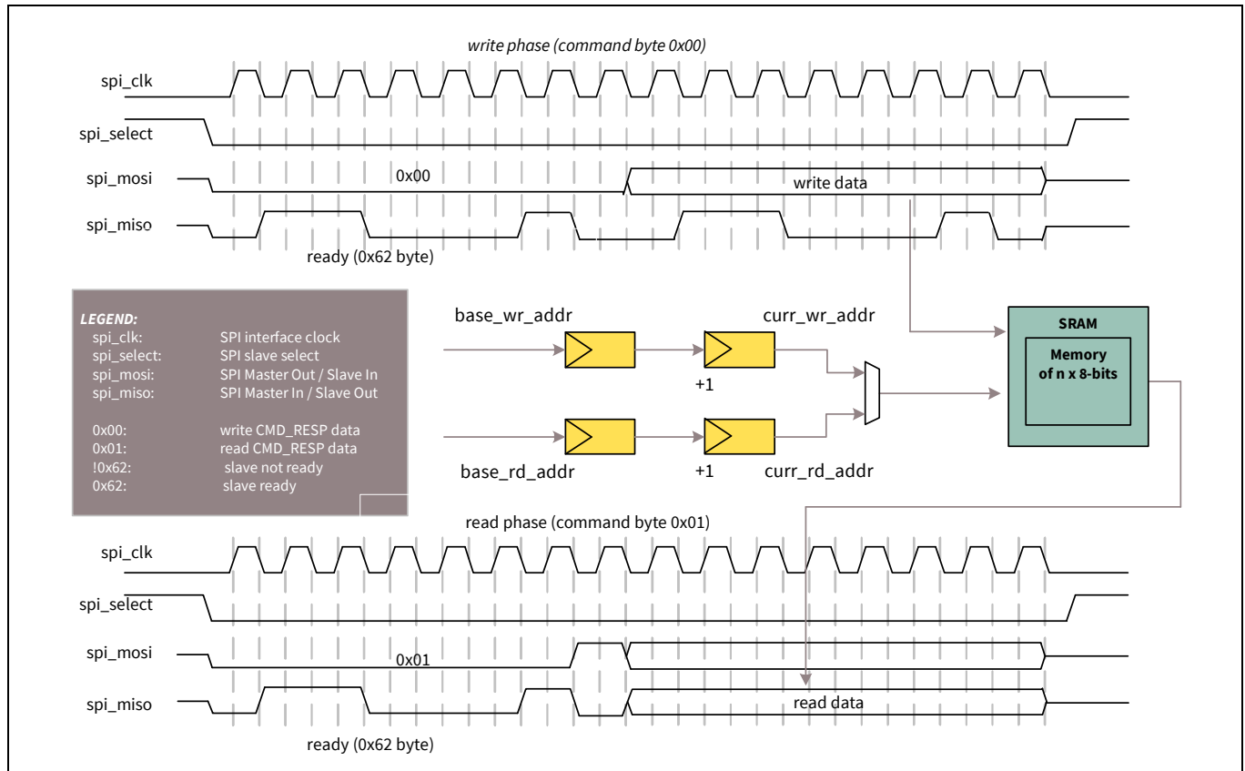
Figure 27-10. Command-response mode example
