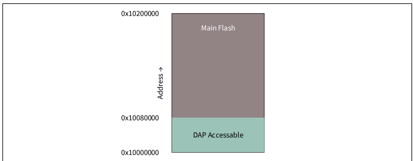
Figure 15-2. FLASH_ALLOWED with encoding “4”
