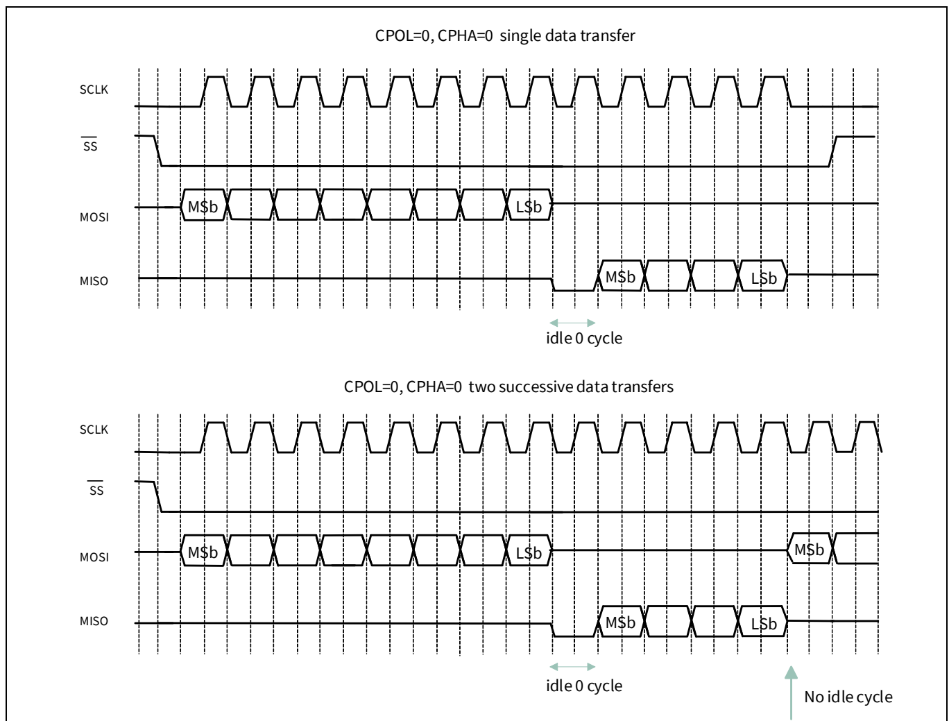
Figure 27-7. SPI NS data transfer example
