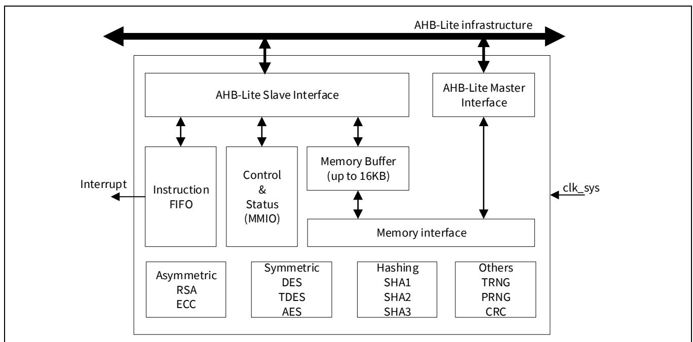
Figure 12-1. Crypto block diagram
