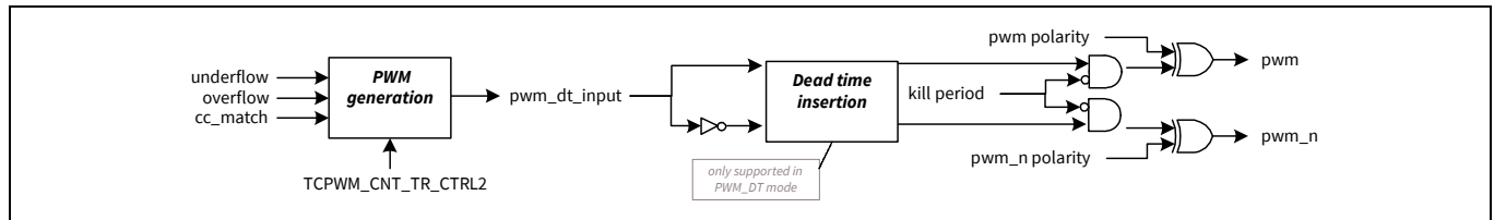
Figure 30-24. PWM output generation
