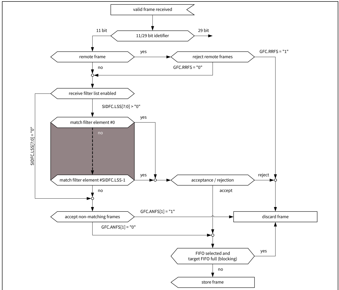
Figure 29-5. Standard Message ID filter
