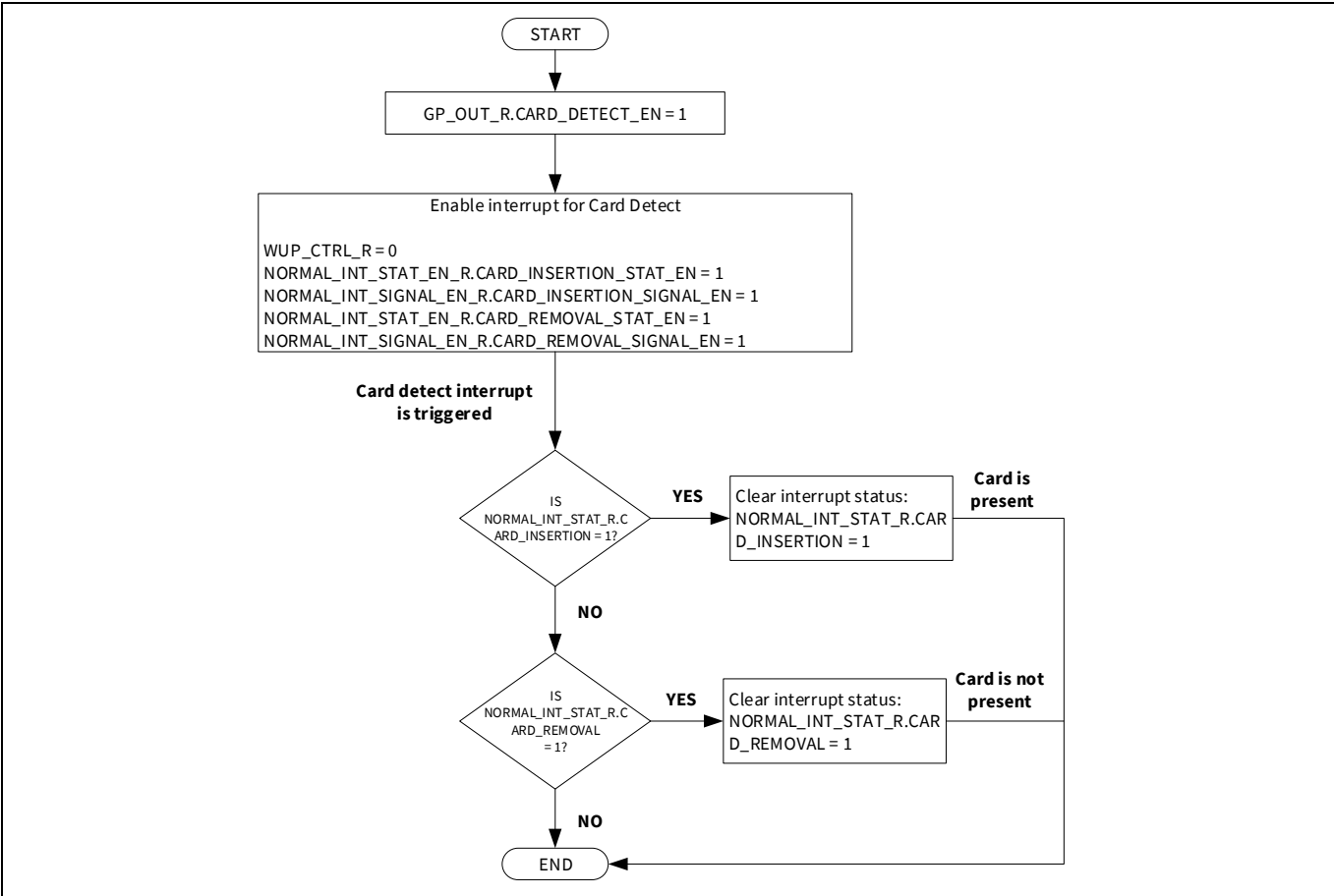
Figure 26-8. Card detection through interrupt
