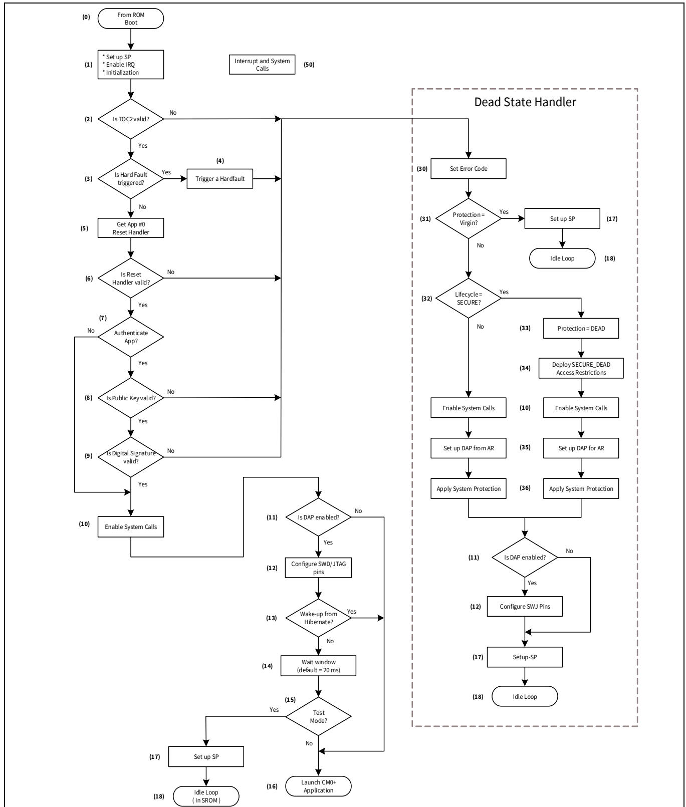
Figure 15-5. Flash boot flow chart
