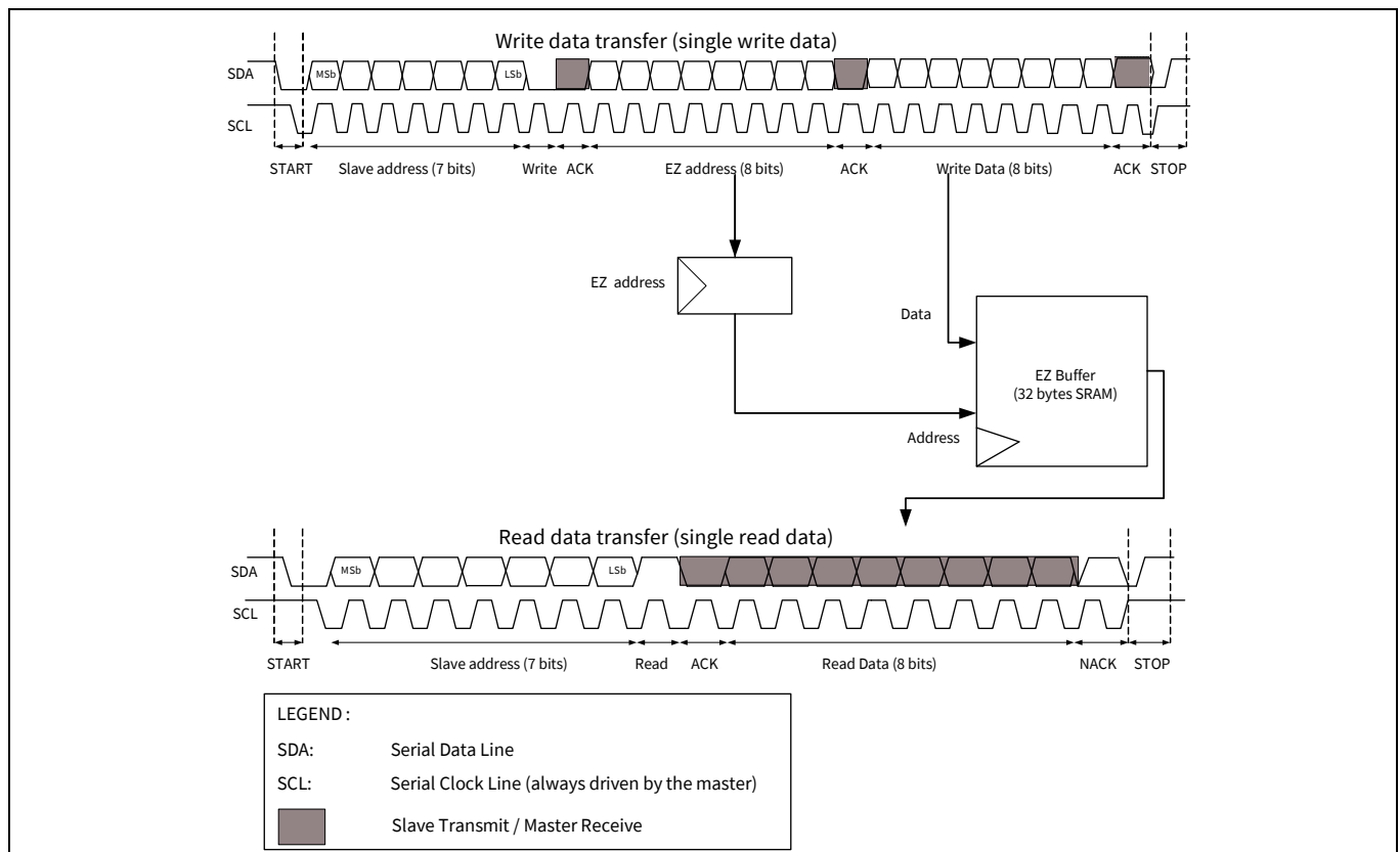
Figure 27-40. EZI2C write and read data transfer
