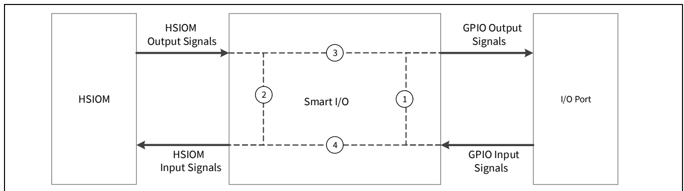
Figure 23-7. Smart I/O interface
