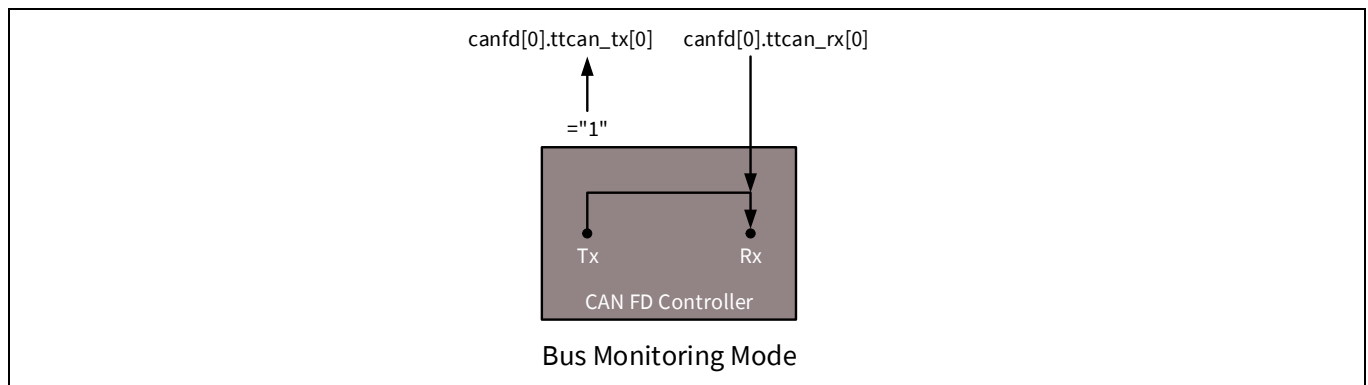
Figure 29-3. Pin Control in Bus Monitoring mode
