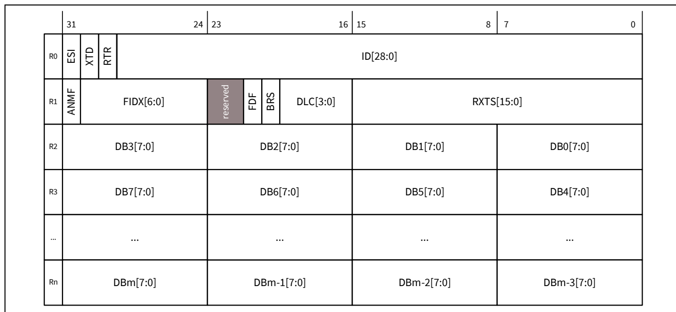
Figure 29-16. RX buffer and FIFO
