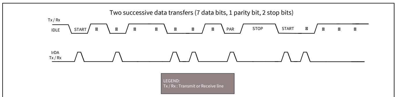
Figure 27-31. IrDA example
