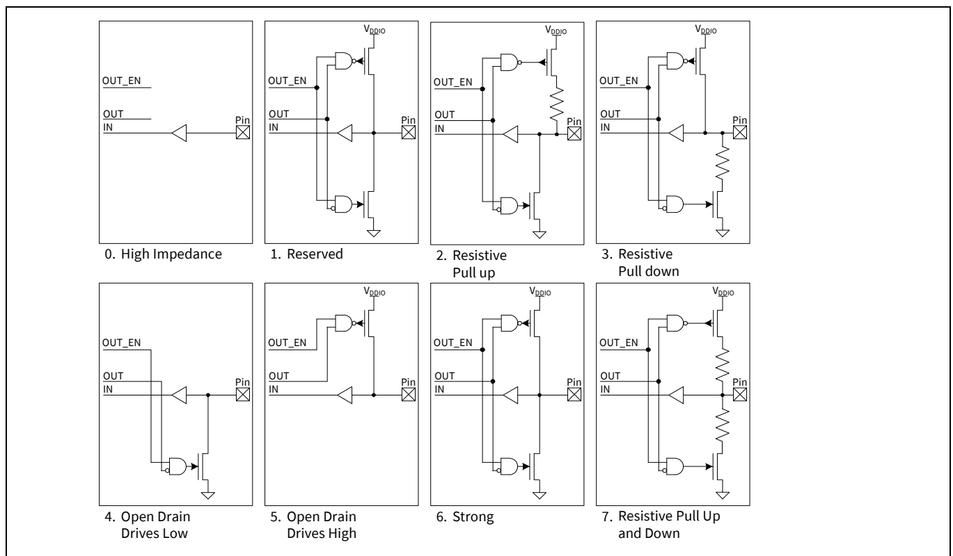
Figure 23-3. CPU and DSI/UDB I/O drive mode block diagram
