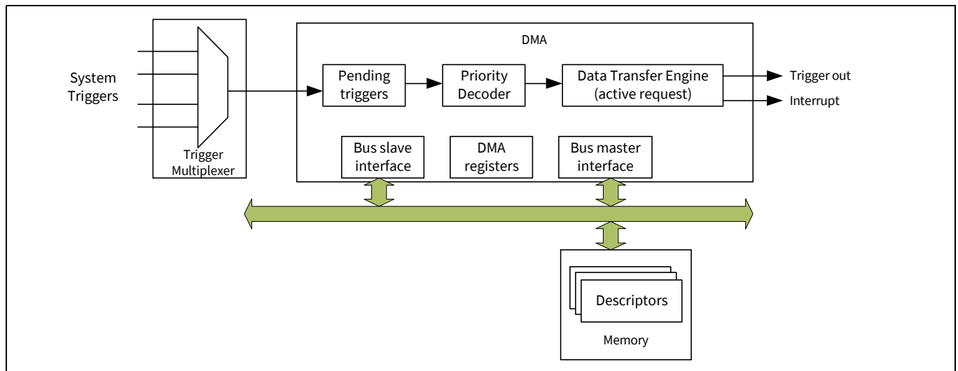
Figure 10-1. DMA controller
