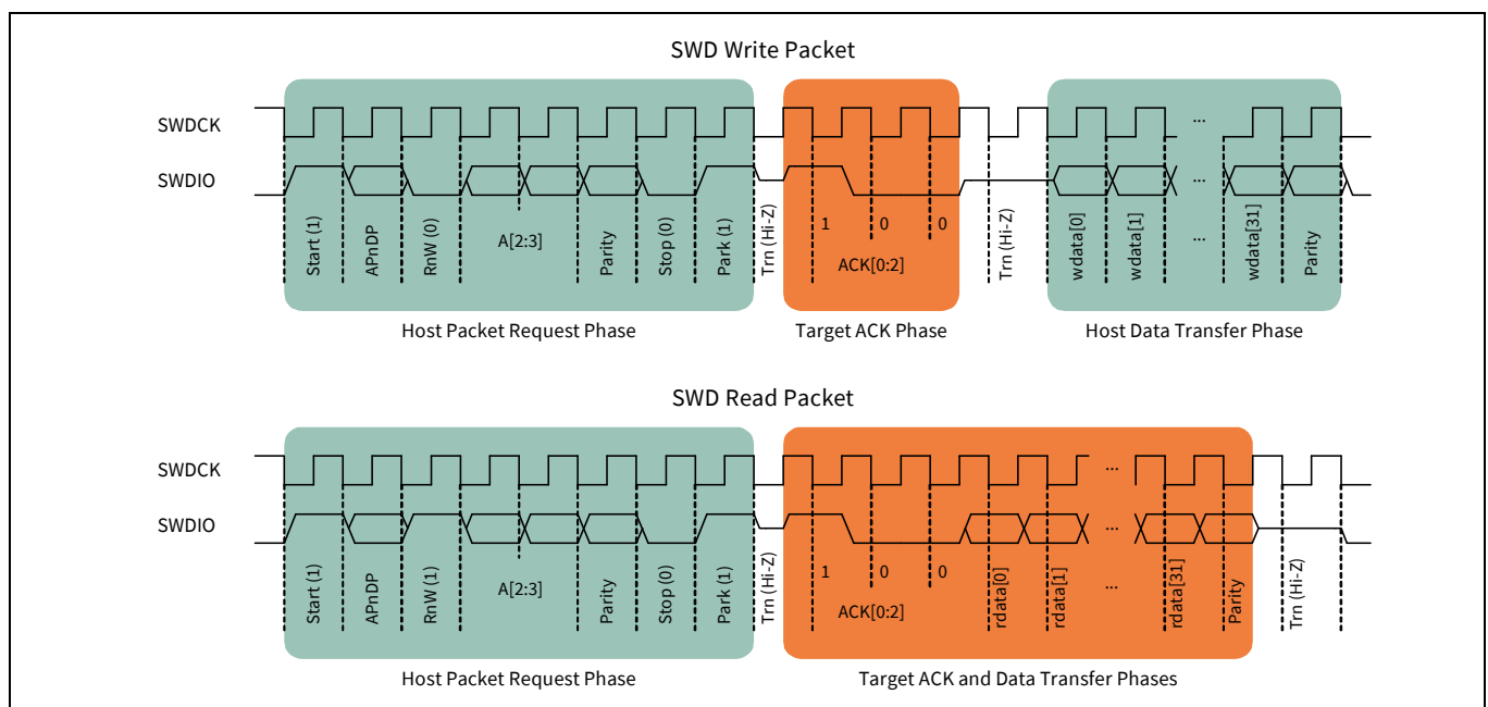
Figure 13-2. SWD write and read packet timing diagrams
