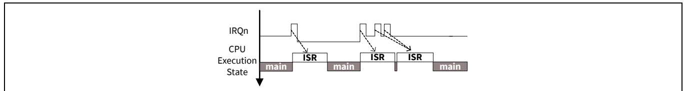
Figure 8-4. Pulse interrupts
