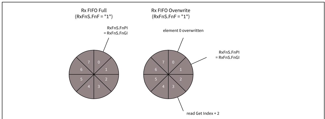
Figure 29-8. RX FIFO overflow handling
