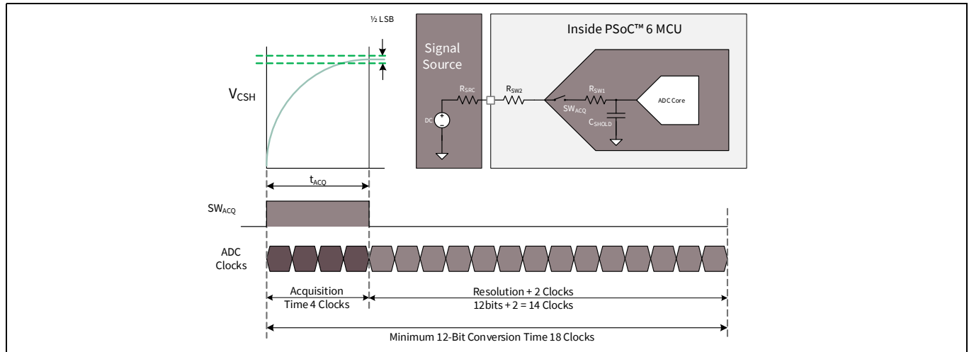
Figure 36-3. Acquisition time
