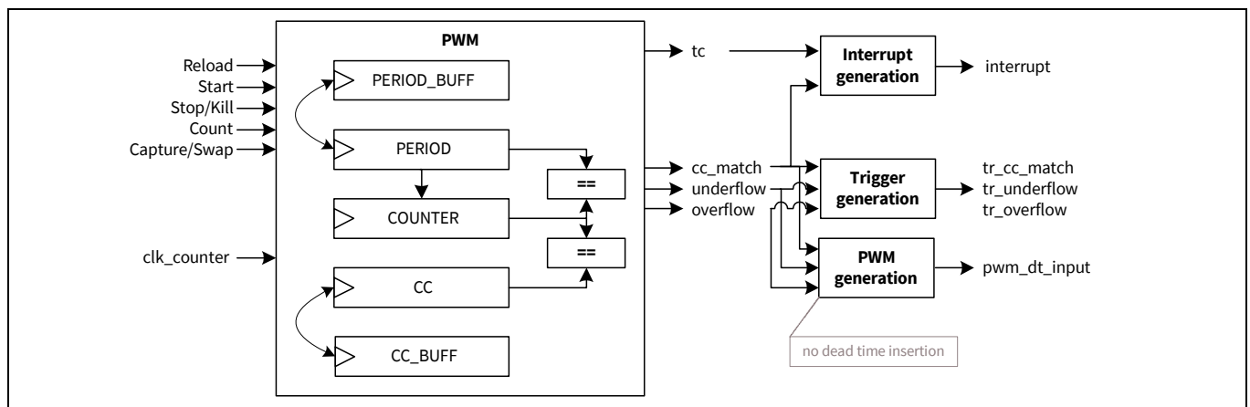
Figure 30-23. PWM mode functionality
