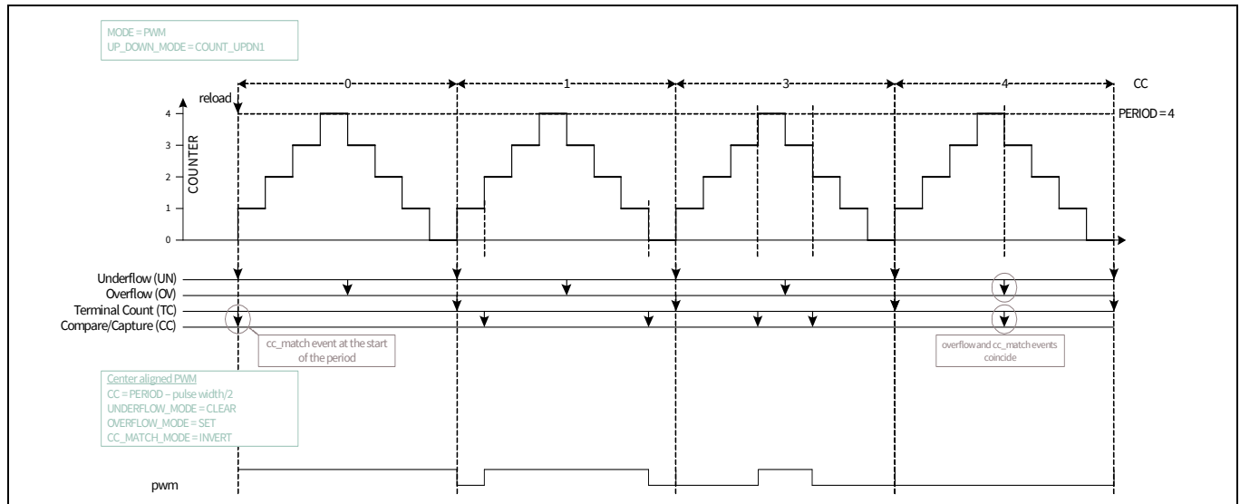
Figure 30-30. Up/down counting center-aligned PWM
