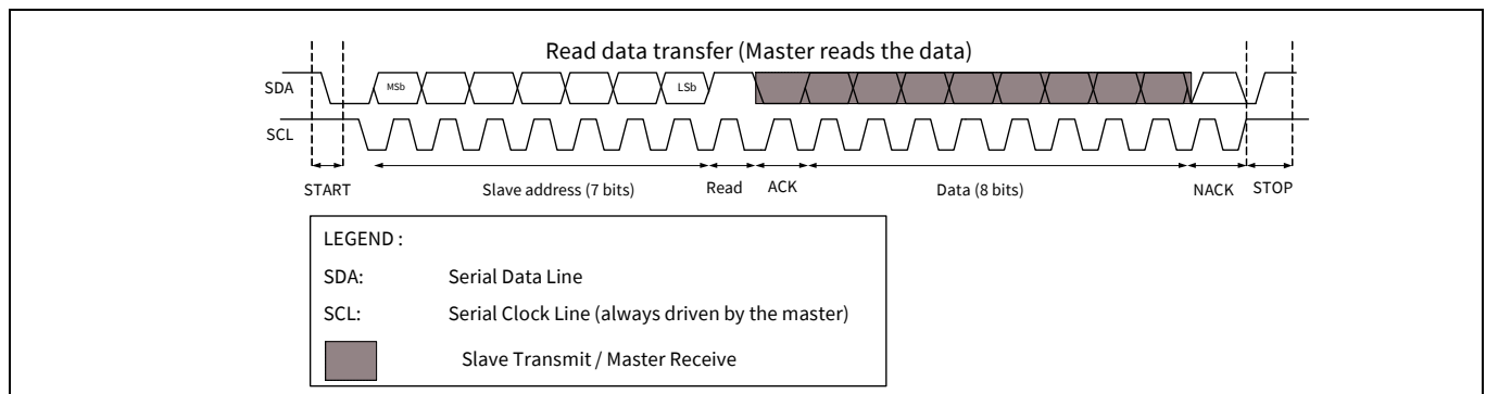
Figure 27-39. Master read data transfer
