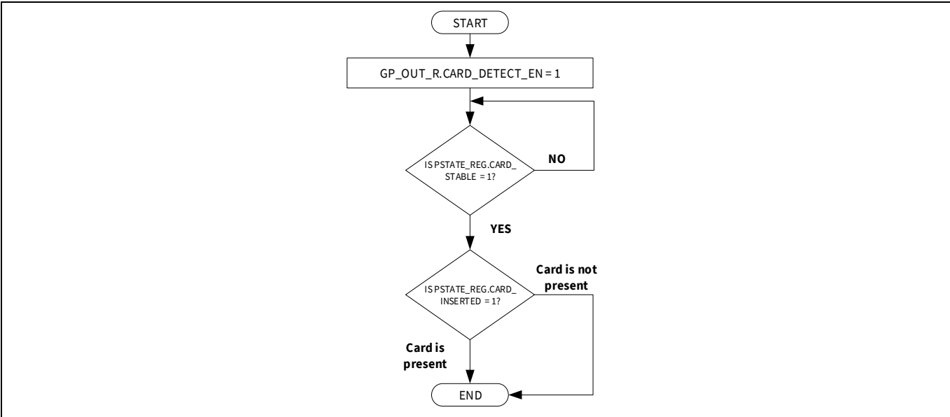
Figure 26-7. Card status check sequence
