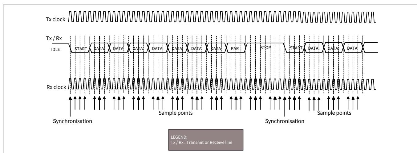
Figure 27-17. UART, standard protocol (multiple samples)
