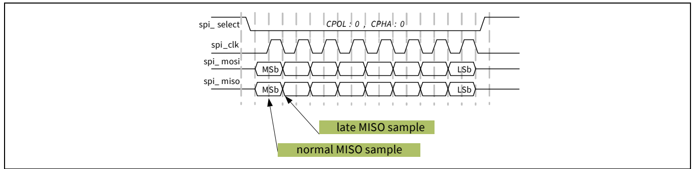
Figure 27-11. MISO sampling timing
