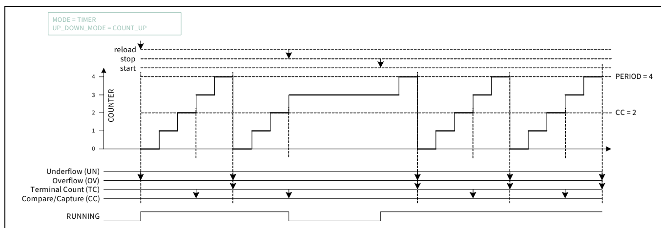
Figure 30-10. Counter start/stopped/continued
