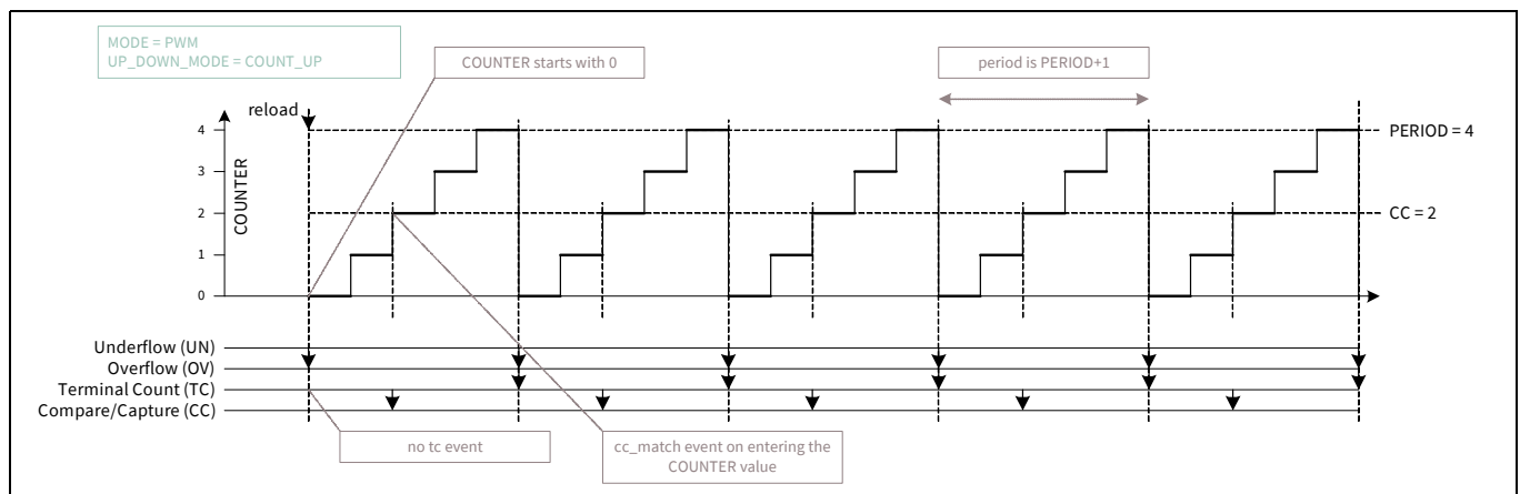
Figure 30-25. PWM in up counting mode
