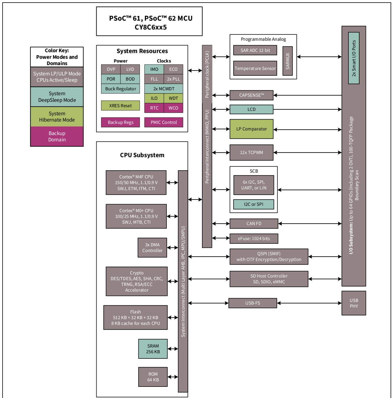
Figure 1-1. PSoC™ 6 MCU architecture block diagram
