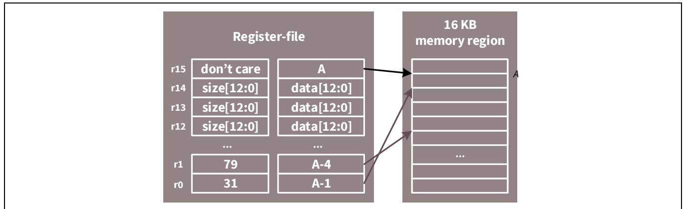
Figure 12-19. Register file state after FREE_MEM instruction
