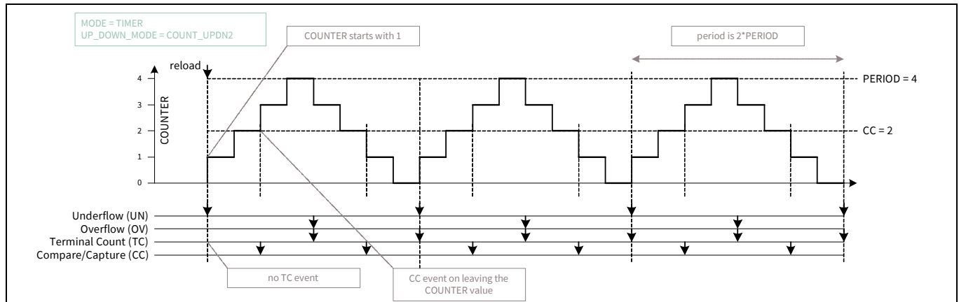
Figure 30-15. Up/down counting mode 2
