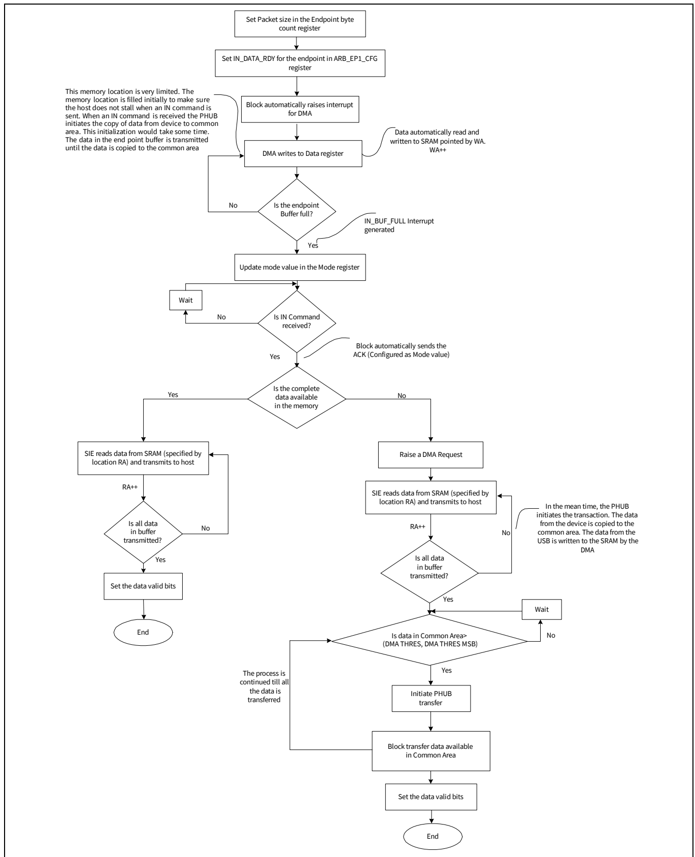
Figure 32-7. IN Transaction using automatic DMA mode
