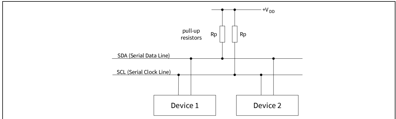
Figure 27-37. Connection of devices to the I2C bus
