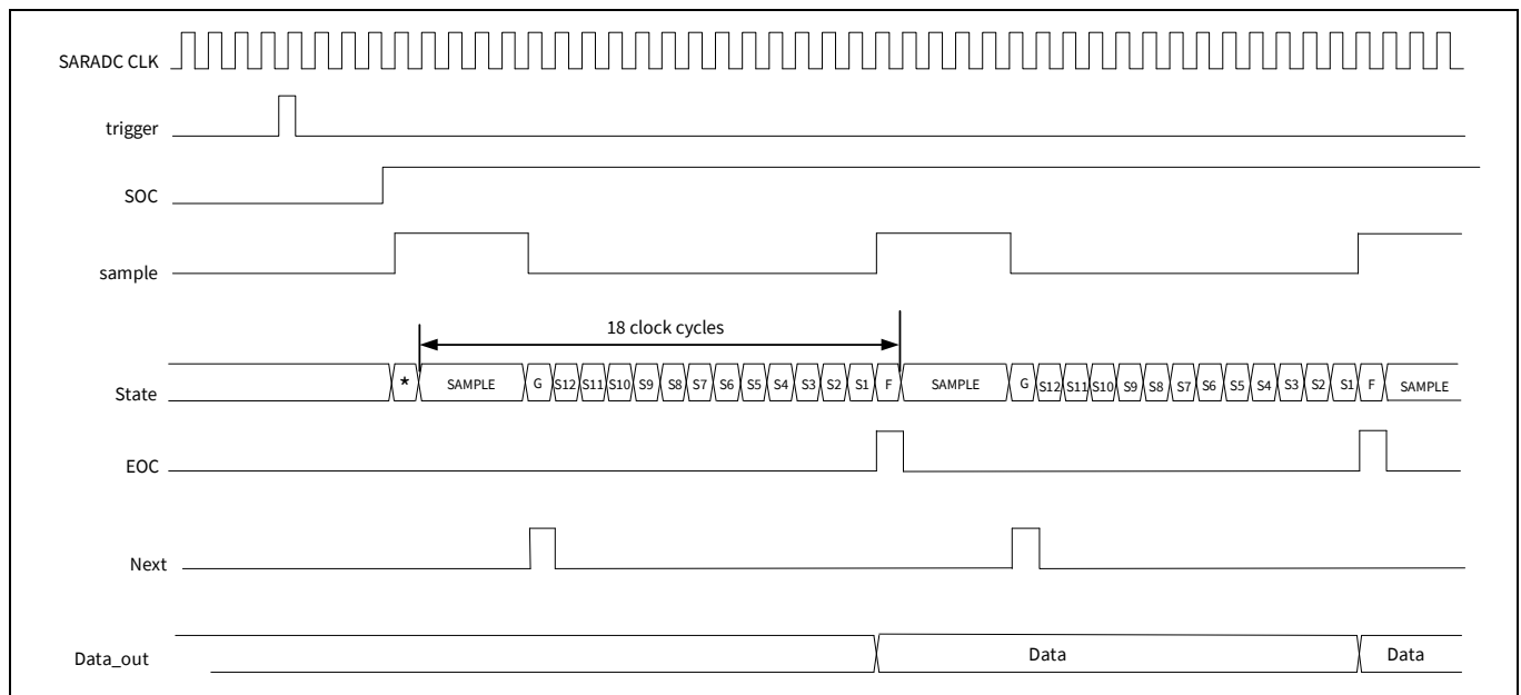
Figure 36-4. SAR ADC timing
