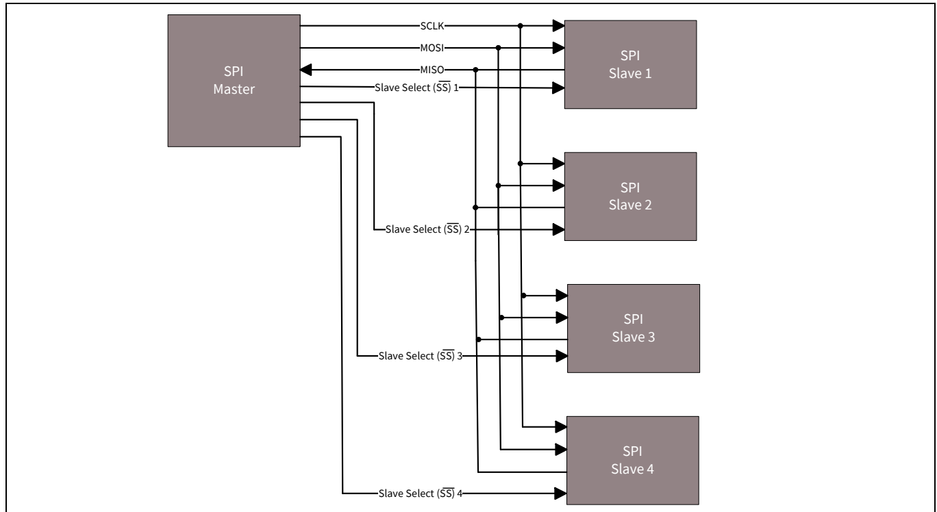
Figure 27-1. SPI example
