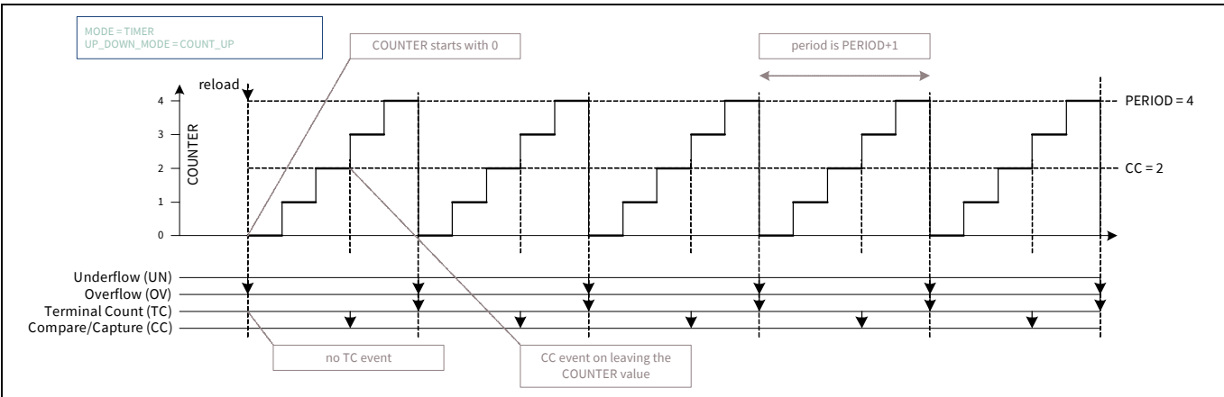
Figure 30-7. Timer in up-counting mode
