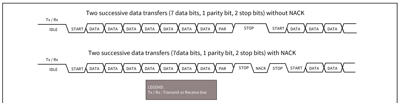
Figure 27-30. SmartCard example
