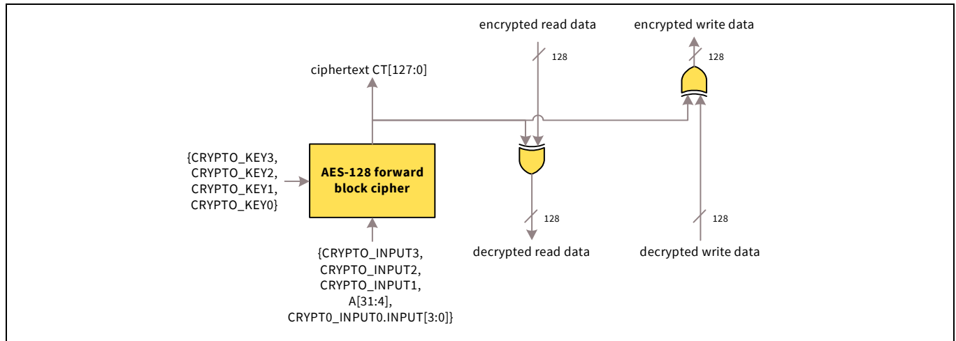
Figure 28-3. XIP mode functionality
