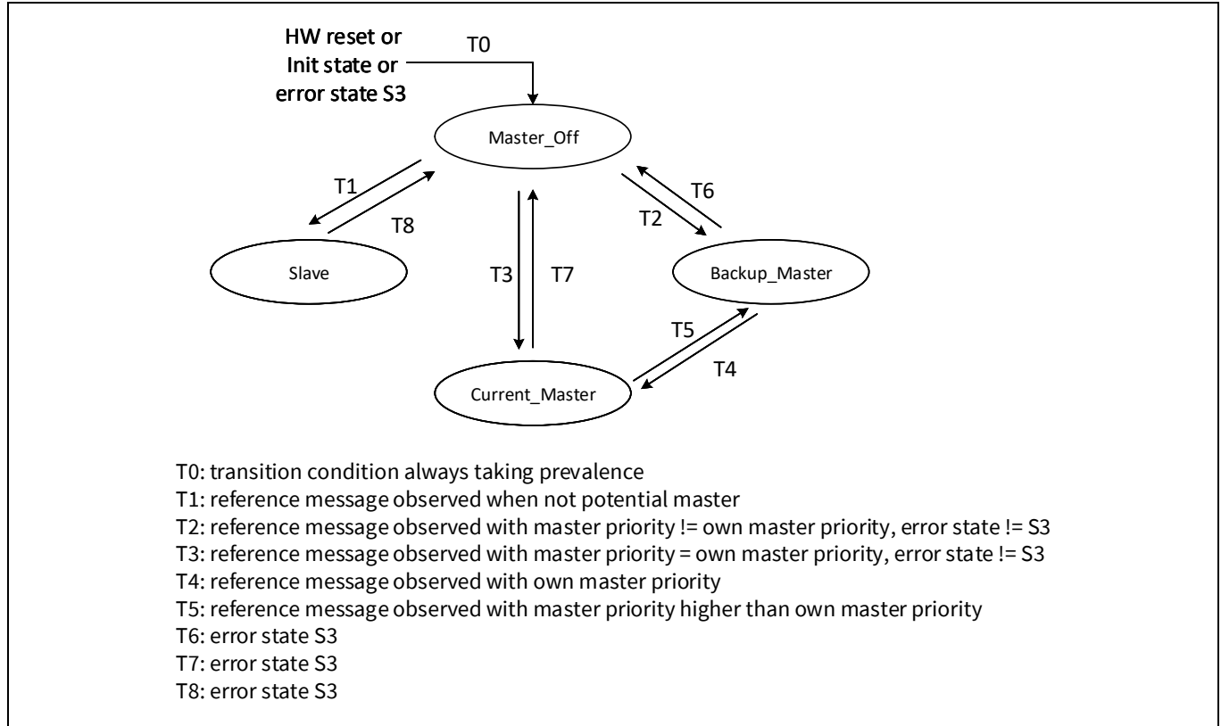
Figure 29-25. Level 0 master to slave relation
