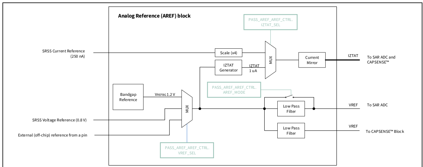
Figure 34-1. AREF block diagram
