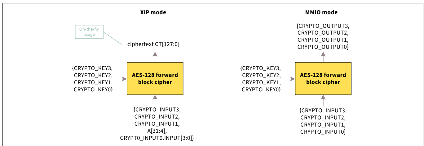
Figure 28-2. Cryptography in XIP and Command modes
