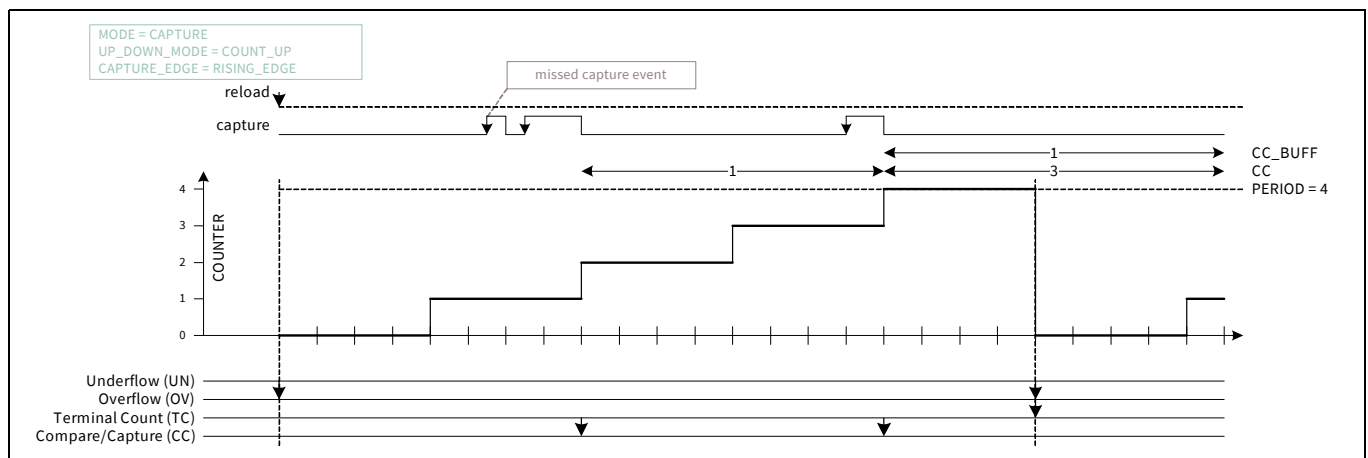
Figure 30-18. Multiple events detected before active-count
