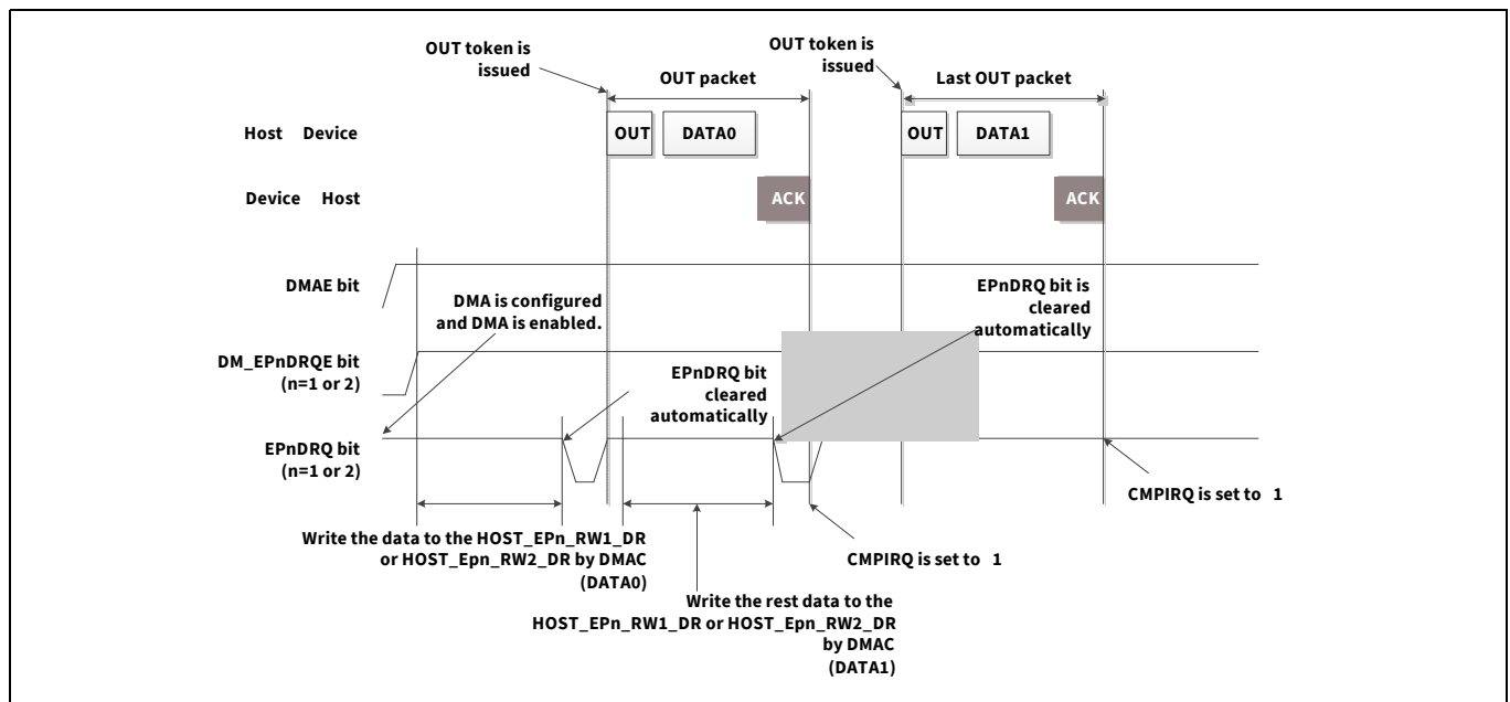
Figure 31-14. Automatic data transfer mode: OUT direction
