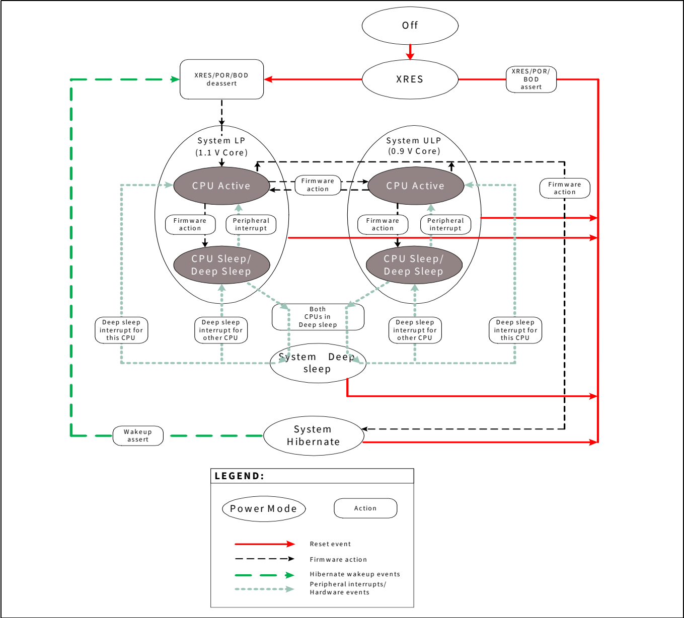
Figure 19-1. Power mode transitions in PSoC™ 6 MCU
