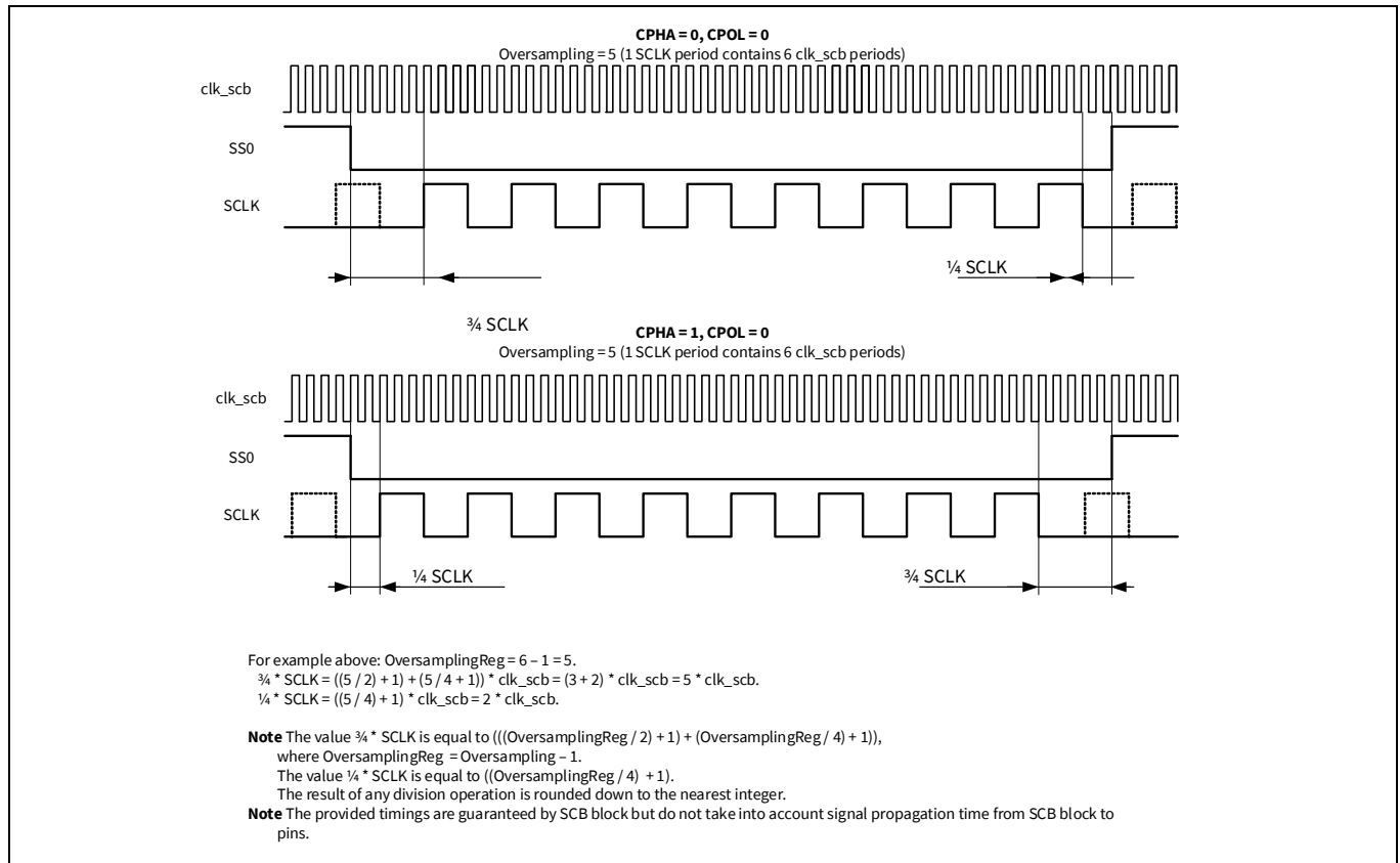
Figure 27-4. SELECT and SCLK timing correlation
