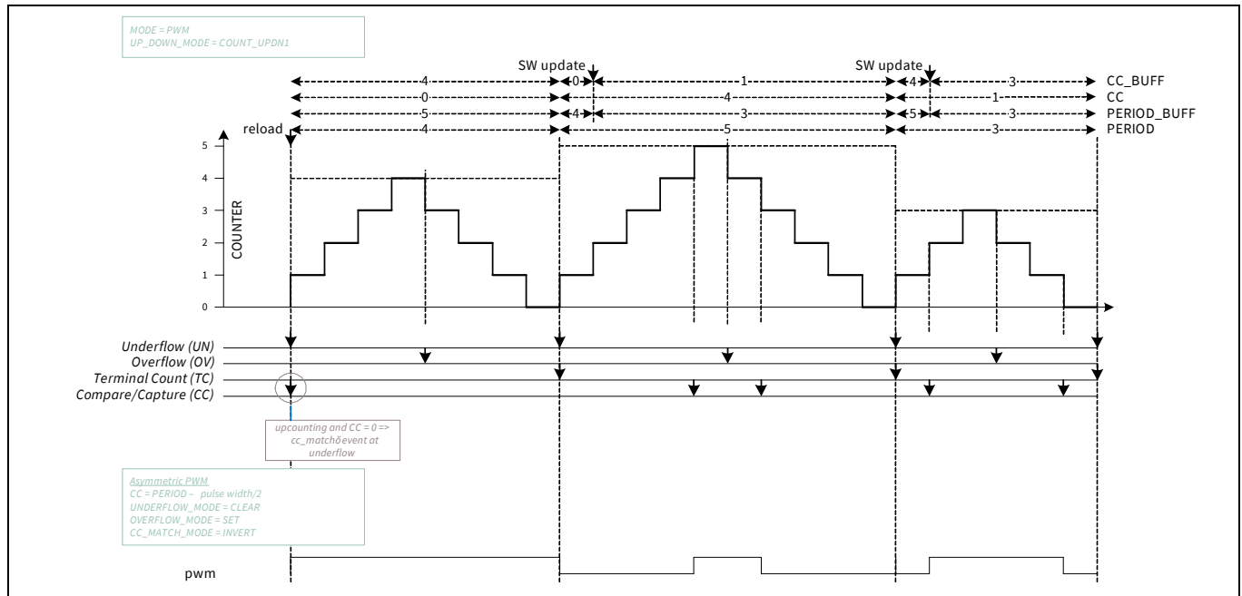
Figure 30-34. PWM mode CC swap event
