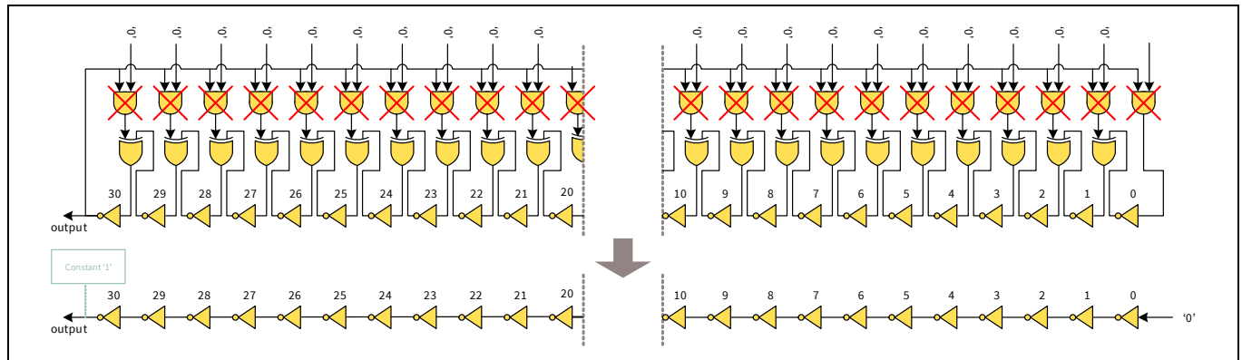
Figure 12-10. GARO31 “stopped”
