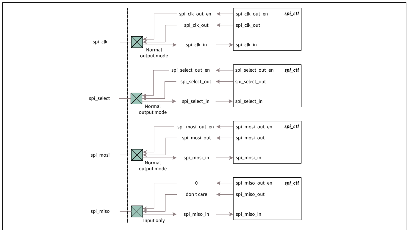
Figure 27-12. SPI master I/O pad connections
