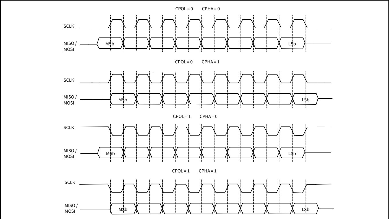
Figure 27-2. SPI Motorola, 4 modes
