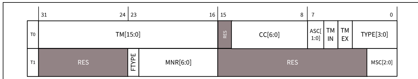
Figure 29-21. Trigger memory element
