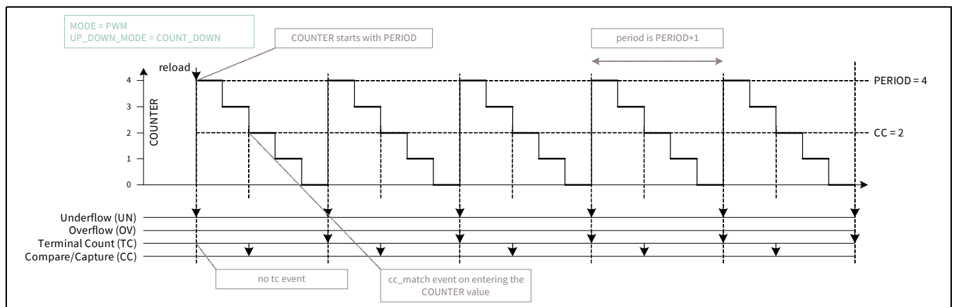
Figure 30-27. PWM in down counting mode
