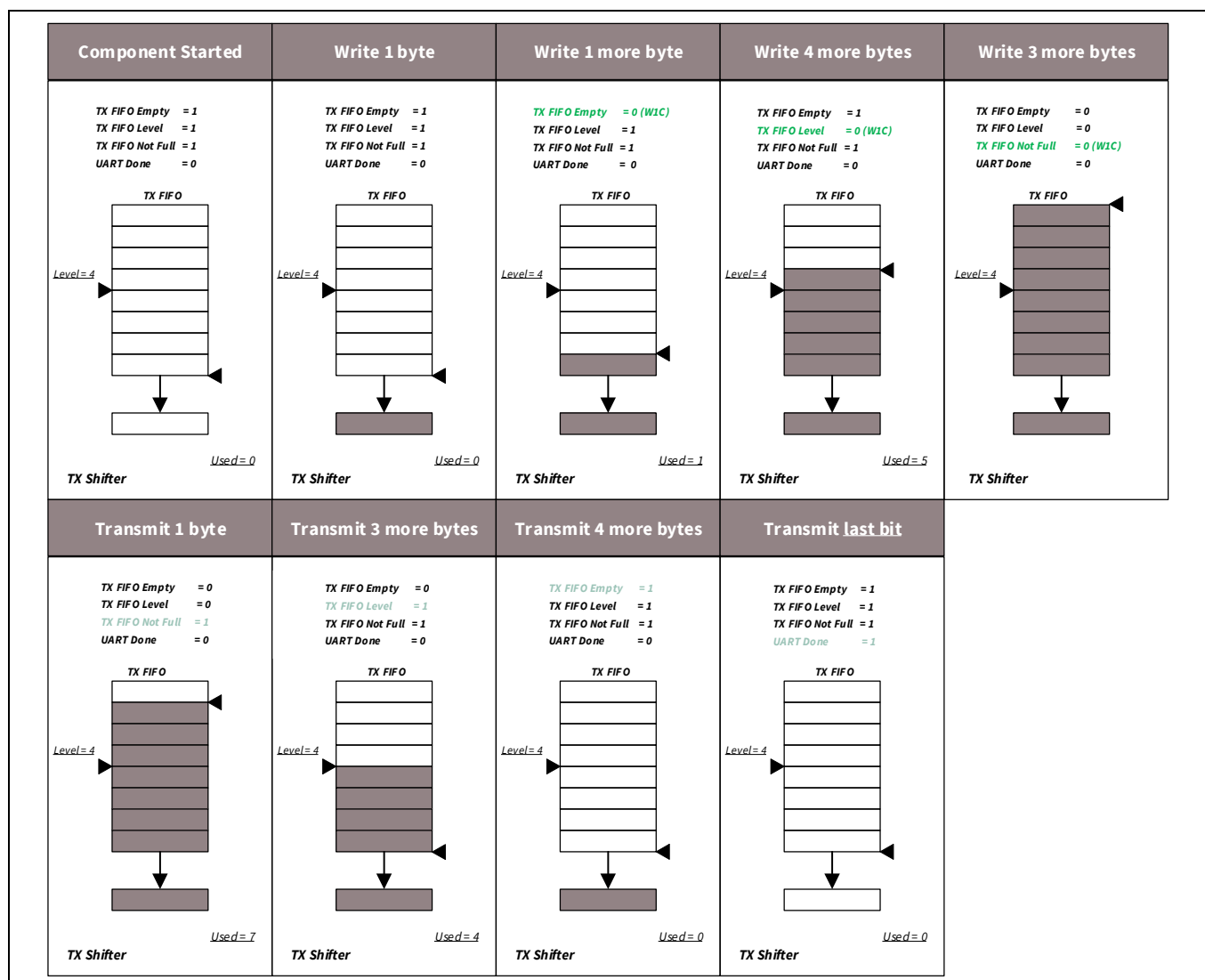
Figure 27-48. TX interrupt source operation
