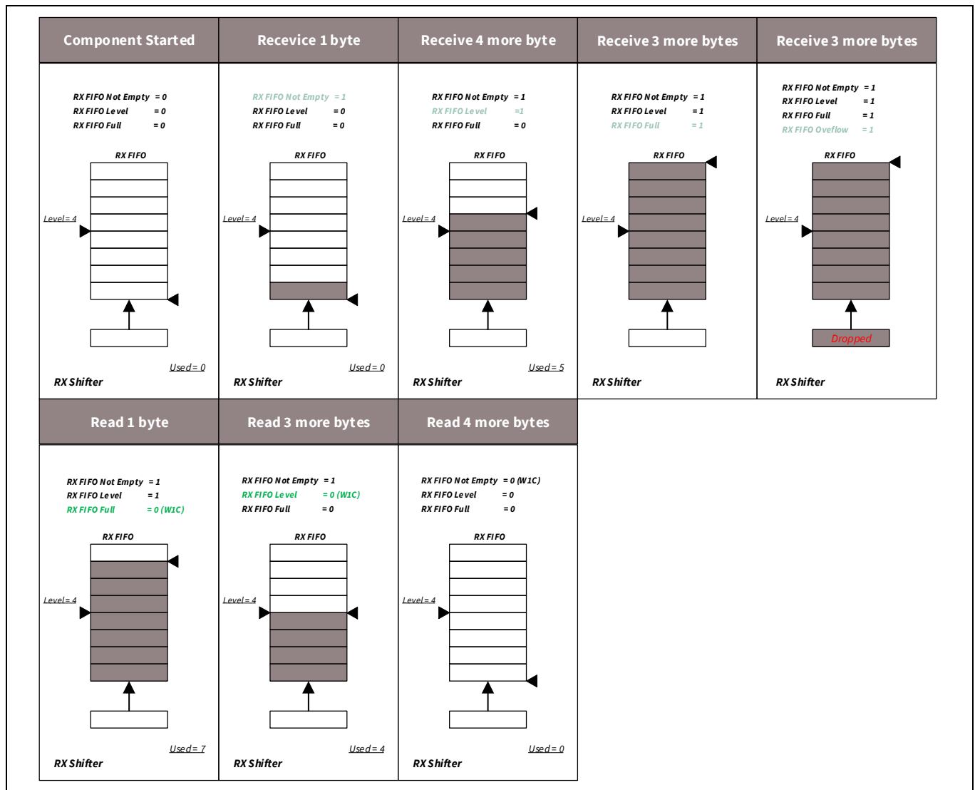
Figure 27-47. RX interrupt source operation
