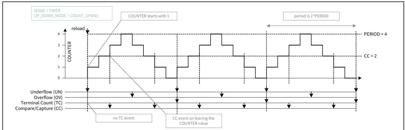
Figure 30-13. Timer in up/down counting mode 1
