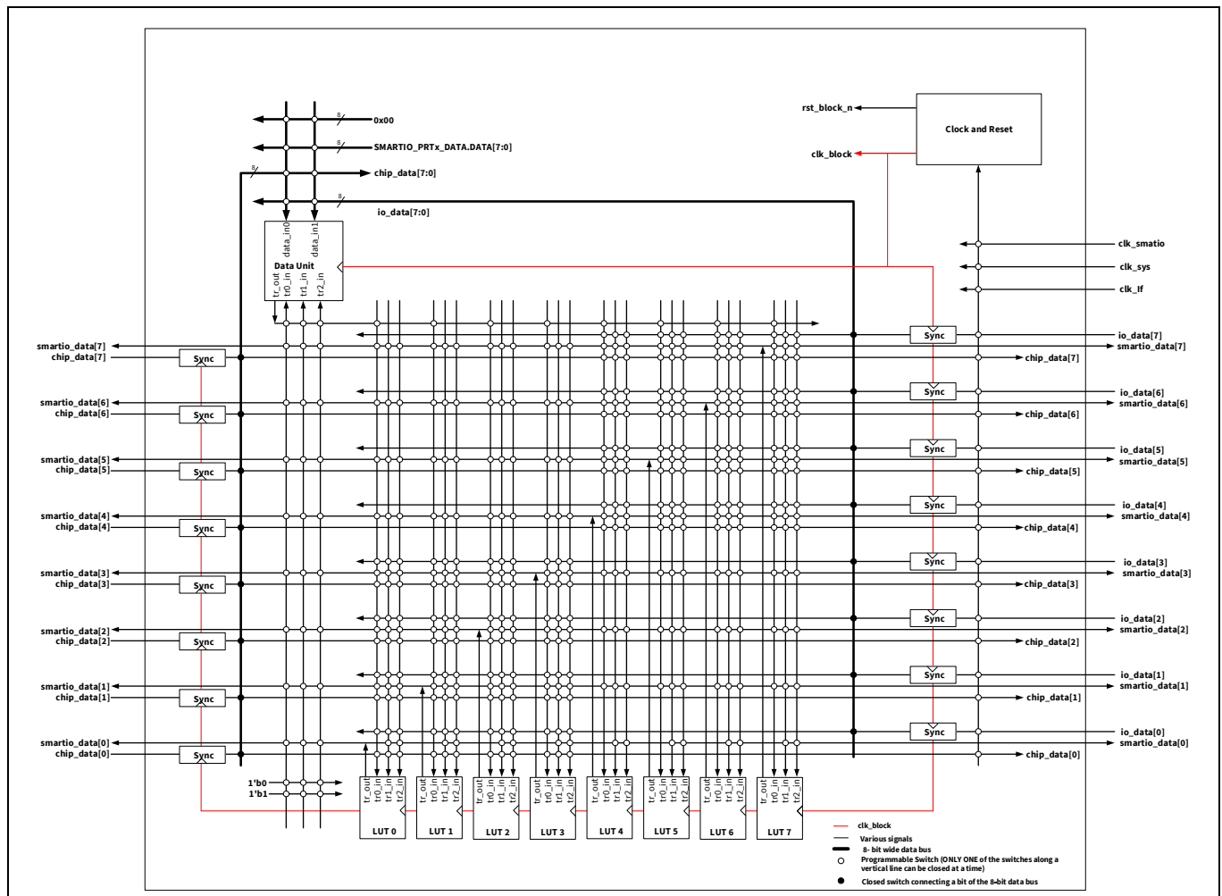
Figure 23-10. Smart I/O routing
