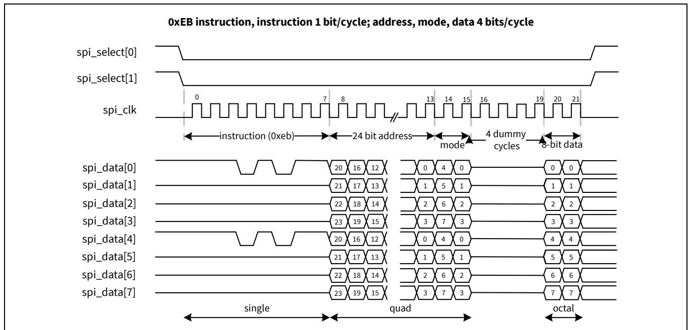
Figure 28-14. Two-byte transfer in dual Quad SPI mode
