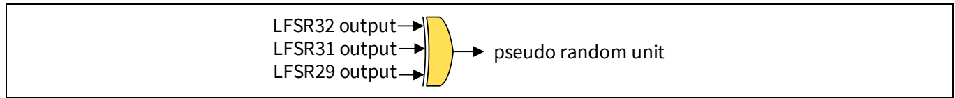
Figure 12-5. XOR reduction logic
