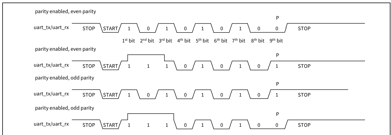
Figure 27-18. UART parity examples
