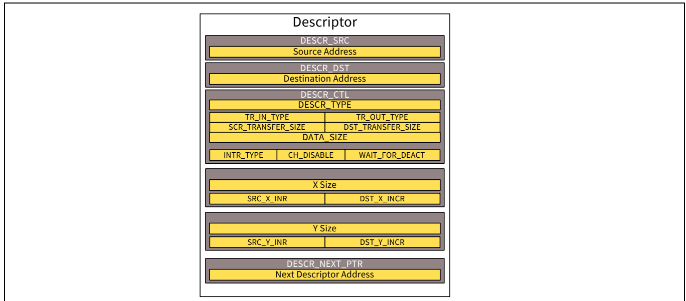
Figure 10-2. Descriptor structure
