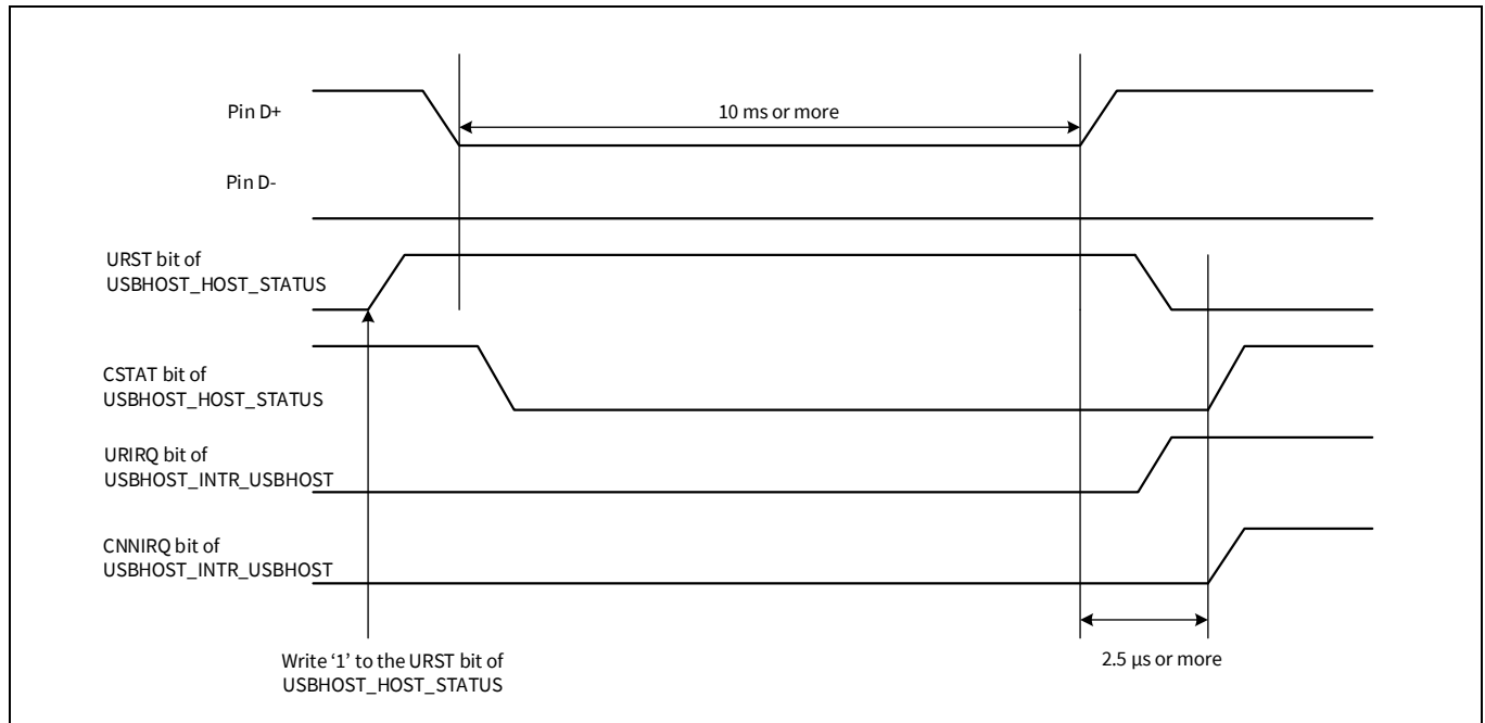
Figure 31-4. Device reset timing diagram
