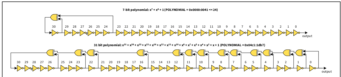
Figure 12-14. FIRO31 – Two examples
