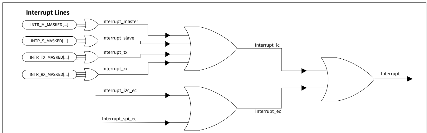
Figure 27-45. Interrupt lines
