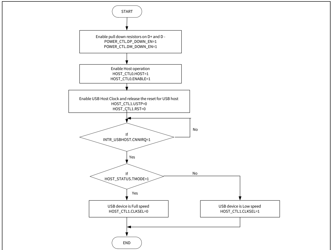
Figure 31-3. Device connection and transfer speed detection flow chart
