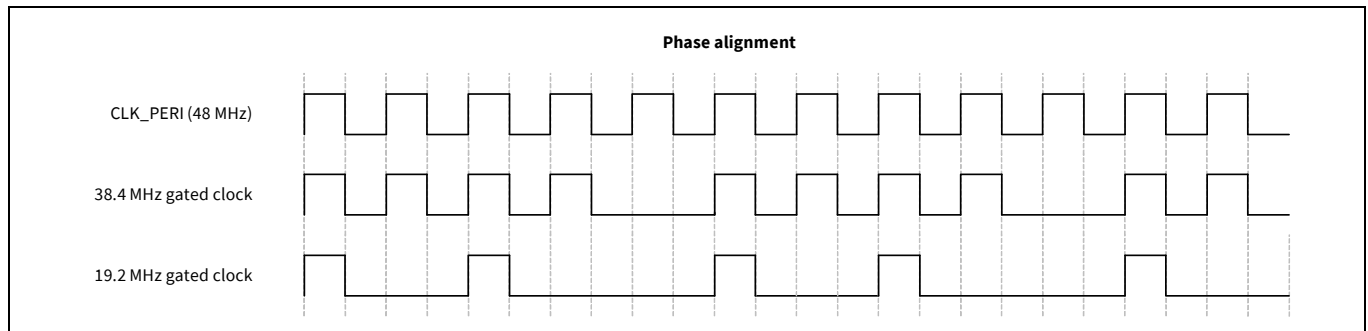
Figure 21-7. Phase-aligned fractional dividers
