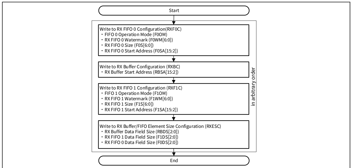
Figure 29-34. RX FIFO and RX buffer configuration
