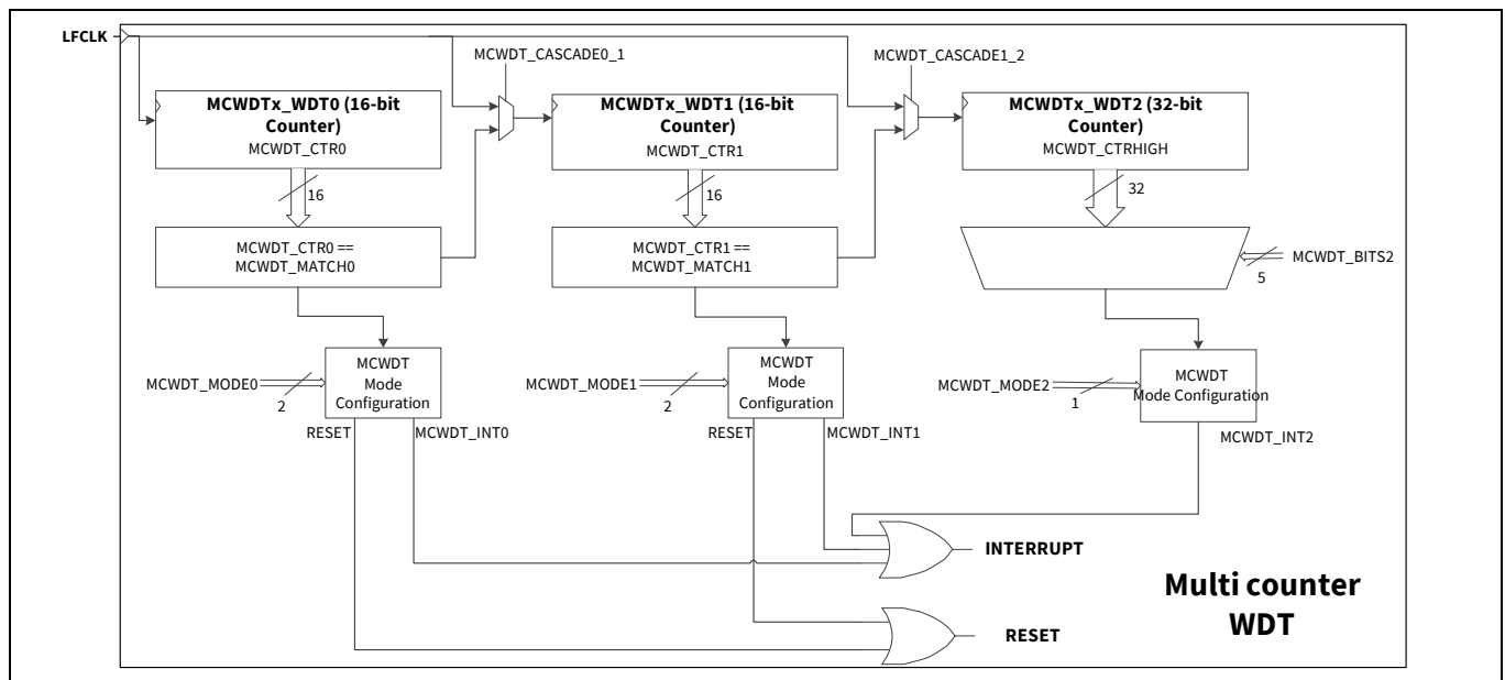
Figure 24-3. Multi-counter WDT functional diagram
