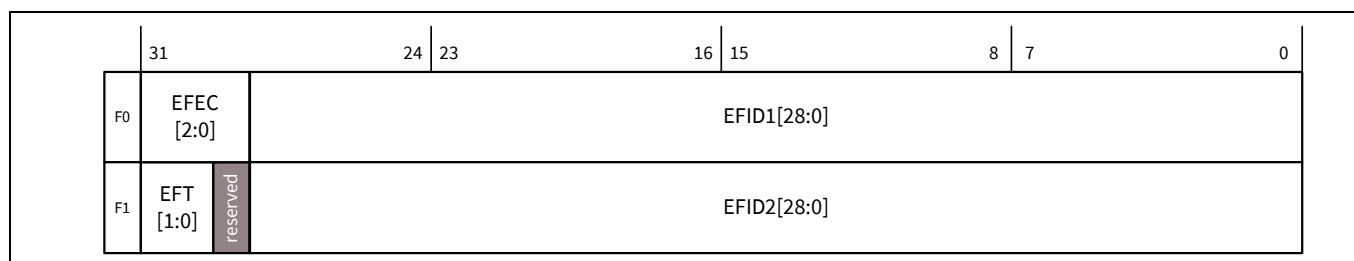
Figure 29-20. Extended Message ID filter
