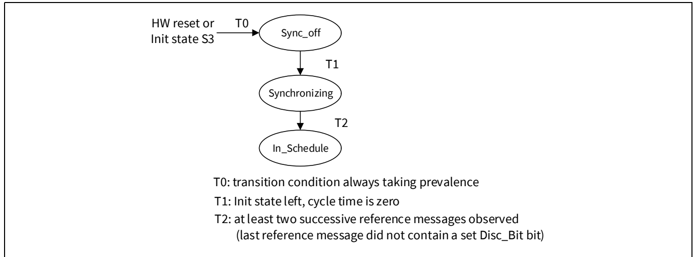
Figure 29-24. Level 0 schedule synchronization state machine
