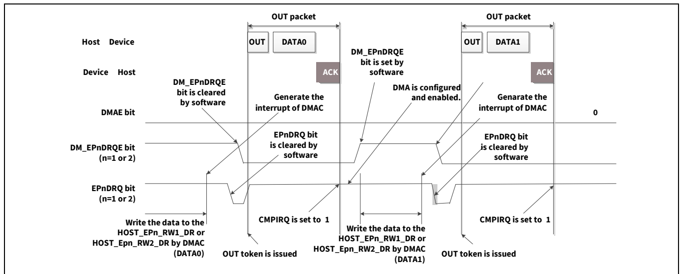
Figure 31-12. Packet transfer mode: OUT direction
