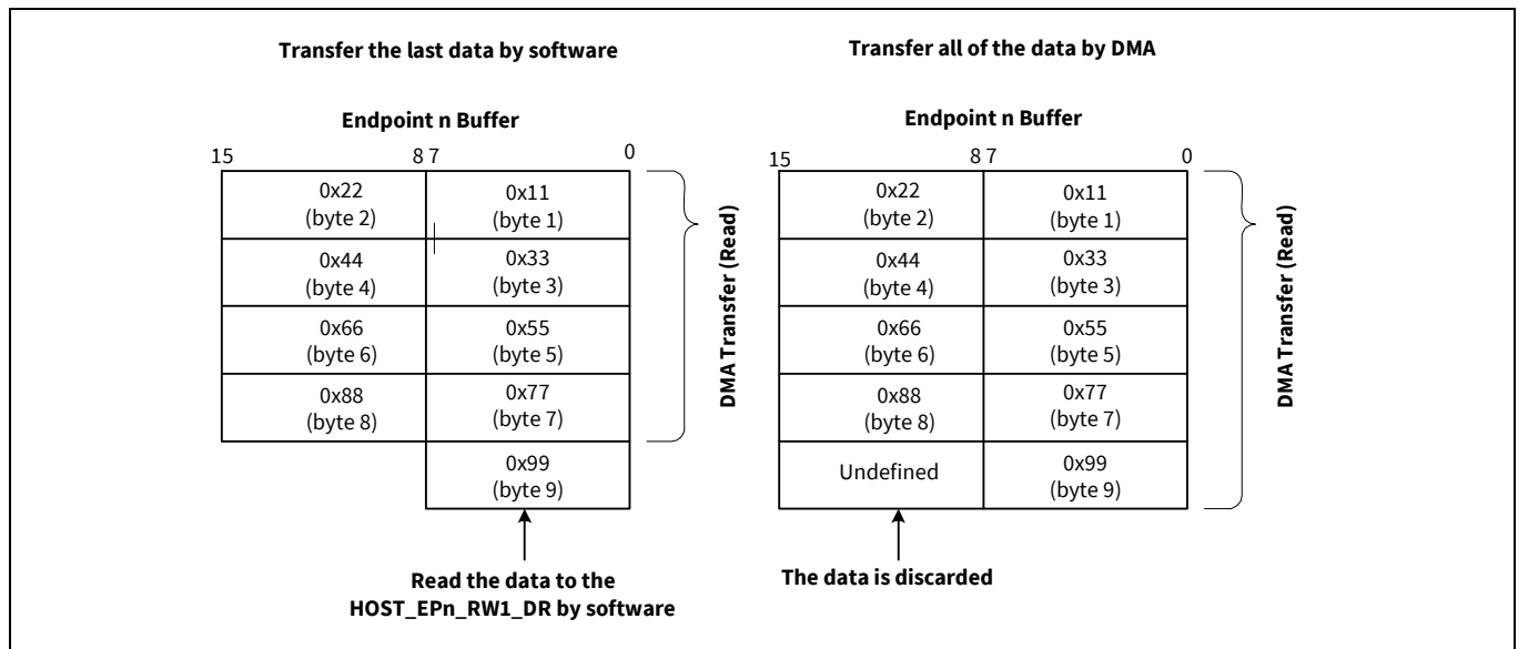
Figure 31-17. Odd bytes transfer in the IN direction
