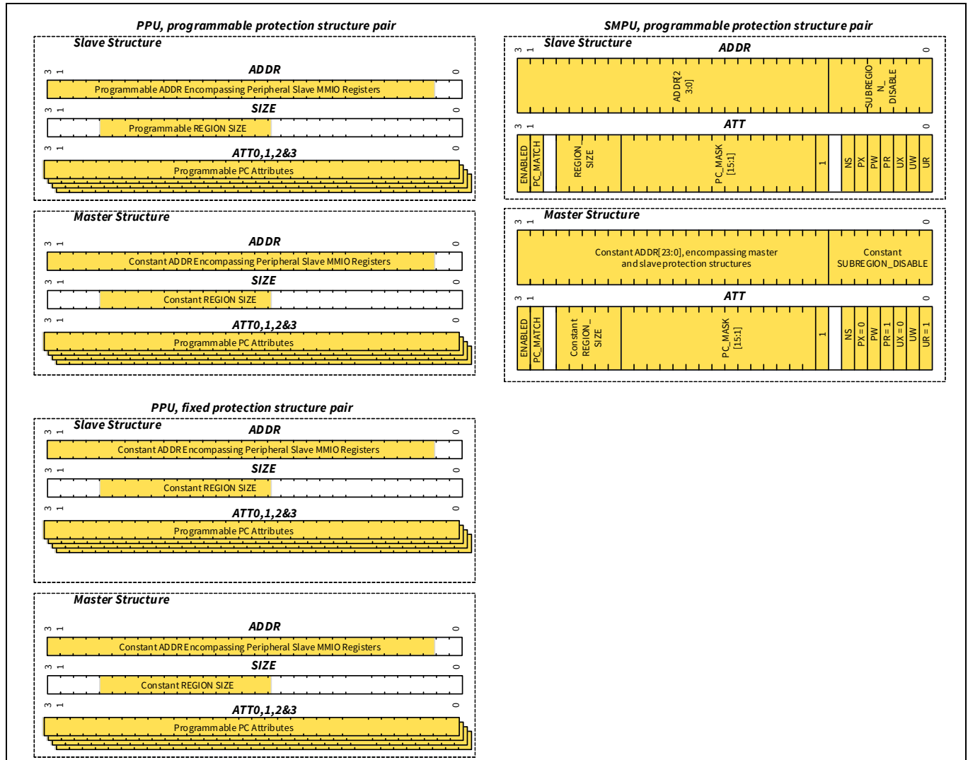
Figure 9-6. PPU and SMPU pairs
