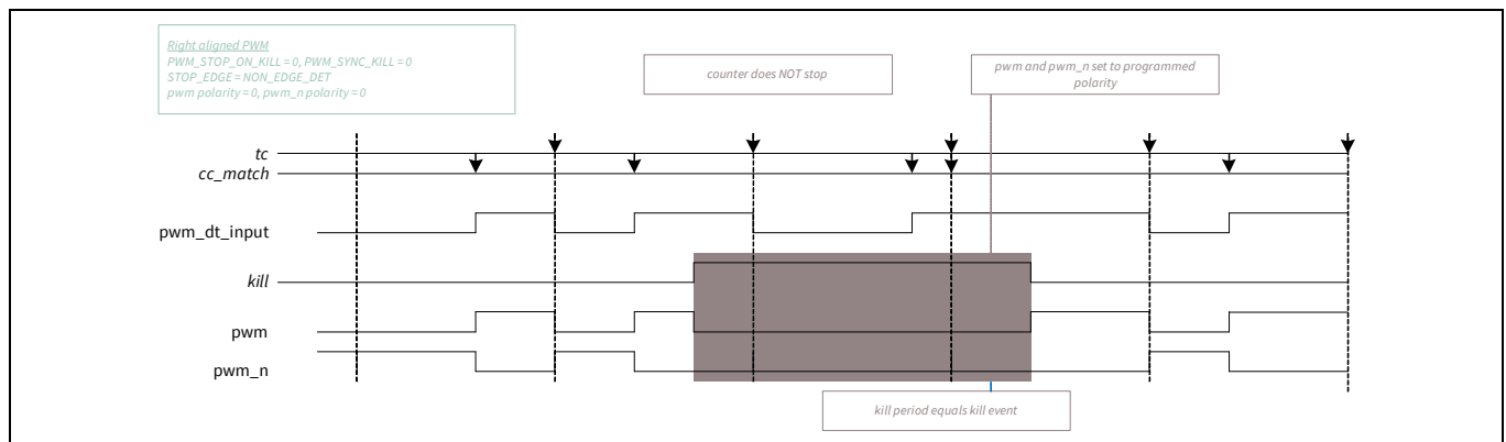
Figure 30-32. PWM async kill
