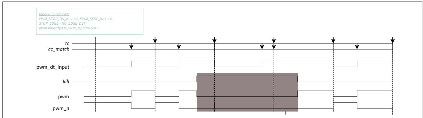
Figure 30-35. PWM outputs when killed
