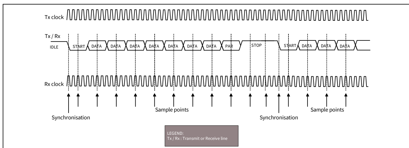
Figure 27-16. UART, standard protocol example (single sample)
