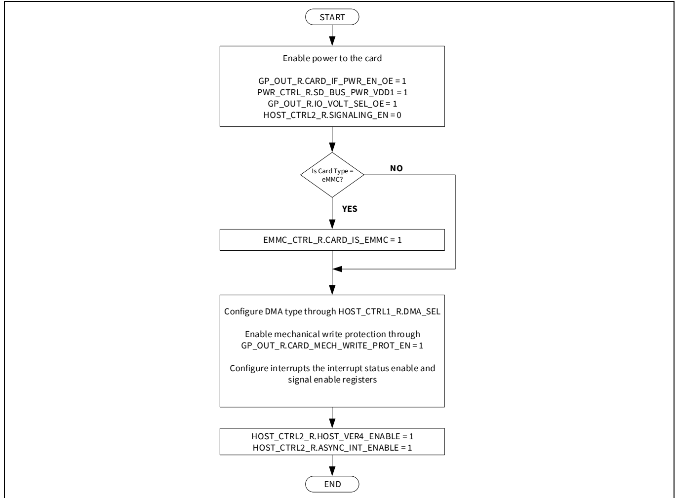
Figure 26-9. SDHC setup
