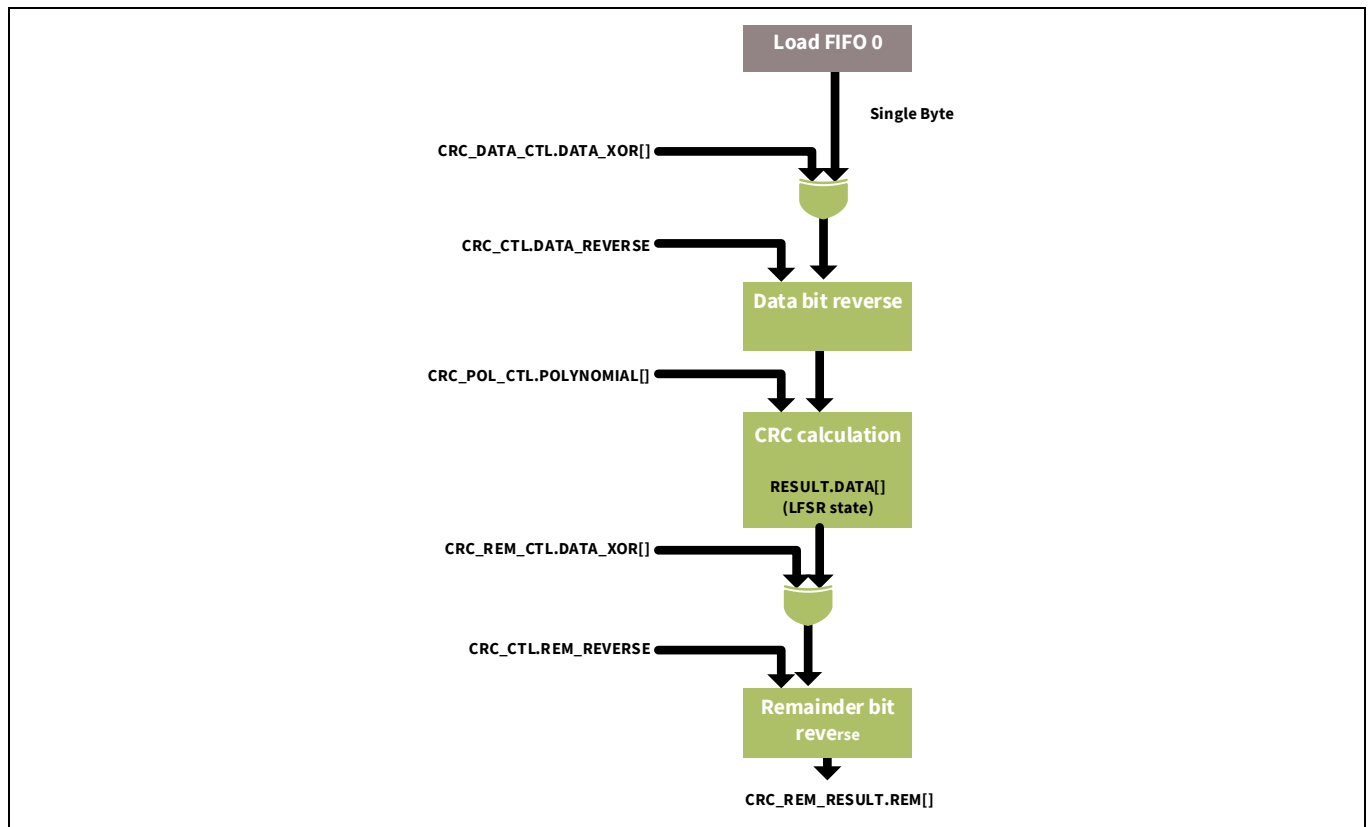
Figure 12-2. CRC functionality
