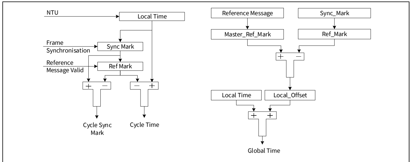
Figure 29-22. Cycle time and global time synchronization
