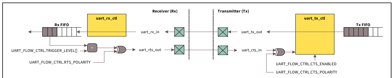
Figure 27-21. UART flow control connection
