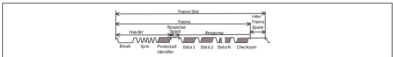
Figure 27-26. LIN frame structure
