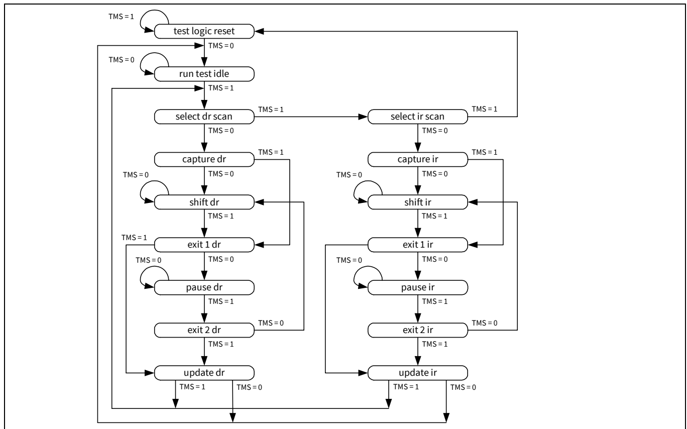
Figure 13-5. TAP state machine
