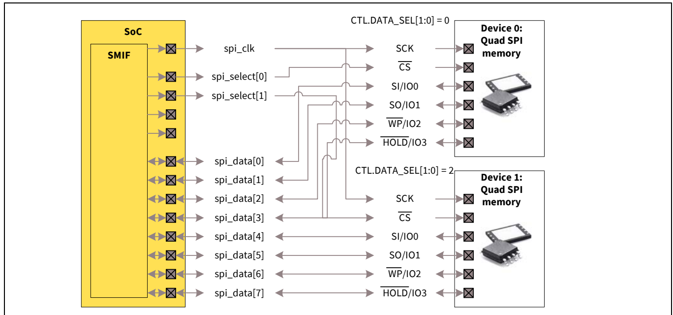
Figure 28-13. Setting up SMIF
