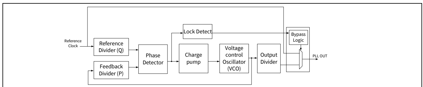
Figure 21-2. PLL block diagram
