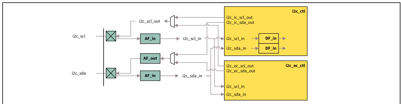
Figure 27-42. I 2 C glitch filtering connection
