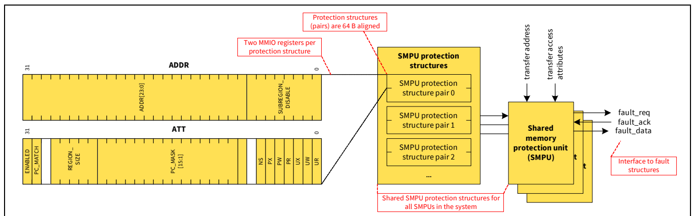
Figure 9-4. SMPU functionality
