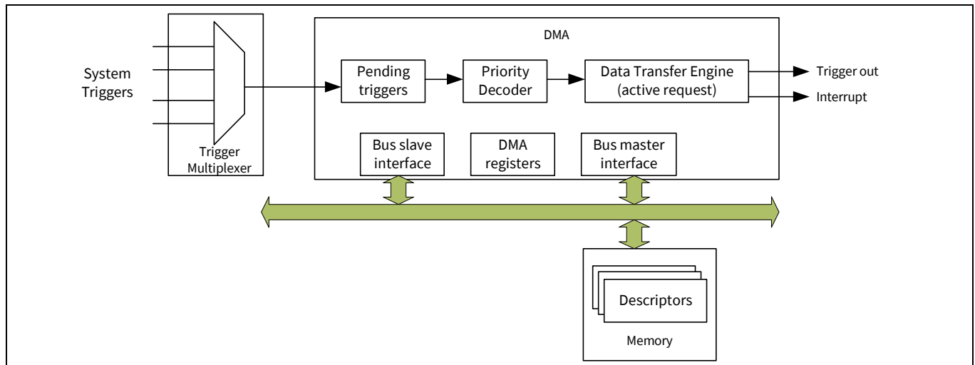
Figure 10-3. DMA controller overview
