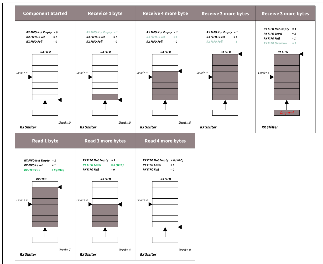
Figure 27-49. RX interrupt source operation
