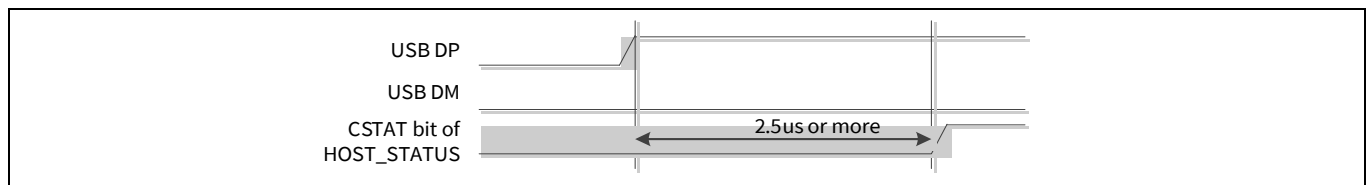
Figure 31-2. Device connection
