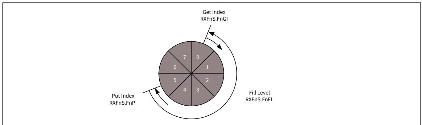
Figure 29-7. RX FIFO status
