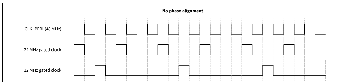
Figure 21-5. Non phase-aligned clock dividers
