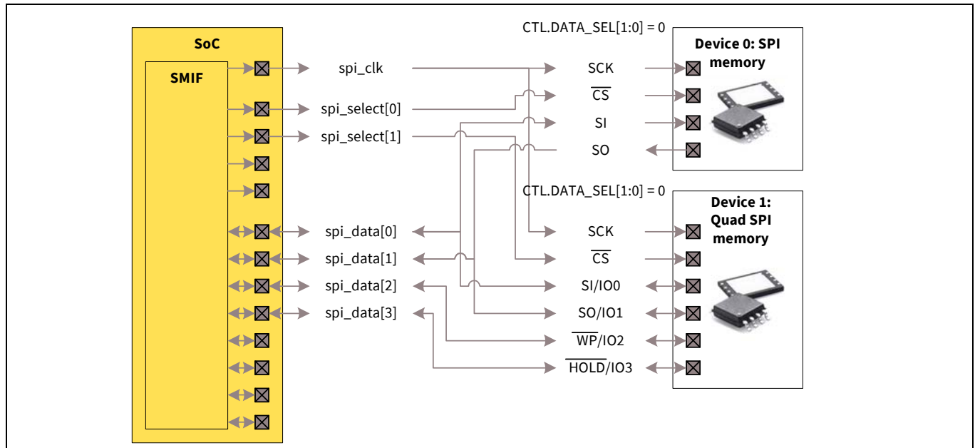
Figure 28-10. Single SPI memory device 0 and Quad SPI memory device 1 - Shared data signal
