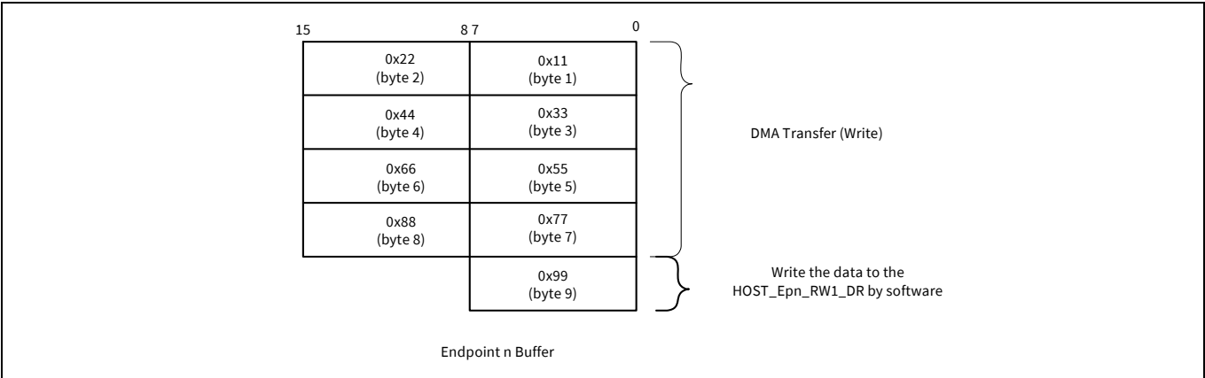
Figure 31-15. Odd bytes transfer in the OUT direction
