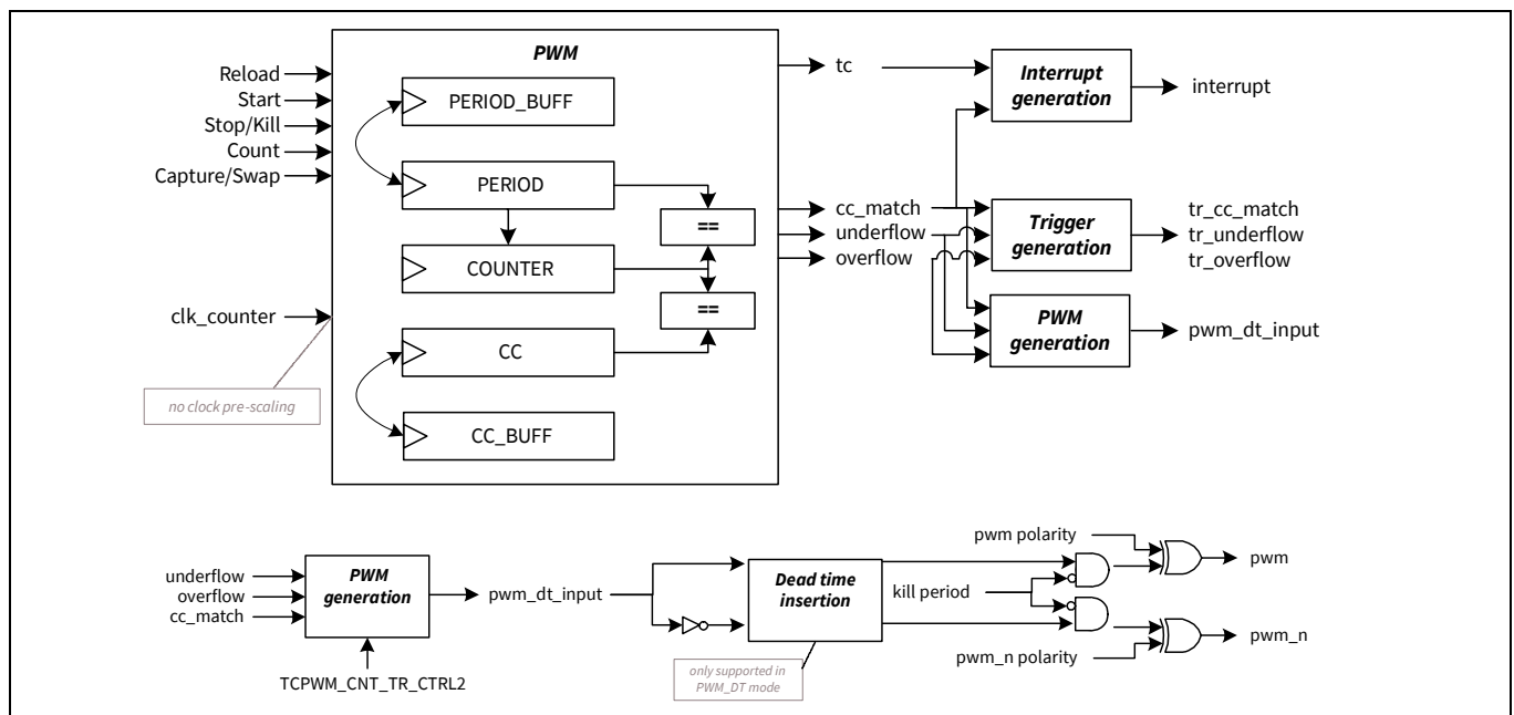
Figure 30-38. PWM with dead time functionality
