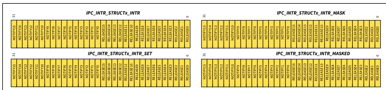
Figure 6-3. IPC interrupt structure
