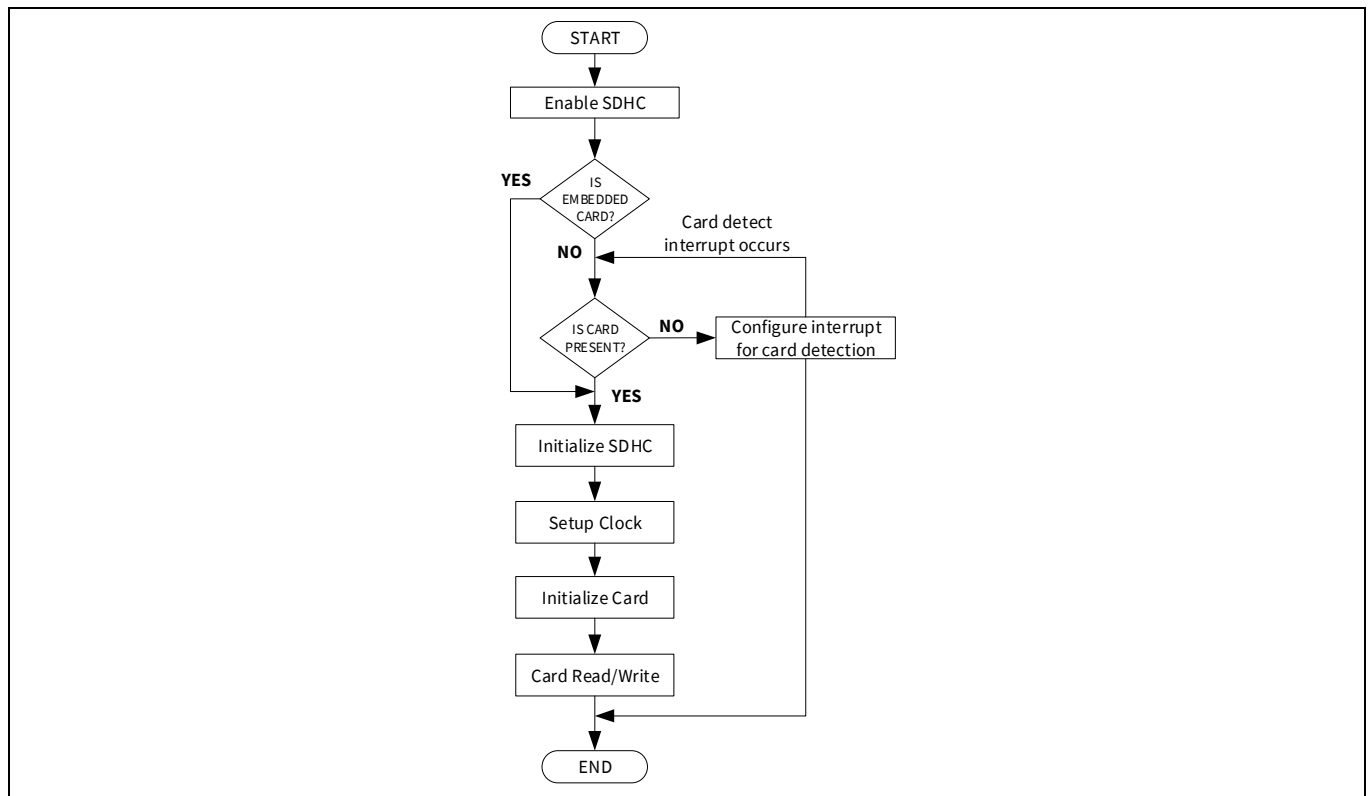
Figure 26-5. SDHC programming sequence
