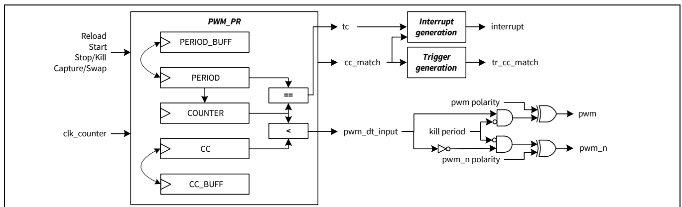
Figure 30-41. PWM_PR functionality
