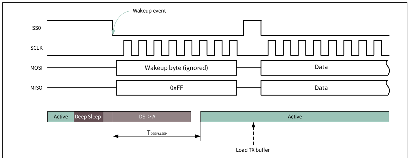
Figure 27-8. SPI slave wakeup from Deep Sleep (Motorola, CPHA = 0, CPOL = 0)
