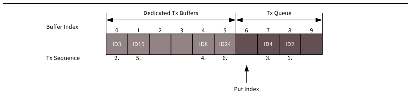
Figure 29-11. Example of mixed configuration dedicated TX buffers/TX Queue
