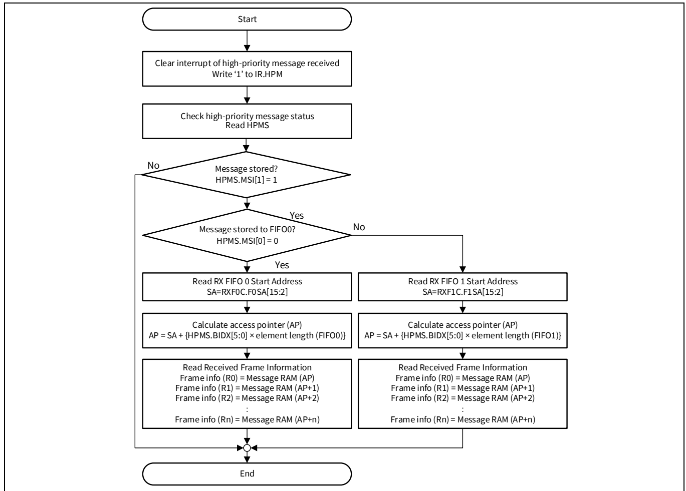
Figure 29-44. High priority message handling
