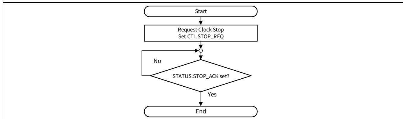
Figure 29-27. Clock stop request procedure
