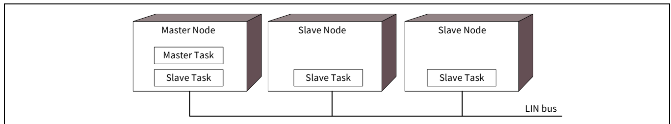
Figure 27-25. LIN bus nodes and tasks
