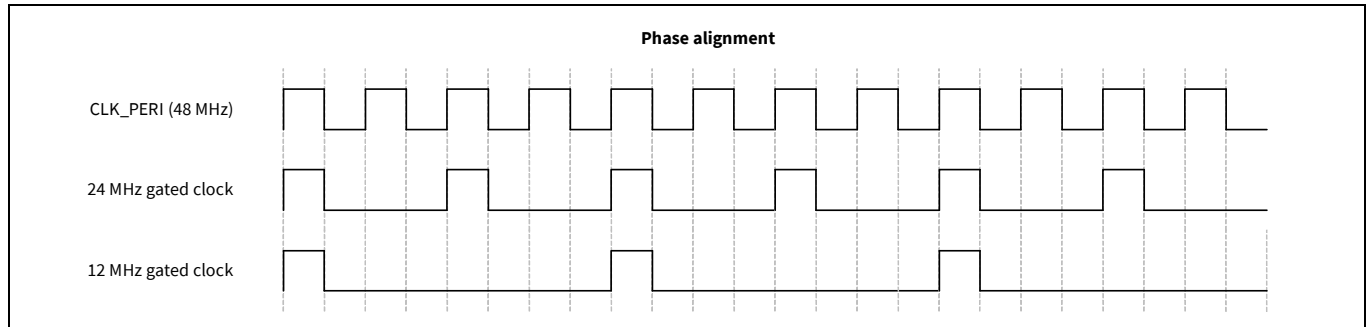
Figure 21-6. Phase-aligned clock dividers
