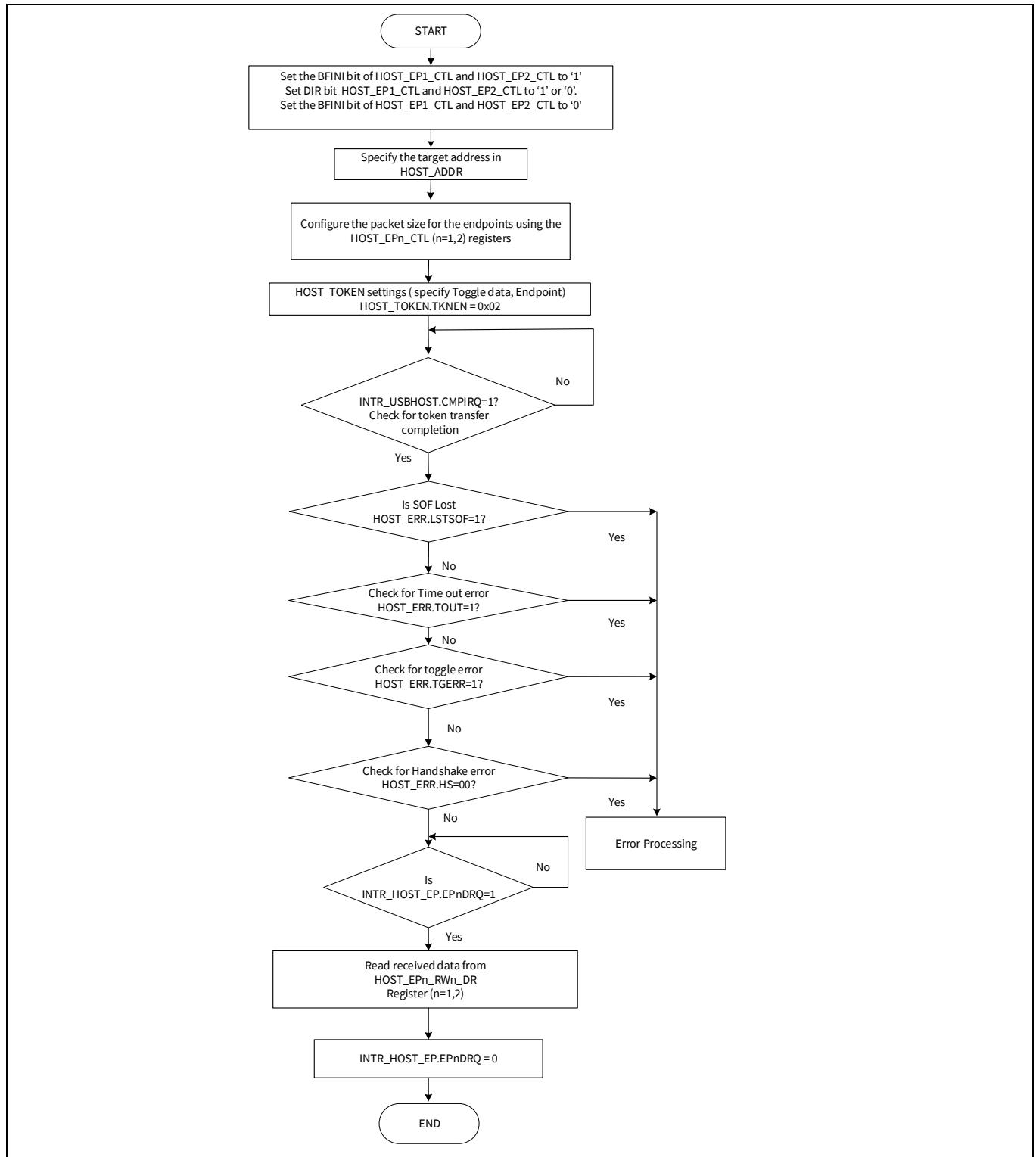
Figure 31-5. IN token flow chart
