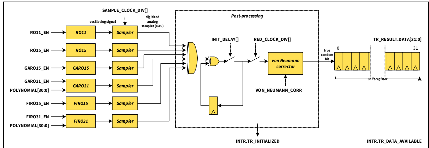
Figure 12-6. TRNG overview
