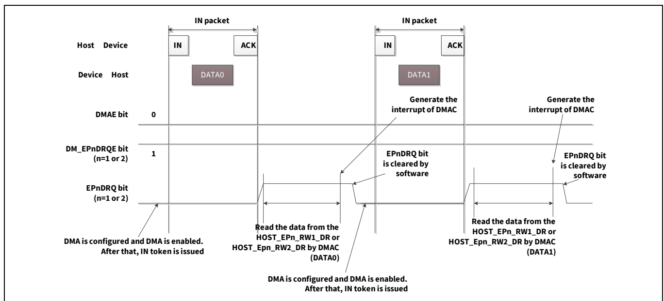
Figure 31-13. Packet transfer mode: IN direction
