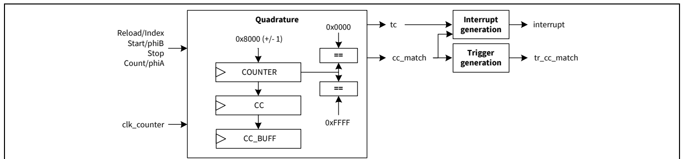
Figure 30-19. Quadrature functionality (16-bit example)
