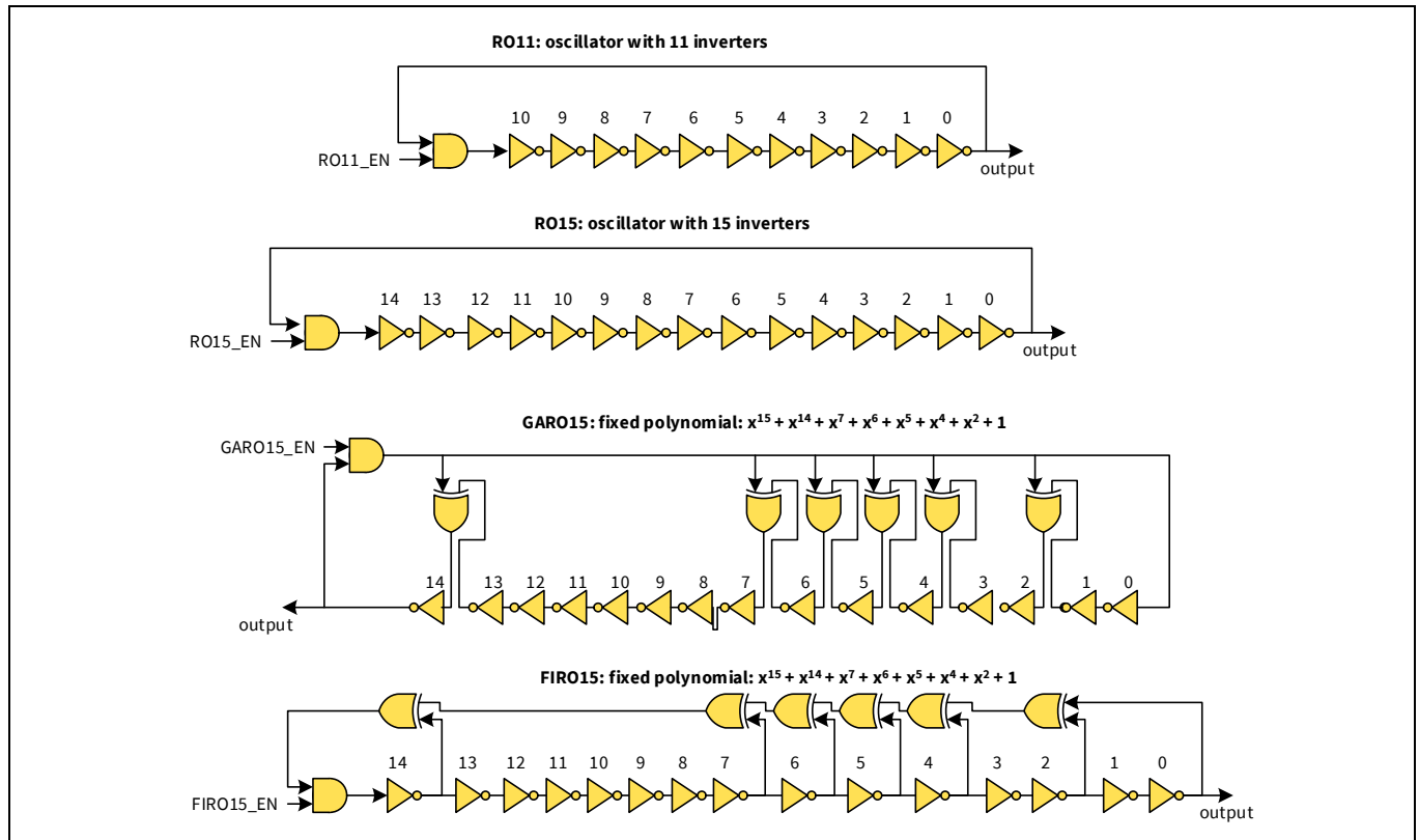
Figure 12-8. Four fixed ring oscillators: RO11, RO15, GARO15, FIRO15
