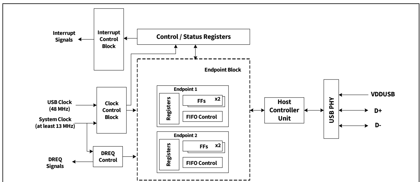
Figure 31-1. USB host block diagram
