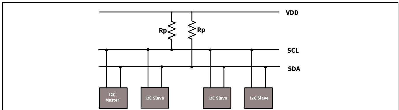
Figure 27-36. I 2 C interface block diagram
