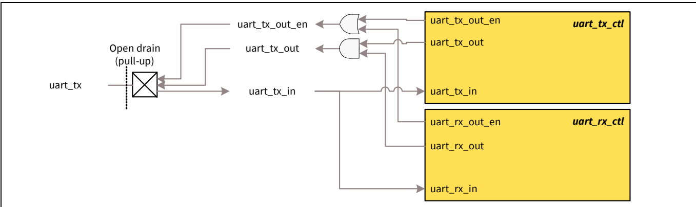
Figure 27-33. SmartCard mode I/O pad connections
