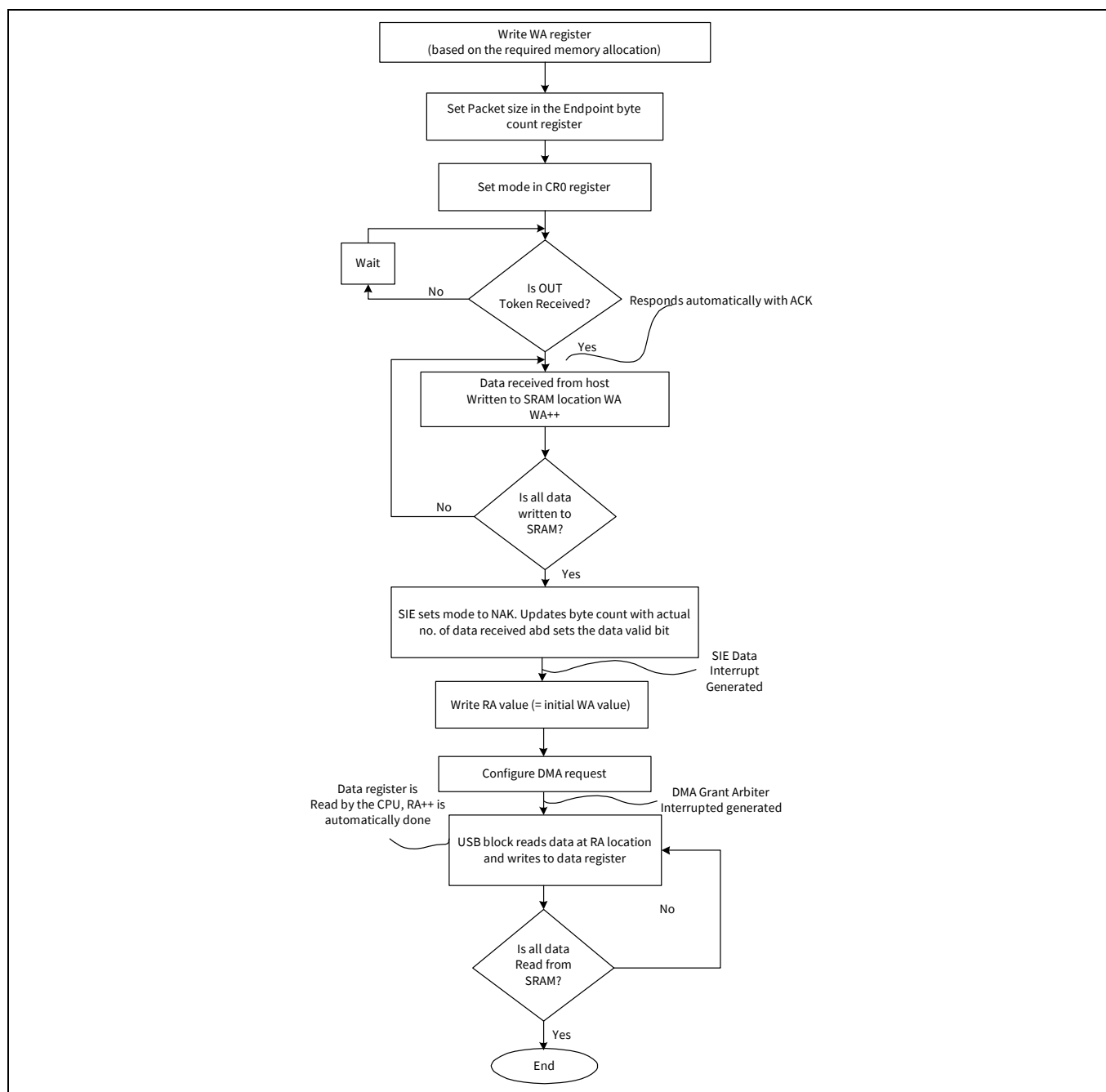
Figure 32-6. Manual DMA OUT transaction
