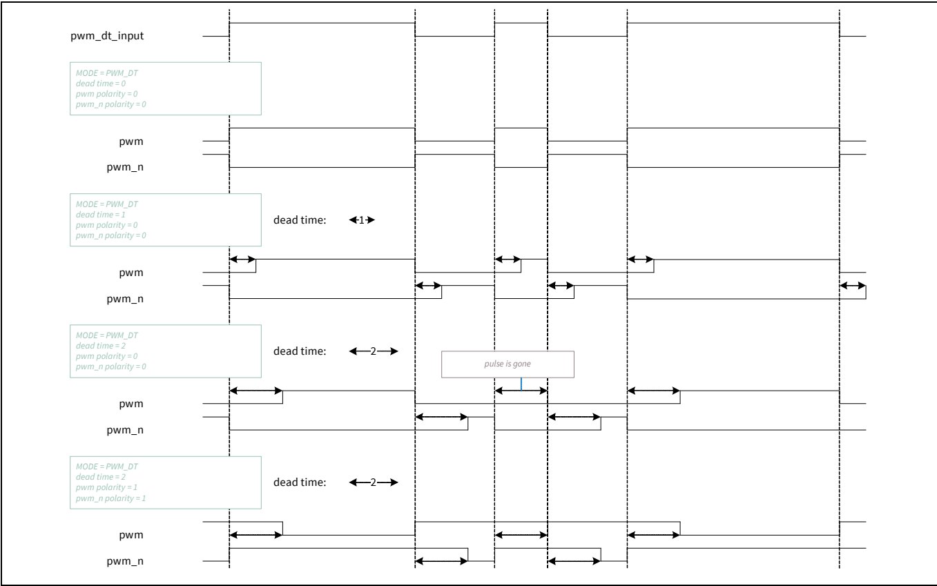
Figure 30-39. Dead-time timing
