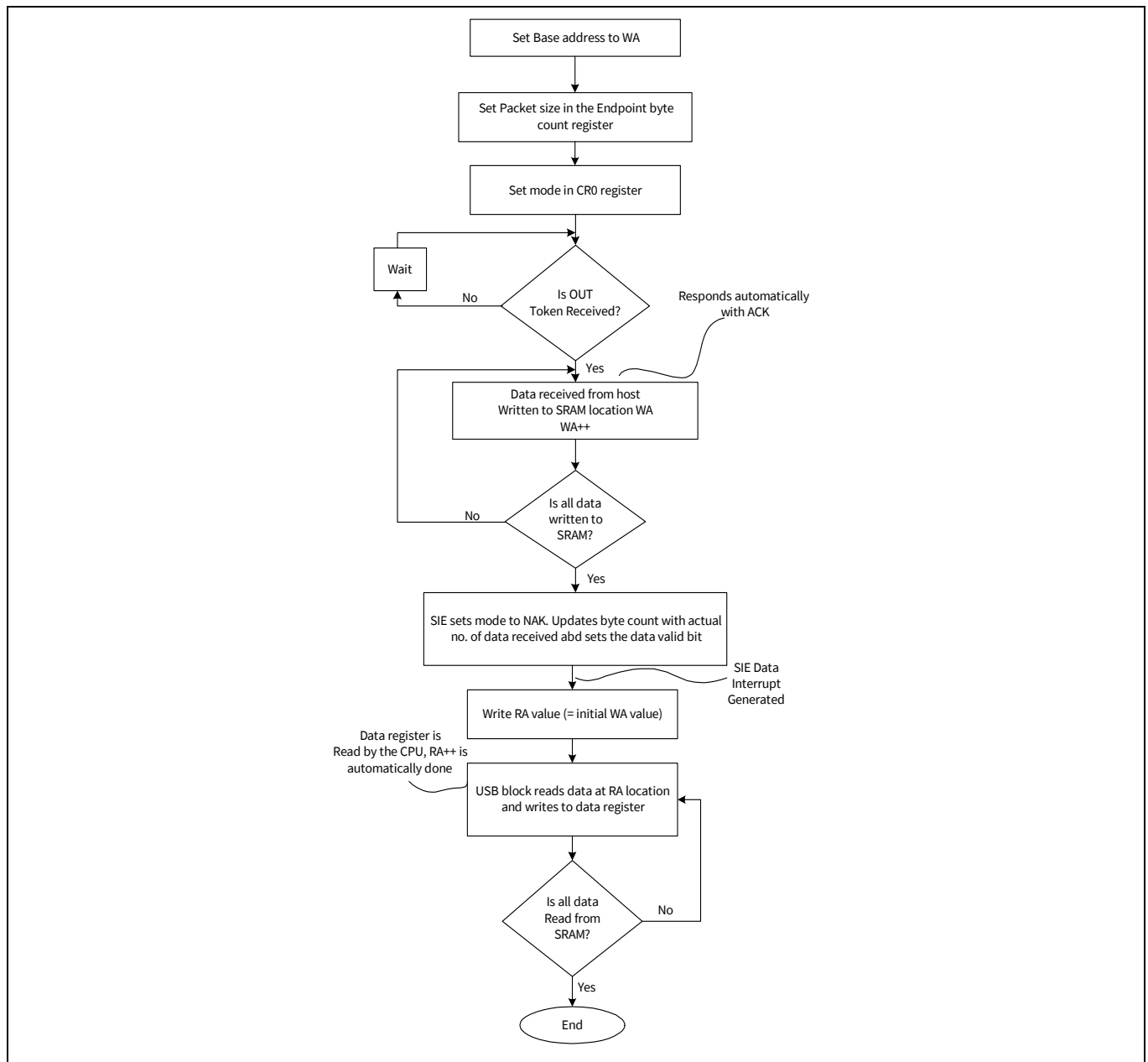
Figure 32-4. No DMA access OUT transaction
