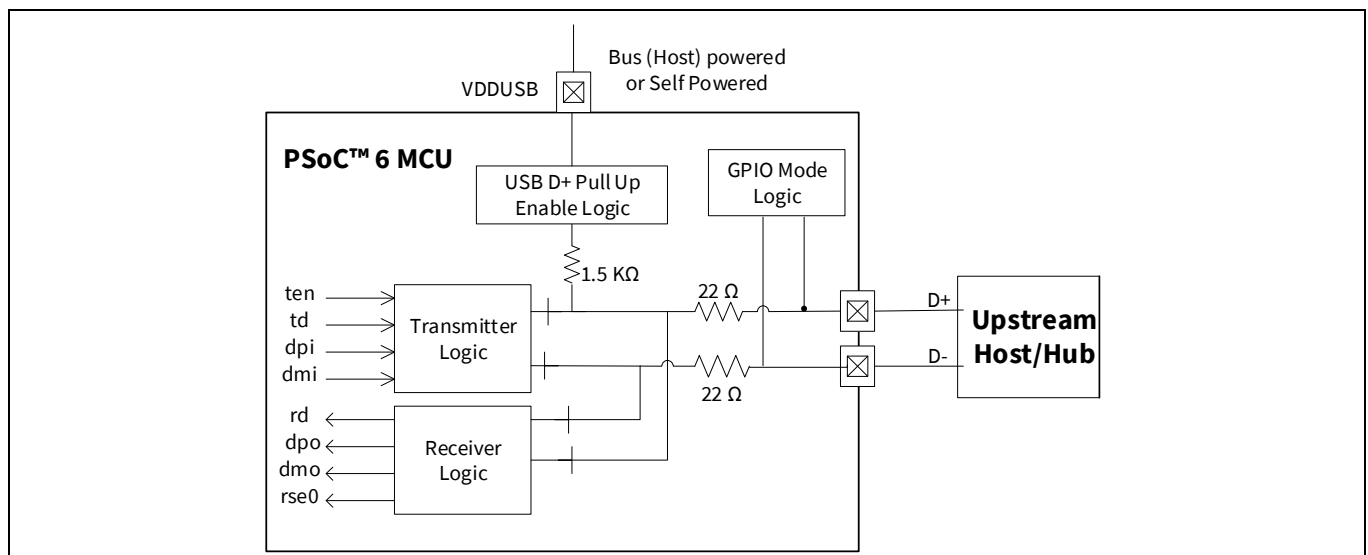
Figure 32-2. USB PHY architecture
