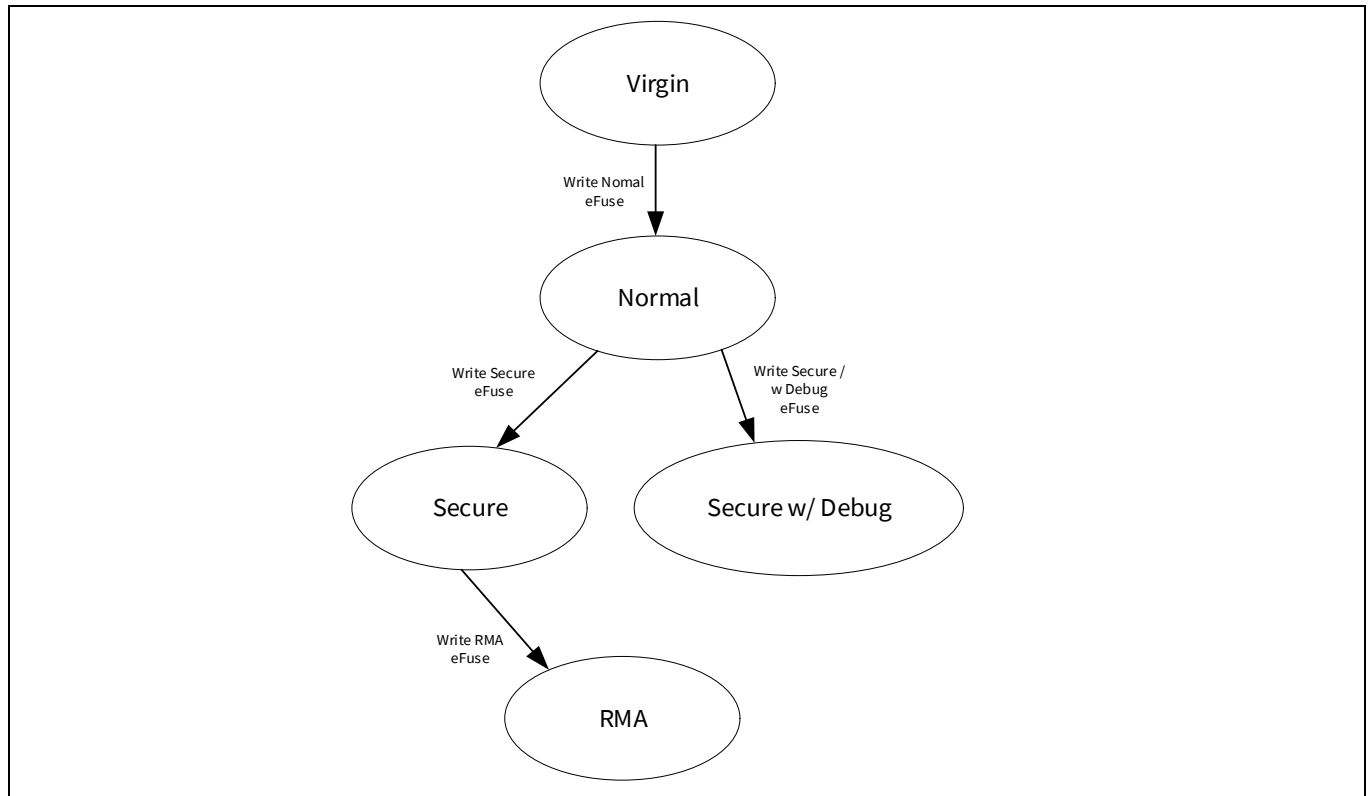
Figure 17-1. PSoC™ 6 MCU life cycle stage transitions
