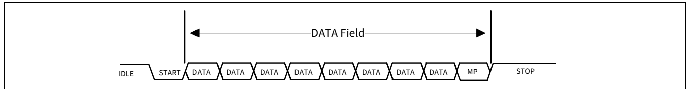
Figure 27-23. UART MP address and data frame
