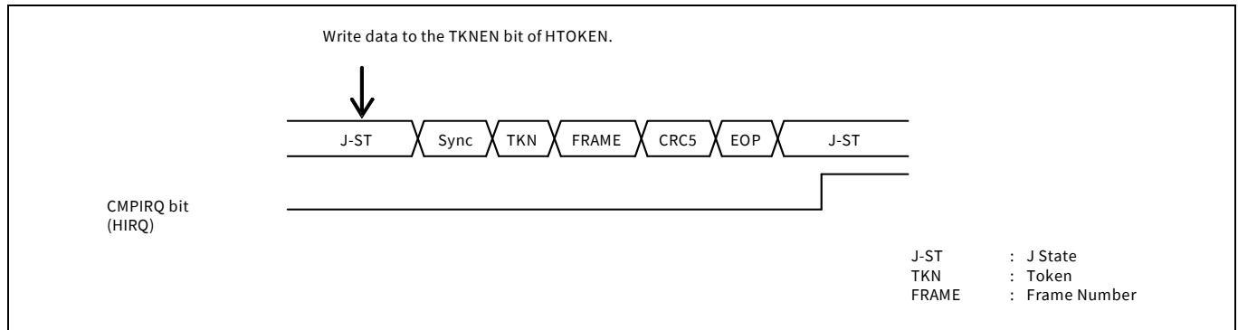
Figure 31-10. EOP interrupt timing diagram (for SOF token)
