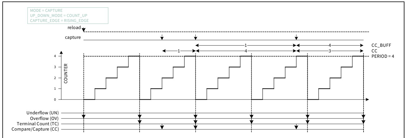
Figure 30-17. Capture in up counting mode
