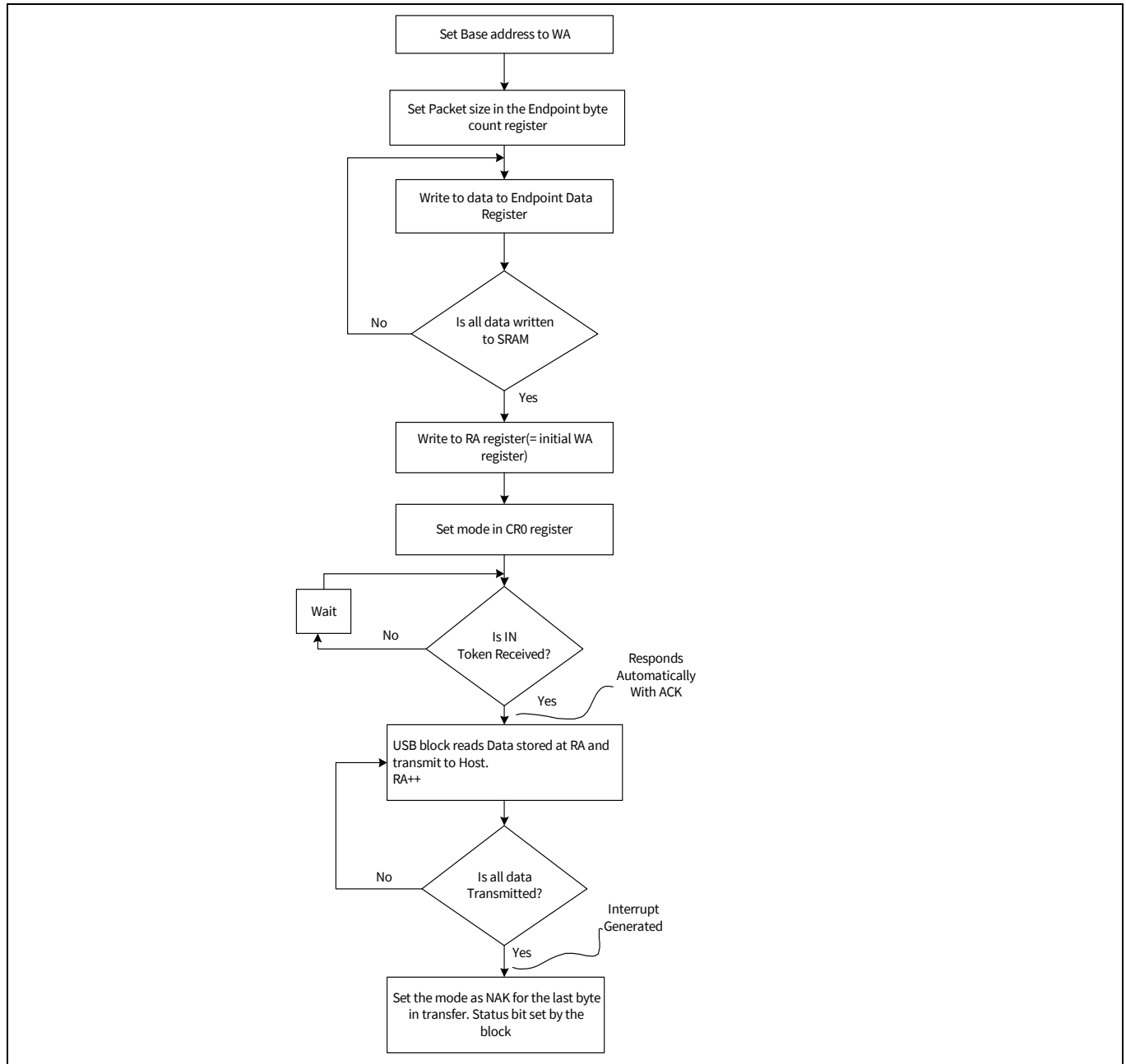
Figure 32-3. No DMA access IN transaction
