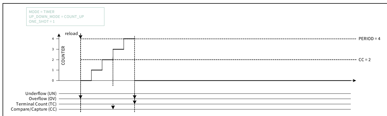
Figure 30-8. Timer in one-shot mode
