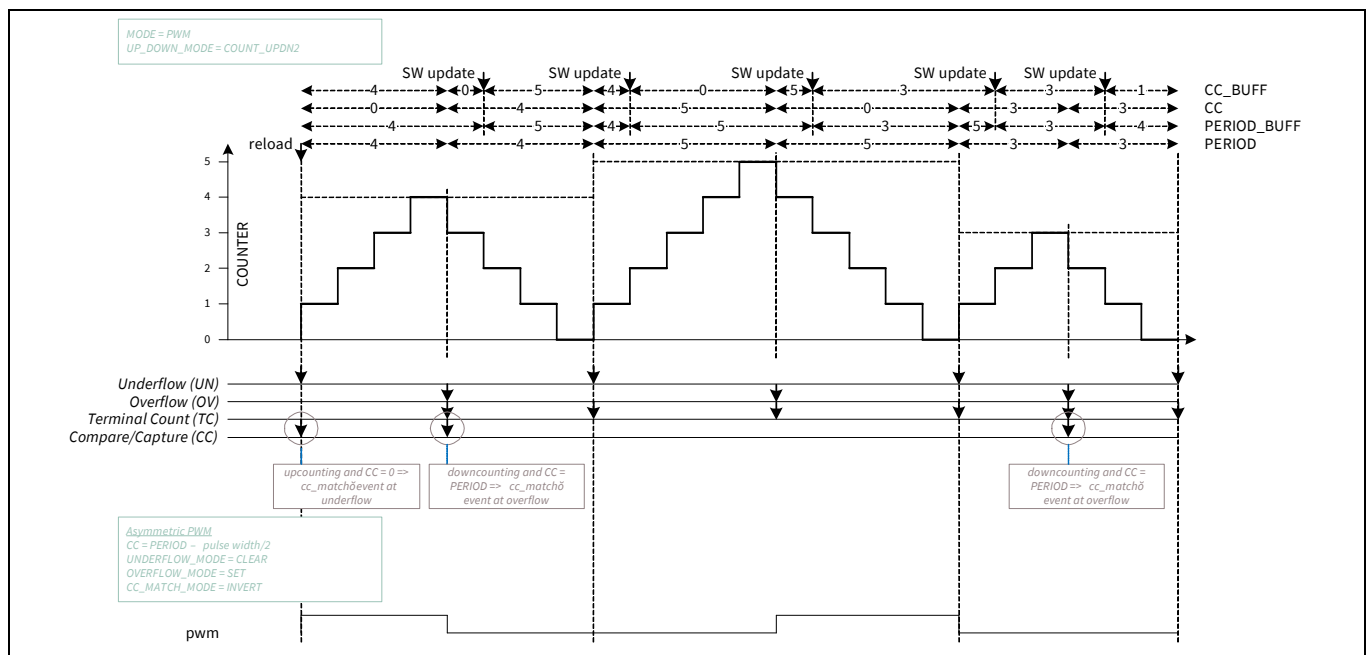
Figure 30-37. Asymmetric PWM when compare = 0 or period
