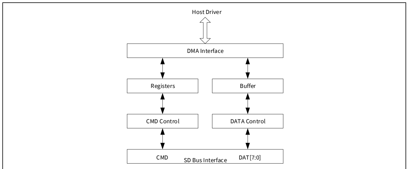
Figure 26-4. Data flow
