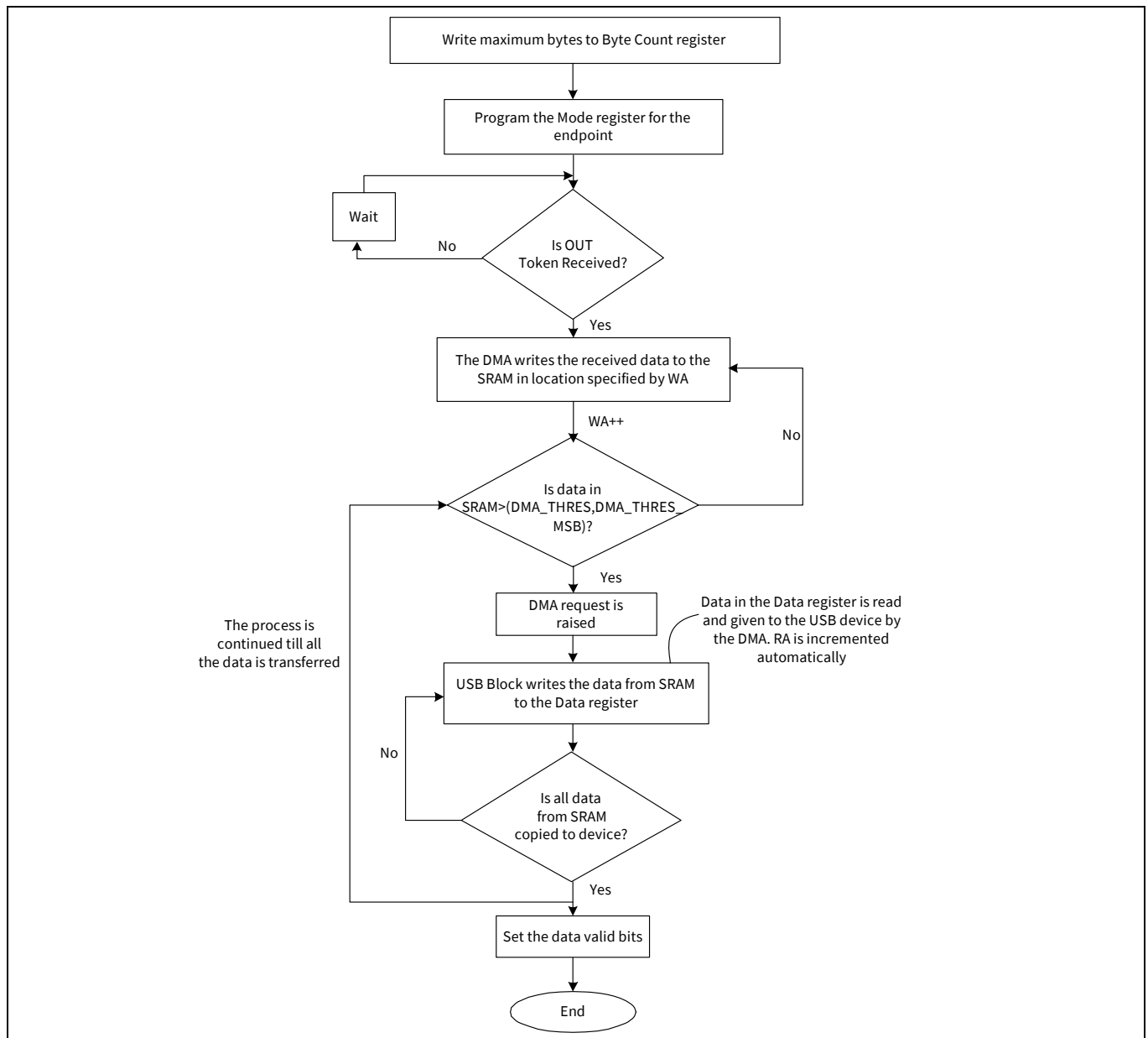
Figure 32-8. OUT Transaction using automatic DMA mode
