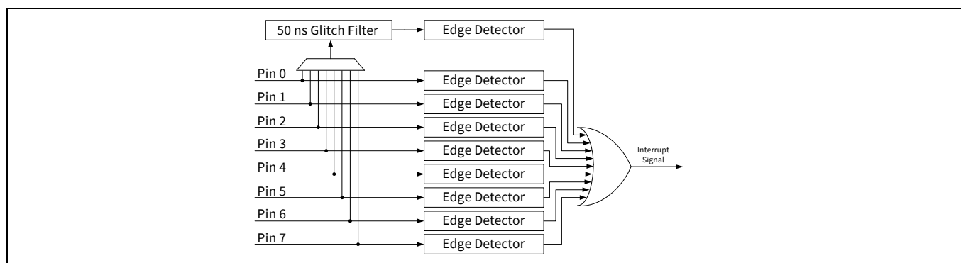
Figure 23-6. GPIO edge detect block architecture
