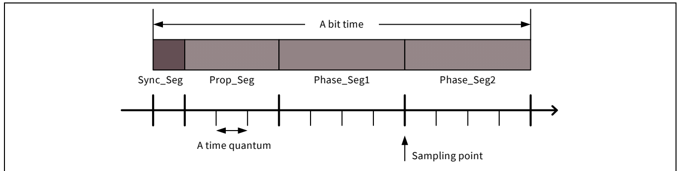
Figure 29-12. Bit time construction
