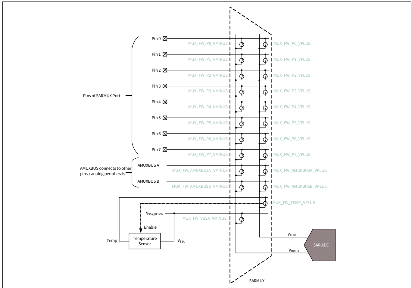
Figure 36-5. SARMUX switches
