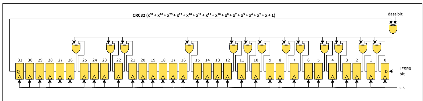
Figure 12-3. CRC32 functionality
