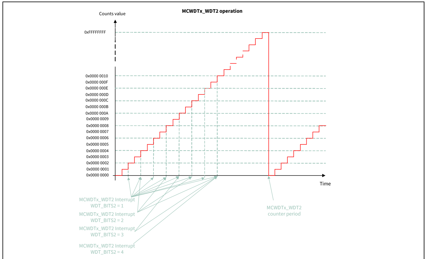
Figure 24-5. MCWDTx_WDT2 operation
