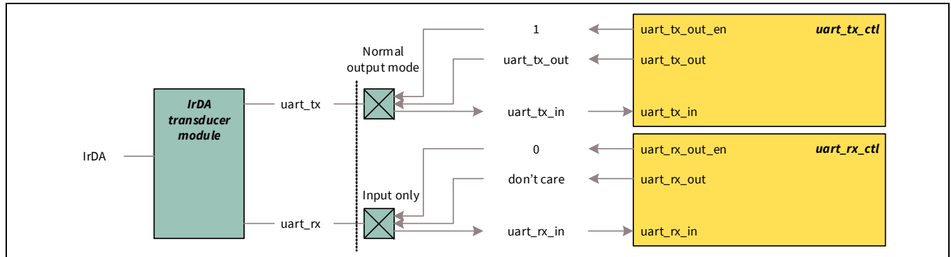
Figure 27-35. IrDA mode I/O pad connections
