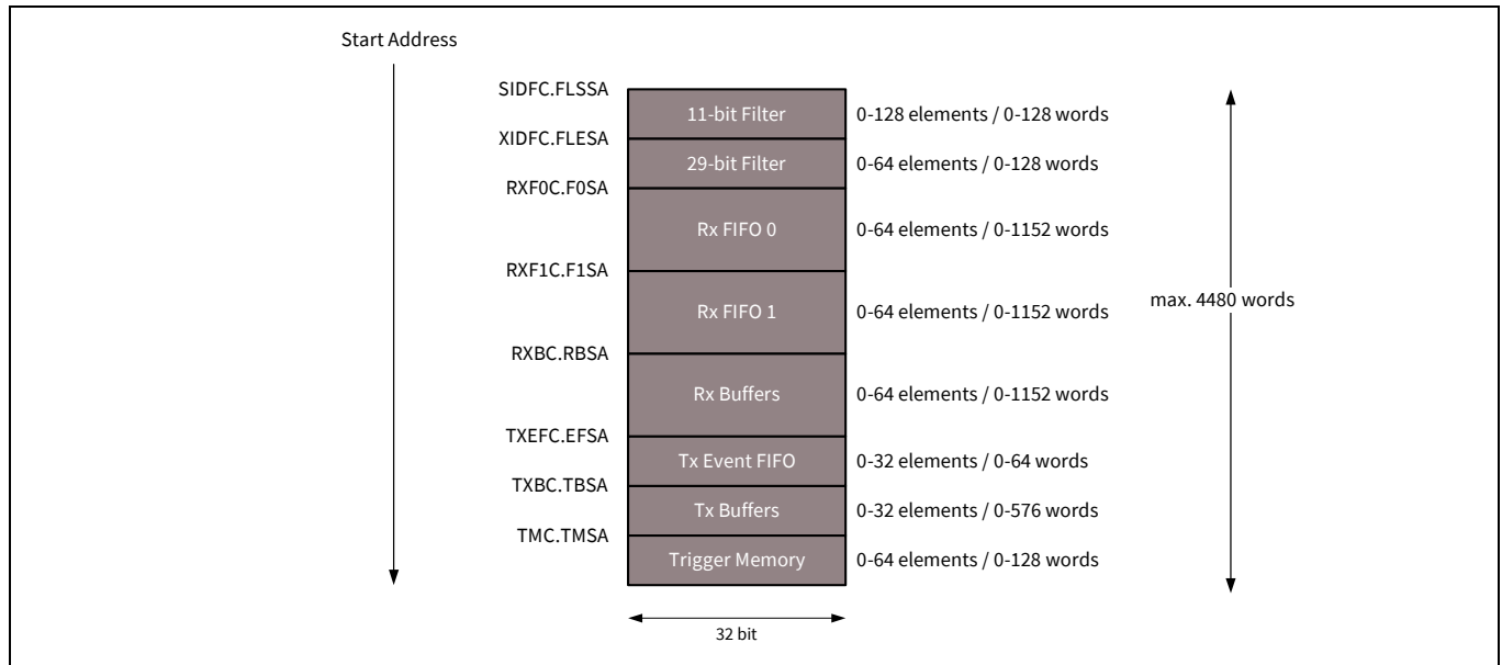
Figure 29-15. Message RAM configuration
