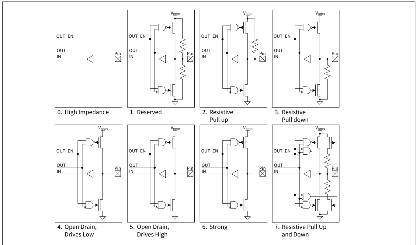
Figure 23-4. Peripheral I/O drive mode block diagrams
