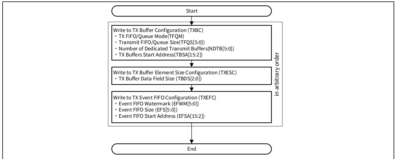
Figure 29-35. TX buffer and TX FIFO/queue configuration
