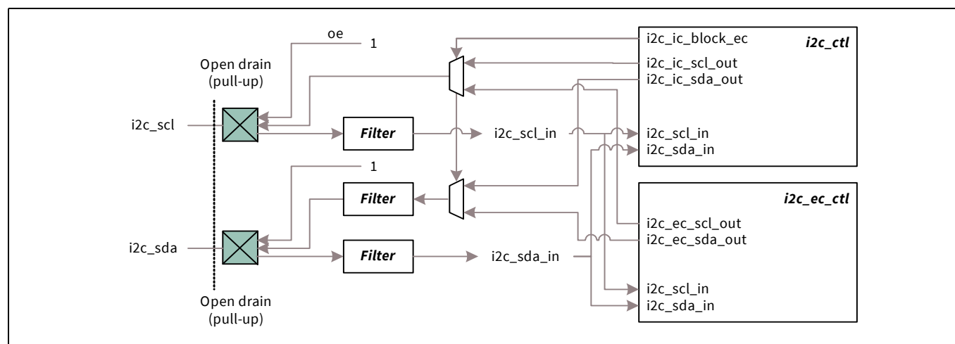
Figure 27-44. I 2 C I/O pad connections
