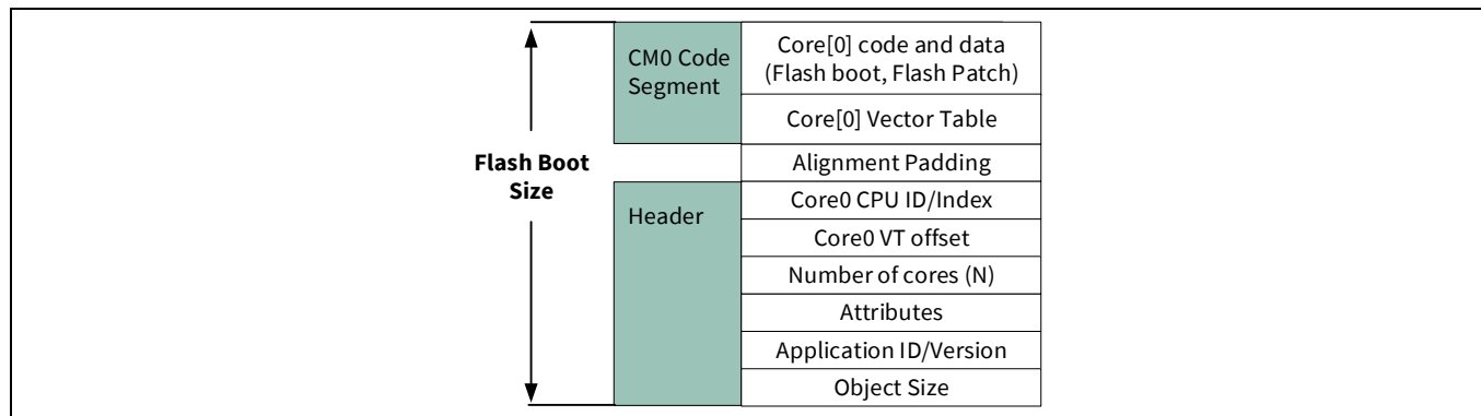
Figure 15-4. Flash boot layout
