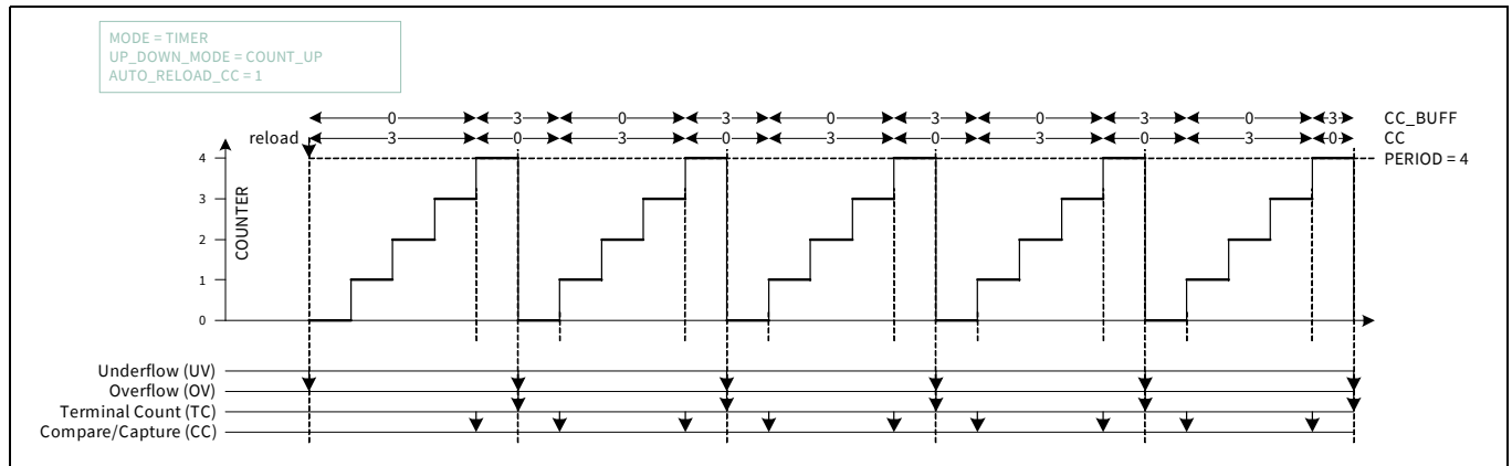
Figure 30-11. Use of CC and CC_BUFF register bits
