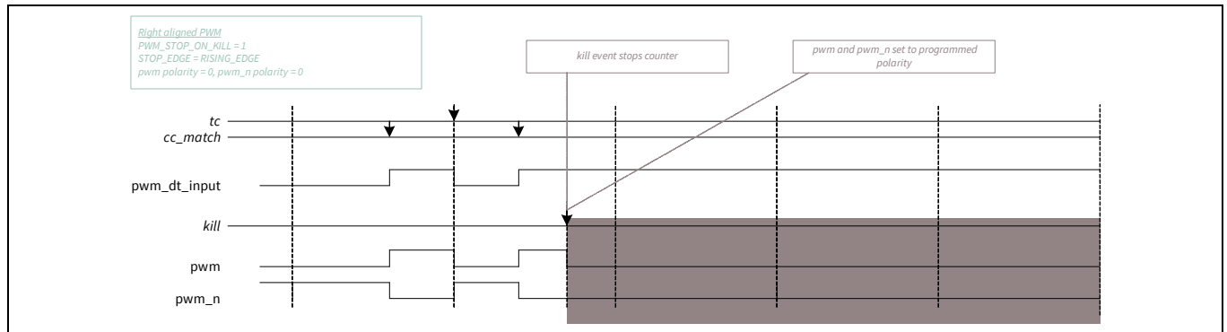
Figure 30-31. PWM stop on kill
