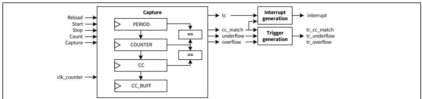
Figure 30-16. Capture functionality
