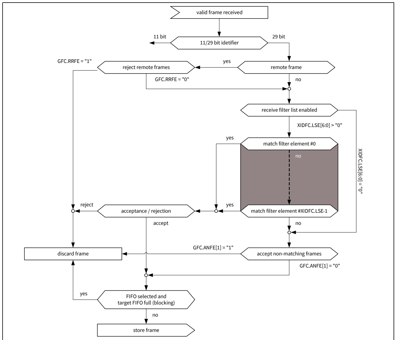
Figure 29-6. Extended Message ID filter path
