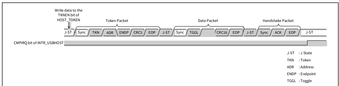
Figure 31-9. EOP interrupt timing diagram (for IN/OUT/SETUP token)
