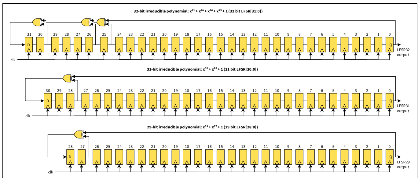
Figure 12-4. Fixed Fibonacci-based LFSRs
