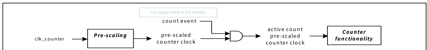
Figure 30-2. Counter clock generation
