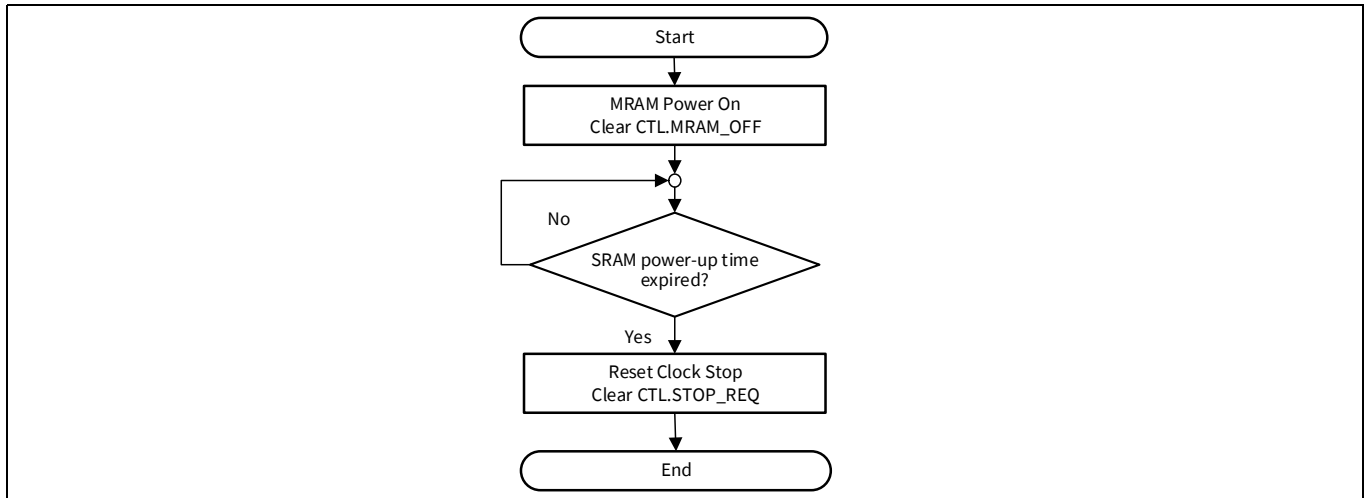
Figure 29-29. Message RAM on procedure
