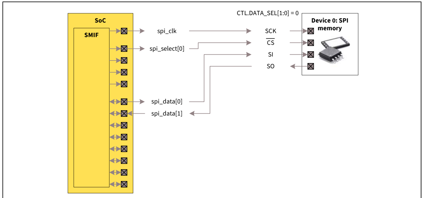
Figure 28-4. Single SPI memory device 0 connected to spi_data[1:0]
