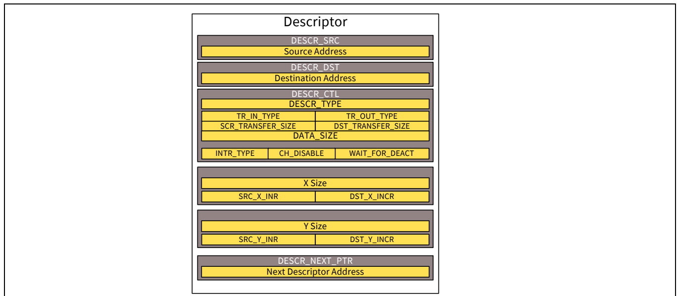
Figure 11-1. Descriptor structure
