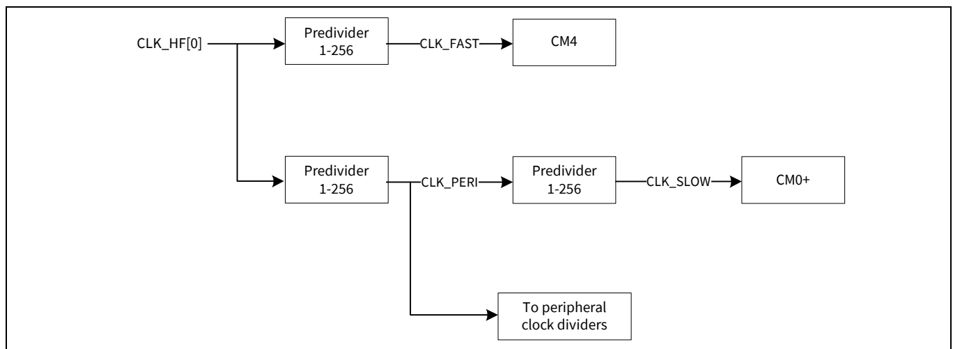
Figure 21-4. CLK_HF[0] distribution
