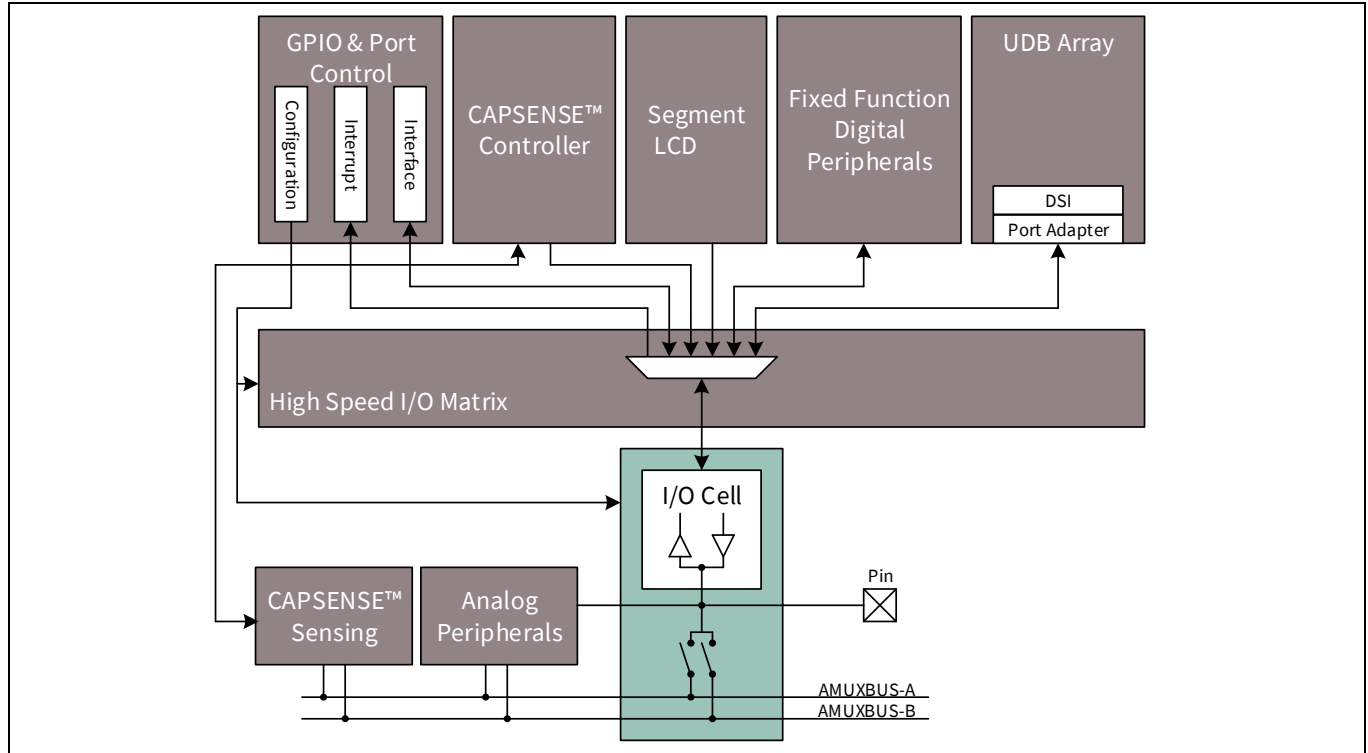
Figure 23-1. GPIO interface overview
