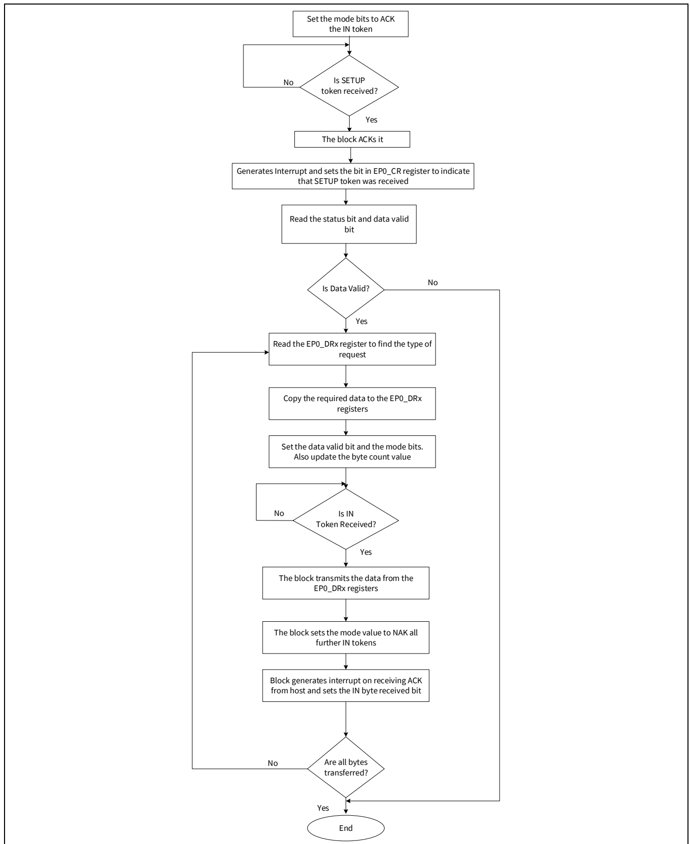
Figure 32-9. Control endpoint IN transaction
