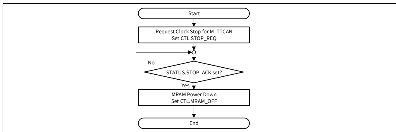
Figure 29-28. Message RAM OFF operation
