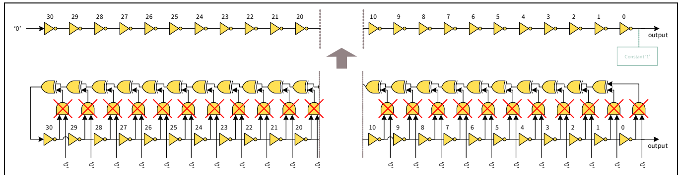
Figure 12-13. FIRO31 “stopped”
