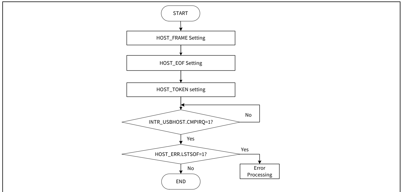
Figure 31-7. SOF token flow chart
