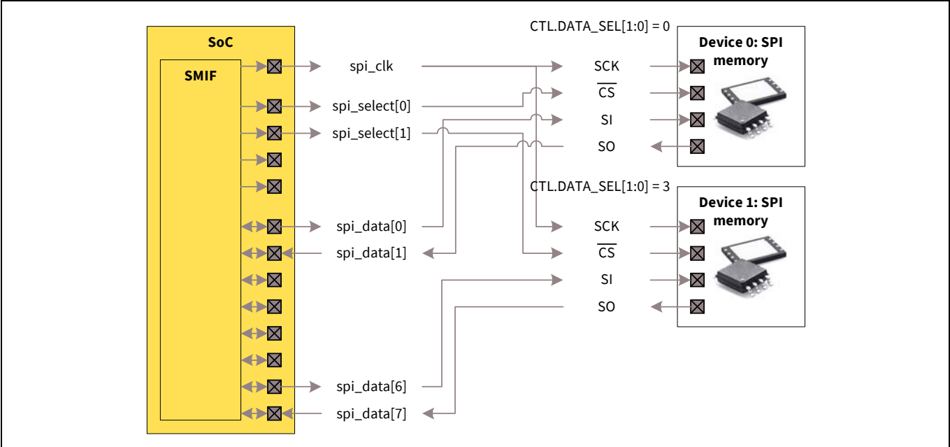
Figure 28-6. Single SPI memory devices 0 and 1 - Dedicated data signal
