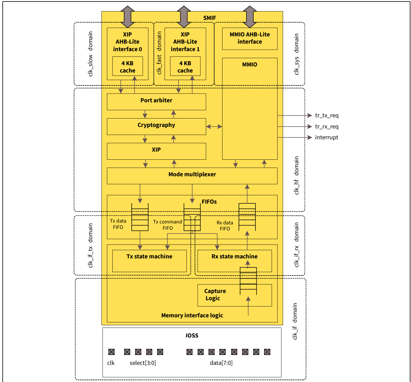
Figure 28-1. SMIF hardware block diagram
