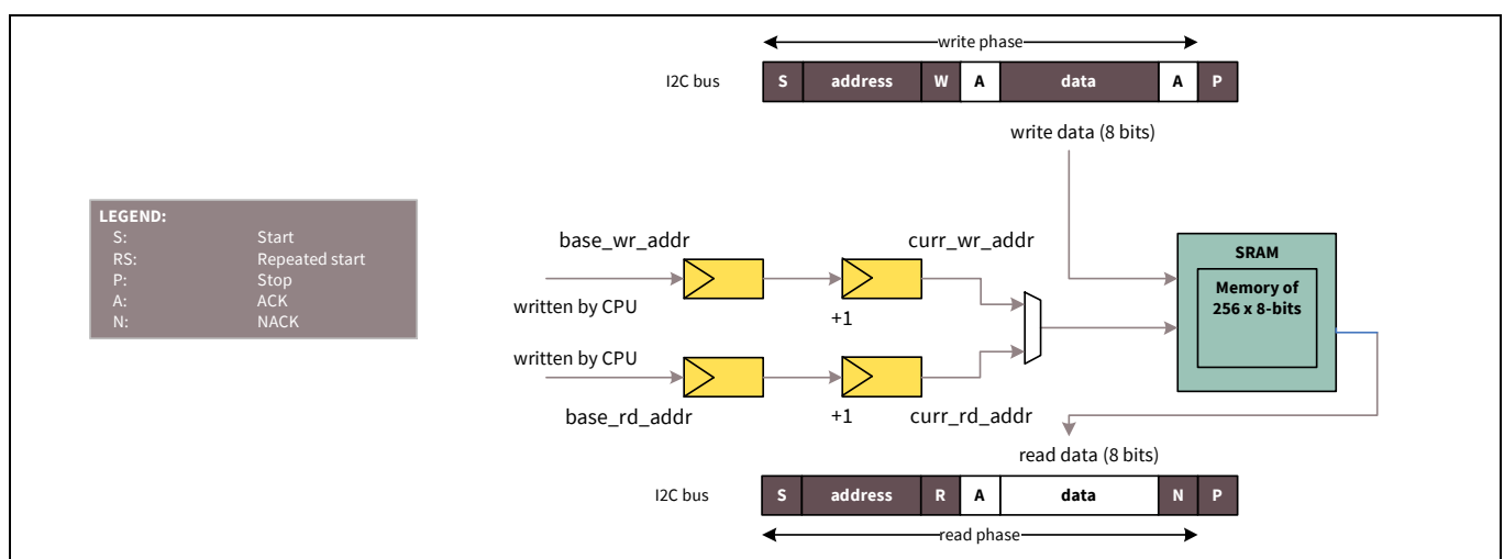
Figure 27-41. I 2 C command-response mode
