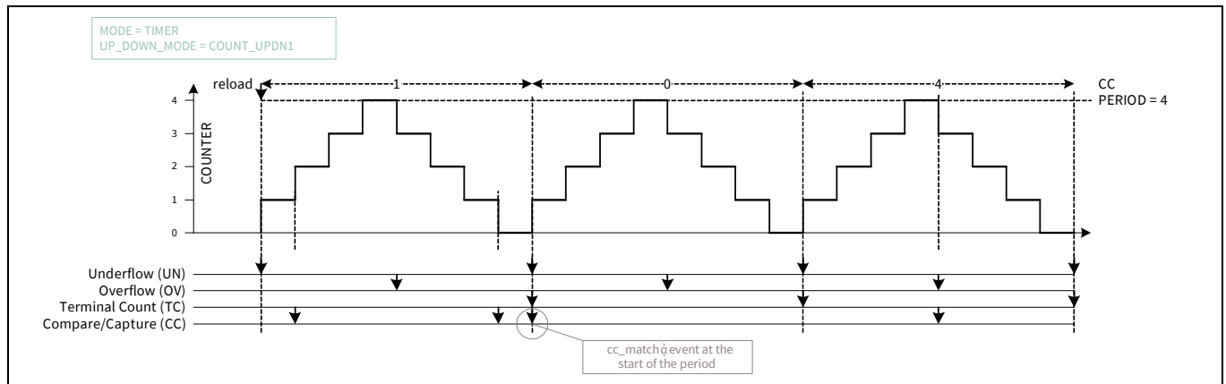
Figure 30-14. Up/down counting mode with different CC values
