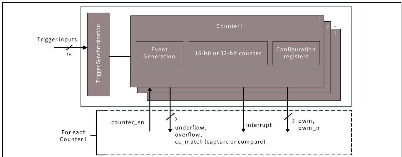
Figure 30-1. TCPWM block diagram
