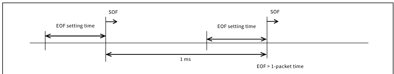
Figure 31-8. SOF timing
