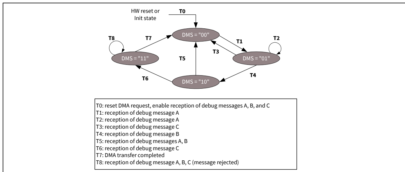
Figure 29-9. Debug message handling state machine
