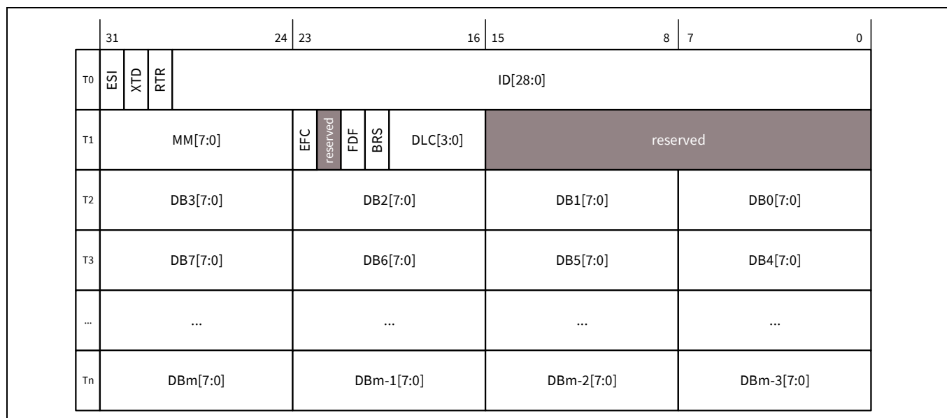
Figure 29-17. TX buffer element
