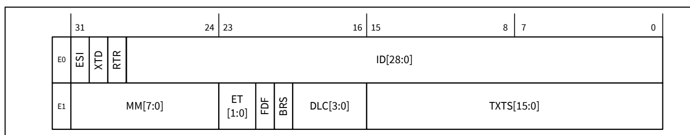
Figure 29-18. TX event FIFO element
