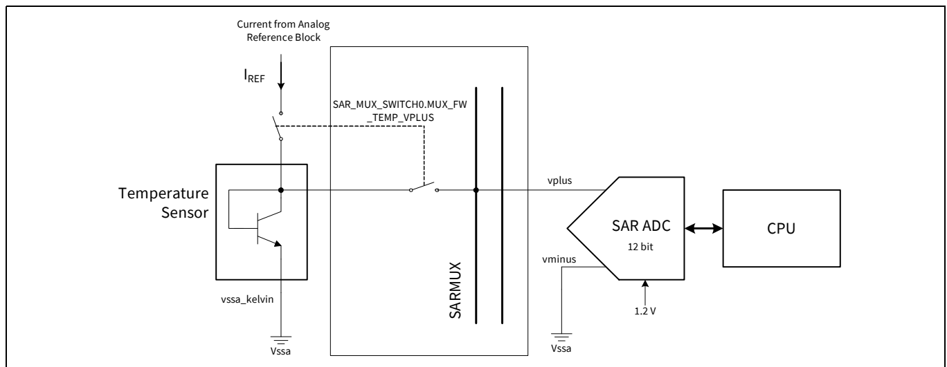
Figure 37-1. Temperature sensing mechanism
