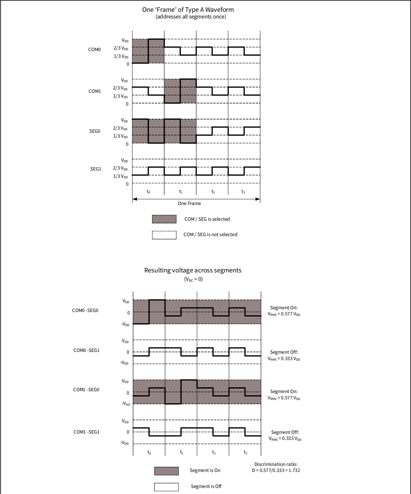
Figure 33-4. PWM1/3 Type-A waveform example
