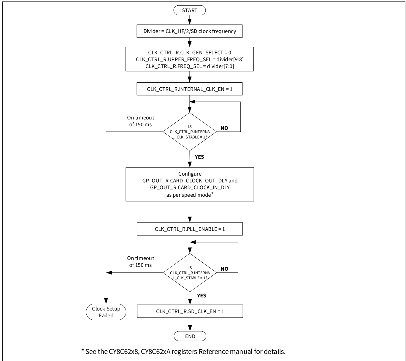
Figure 26-10. Clock setup
