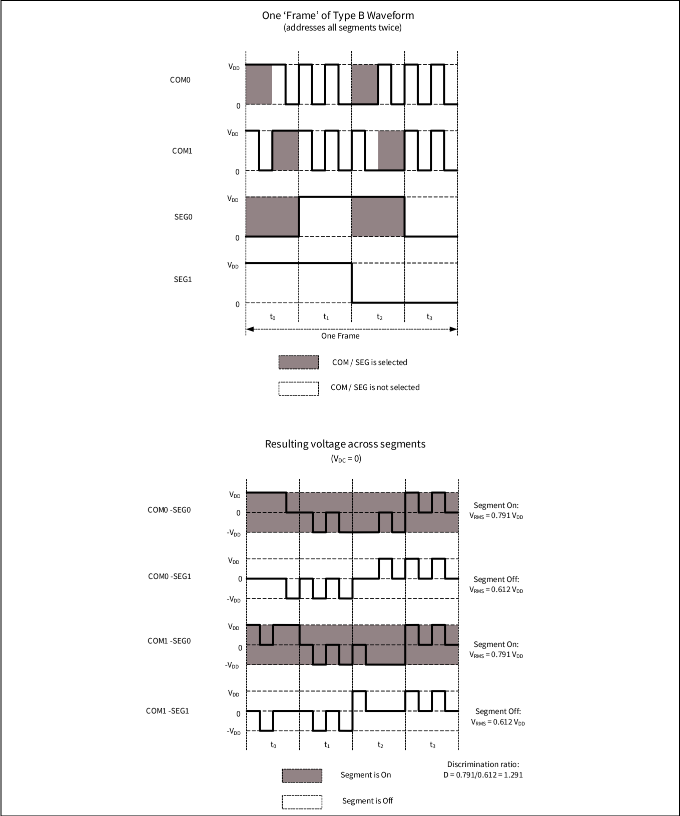
Figure 33-7. Digital correlation Type-B waveform
