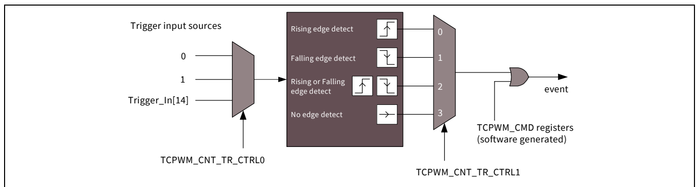
Figure 30-5. TCPWM input events
