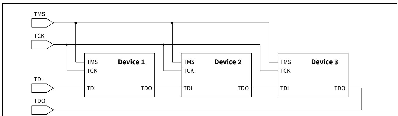
Figure 13-3. JTAG interface to multiple ICs on a circuit board
