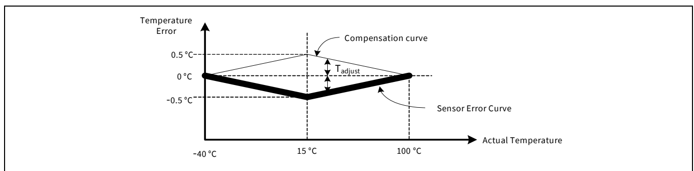
Figure 37-2. Temperature error compensation
