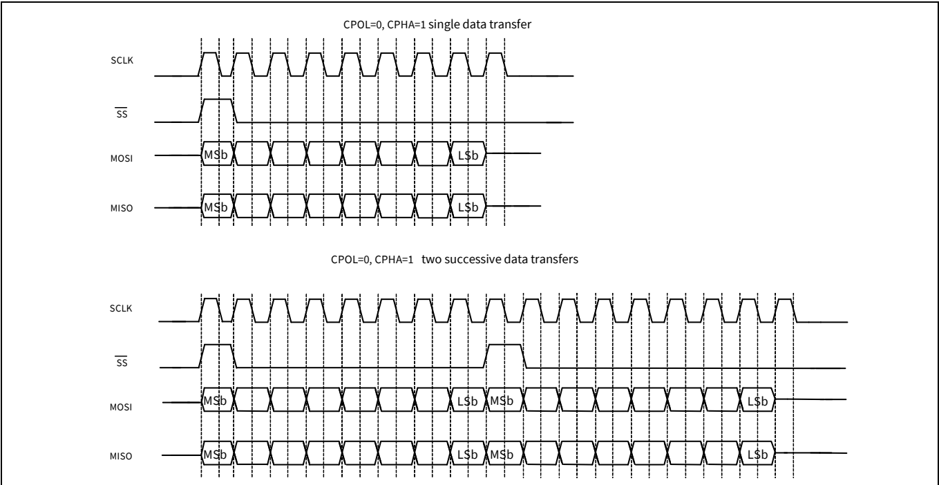
Figure 27-6. SPI TI data transfer example
