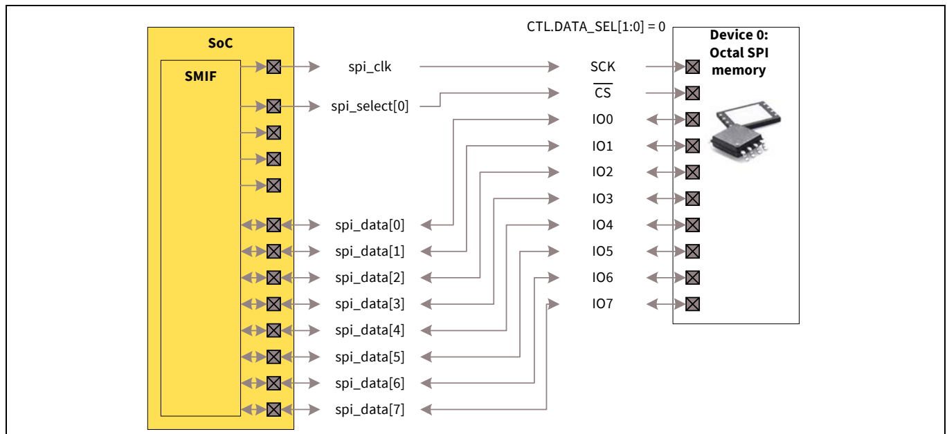
Figure 28-12. Octal SPI memory device 0
