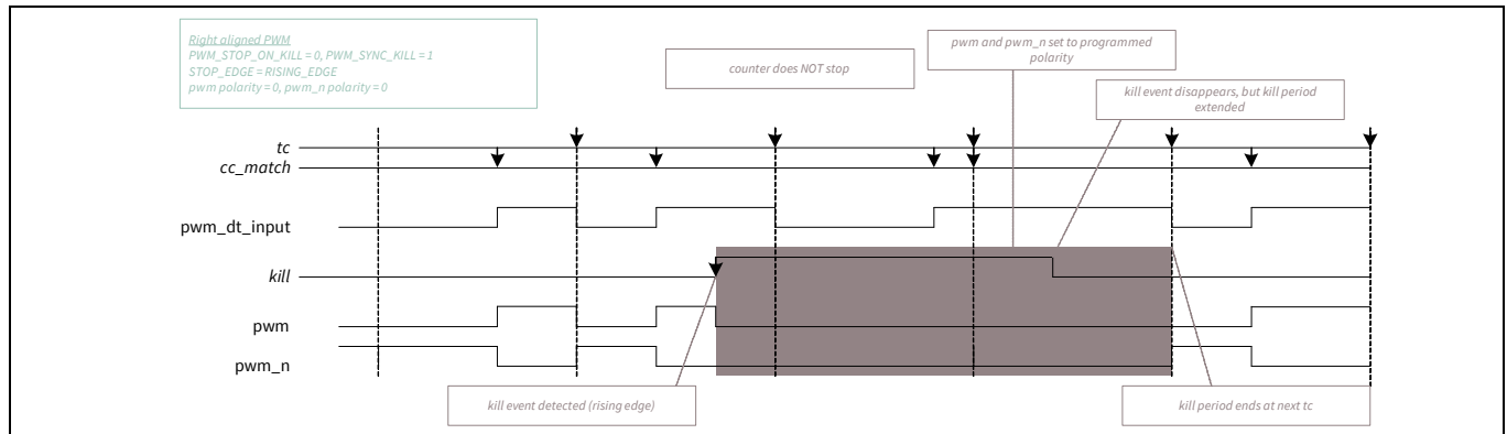
Figure 30-33. PWM sync kill
