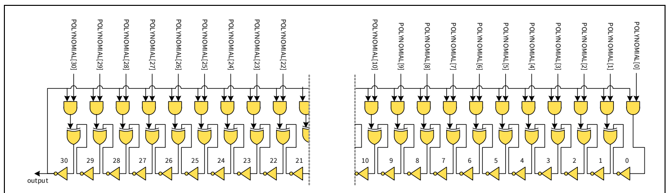
Figure 12-9. Flexible Galois-based ring oscillators: GARO31
