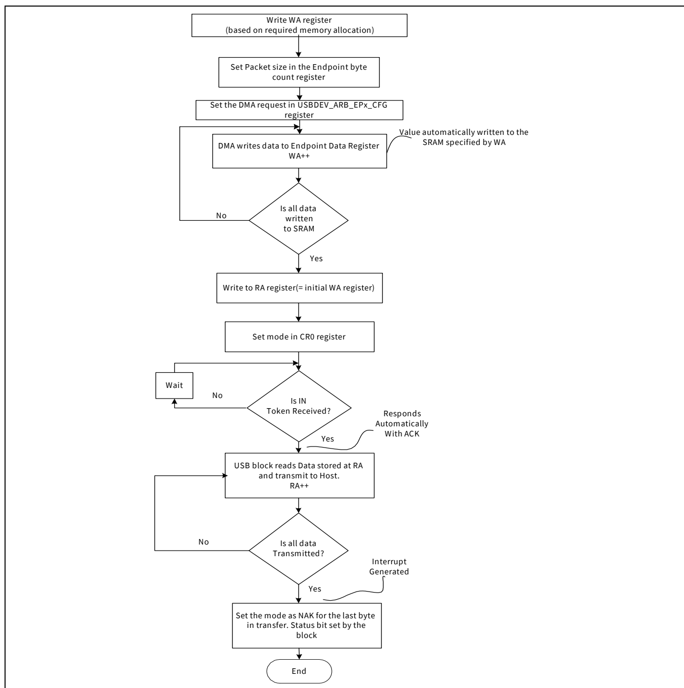
Figure 32-5. Manual DMA IN transaction
