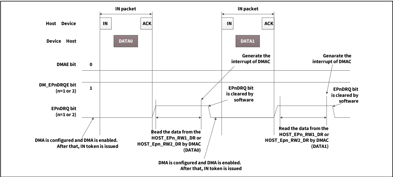
Figure 31-16. Automatic data transfer mode: IN direction
