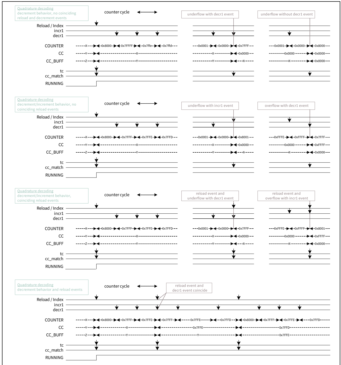
Figure 30-22. Quadrature mode timing cases
