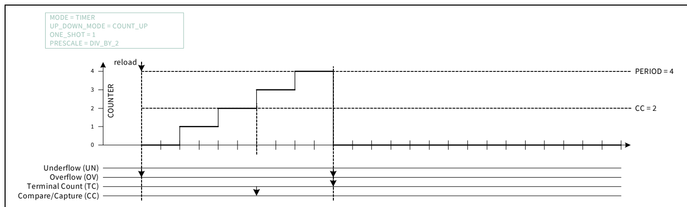
Figure 30-9. Timer clock pre-scaling
