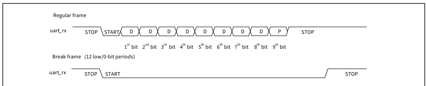
Figure 27-20. UART – Regular frame and break frame
