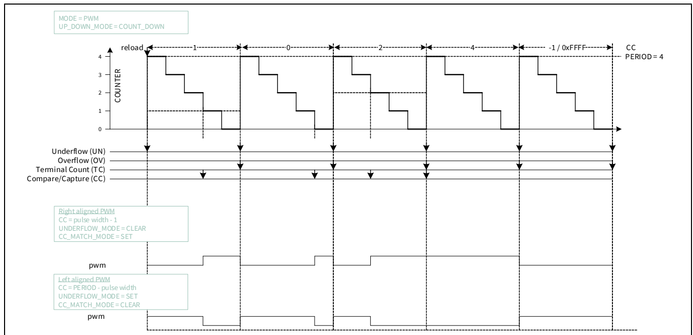
Figure 30-28. Right- and left-aligned down counting PWM
