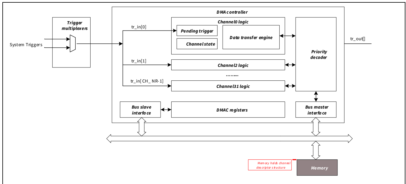
Figure 11-2. DMAC controller overview
