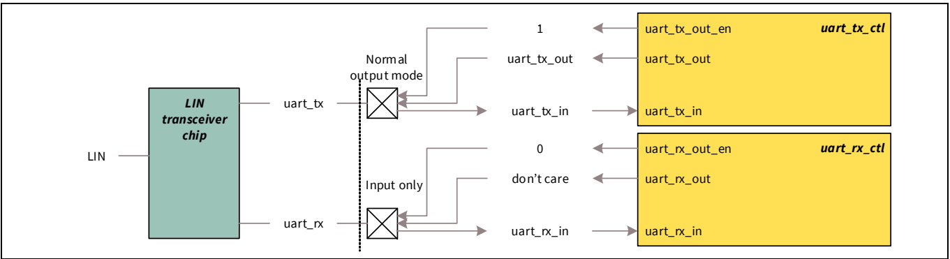
Figure 27-34. LIN mode I/O pad connections
