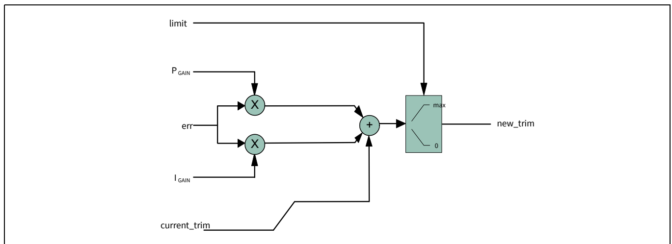
Figure 21-3. FLL error correction diagram
