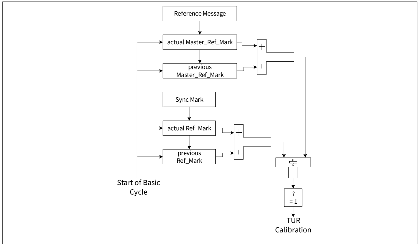
Figure 29-23. TTCAN level 0 and level 2 drift compensation
