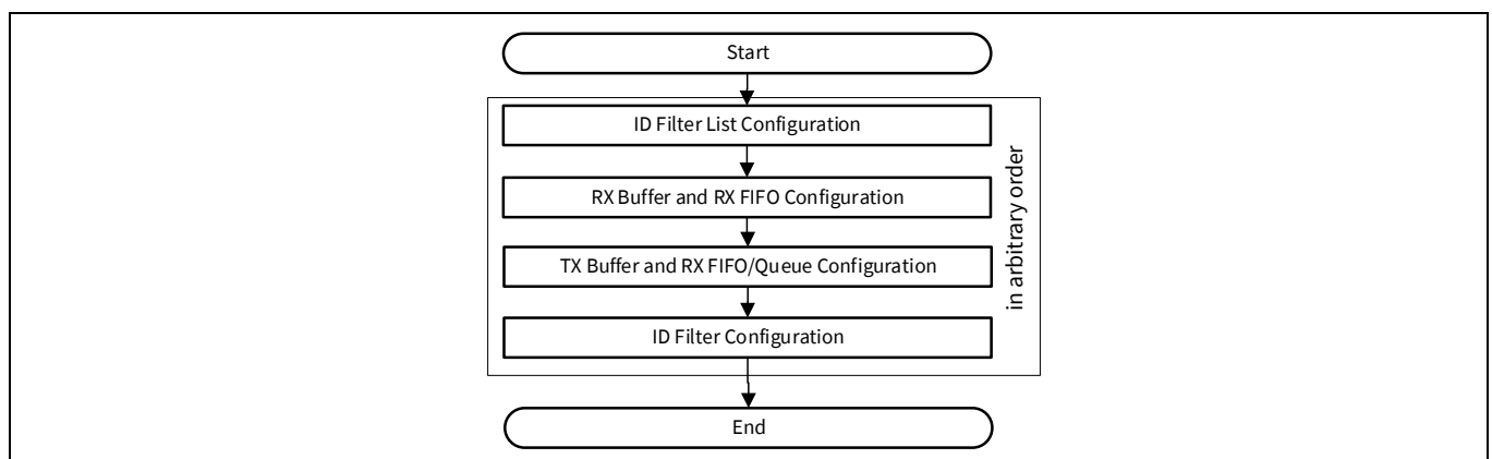
Figure 29-32. Message RAM configuration overview
