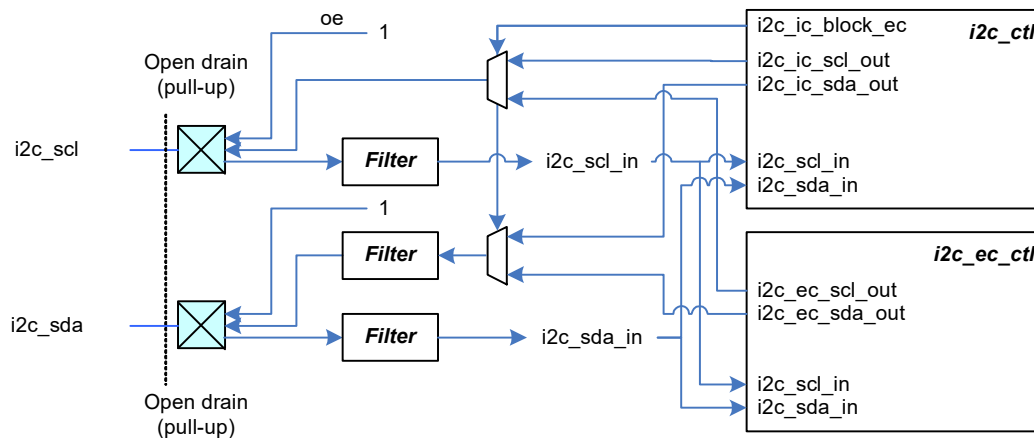
Figure 28-44. I 2 C I/O Pad Connections
