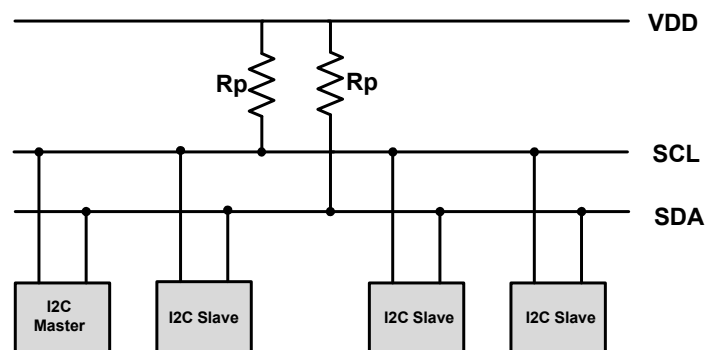
Figure 28-36. I 2 C Interface Block Diagram
