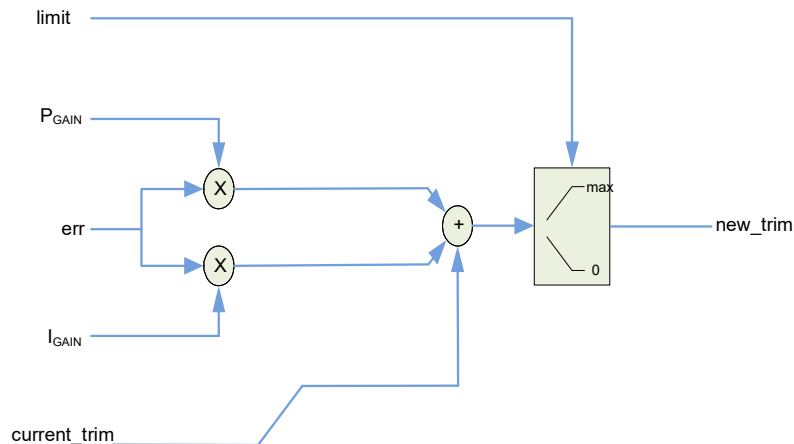
Figure 21-3. FLL Error Correction Diagram
