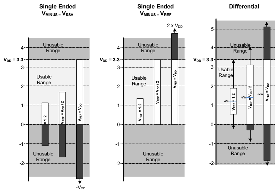
Figure 38-2. Input Range
