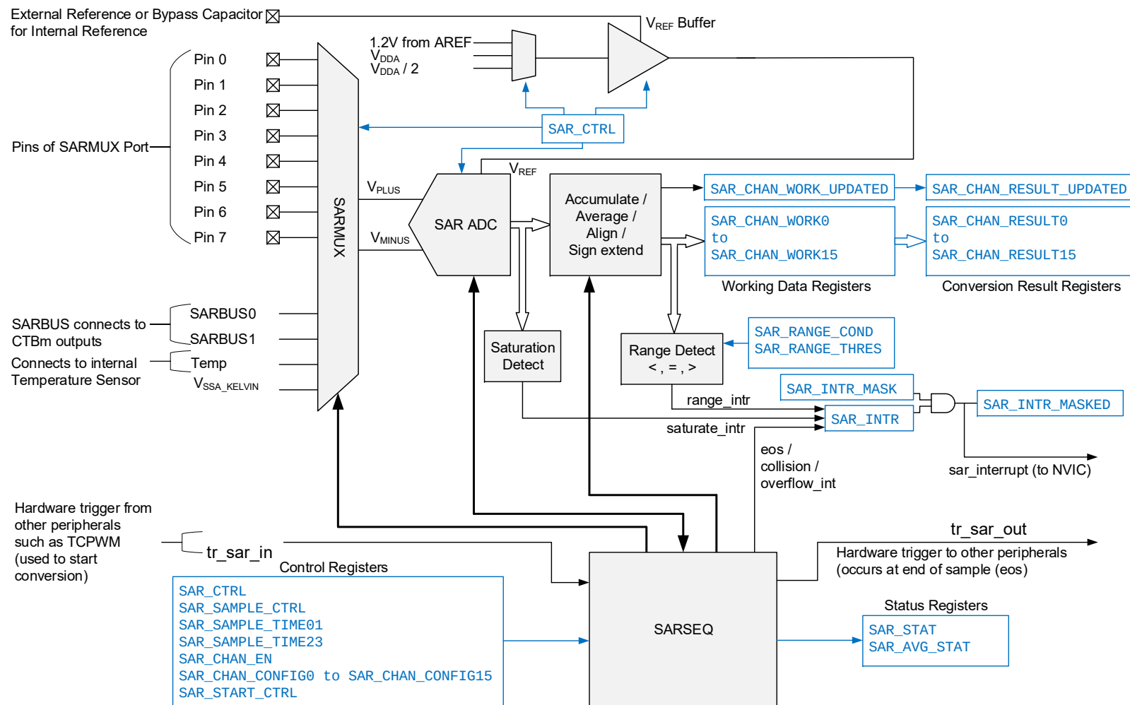
Figure 38-1. Block Diagram
