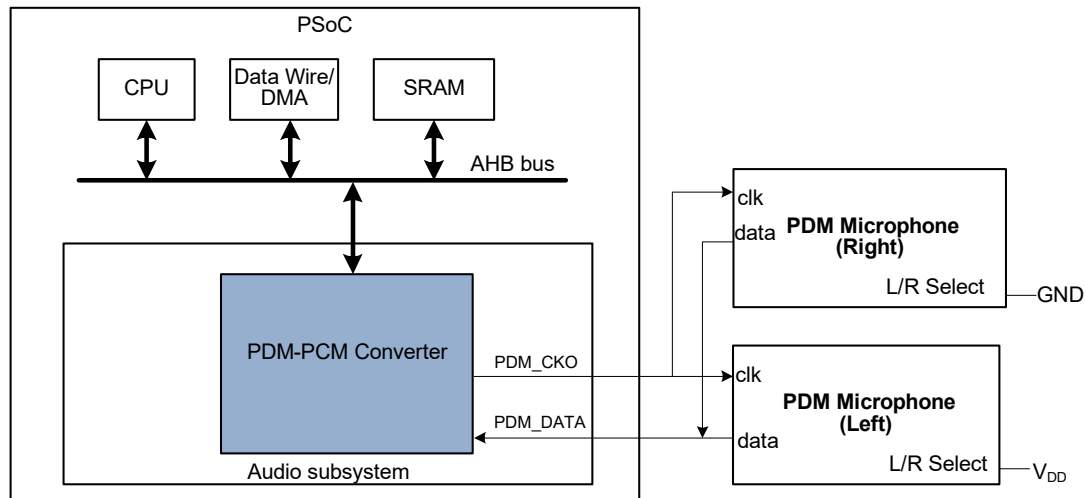
Figure 32-1. Block Diagram
