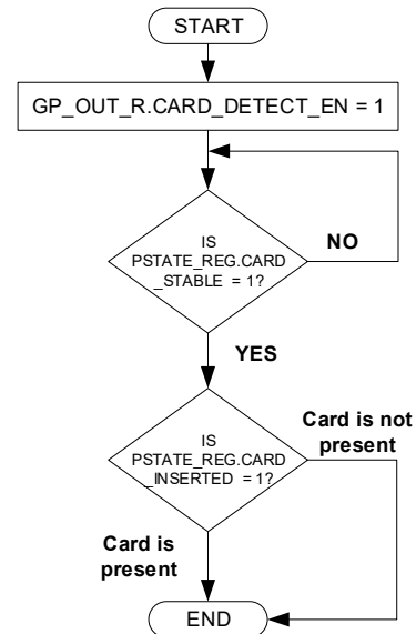
Figure 27-7. Card Status Check Sequence
