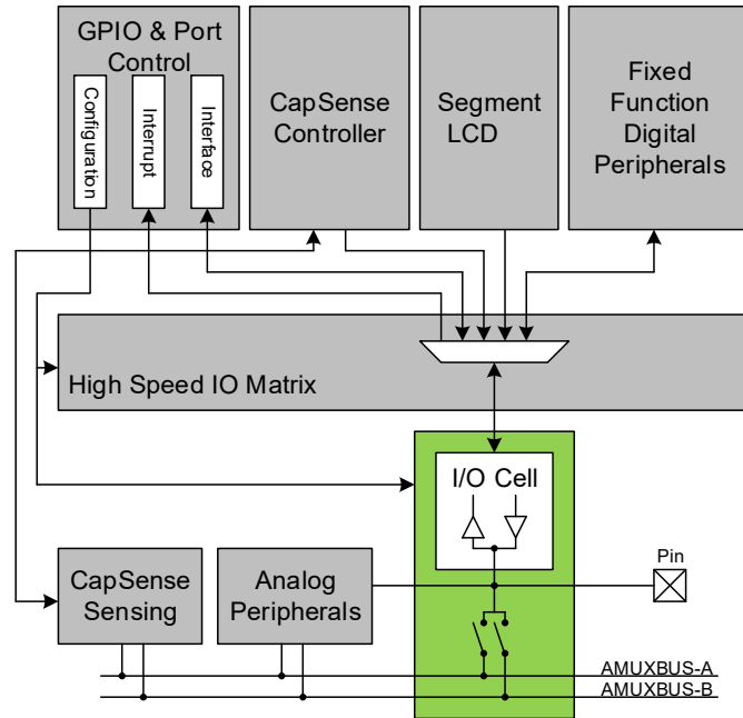
Figure 23-1. GPIO Interface Overview
