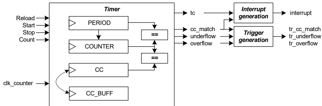
Figure 30-6. Timer Functionality
