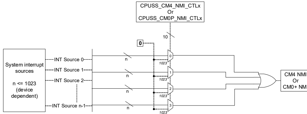
Figure 8-5. NMI Trigger
