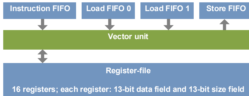
Figure 12-16. Vector Unit
