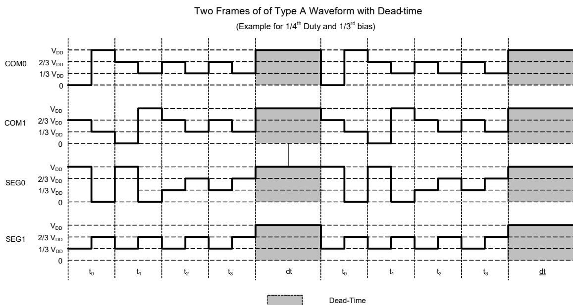
Figure 35-8. Dead-Time Contrast Control
