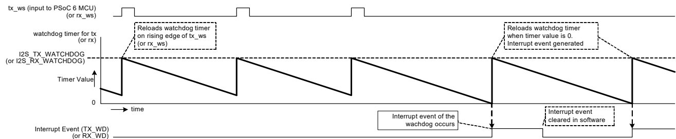
Figure 31-10. Watchdog Timer Working
