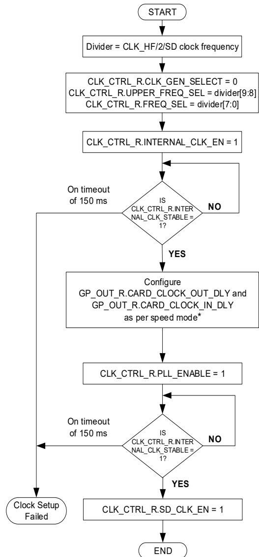
Figure 27-10. Clock Setup
