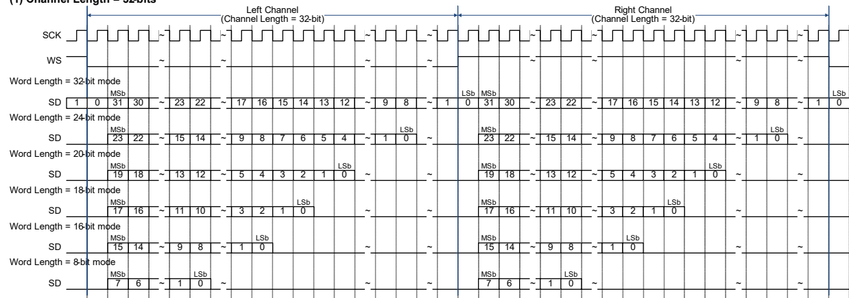
Figure 31-2. Standard I 2 S Format (Word Length and Channel Length Combination Timing Diagrams)
