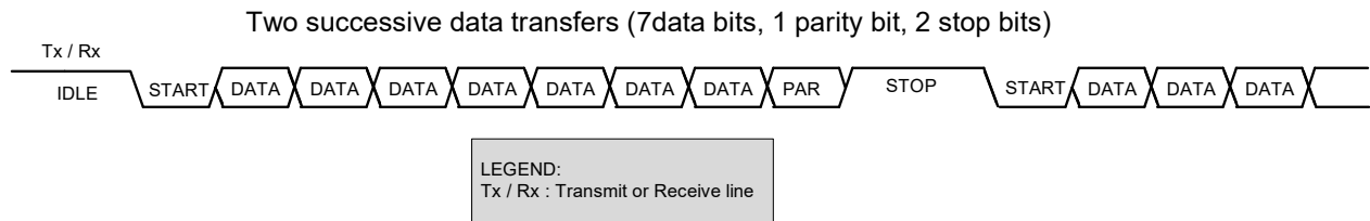
Figure 28-15. UART, Standard Protocol Example
