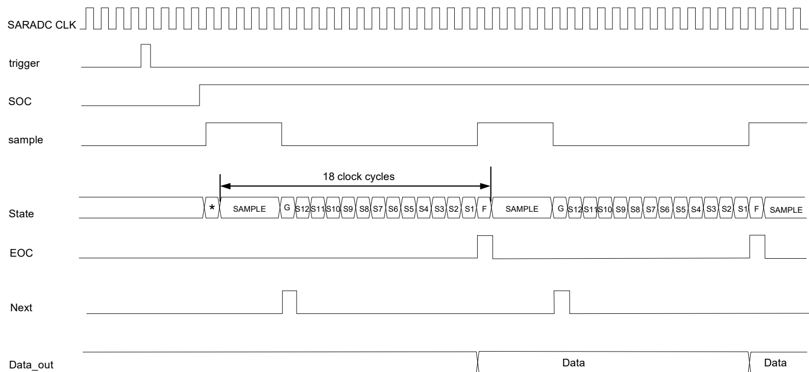
Figure 38-4. SAR ADC Timing
