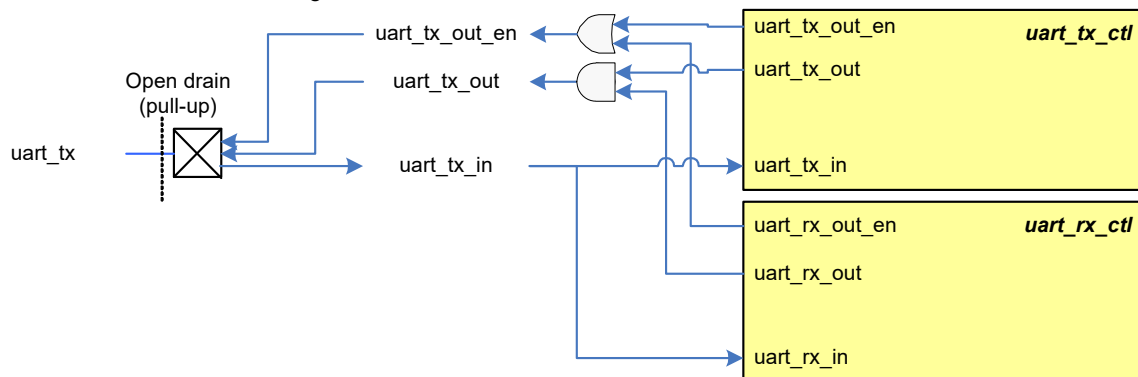
Figure 28-33. SmartCard Mode I/O Pad Connections
