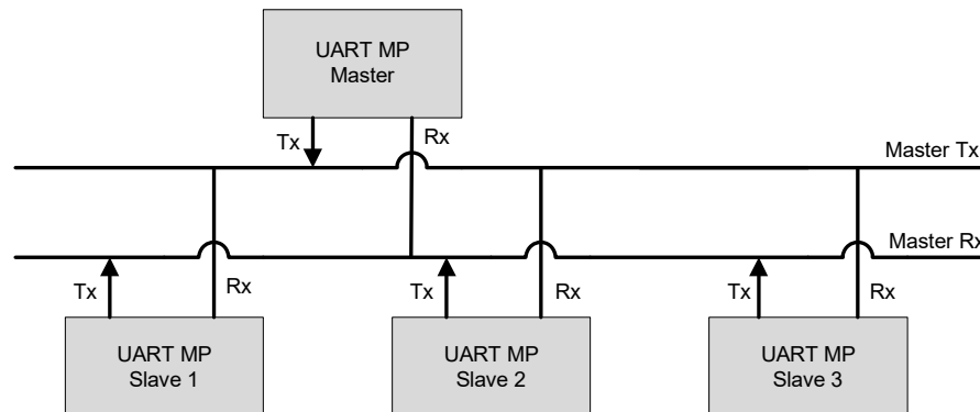
Figure 28-22. UART MP Mode Bus Connections
