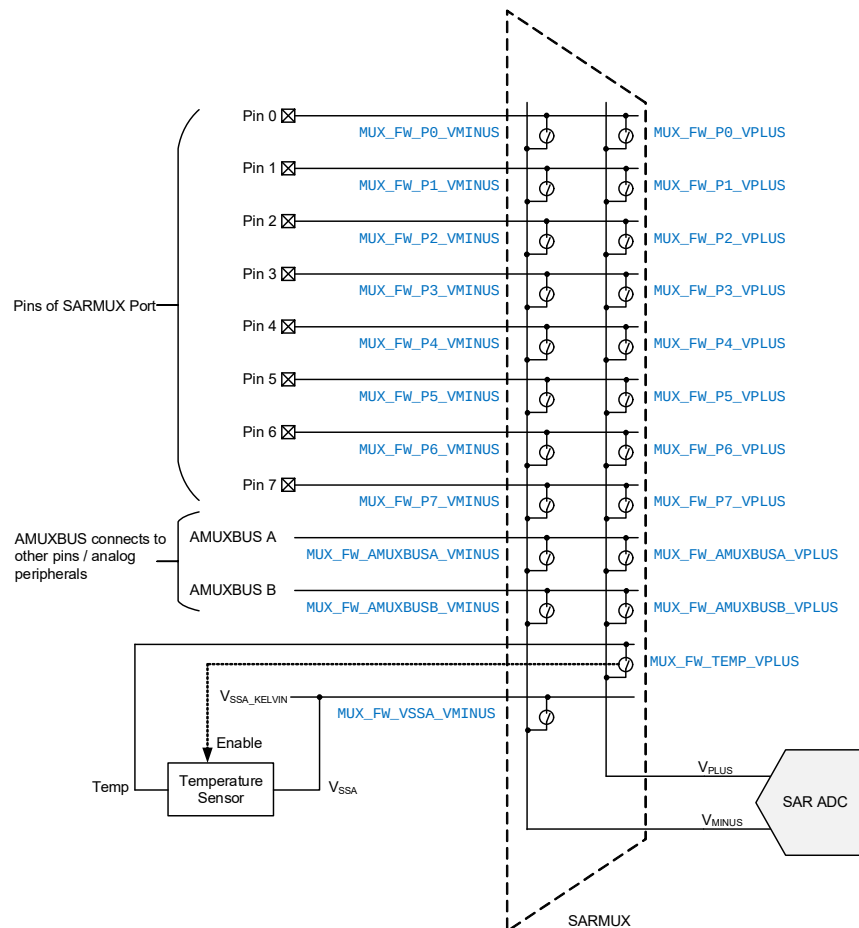
Figure 38-5. SARMUX Switches
