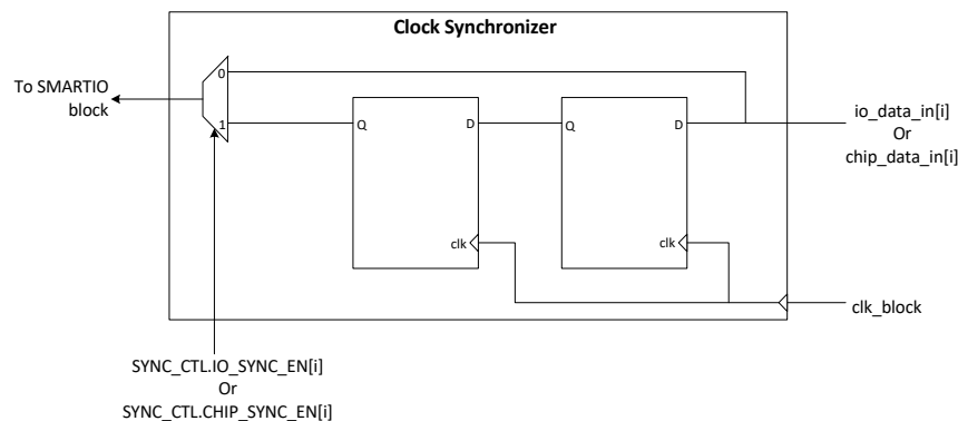
Figure 23-8. Smart I/O Clock Synchronizer
