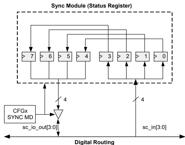
Figure 34-38. Sync Mode
