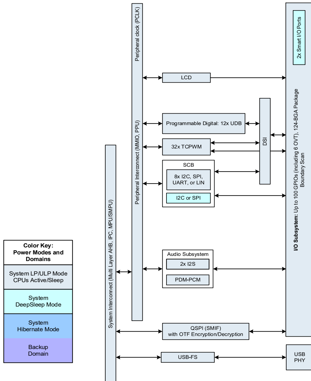
Figure D-1. Digital System Block Diagram
