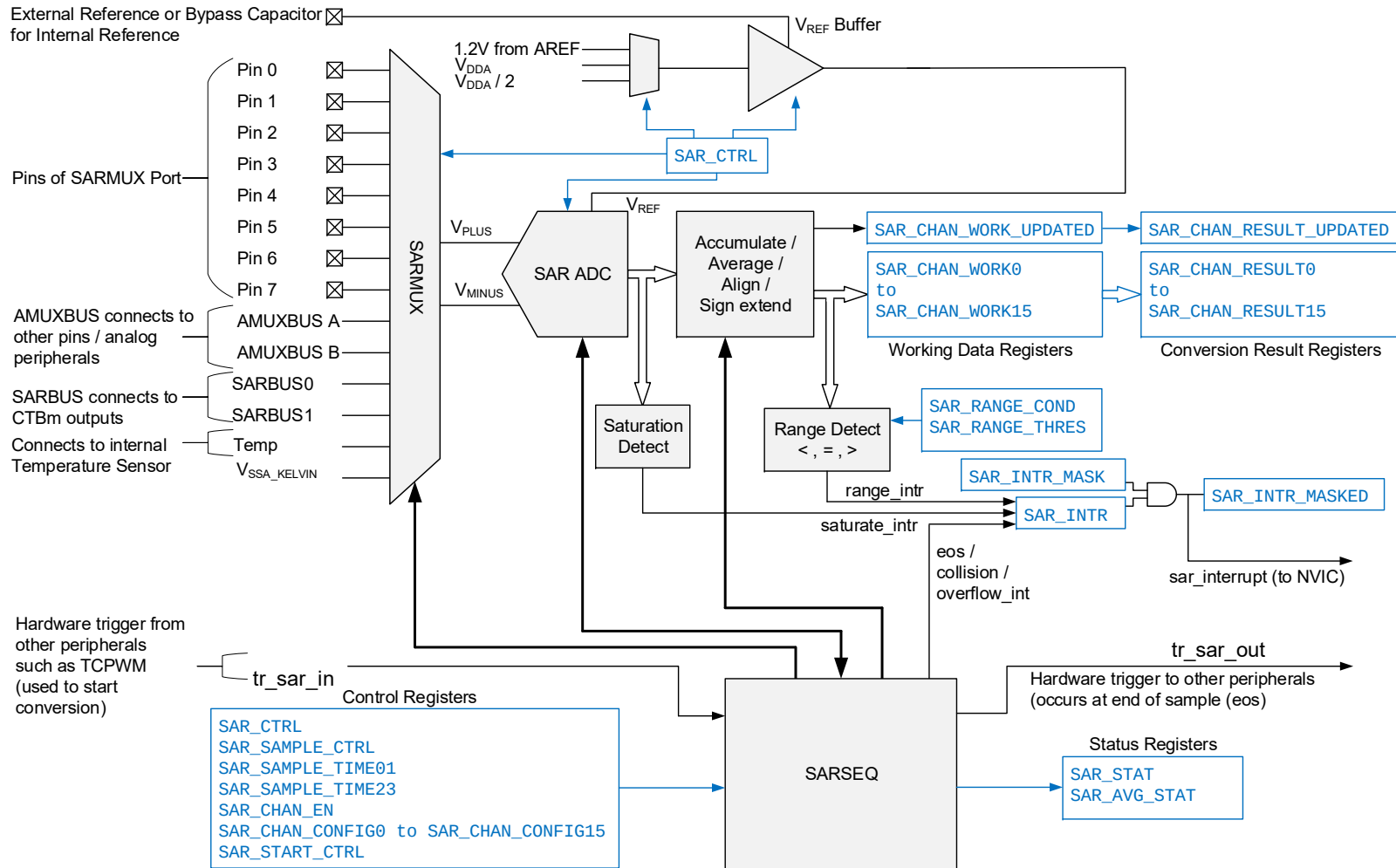
Figure 39-1. Block Diagram
