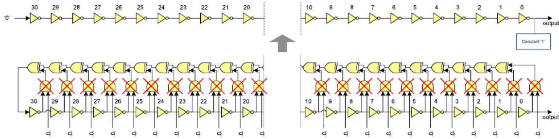
Figure 11-13. FIRO31 “stopped”
