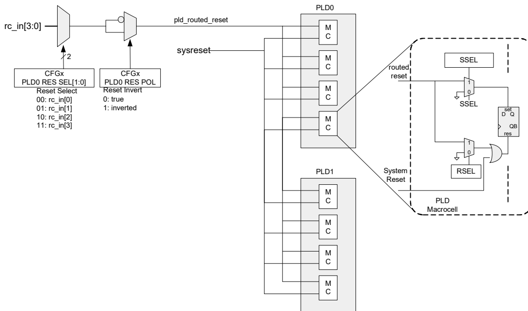
Figure 34-41. Compatible PLD Reset Structure
