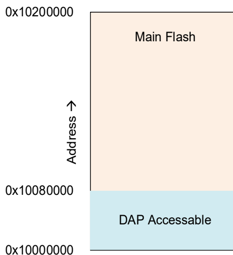
Figure 14-2. FLASH_ALLOWED with encoding “4”
