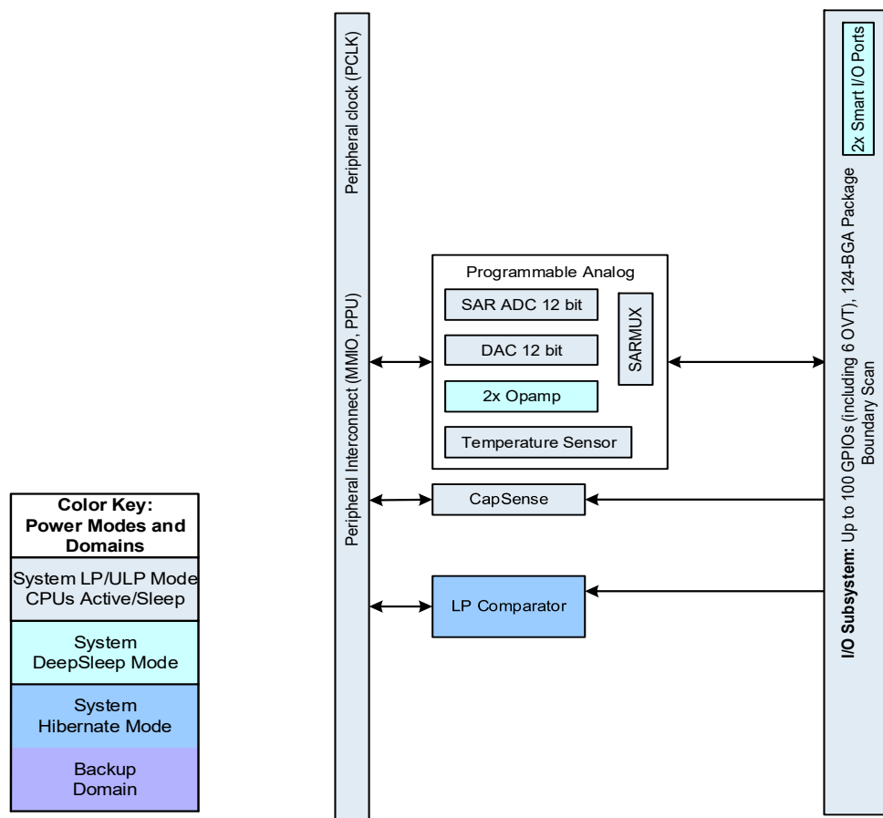
Figure E-1. Analog System Block Diagram
