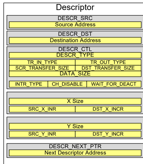
Figure 10-2. Descriptor Structure
