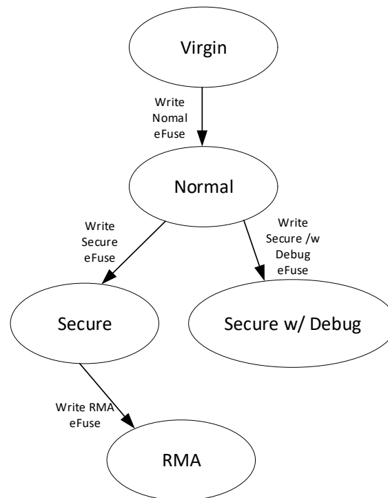
Figure 16-1. PSoC 6 MCU Life Cycle Stage Transitions
