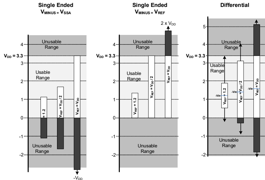
Figure 39-2. Input Range
