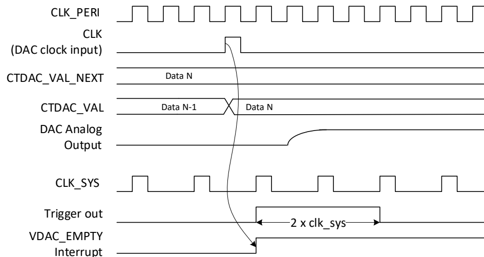
Figure 38-12. Buffered Write
