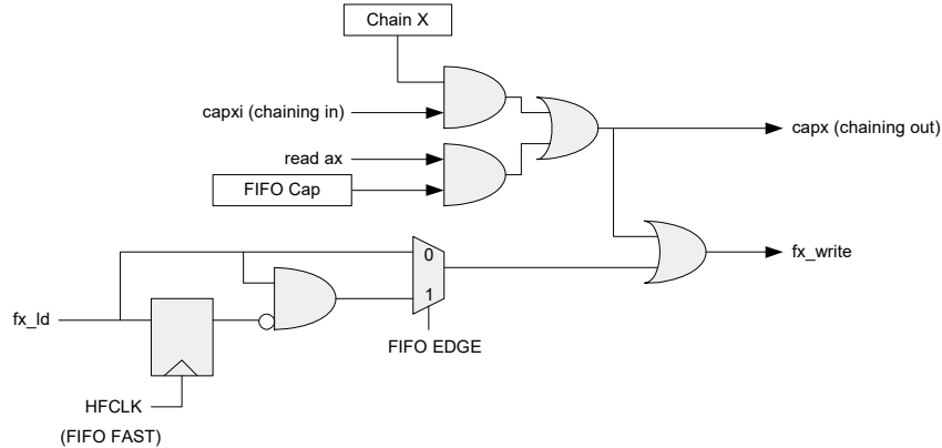
Figure 34-12. Software Capture Configuration
