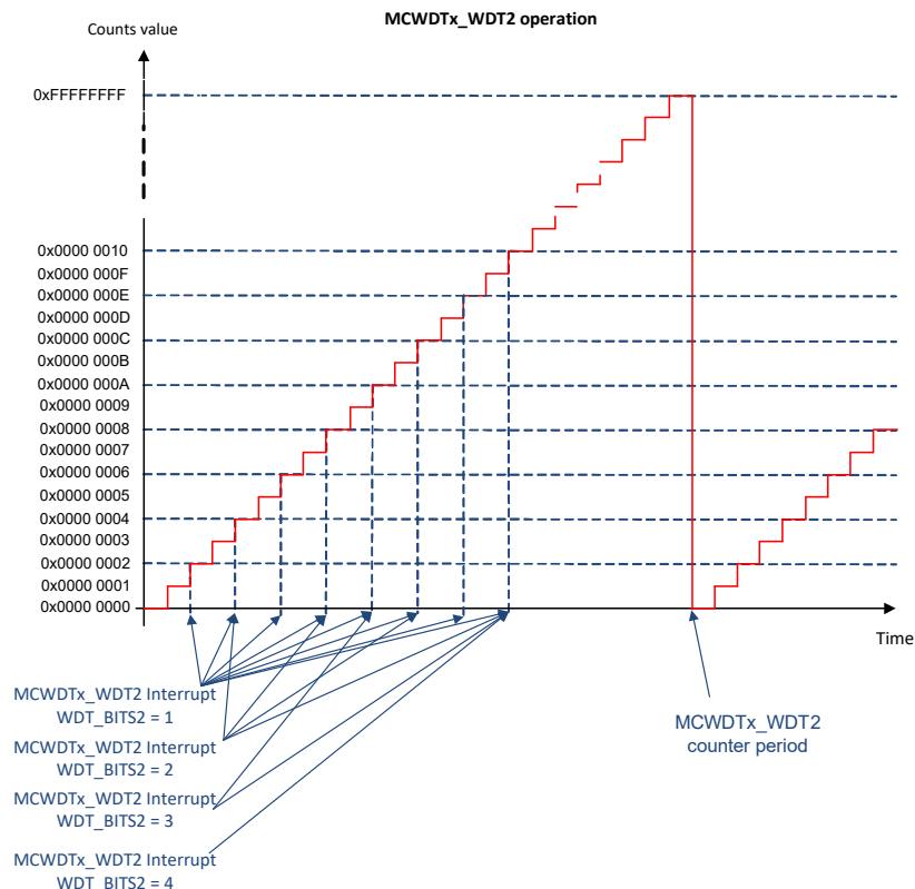
Figure 23-5. MCWDTx_WDT2 Operation
