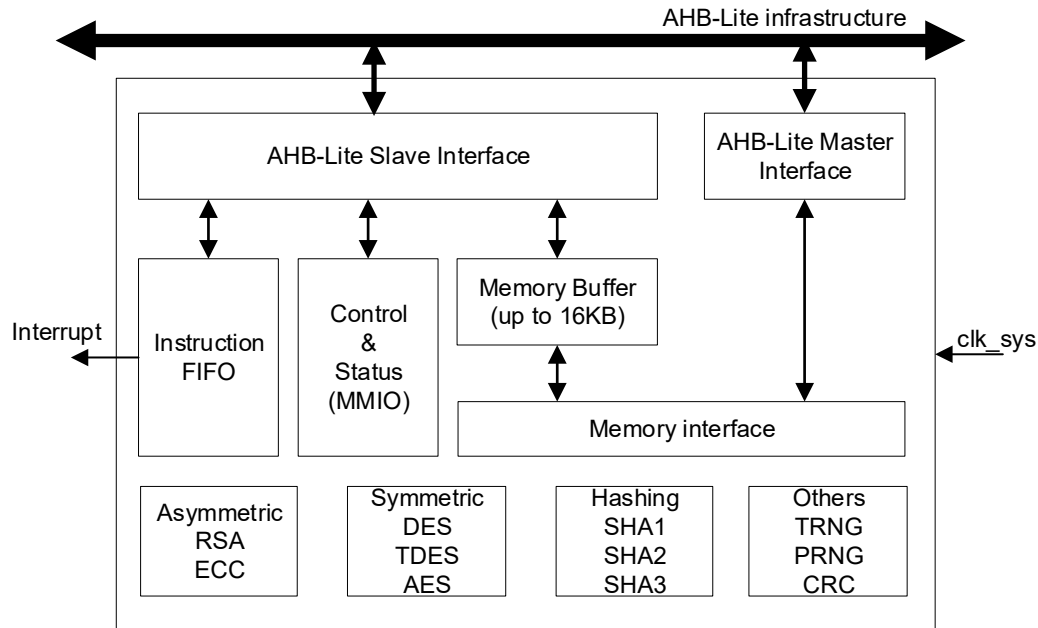
Figure 11-1. Crypto Block Diagram
