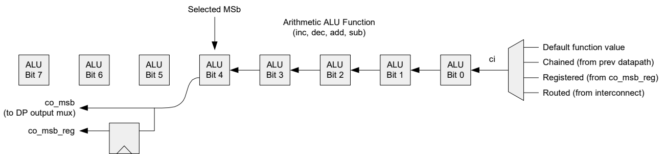
Figure 34-15. Carry Operation
