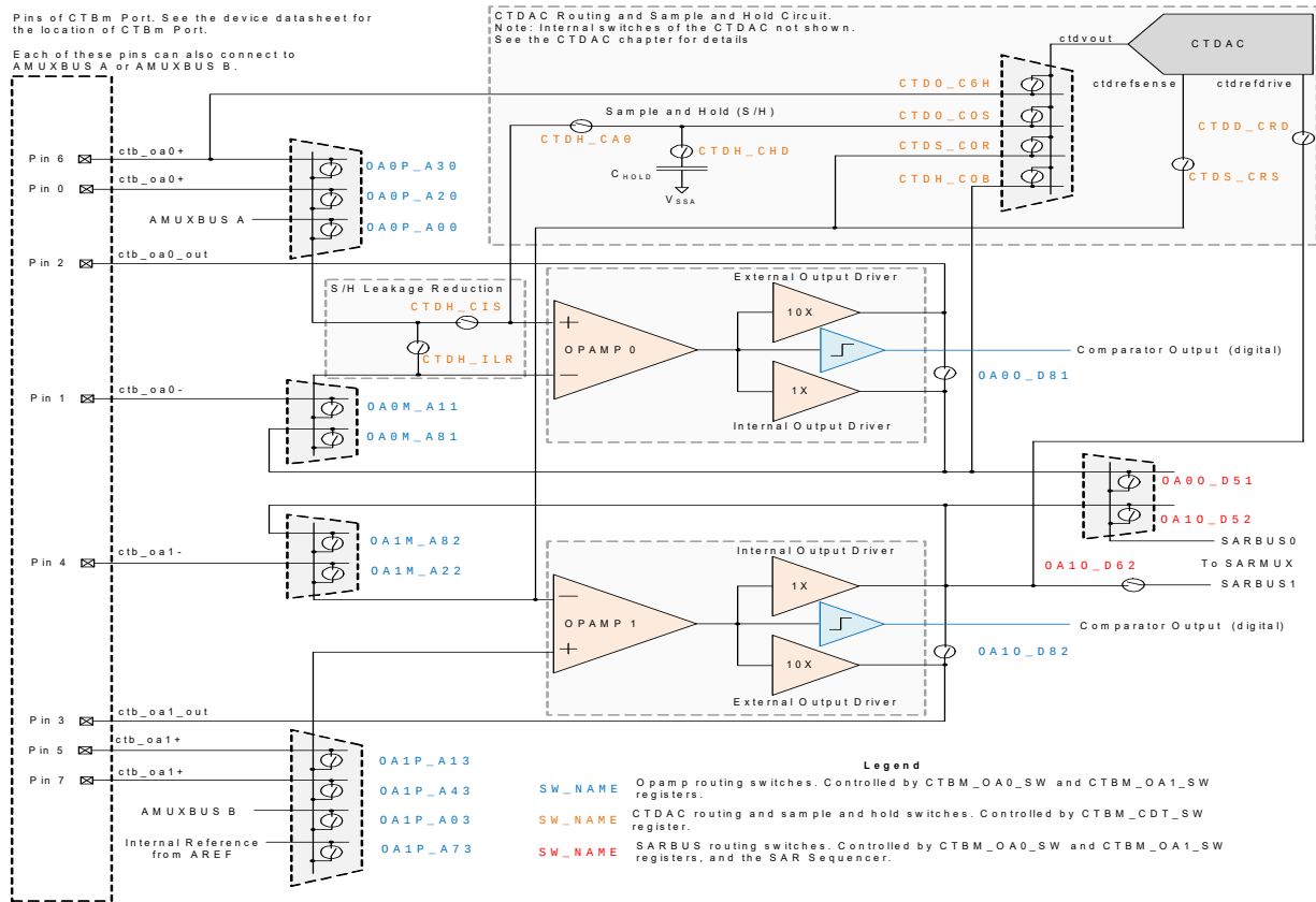
Figure 37-1. CTBm Block Diagram
