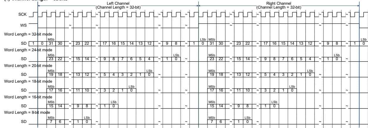
Figure 29-2. Standard I 2 S Format (Word Length and Channel Length Combination Timing Diagrams)
