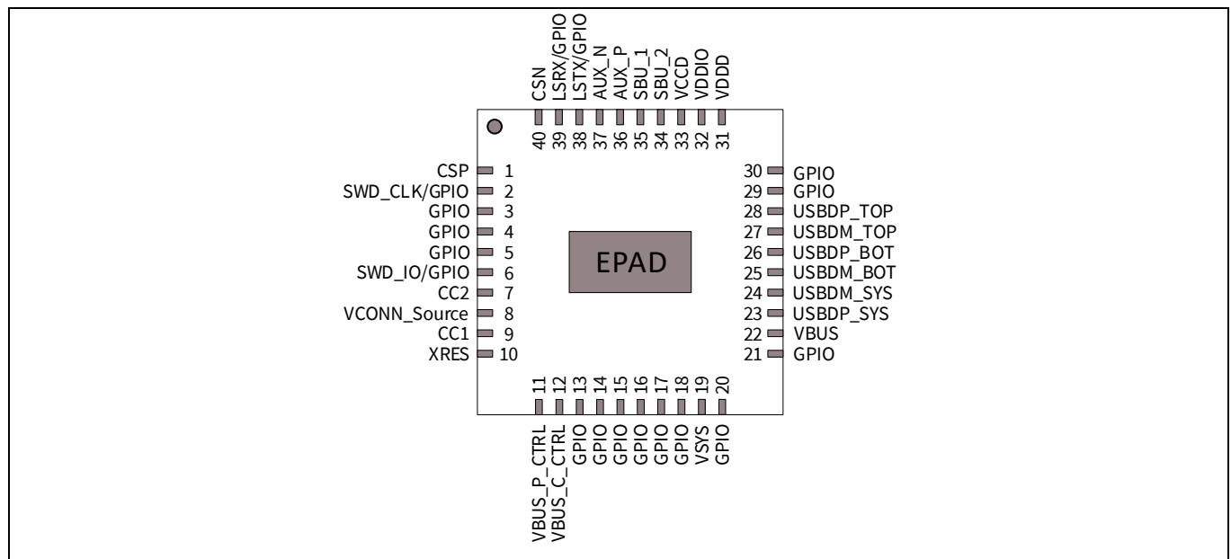
Figure 5 40-pin QFN pin map (top view) for CYPM1111-40LQXI
