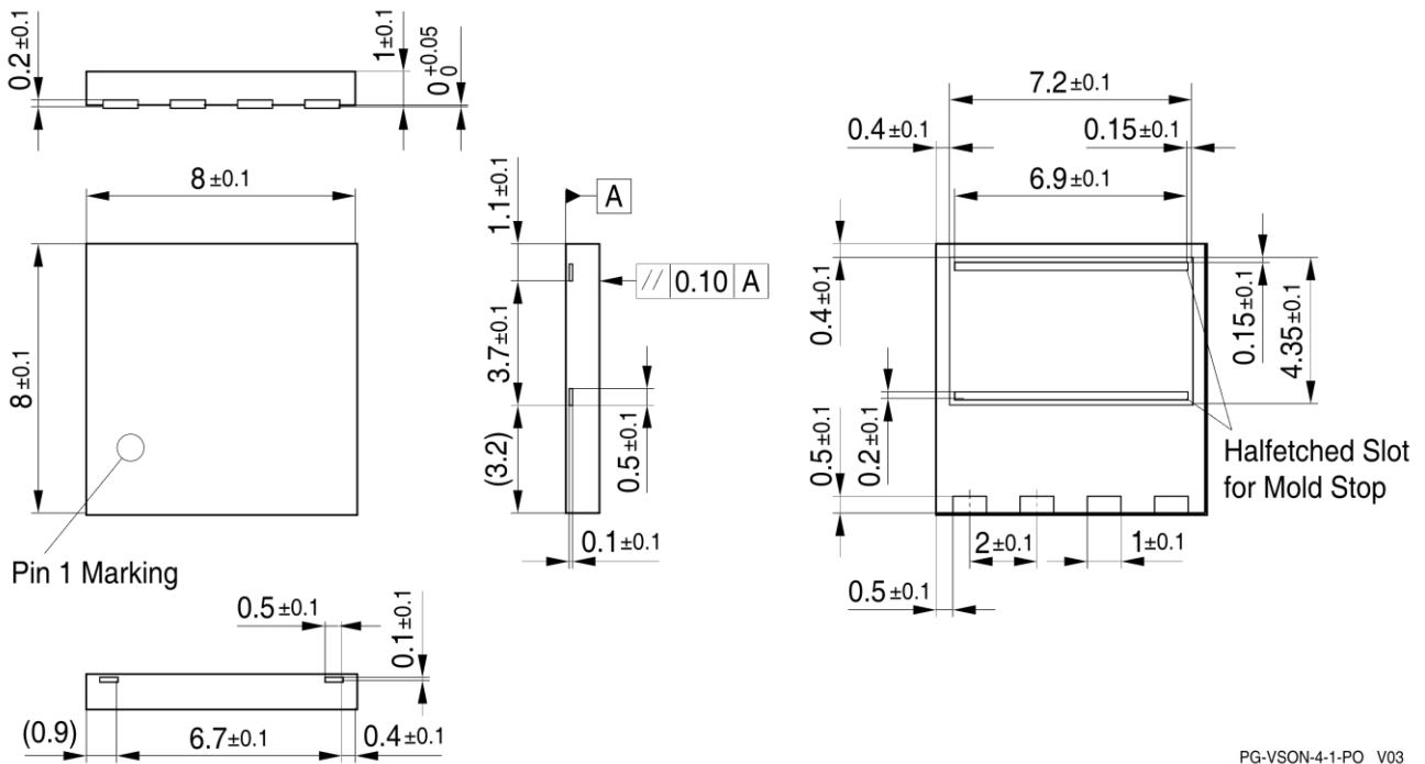
PG-VSON-4-1-PO V03
