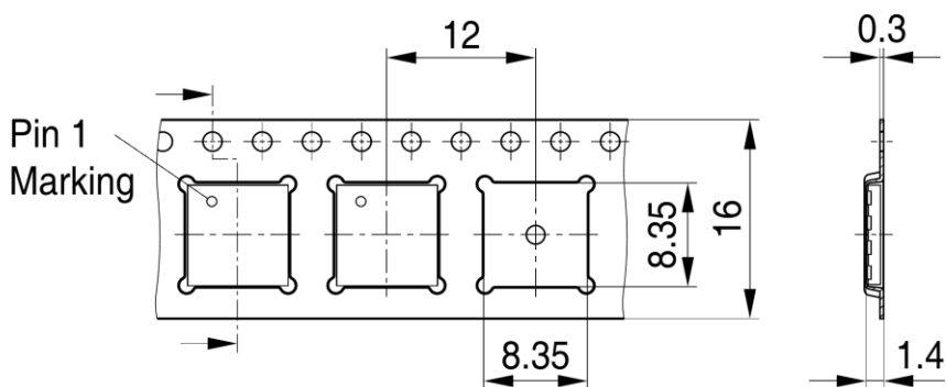
PG-VSON-4-1-TP V03
