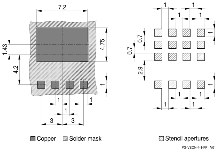
PG-VSON-4-1-FP V01
