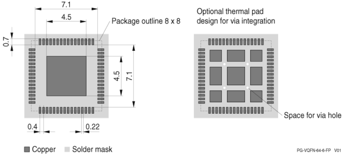
PG-VQFN-64-6-FP V01
