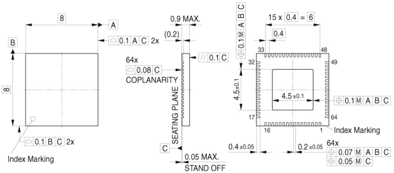
PG-VQFN-64-6-PO V04
