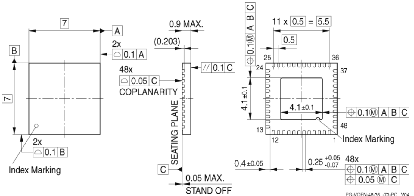
PG-VQFN-48-35, -73-PO V04
