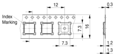
PG-VQFN-48-15, -19, -20, -22, -24, -48, -51, -52, -53, -54, -55, -56, -201, -202-TP V01
