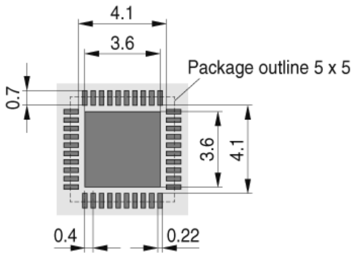
PG-VQFN-40-13, -14, -17-FP V01
