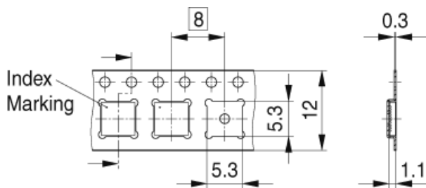
PG-VQFN-40-13, -14, -17-TP V01
