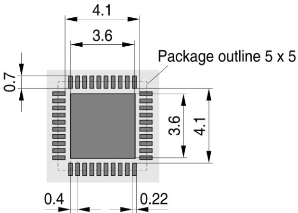
PG-VQFN-40-13, -14, -17-FP V01
