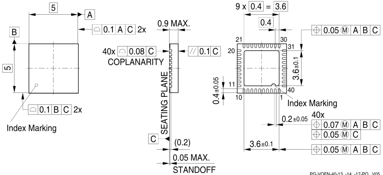
PG-VQFN-40-13, -14, -17-PO V05
