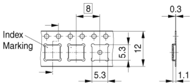
PG-VQFN-40-13, -14, -17-TP V01
