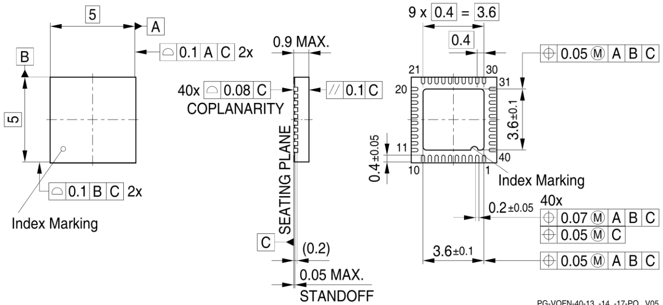
PG-VQFN-40-13, -14, -17-PO V05
