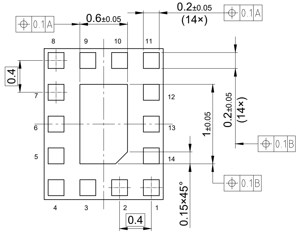
Bottom view
