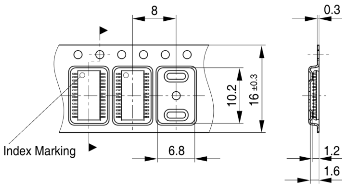
P/PG-TSSOP-28-9-TP V03
