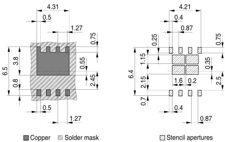
PG-TSON-8-2-FP V01
