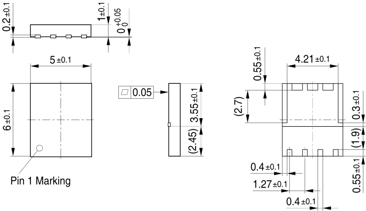
PG-TSON-8-2-PO V01
