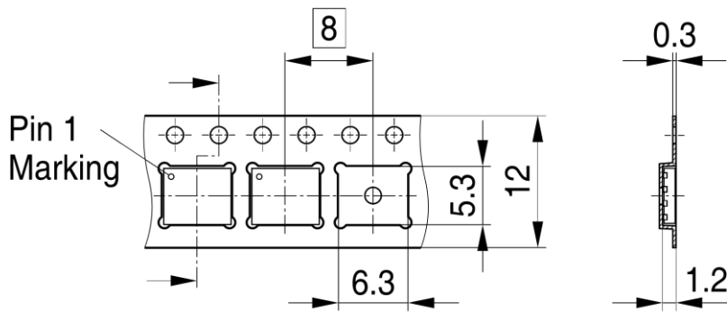
PG-TSON-8-2-TP V01
