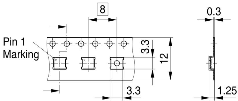
PG-TSON-8-1-TP V01
