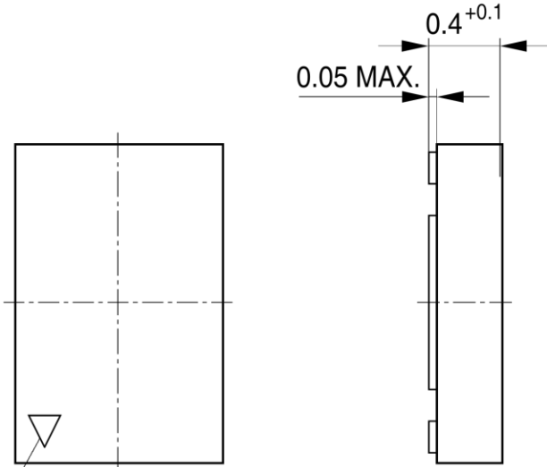
Pin 1 marking
