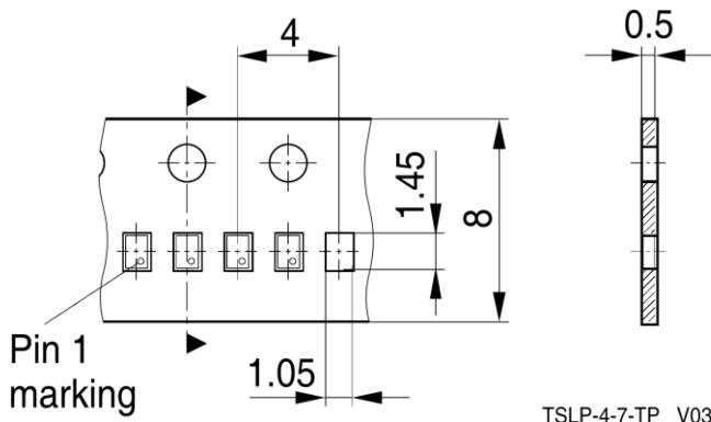
TSLP-4-7-TP V03
