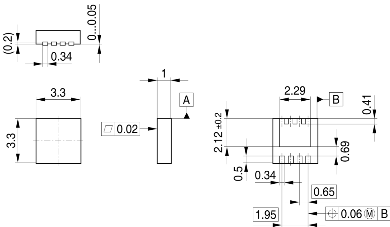
PG-TSDSON-8-1, -2-PO V02
