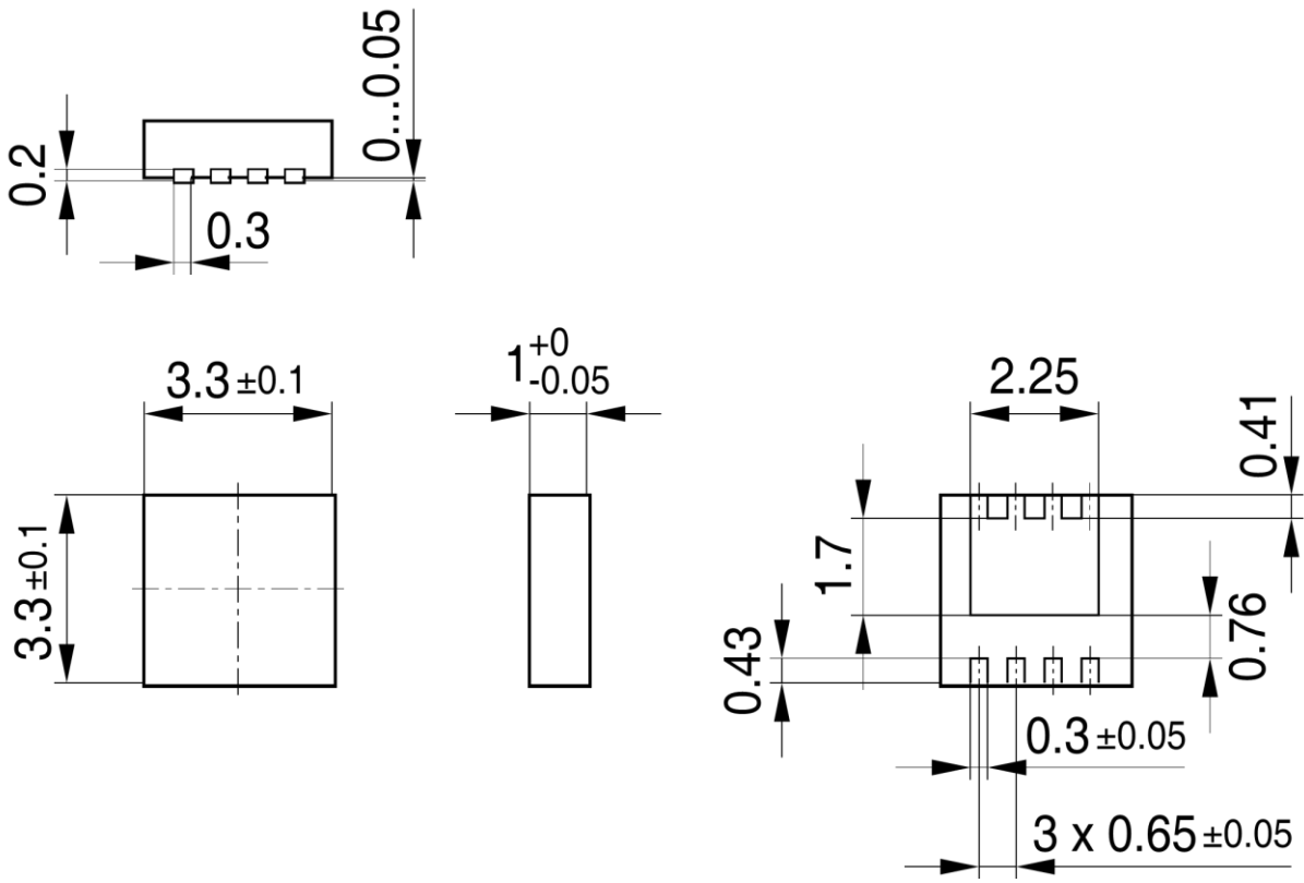
PG-TSDSON-8-21, -22-PO V02
