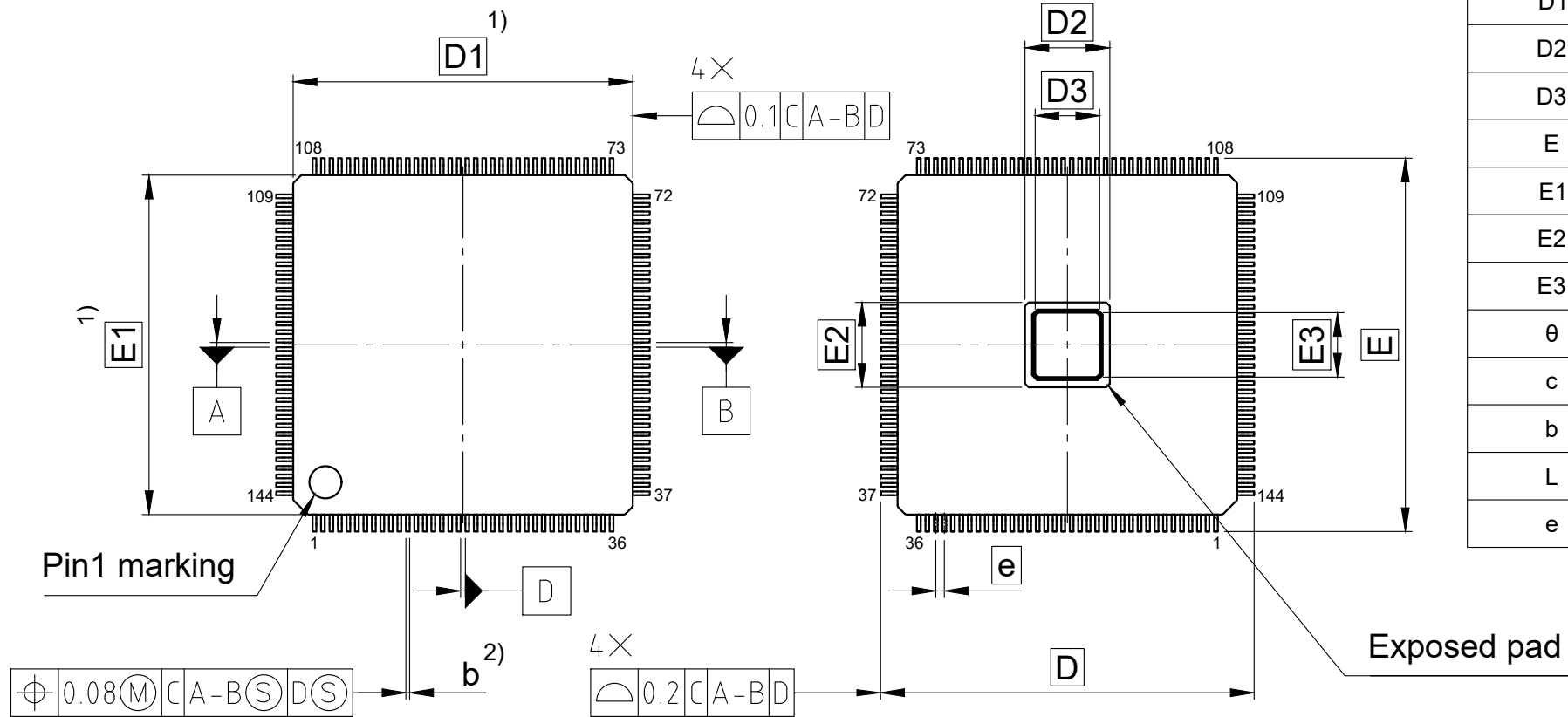
Bottom view
