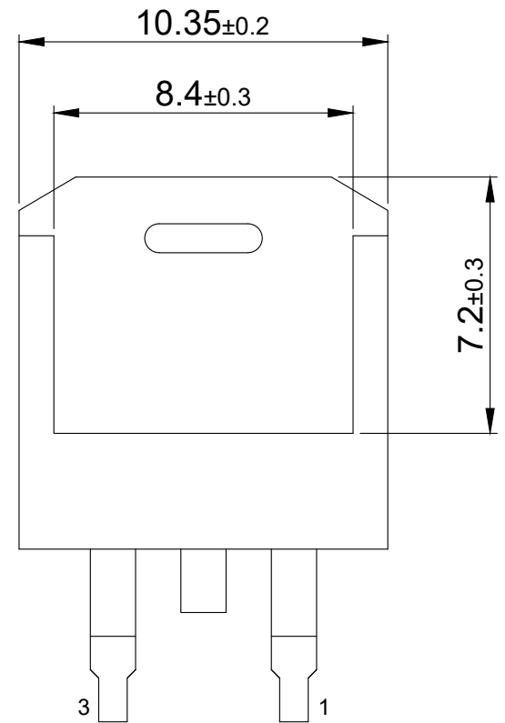
Bottom view
