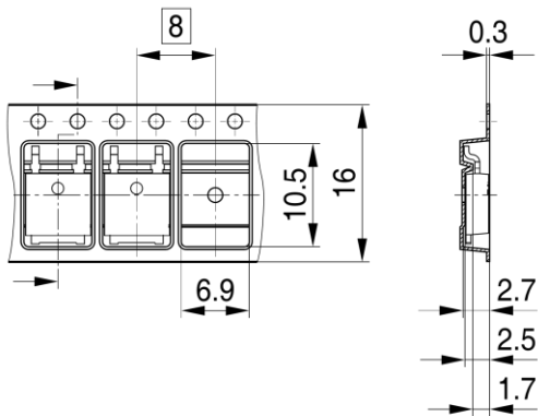
PG-TO252-2-1-TP V04
