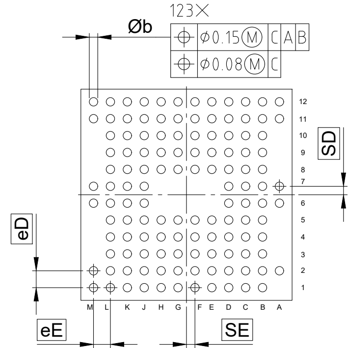
Bottom view
