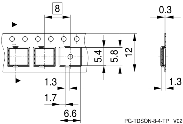
PG-TDSON-8-4-TP V02
